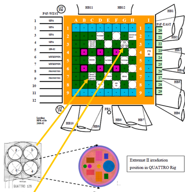
Fig. 1. Schematic representation of the location ExtreMat-II capsule in the HFR. The irradiation was carried out in leg 4 of a QUATTRO rig, positioned at C7.
