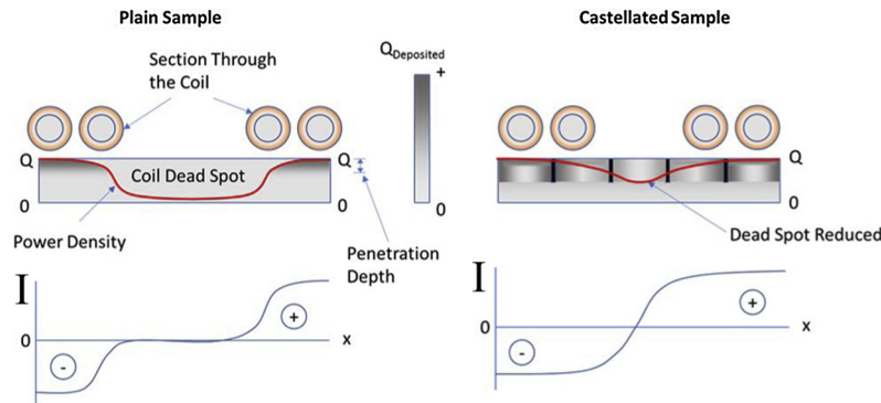
Fig. 1. Illustration of the End/Edge Effects & Coil ‘Dead-Spot’.
