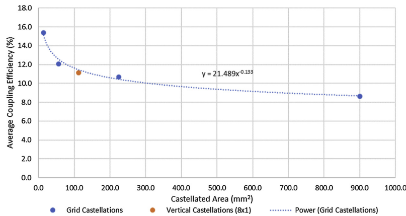
Fig. 5. Av. Coupling Efficiency Against Castellation Area.
