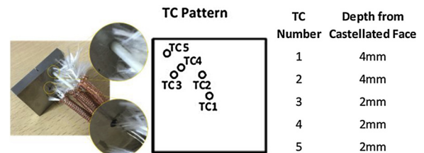
Fig. 3. Thermocouple Installation.
