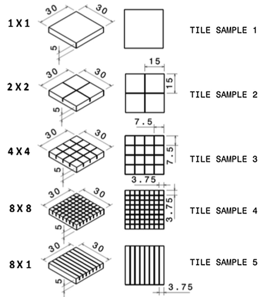
Fig. 2. The Five Tungsten Samples.
