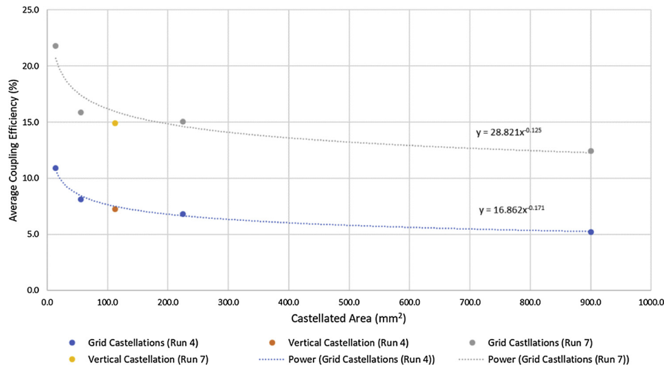
Fig. 6. Coupling Efficiency Against Castellation Area for 3 kW and 15 kW.
