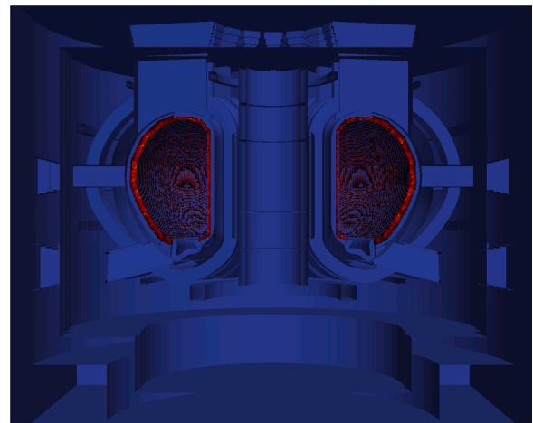
Fig. 3. The OpenMC neutronics model, showing the regions of tritium production in red. (For interpretation of the references to color in this figure legend, the reader is referred to the web version of this article).
