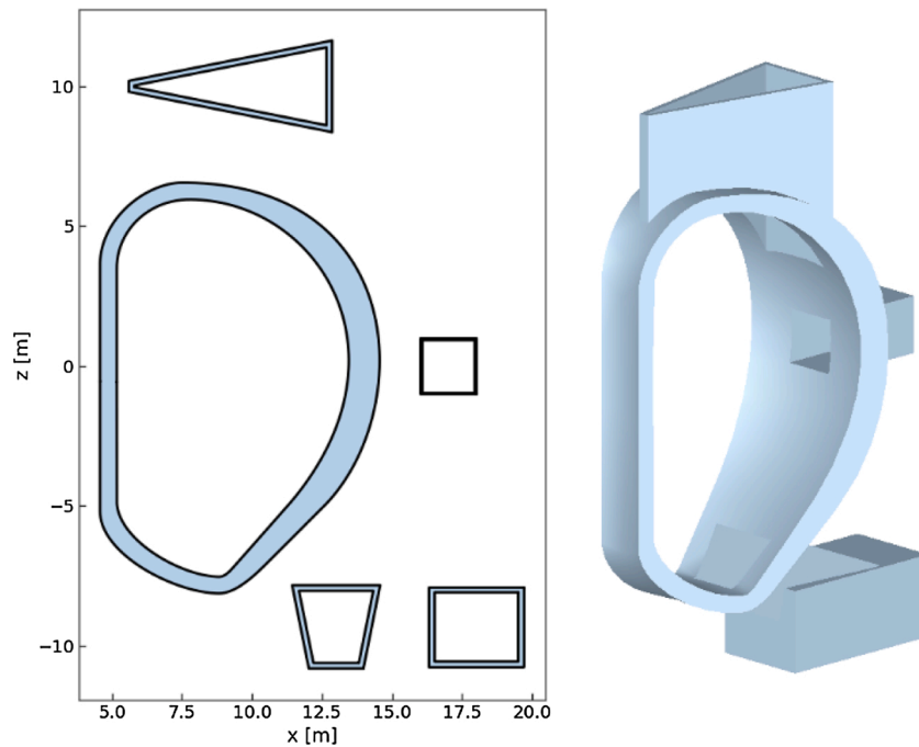
Fig. 2. (left) 2-D cross-sections of the vacuum vessel space reservation (right) the assembled CAD component. The main body is toroidally revolved about the machine axis, the port cross-sections are extruded into the main body, and Boolean cuts hollow out the penetrations into the main body.
