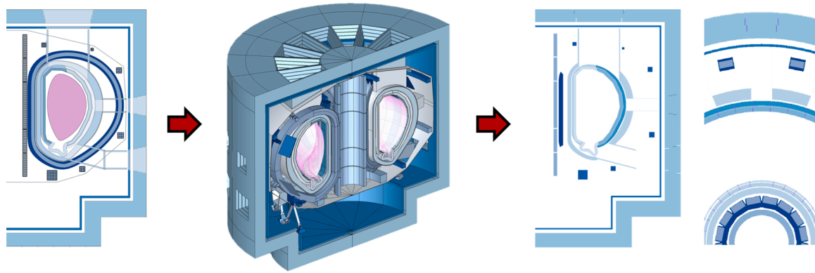
Fig. 1. The geometry creation procedure in BLUEPRINT, showing: (left) the 2-D reactor cross-section, (centre) the resulting 3-D CAD model, and (right) cropped views of the reactor cross-section and mid-plane plan in the radiation transport model.
