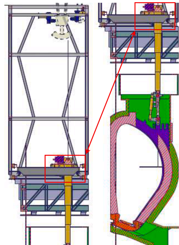
Fig. 12. End-effector mounted on a telescopic mast.
