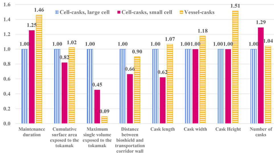
Fig. 20. Comparison of metrics for the large cell, small cell and the vessel cask approaches for the maintenance of the Lower Port.
