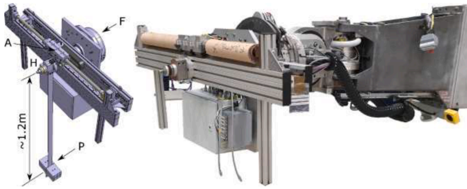
Fig. 29. Left: flexible pendulum model used to validate APCS; right: partial installation of flexible pendulum on TARM
