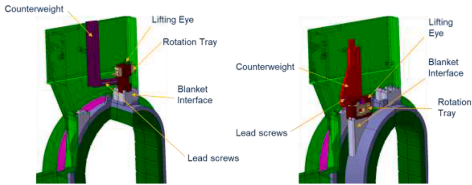
Fig. 10. Crane-lifted counterbalance concepts
