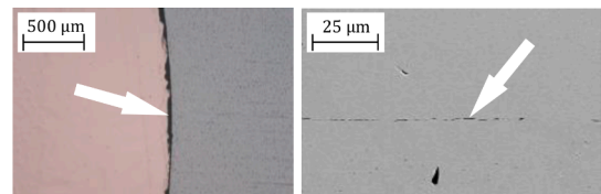
Fig. 4. A micrographic view of the Cu/W interface (left) and an SEM view of the CuCrZr/Cu interface (right) of the sectioned 825 °C diffusion bond sample. Voids are indicated by the white arrows.
