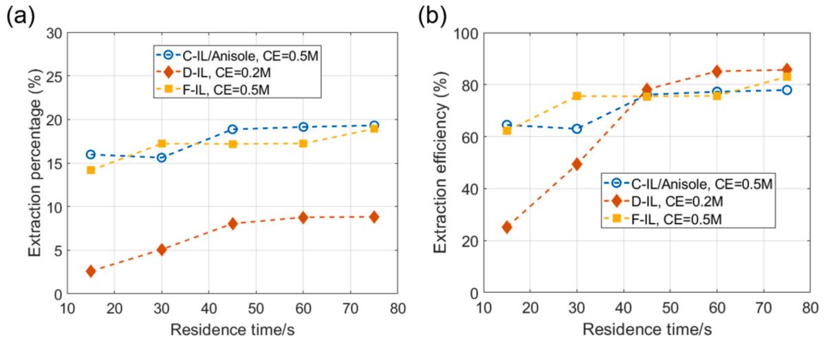
Fig. 7. (a) Extraction percentage of lithium ions in microfluidic channels at different residence times. (b) Extraction efficiency of lithium ions in microfluidic channels at different residence times.
