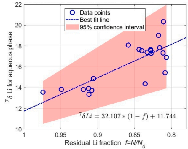
Fig. 8. Li isotope separation factor determined in microfluidic channels.
