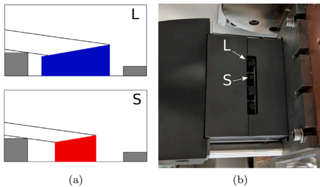
Fig. 1. (a) Probe cross sections showing the geometric area projected along the magnetic field lines for the L and S probes. (b) Photograph showing the DSF probe array installed in Magnum-PSI with the S and L probes labelled.
