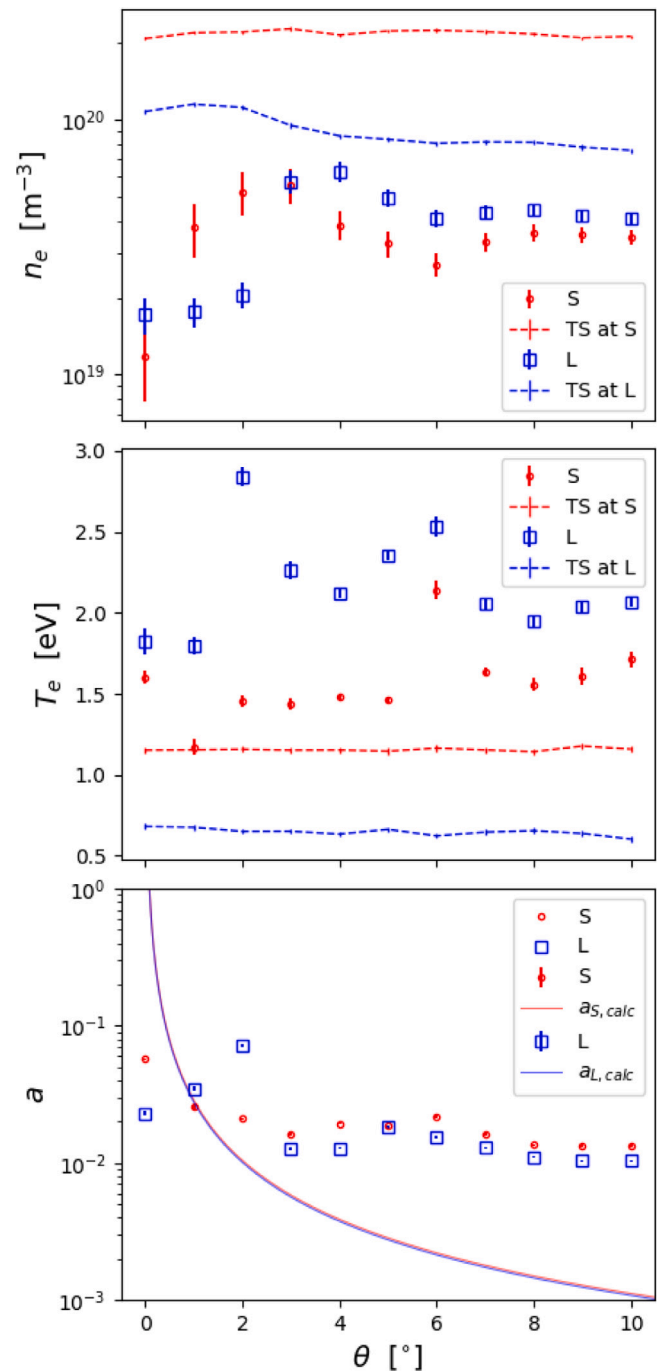
Fig. 5. The measured plasma parameters at each value of \theta for the 0.8T hydrogen plasma. T_e is temperature, n_e is electron density, and a is the sheath expansion parameter as per Eq. (1). The interpolated TS values at each probe’s approximate radial position are overlaid for n_e . Bergmann’s analytical model for sheath expansion (see Eq. (2)), calculated as a function of \theta and using the mean TS T_e and n_e for each probe, is overlaid on the sheath expansion plot.
