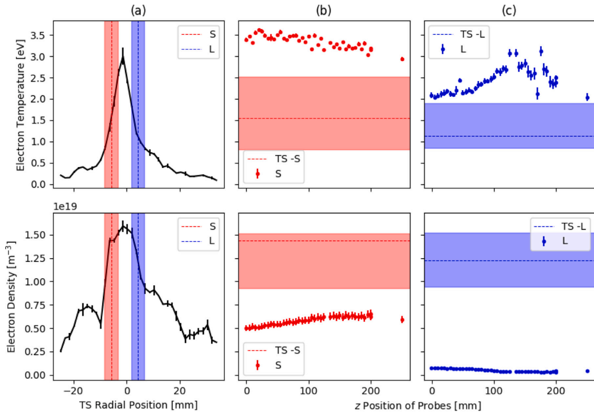
Fig. 6. Results of the axial-scan, i.e. the probe measurements taken along the Magnum-PSI beam axis. The top and bottom rows show T_e and n_e respectively, with (a) being TS profiles, (b) and (c) being the fit parameters from the S and L probes' IVs respectively. The dotted lines and associated bounds indicate the interpolated TS measurement at the position of the S (red) and L (blue) probes and the corresponding uncertainty. The different probe measurements show axial density and temperature profiles with opposite trends, implying that the probes are translating through the radial beam profile with increased z .
