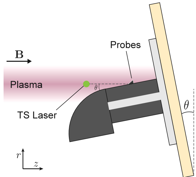
Fig. 2. Experimental setup diagram showing relative location of probes and TS laser, and \theta as the magnetic field incidence angle. r and z correspond to the radial and axial coordinates used throughout.
