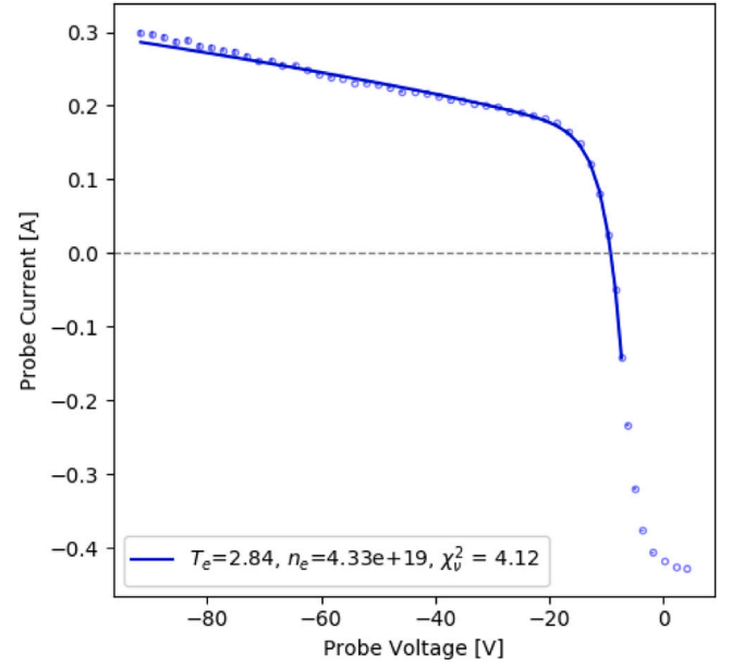
Fig. 4. An example IV characteristic (L probe, \theta = 2^\circ ) with Bergmann's 4-parameter model overlaid. The fit was achieved using the 3-stage method developed on MAST.
