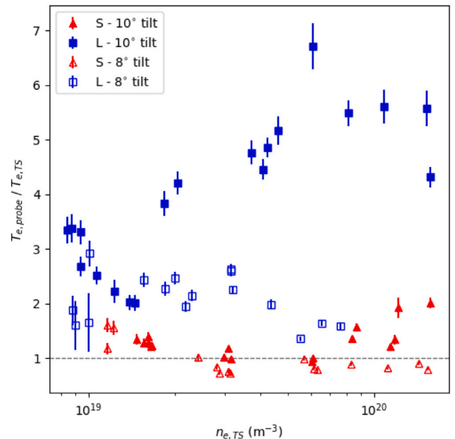
Fig. 7. The temperature overestimation factor plotted as a function of TS density at probe radial position, for the S (triangles) and L (squares) probes at \theta = 8^\circ (empty) and \theta = 10^\circ (filled). The shots at \theta = 10 on both probes show increasing overestimation of temperature at high densities.
