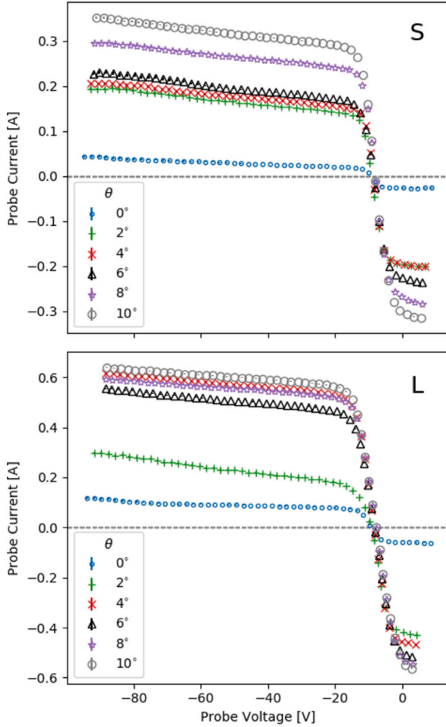
Fig. 3. Results of the scan over magnetic field incidence angle for the 0.8T hydrogen plasma. The IV characteristics for the S and the L probe are featured on the top and bottom respectively.
