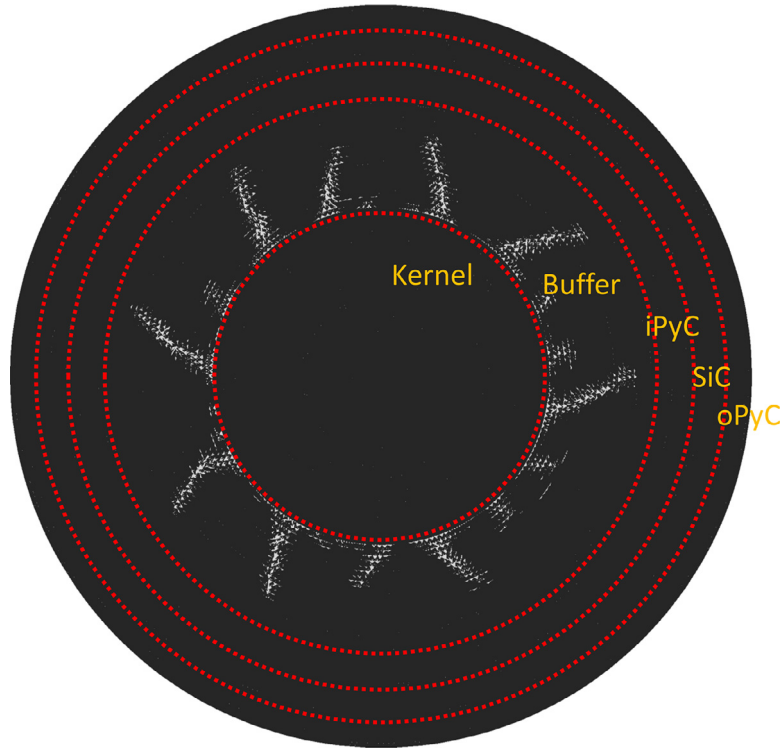
Fig. 6. Fracture patterns in the TRISO particle at the end of the rise to 100% power over 24 h. Red lines define the layer boundaries and white denotes bond failure, a surrogate for damage / cracking.
