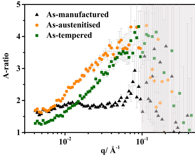
Fig. 9. Plots of A-ratio vs. q as calculated from the SANS data presented in Fig. 7a–c for all three sample conditions.
