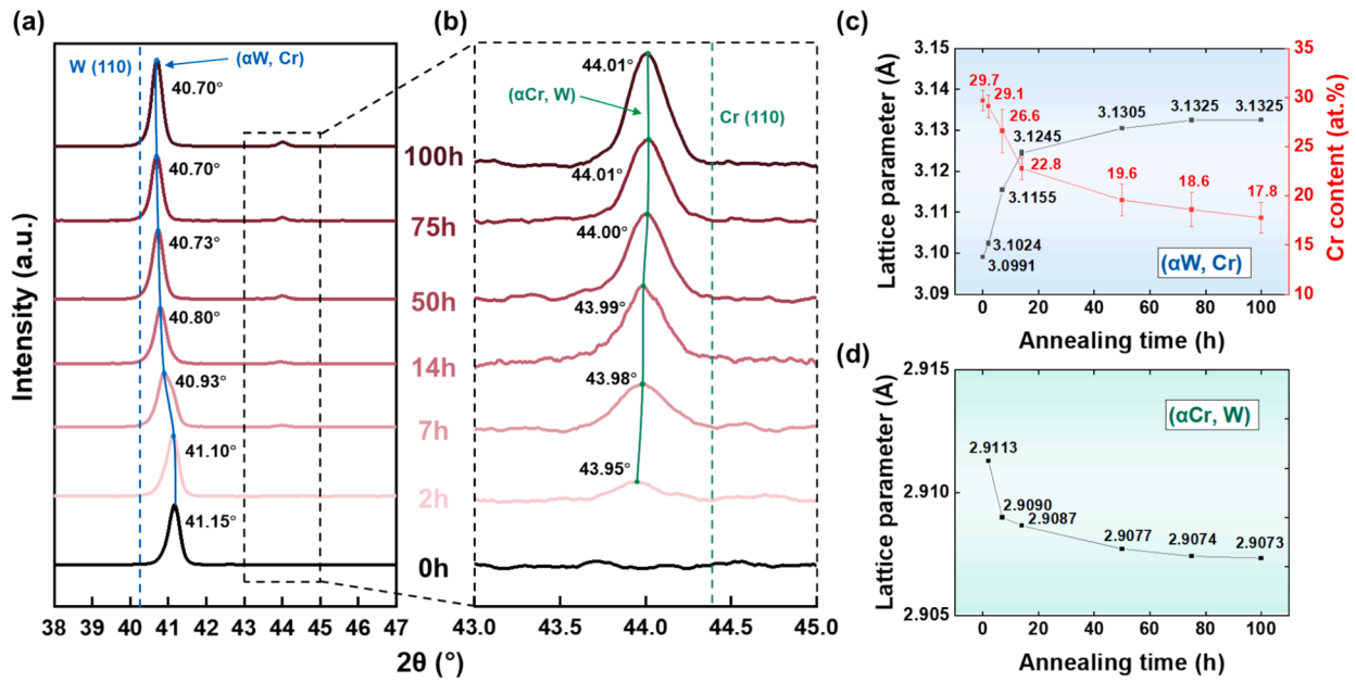
Fig. 4. (1 1 0) peak positions in XRD spectra of (a) (αW, Cr) and (b) (αCr, W) at different annealing times. Both phases have a BCC structure. Lattice parameters and Cr contents of (c) (αW, Cr) phases and (d) lattice parameters of (αCr, W) phases at different annealing stages. Lattice parameters of (αW, Cr) were calculated based on (1 1 0), (2 0 0), (2 1 1) peaks while those of (αCr, W) were calculate only using (1 1 0) peaks, the only visible peaks with weak intensity in XRD spectra. The Cr content of (αW, Cr) in (c) is measured by EDS.
