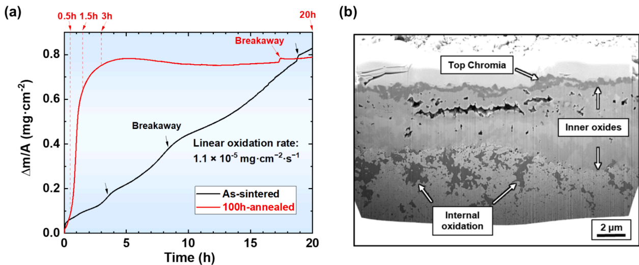
Fig. 8. (a) Specific mass change of the as-sintered and 100 h-annealed material during 20 h' oxidation, which shows different kinetics in the process but lands at the close values ( \sim 0.8 \text{ mg} \cdot \text{cm}^{-2} ) at 20 h. (b) cross sectional microstructure of the as-sintered material after 20 h oxidation.
