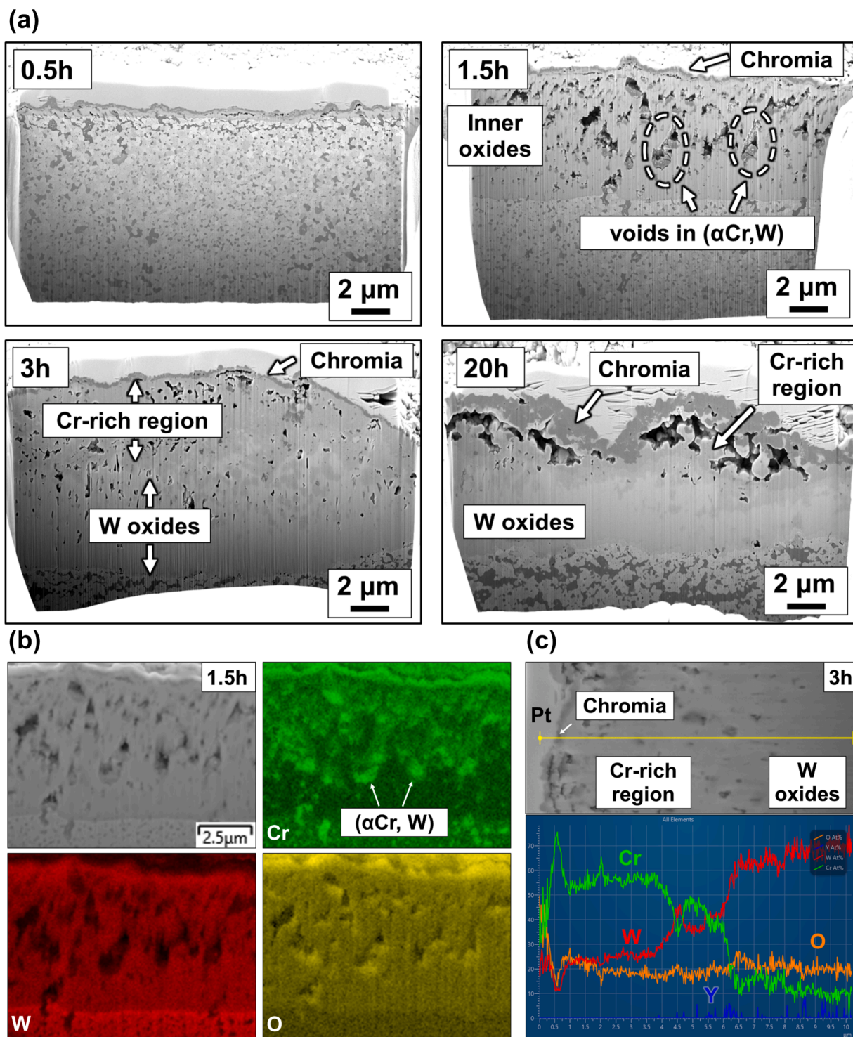
Fig. 10. (a) Cross section views of microstructural evolution at different oxidation stages of the 100 h-annealed material. (b) EDS mapping of the cross section at 1.5 h. ( \alpha Cr, W) is present in the inner oxide layer. (c) EDS line scan of the cross section at 3 h, from top (left) to bottom (right). The variation in elemental concentrations shows a Cr-rich region in the upper area of the inner oxide layer.
