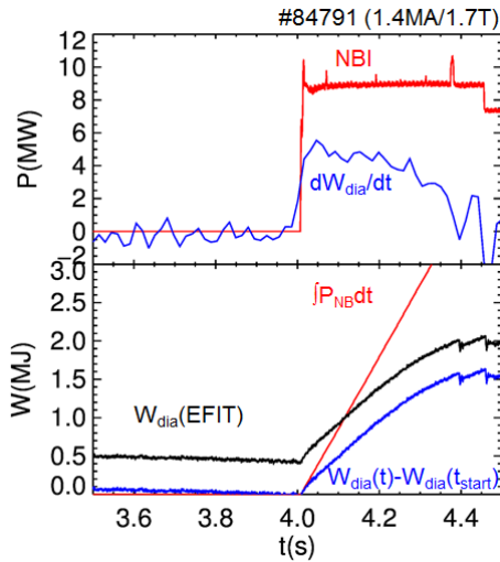
Figure 2: Transient plasma stored energy compared with neutral beam power (first pane) and stored energy compared with integral of neutral beam power (second pane).
