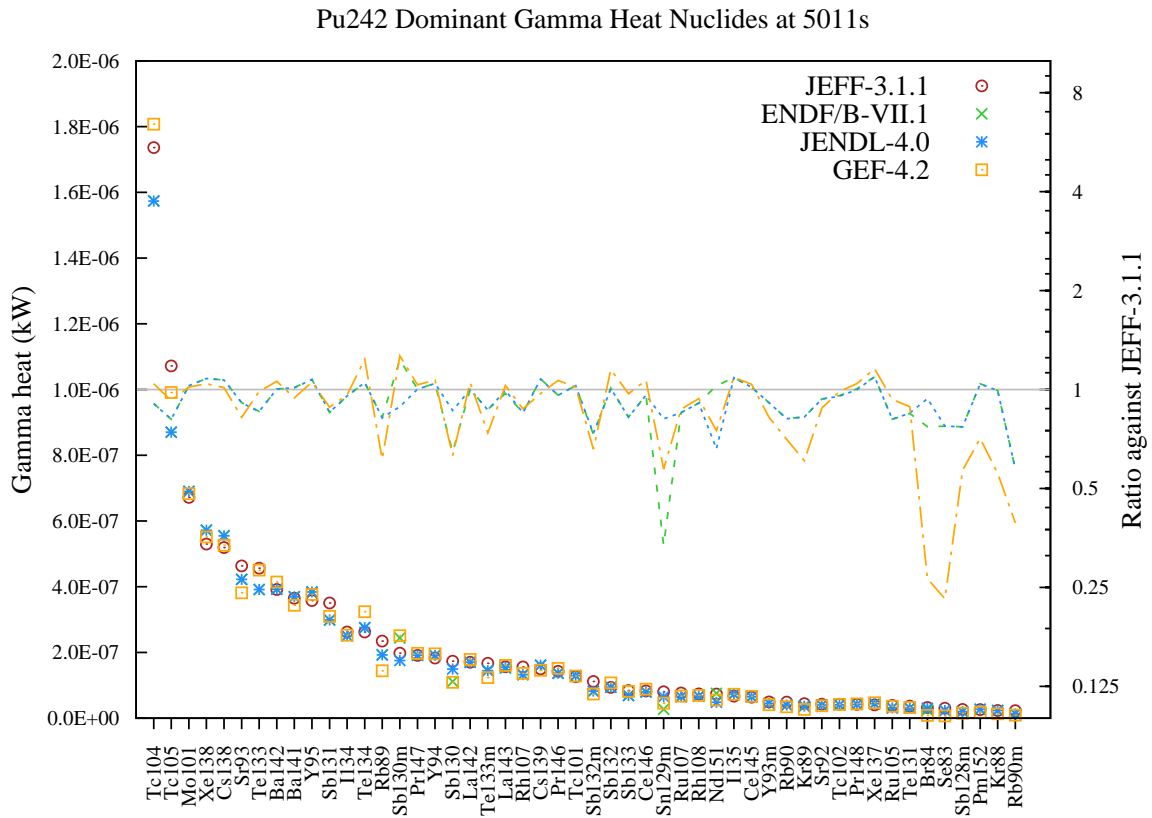
Figure 145: Gamma decay heat (in kW) fission yield comparison for Pu242 fission pulse after 5011s cooling.
