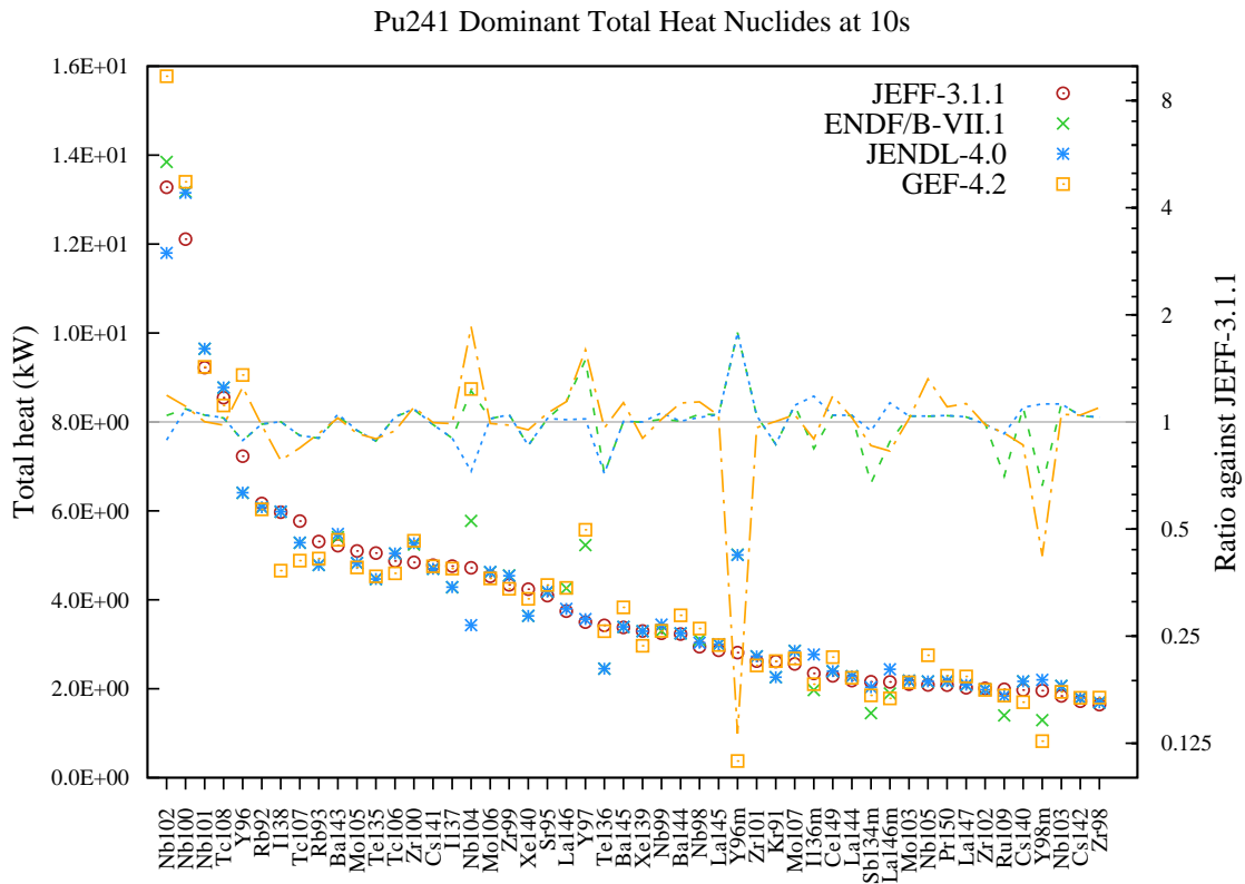
Figure 123: Total decay heat (in kW) fission yield comparison for Pu241 fission pulse after 10s cooling.
