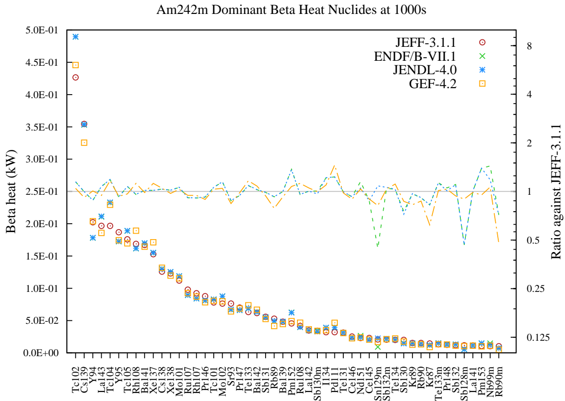
Figure 173: Beta decay heat (in kW) fission yield comparison for Am242m fission pulse after 1000s cooling.
