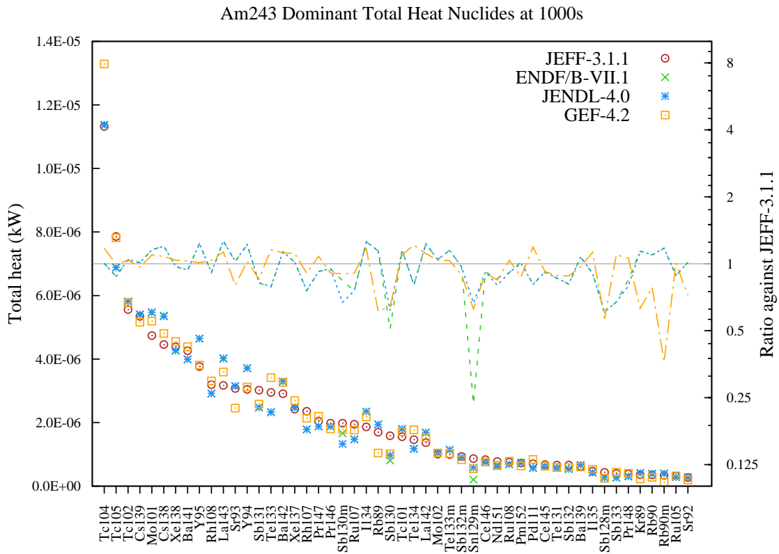
Figure 189: Total decay heat (in kW) fission yield comparison for Am243 fission pulse after 1000s cooling.
