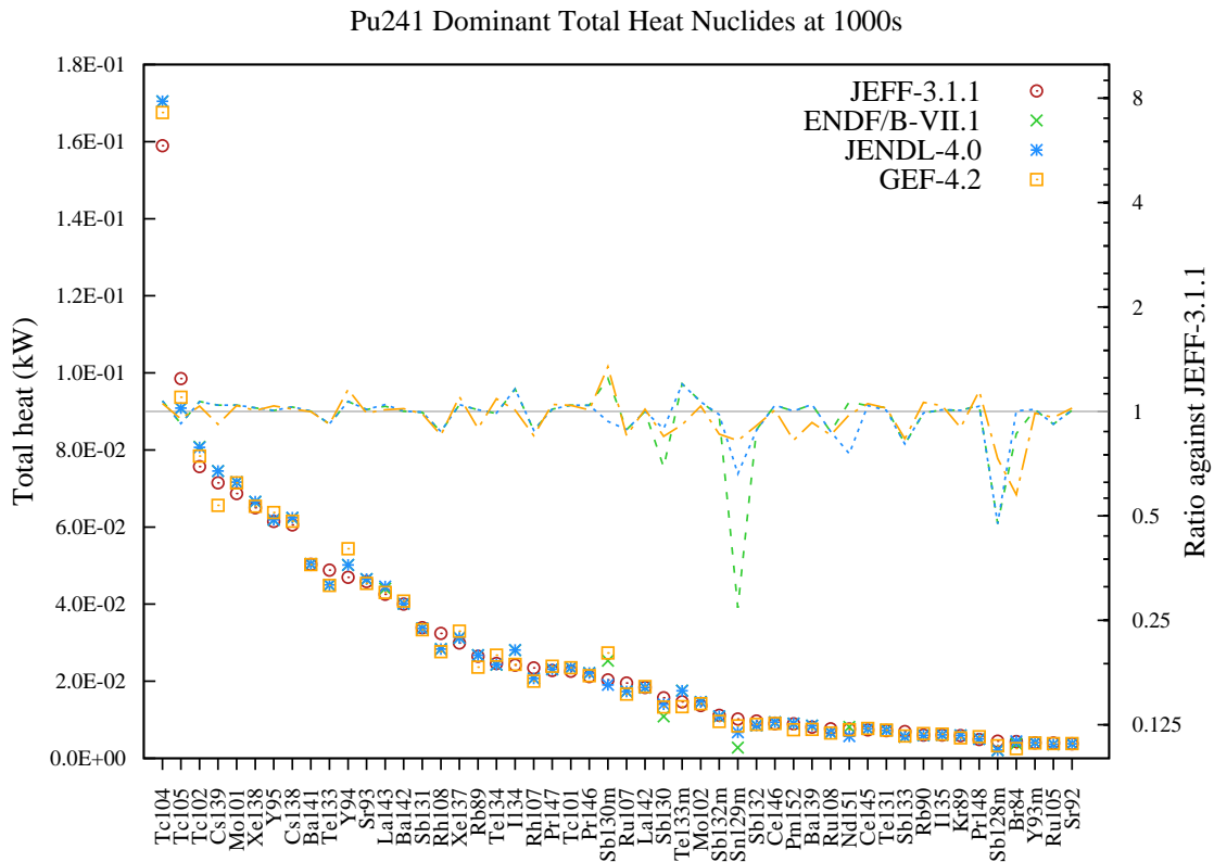
Figure 129: Total decay heat (in kW) fission yield comparison for Pu241 fission pulse after 1000s cooling.
