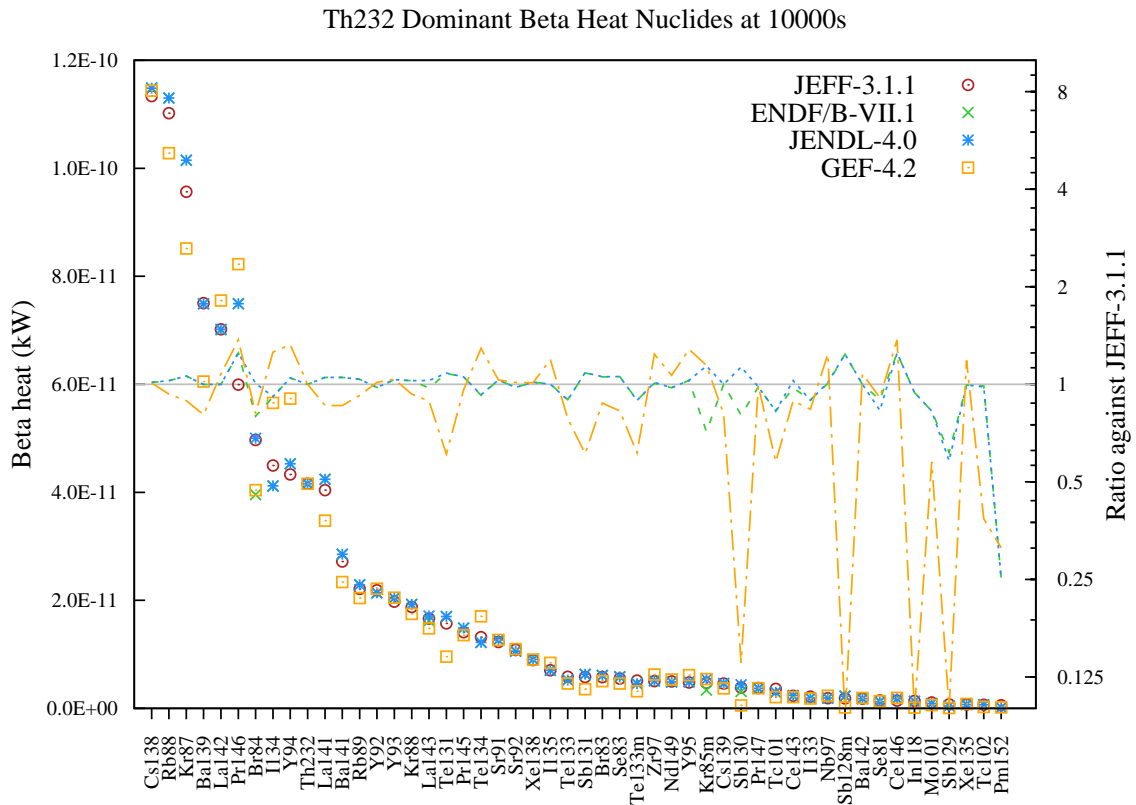
Figure 14: Beta decay heat (in kW) fission yield comparison for Th232 fission pulse after 10000s cooling.
