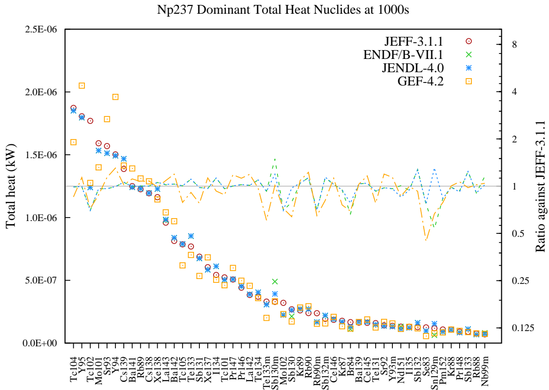
Figure 69: Total decay heat (in kW) fission yield comparison for Np237 fission pulse after 1000s cooling.
