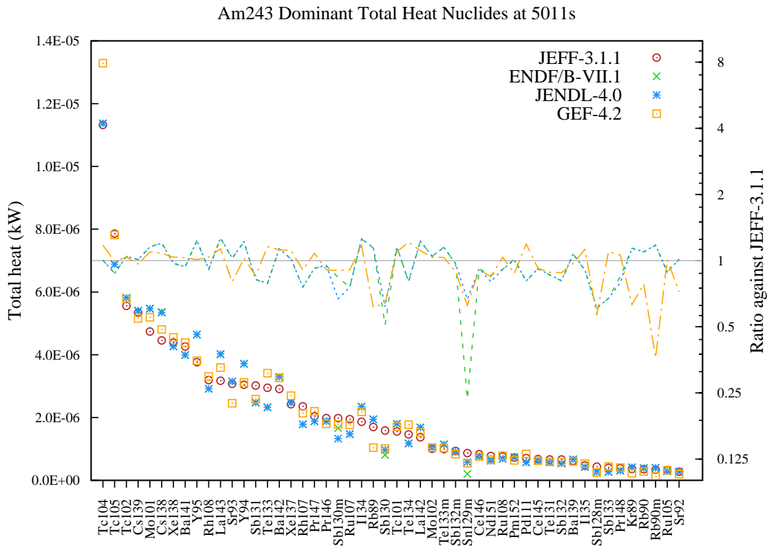
Figure 192: Total decay heat (in kW) fission yield comparison for Am243 fission pulse after 5011s cooling.
