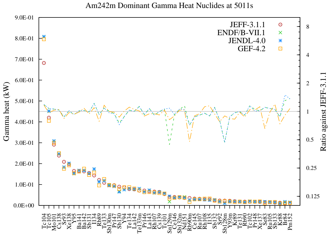
Figure 175: Gamma decay heat (in kW) fission yield comparison for Am242m fission pulse after 5011s cooling.
