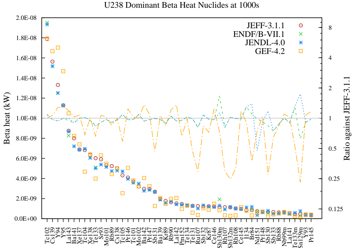
Figure 53: Beta decay heat (in kW) fission yield comparison for U238 fission pulse after 1000s cooling.
