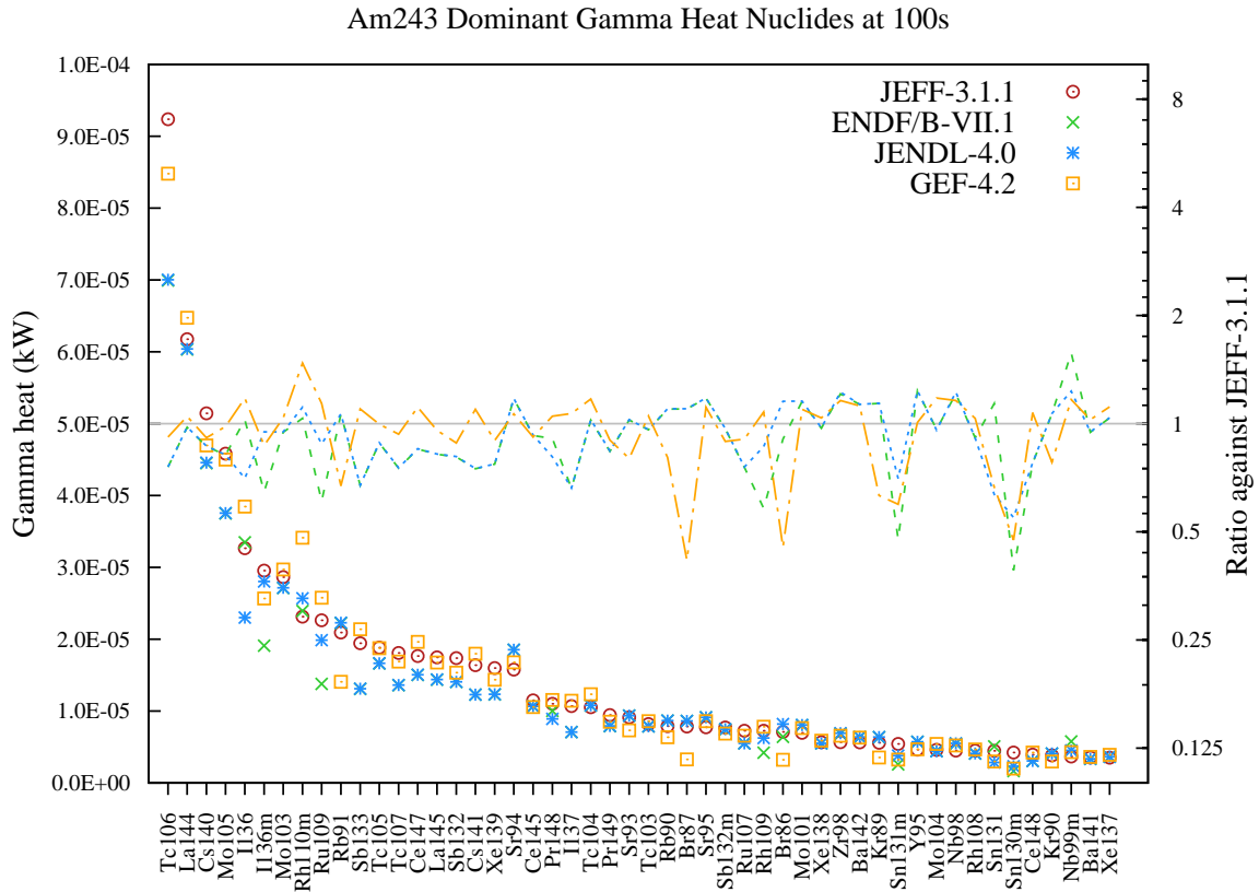
Figure 184: Gamma decay heat (in kW) fission yield comparison for Am243 fission pulse after 100s cooling.
