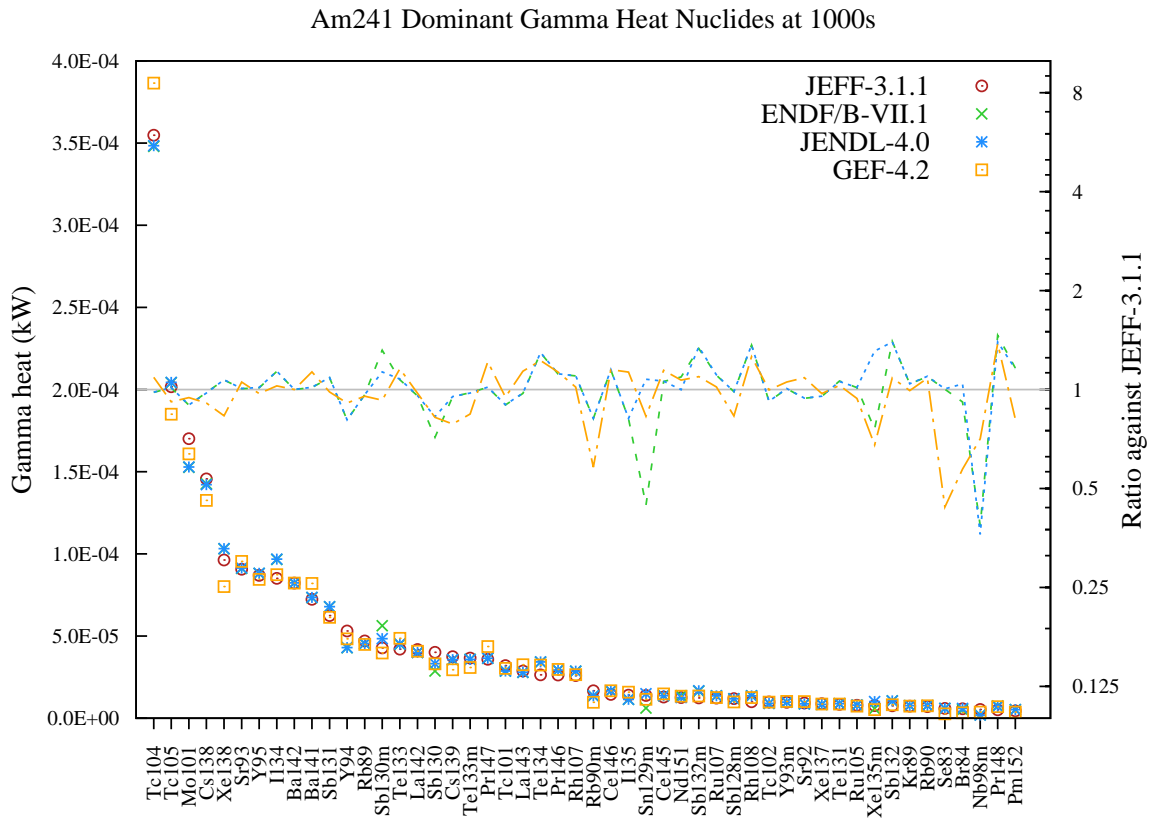
Figure 157: Gamma decay heat (in kW) fission yield comparison for Am241 fission pulse after 1000s cooling.
