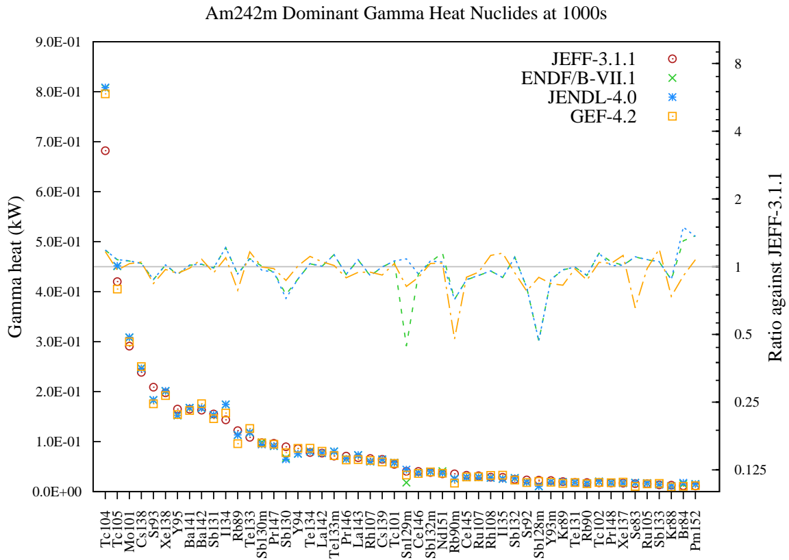
Figure 172: Gamma decay heat (in kW) fission yield comparison for Am242m fission pulse after 1000s cooling.
