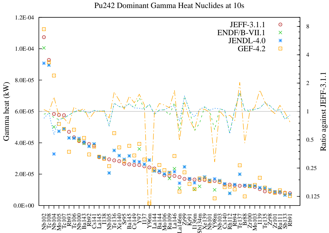
Figure 136: Gamma decay heat (in kW) fission yield comparison for Pu242 fission pulse after 10s cooling.
