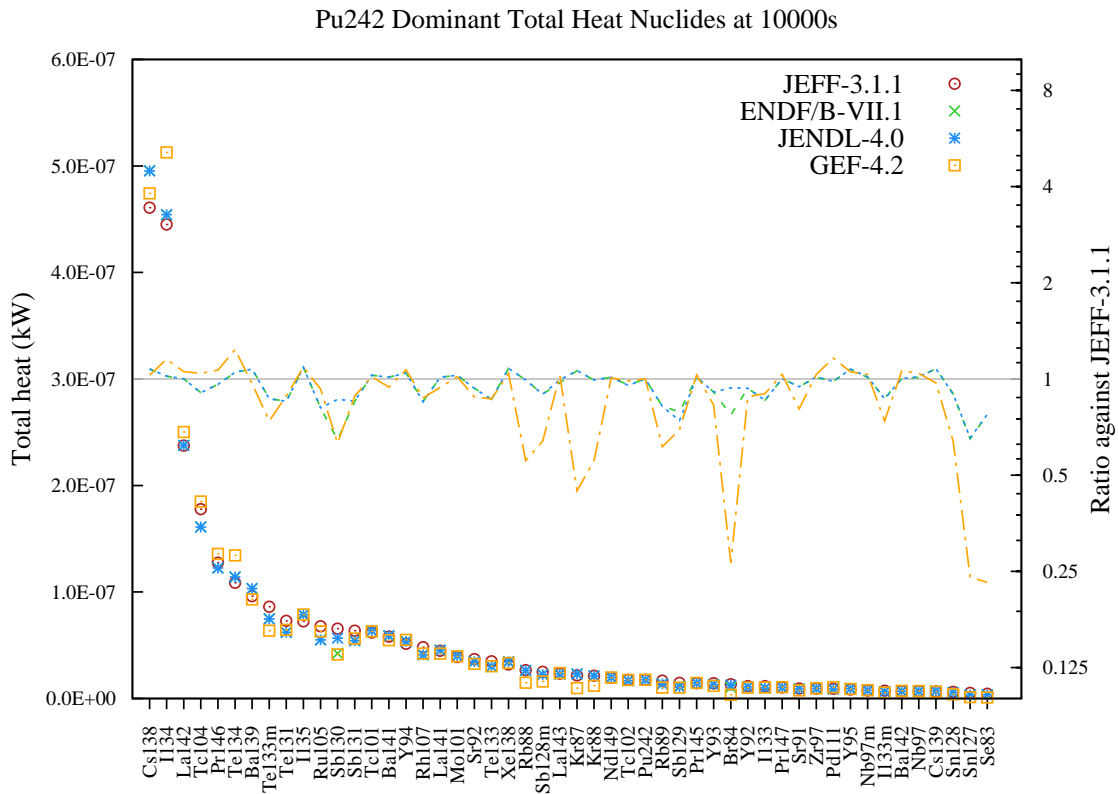
Figure 150: Total decay heat (in kW) fission yield comparison for Pu242 fission pulse after 10000s cooling.
