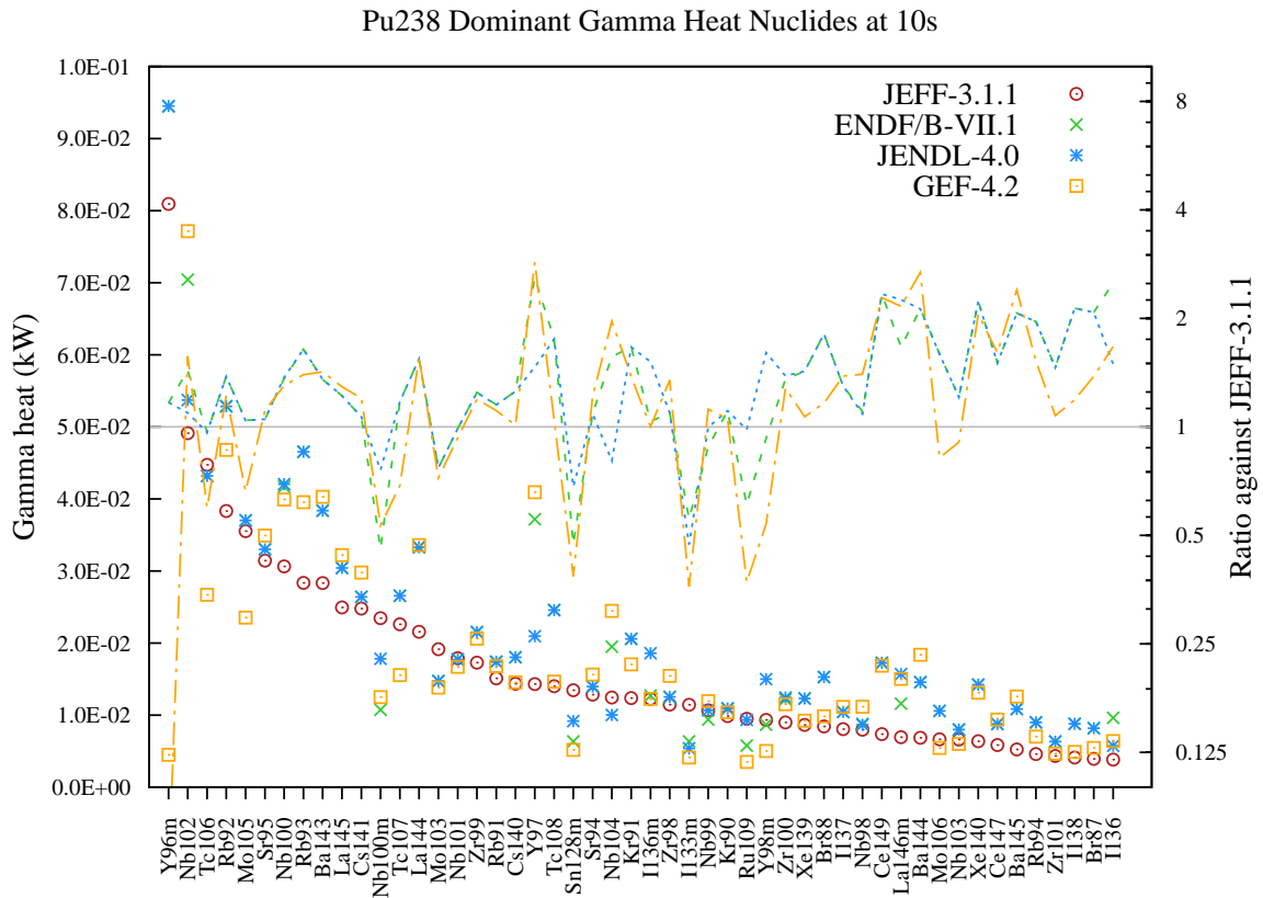
Figure 76: Gamma decay heat (in kW) fission yield comparison for Pu238 fission pulse after 10s cooling.
