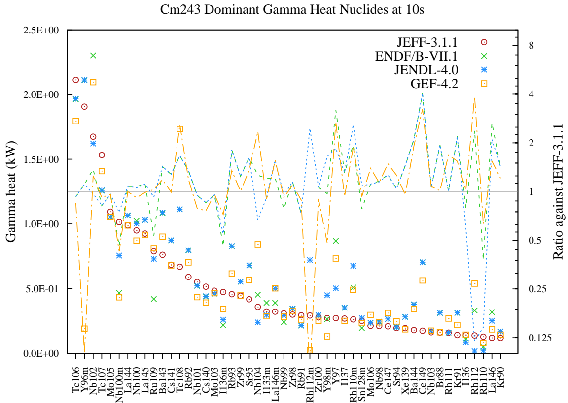
Figure 196: Gamma decay heat (in kW) fission yield comparison for Cm243 fission pulse after 10s cooling.
