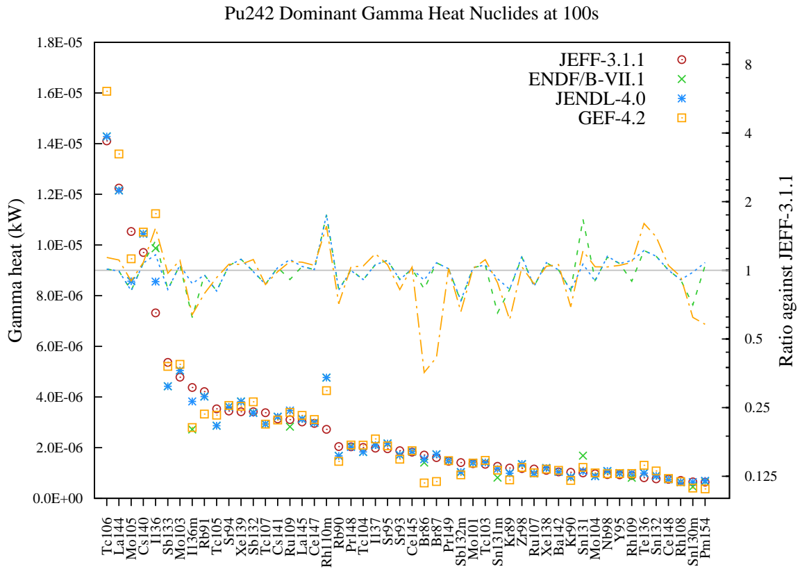
Figure 139: Gamma decay heat (in kW) fission yield comparison for Pu242 fission pulse after 100s cooling.
