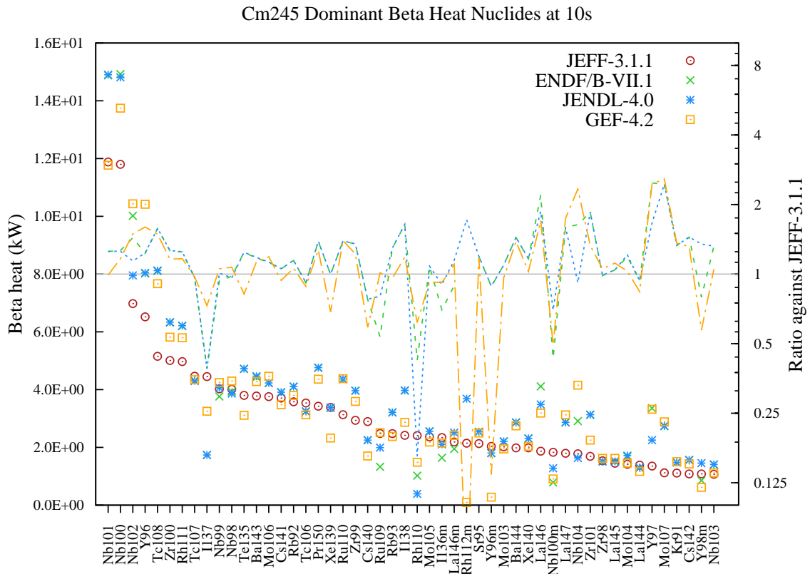
Figure 212: Beta decay heat (in kW) fission yield comparison for Cm245 fission pulse after 10s cooling.
