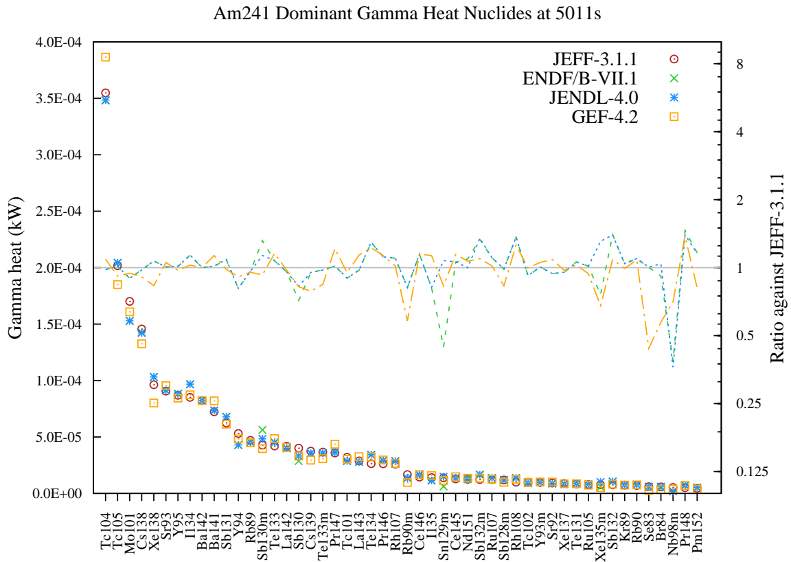
Figure 160: Gamma decay heat (in kW) fission yield comparison for Am241 fission pulse after 5011s cooling.
