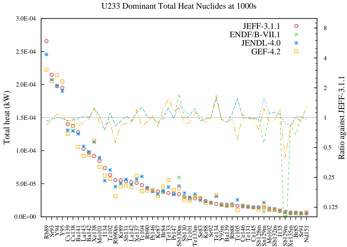
Figure 24: Total decay heat (in kW) fission yield comparison for U233 fission pulse after 1000s cooling.
