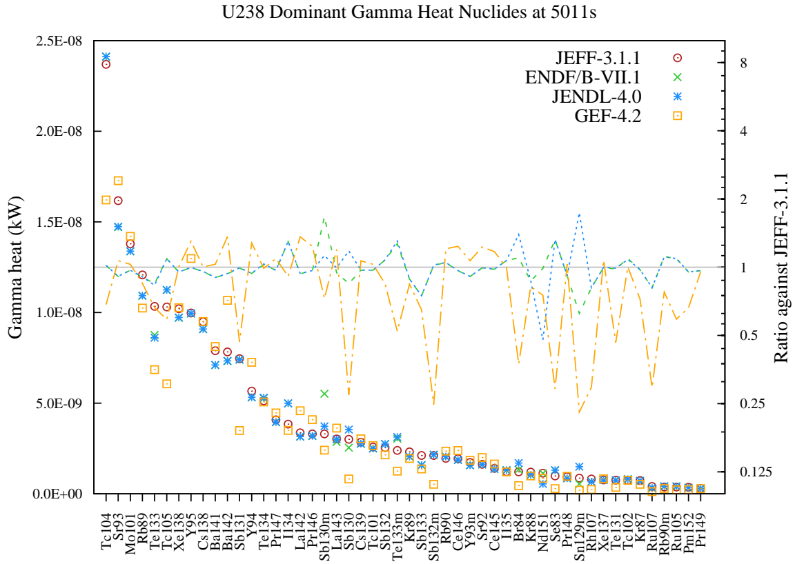
Figure 55: Gamma decay heat (in kW) fission yield comparison for U238 fission pulse after 5011s cooling.
