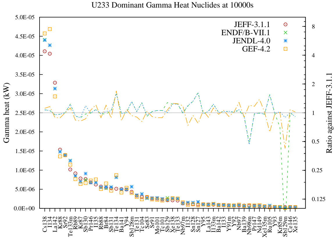
Figure 28: Gamma decay heat (in kW) fission yield comparison for U233 fission pulse after 10000s cooling.
