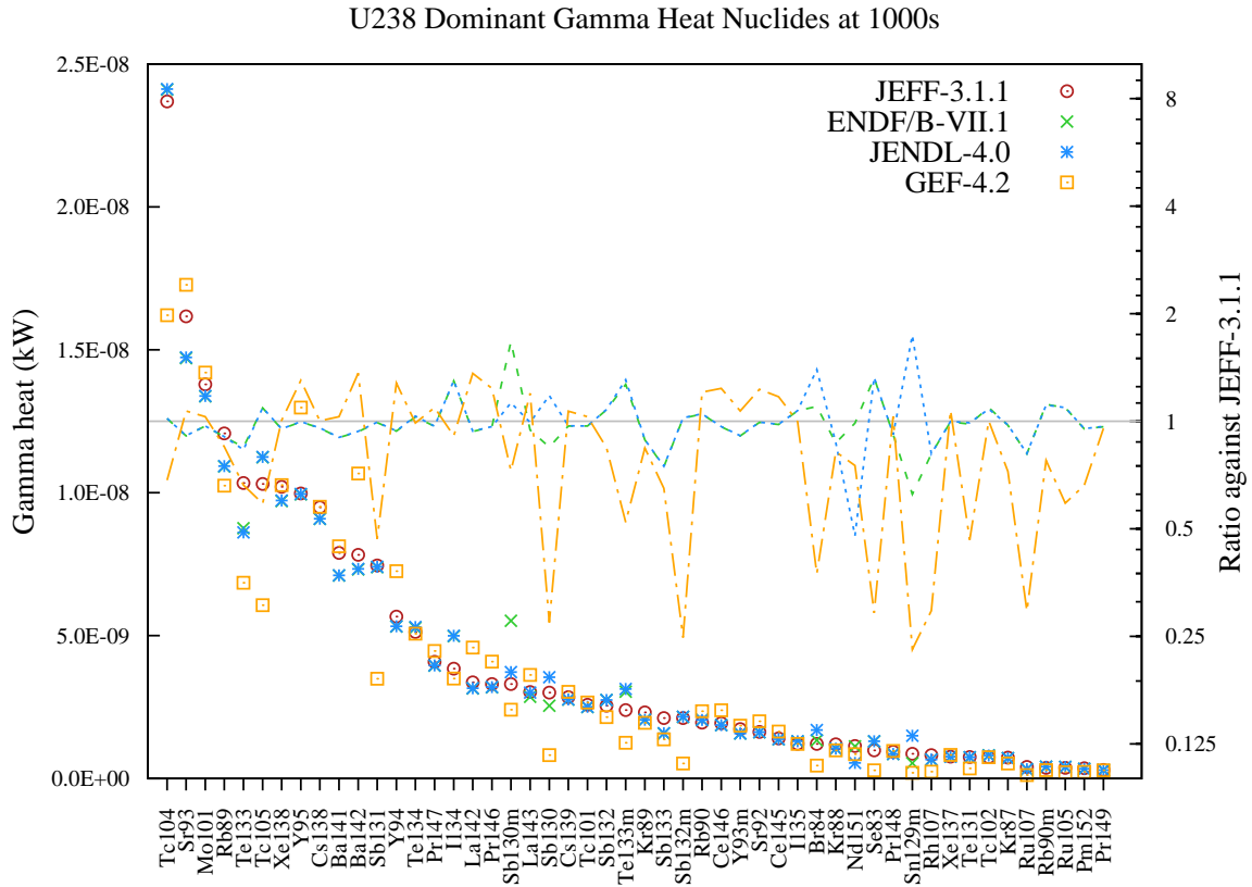
Figure 52: Gamma decay heat (in kW) fission yield comparison for U238 fission pulse after 1000s cooling.
