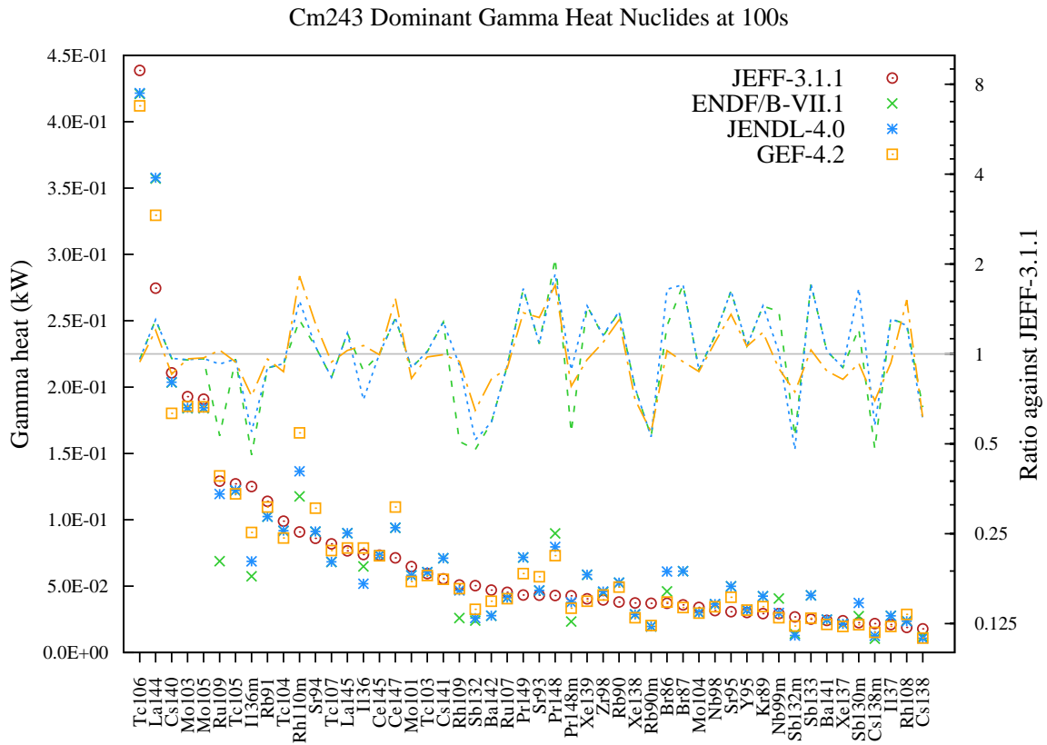
Figure 199: Gamma decay heat (in kW) fission yield comparison for Cm243 fission pulse after 100s cooling.
