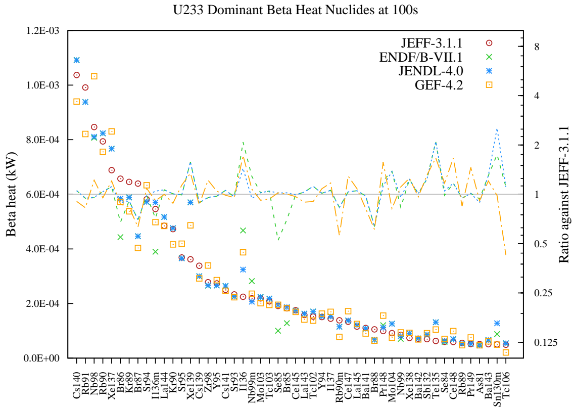
Figure 20: Beta decay heat (in kW) fission yield comparison for U233 fission pulse after 100s cooling.
