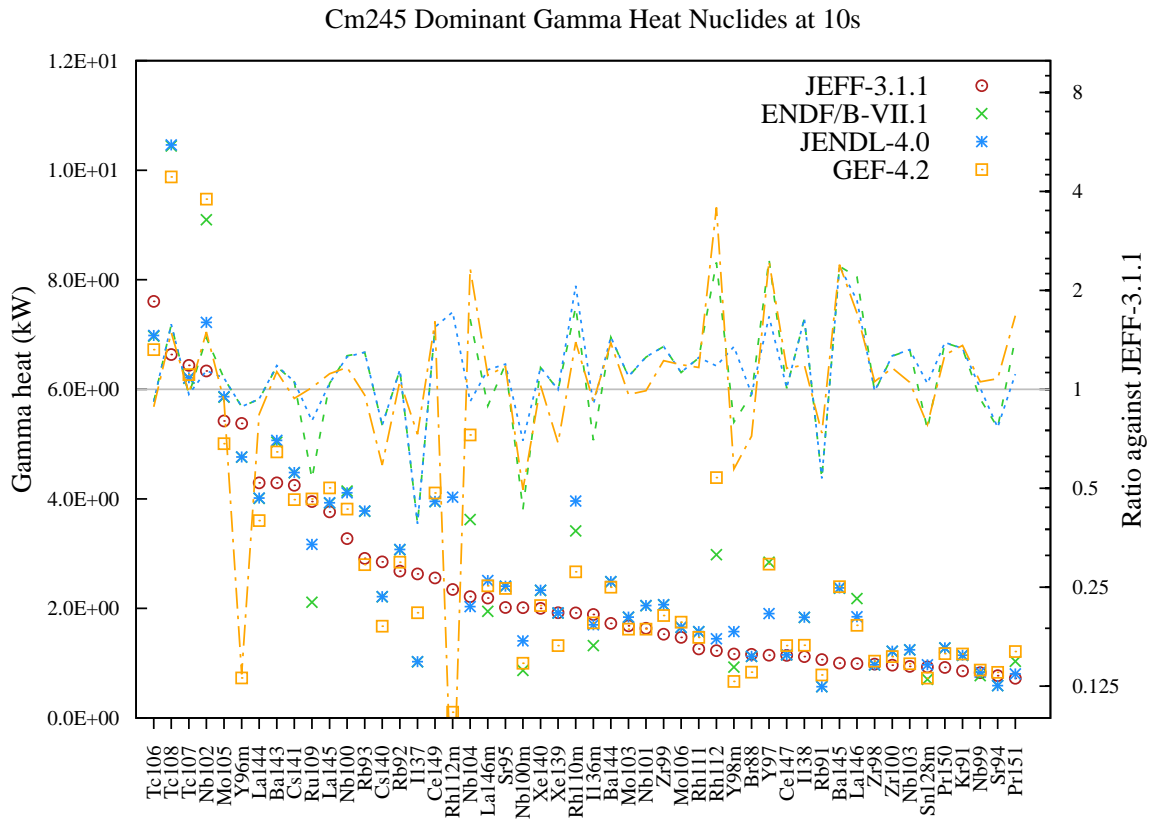
Figure 211: Gamma decay heat (in kW) fission yield comparison for Cm245 fission pulse after 10s cooling.
