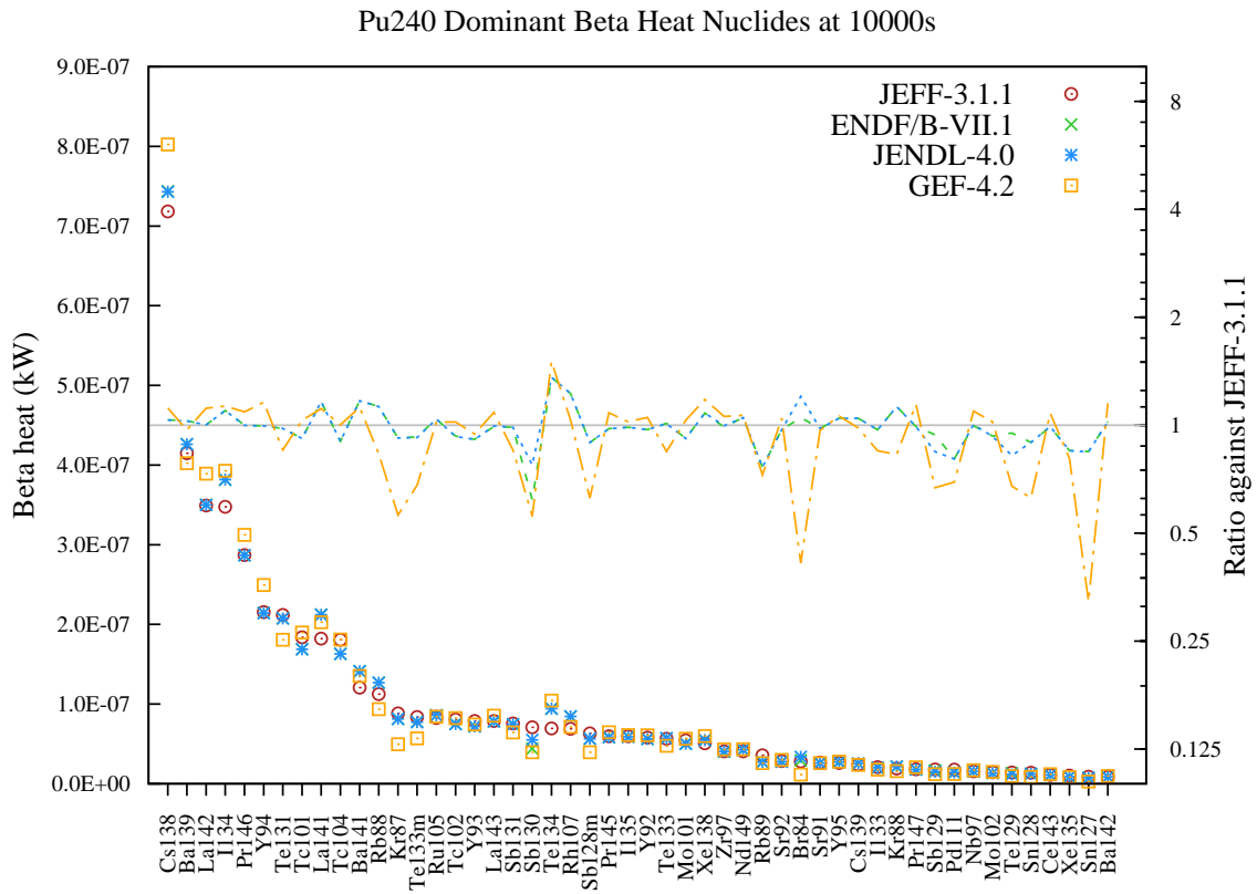
Figure 119: Beta decay heat (in kW) fission yield comparison for Pu240 fission pulse after 10000s cooling.
