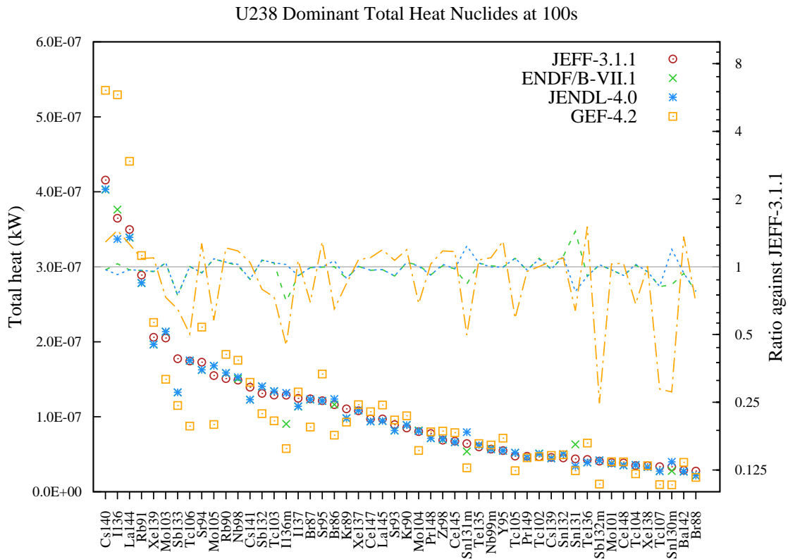
Figure 51: Total decay heat (in kW) fission yield comparison for U238 fission pulse after 100s cooling.
