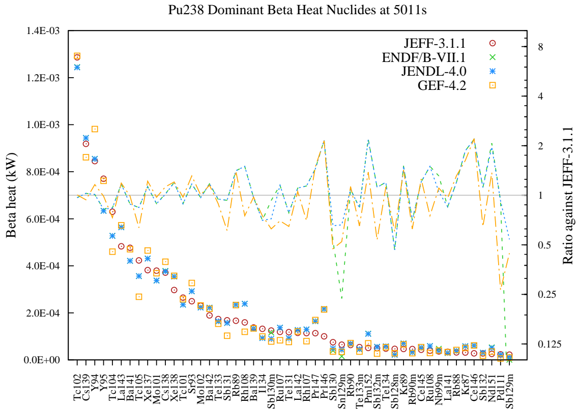
Figure 86: Beta decay heat (in kW) fission yield comparison for Pu238 fission pulse after 5011s cooling.
