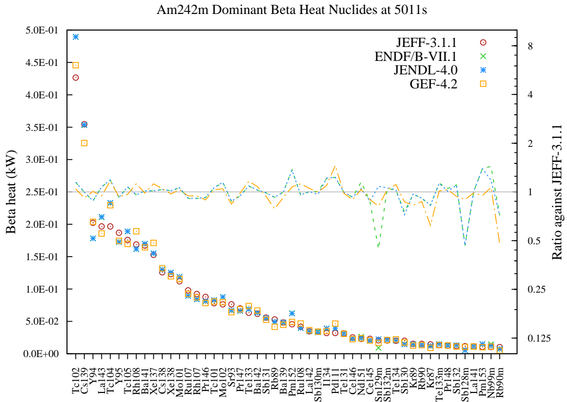
Figure 176: Beta decay heat (in kW) fission yield comparison for Am242m fission pulse after 5011s cooling.
