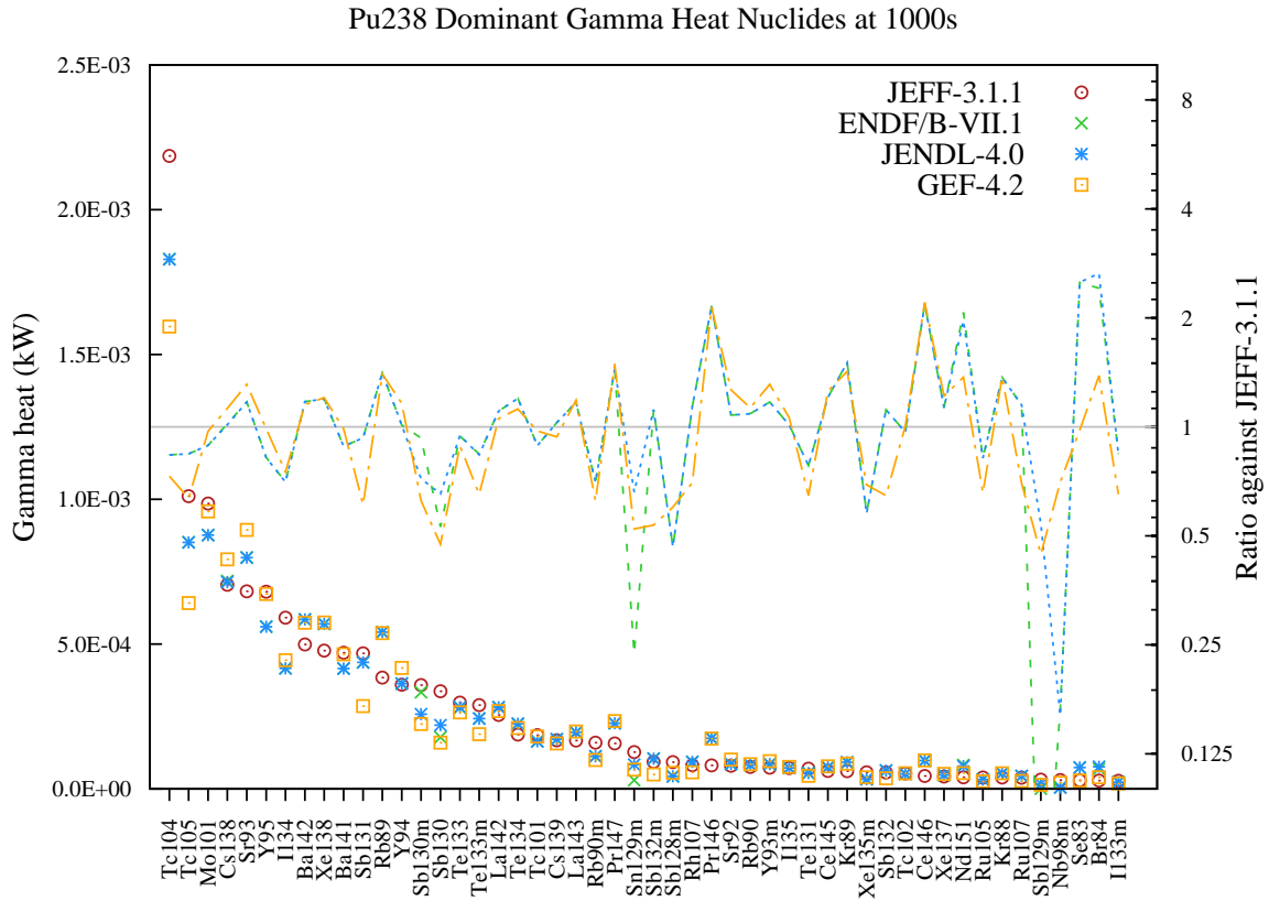
Figure 82: Gamma decay heat (in kW) fission yield comparison for Pu238 fission pulse after 1000s cooling.
