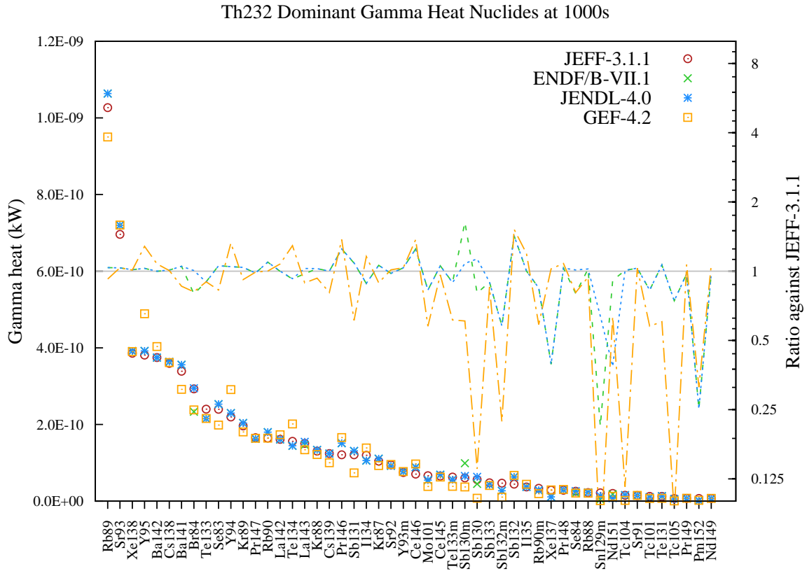
Figure 7: Gamma decay heat (in kW) fission yield comparison for Th232 fission pulse after 1000s cooling.
