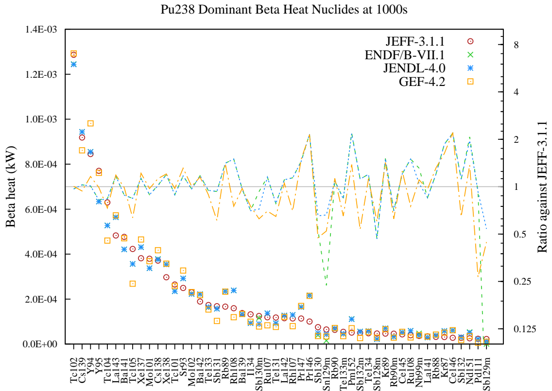
Figure 83: Beta decay heat (in kW) fission yield comparison for Pu238 fission pulse after 1000s cooling.
