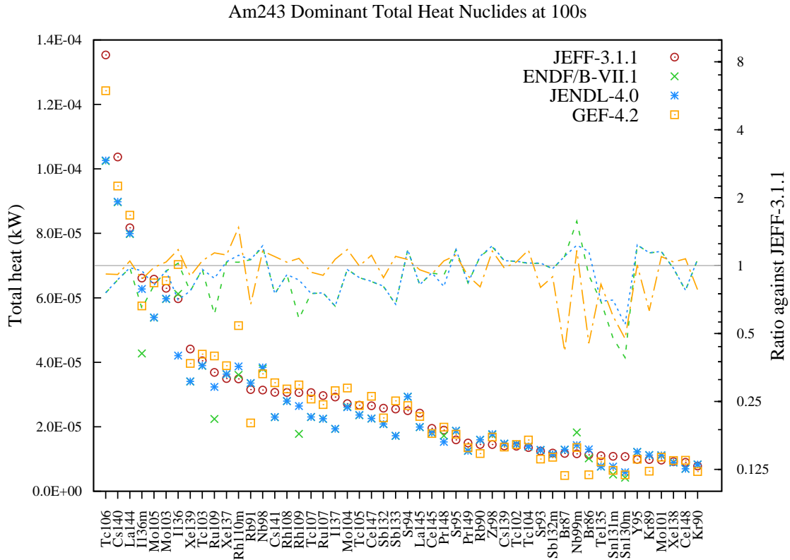
Figure 186: Total decay heat (in kW) fission yield comparison for Am243 fission pulse after 100s cooling.
