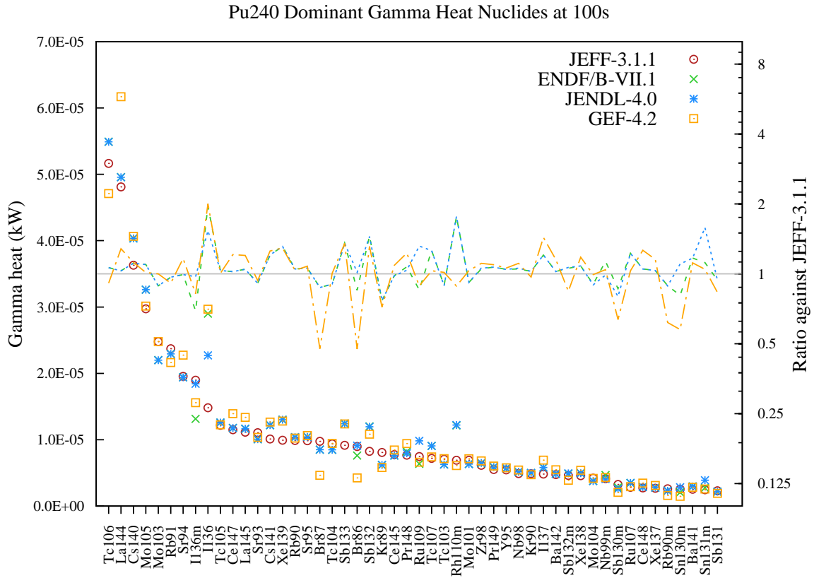
Figure 109: Gamma decay heat (in kW) fission yield comparison for Pu240 fission pulse after 100s cooling.
