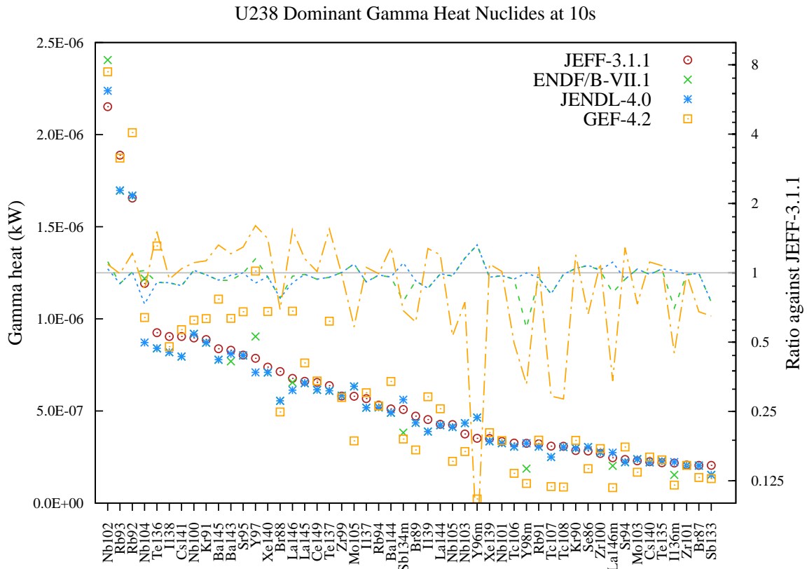
Figure 46: Gamma decay heat (in kW) fission yield comparison for U238 fission pulse after 10s cooling.
