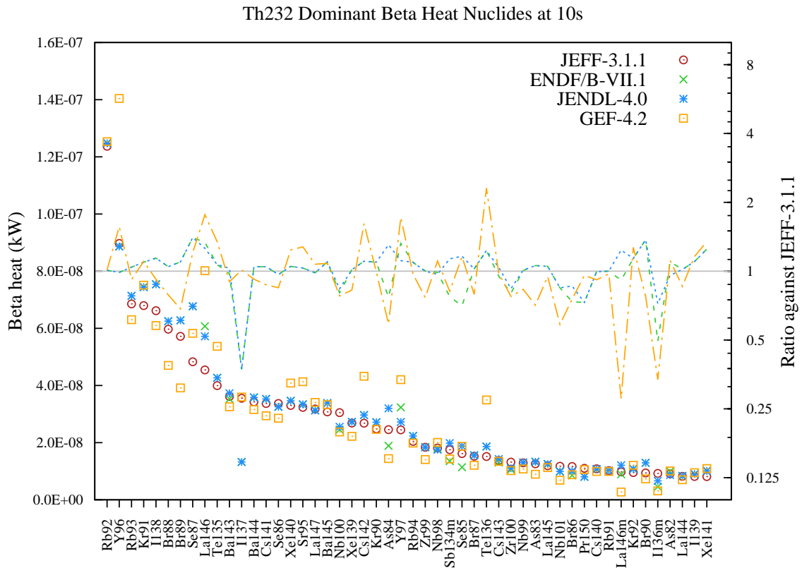
Figure 2: Beta decay heat (in kW) fission yield comparison for Th232 fission pulse after 10s cooling.
