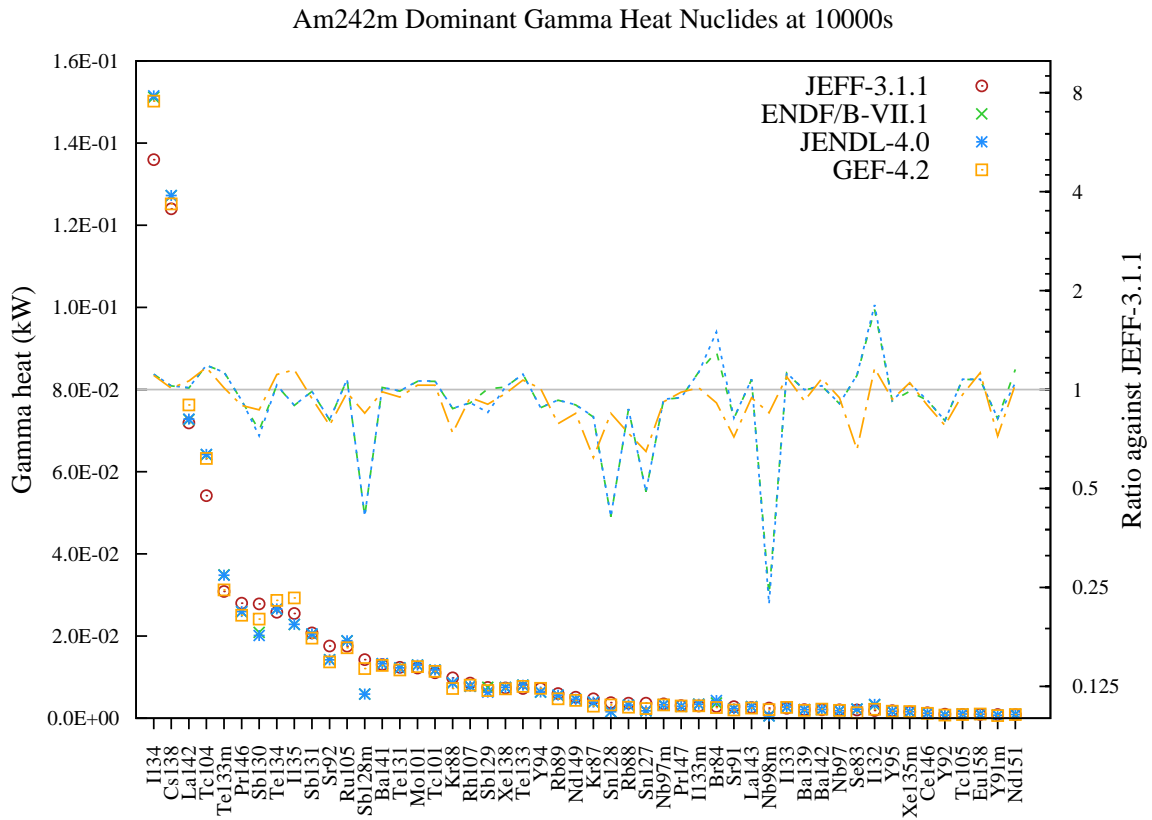
Figure 178: Gamma decay heat (in kW) fission yield comparison for Am242m fission pulse after 10000s cooling.
