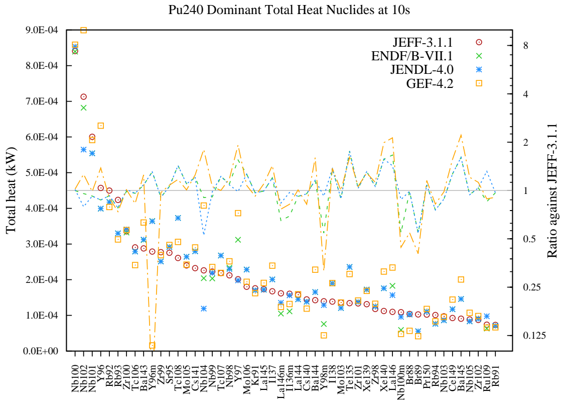
Figure 108: Total decay heat (in kW) fission yield comparison for Pu240 fission pulse after 10s cooling.
