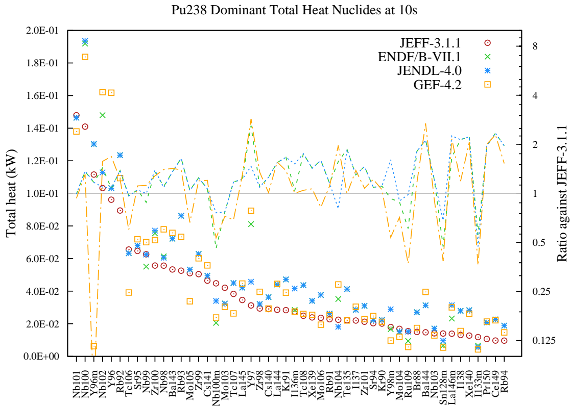
Figure 78: Total decay heat (in kW) fission yield comparison for Pu238 fission pulse after 10s cooling.
