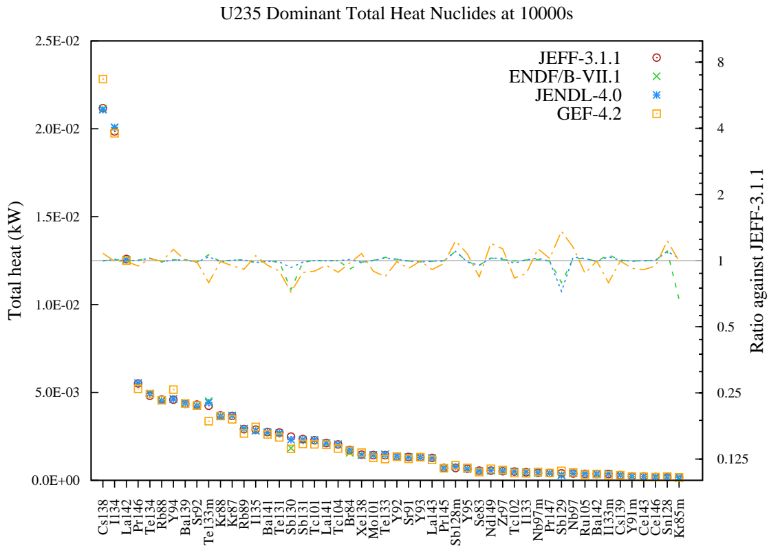
Figure 45: Total decay heat (in kW) fission yield comparison for U235 fission pulse after 10000s cooling.
