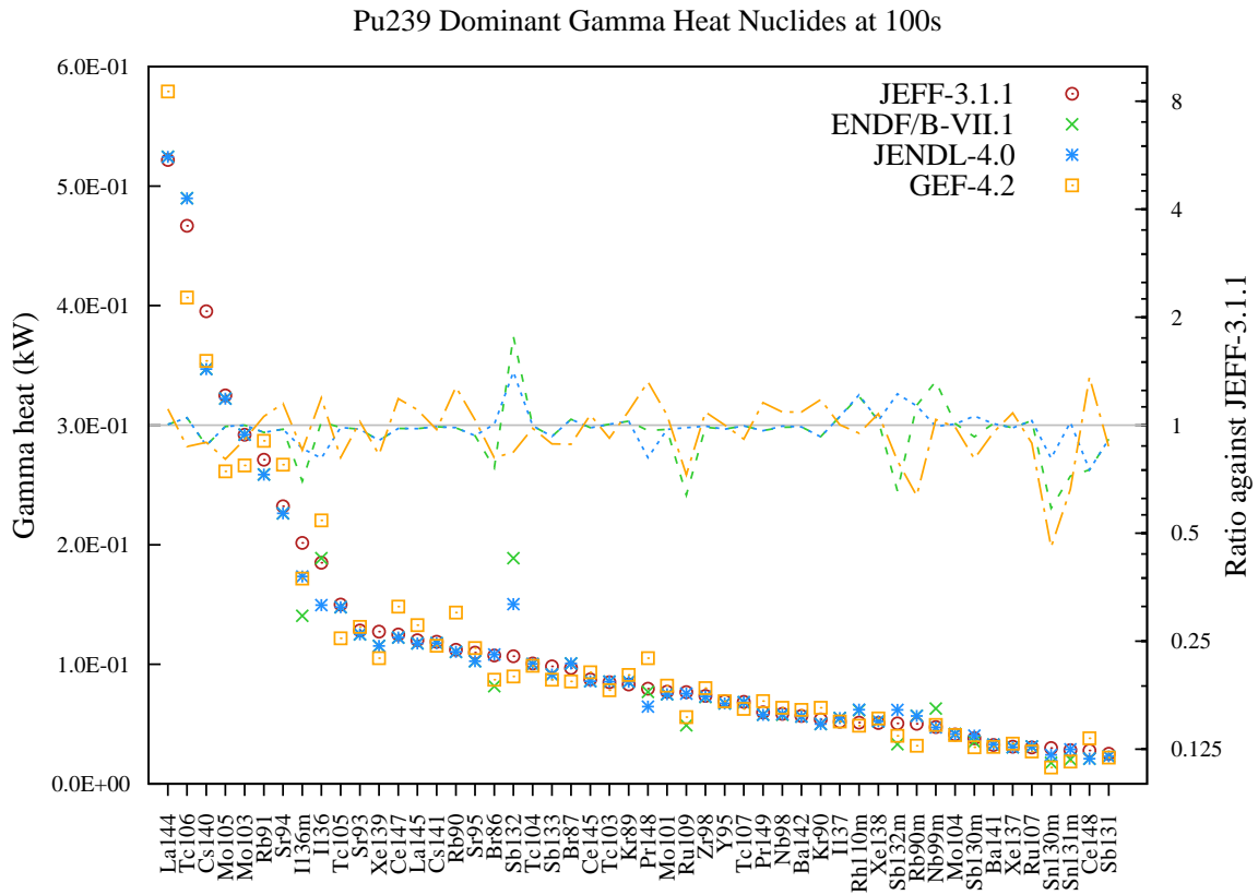
Figure 94: Gamma decay heat (in kW) fission yield comparison for Pu239 fission pulse after 100s cooling.
