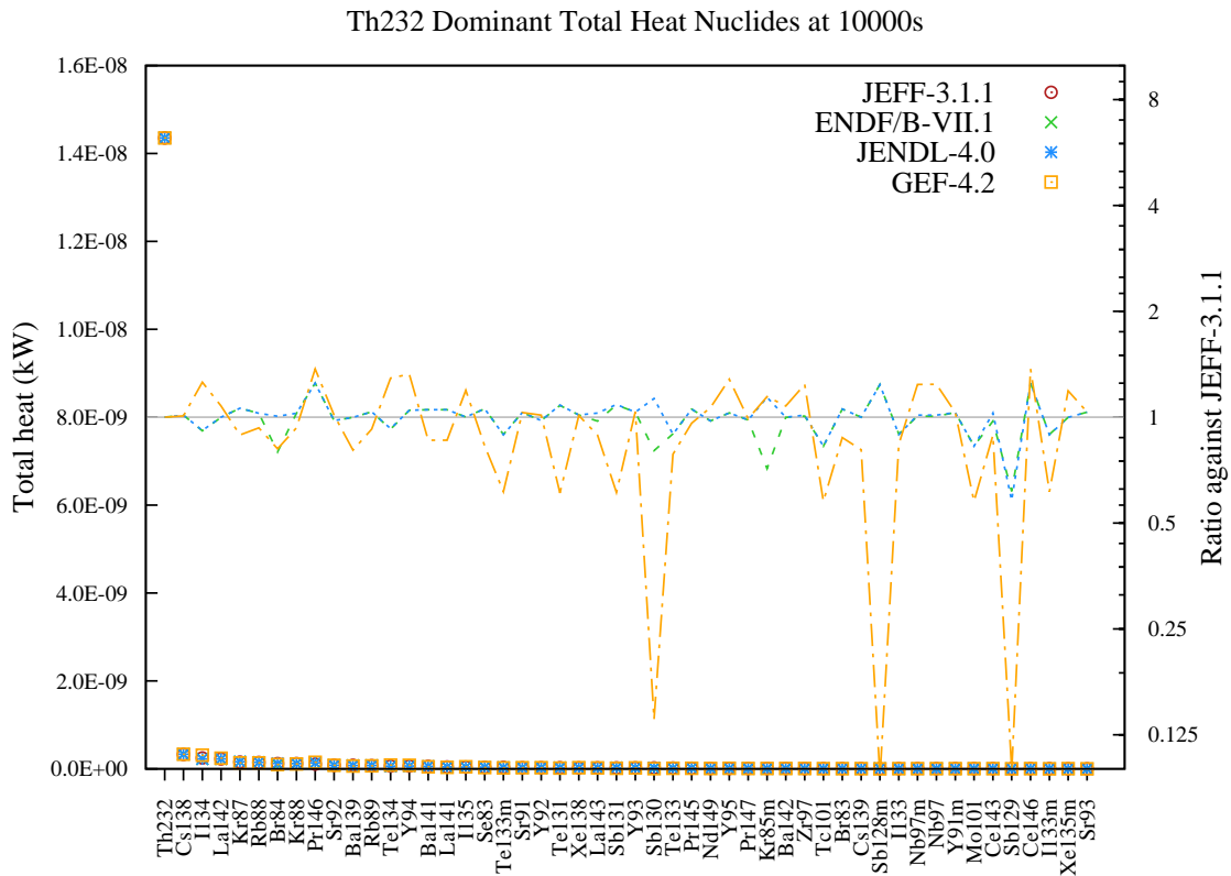
Figure 15: Total decay heat (in kW) fission yield comparison for Th232 fission pulse after 10000s cooling.
