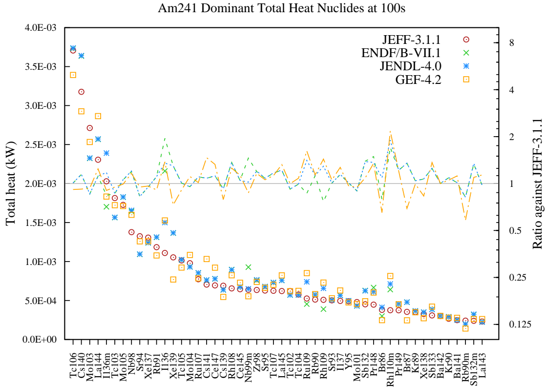
Figure 156: Total decay heat (in kW) fission yield comparison for Am241 fission pulse after 100s cooling.
