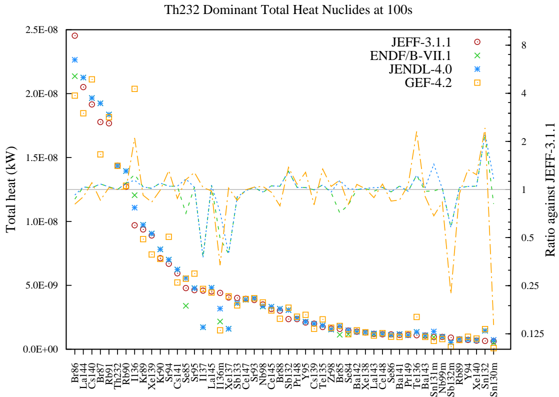
Figure 6: Total decay heat (in kW) fission yield comparison for Th232 fission pulse after 100s cooling.
