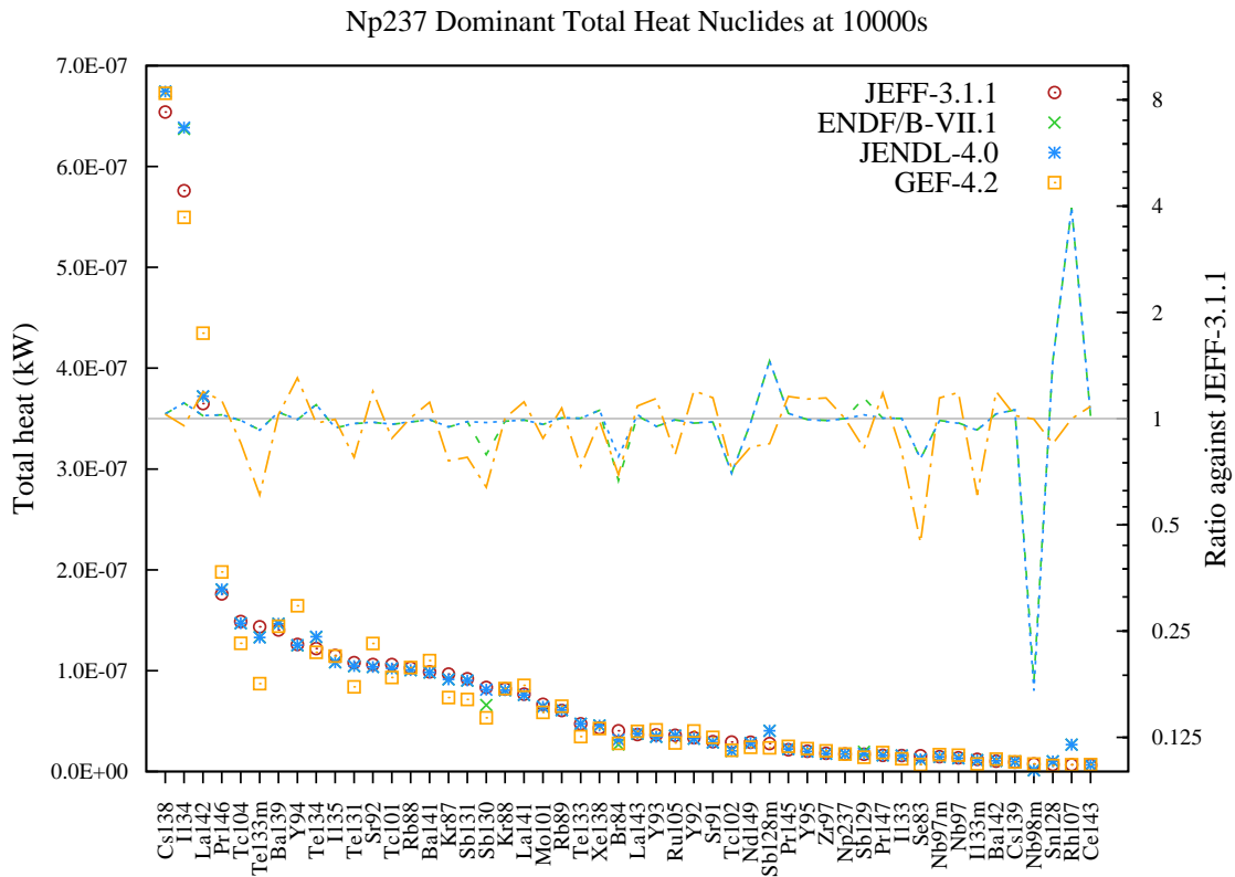
Figure 75: Total decay heat (in kW) fission yield comparison for Np237 fission pulse after 10000s cooling.
