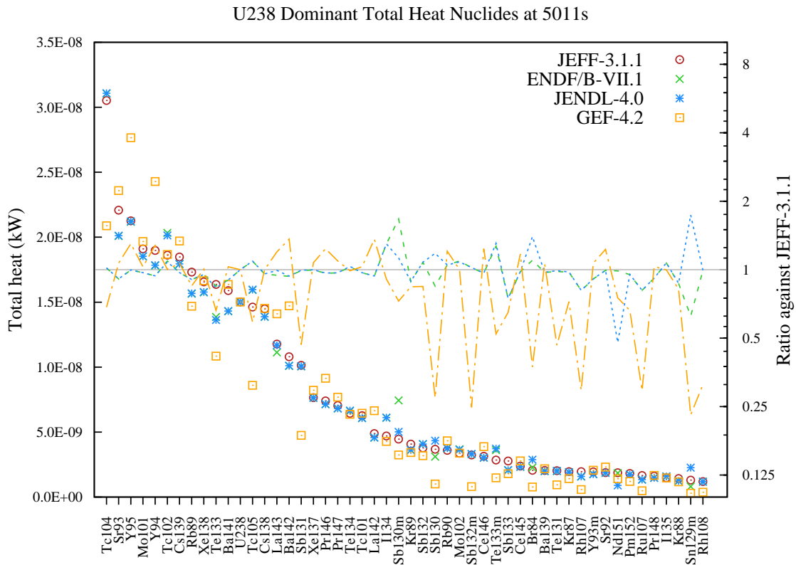
Figure 57: Total decay heat (in kW) fission yield comparison for U238 fission pulse after 5011s cooling.
