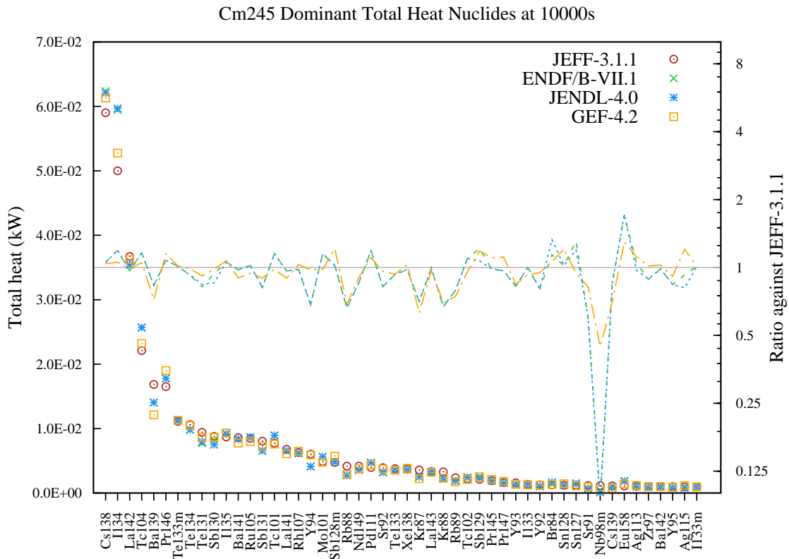
Figure 225: Total decay heat (in kW) fission yield comparison for Cm245 fission pulse after 10000s cooling.
