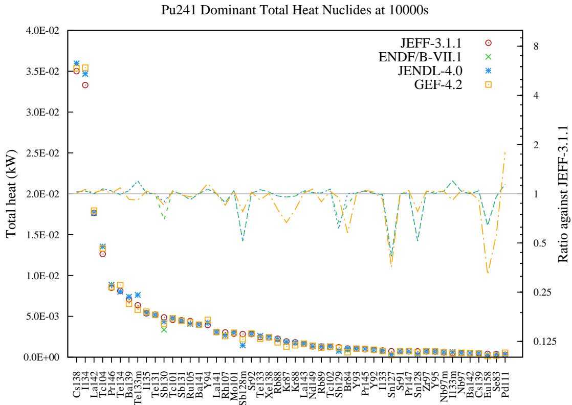
Figure 135: Total decay heat (in kW) fission yield comparison for Pu241 fission pulse after 10000s cooling.
