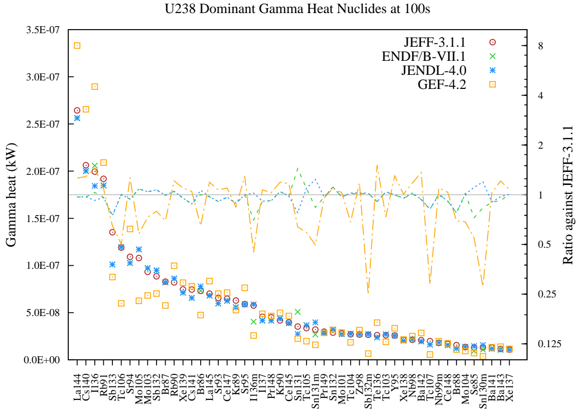
Figure 49: Gamma decay heat (in kW) fission yield comparison for U238 fission pulse after 100s cooling.
