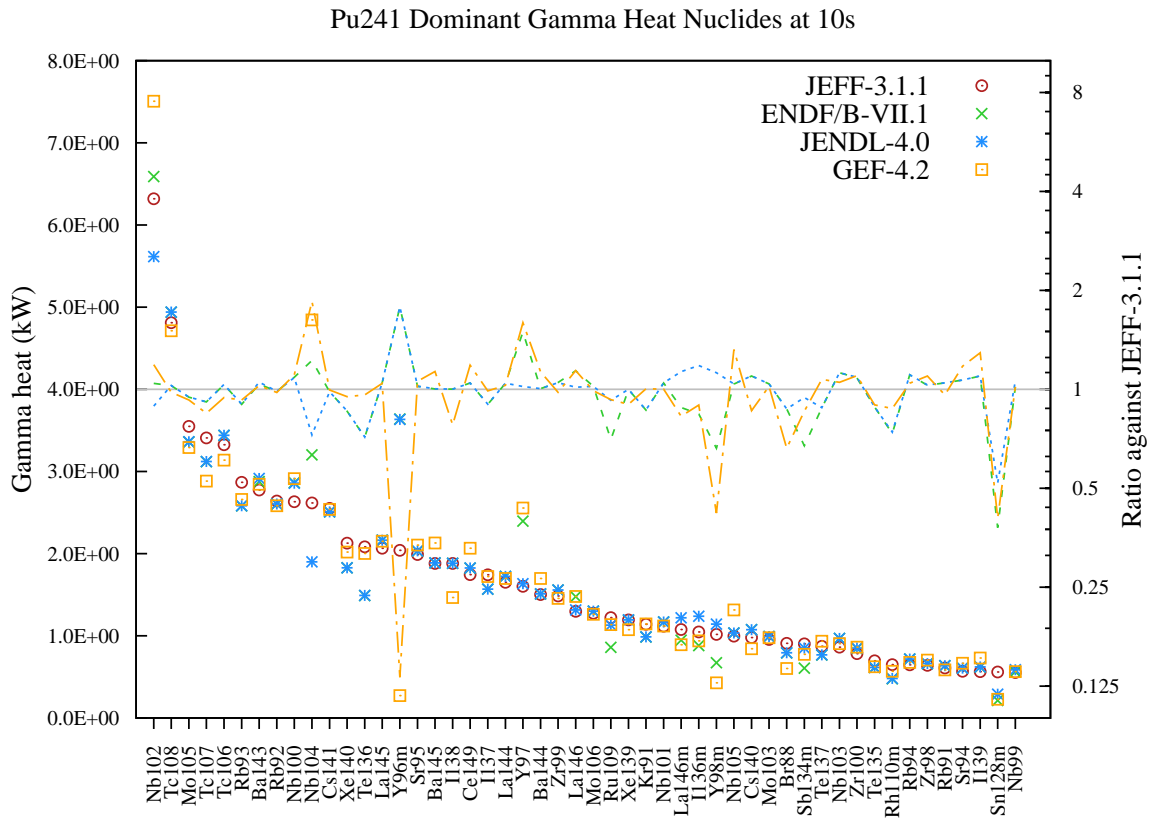
Figure 121: Gamma decay heat (in kW) fission yield comparison for Pu241 fission pulse after 10s cooling.
