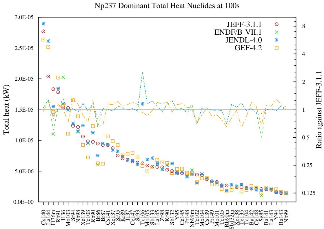
Figure 66: Total decay heat (in kW) fission yield comparison for Np237 fission pulse after 100s cooling.
