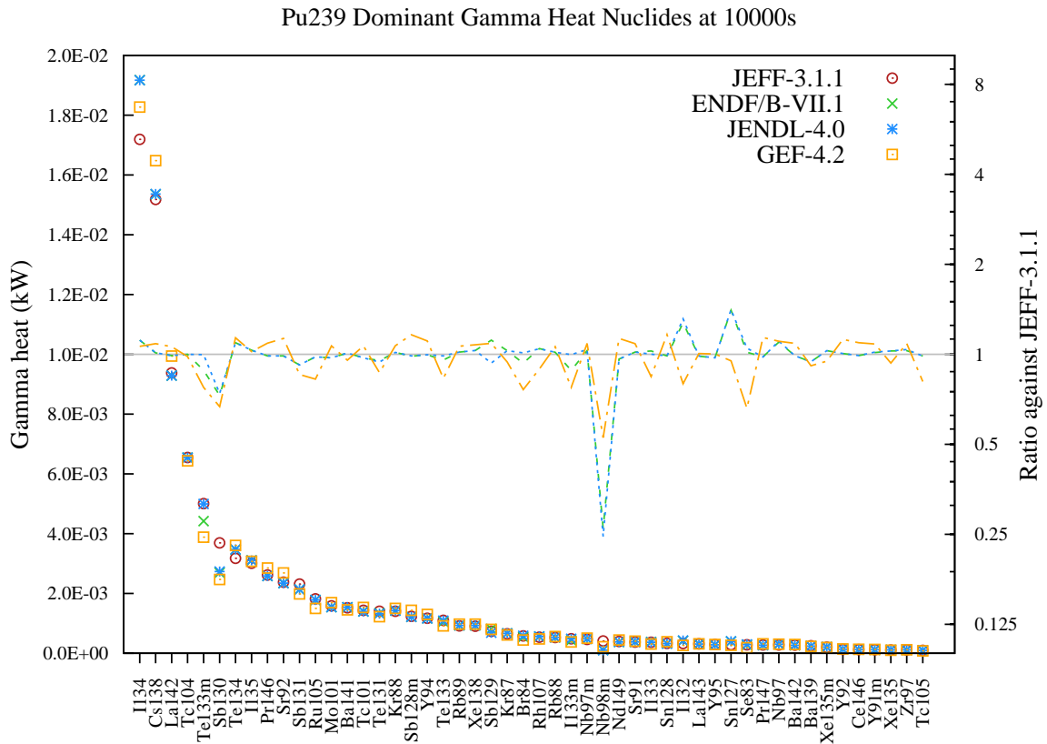
Figure 103: Gamma decay heat (in kW) fission yield comparison for Pu239 fission pulse after 10000s cooling.
