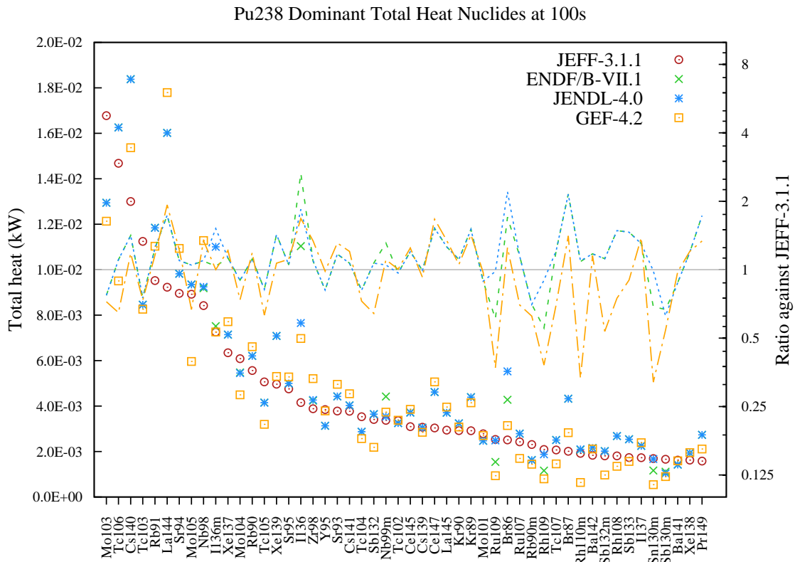
Figure 81: Total decay heat (in kW) fission yield comparison for Pu238 fission pulse after 100s cooling.
