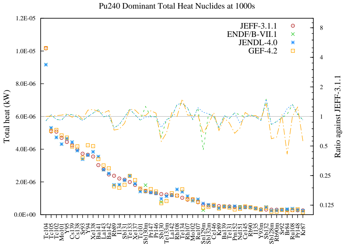
Figure 114: Total decay heat (in kW) fission yield comparison for Pu240 fission pulse after 1000s cooling.
