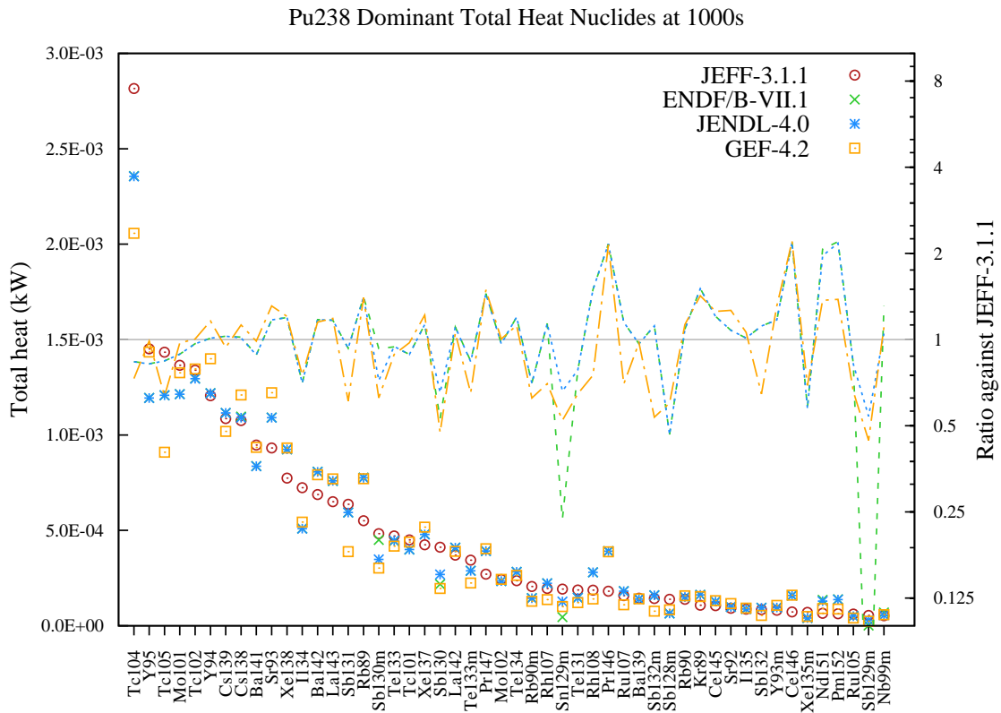
Figure 84: Total decay heat (in kW) fission yield comparison for Pu238 fission pulse after 1000s cooling.
