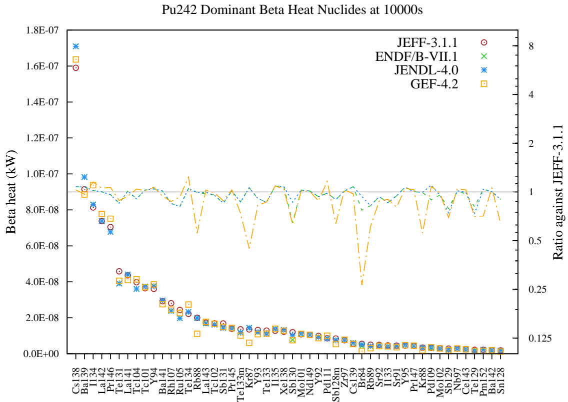
Figure 149: Beta decay heat (in kW) fission yield comparison for Pu242 fission pulse after 10000s cooling.
