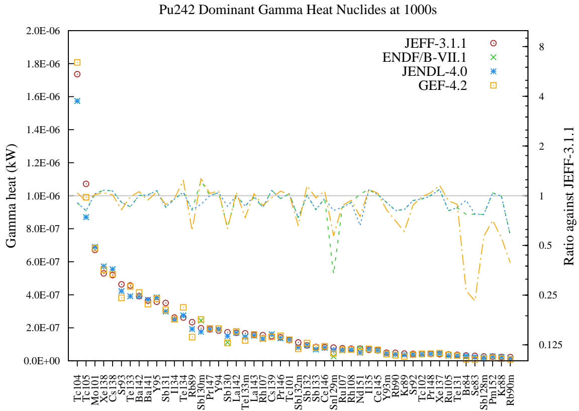
Figure 142: Gamma decay heat (in kW) fission yield comparison for Pu242 fission pulse after 1000s cooling.
