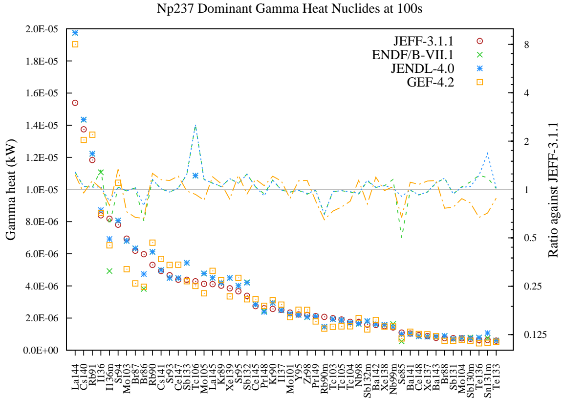
Figure 64: Gamma decay heat (in kW) fission yield comparison for Np237 fission pulse after 100s cooling.
