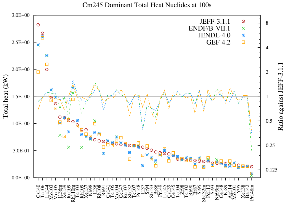
Figure 216: Total decay heat (in kW) fission yield comparison for Cm245 fission pulse after 100s cooling.
