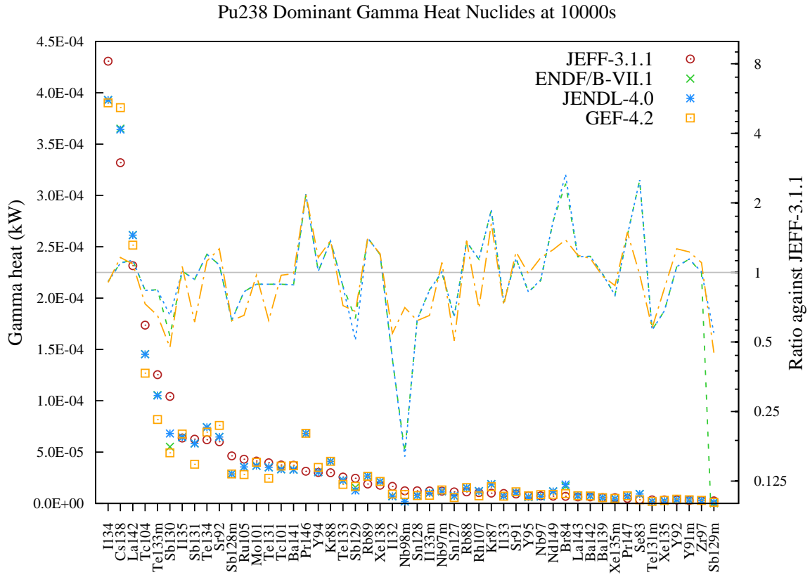
Figure 88: Gamma decay heat (in kW) fission yield comparison for Pu238 fission pulse after 10000s cooling.
