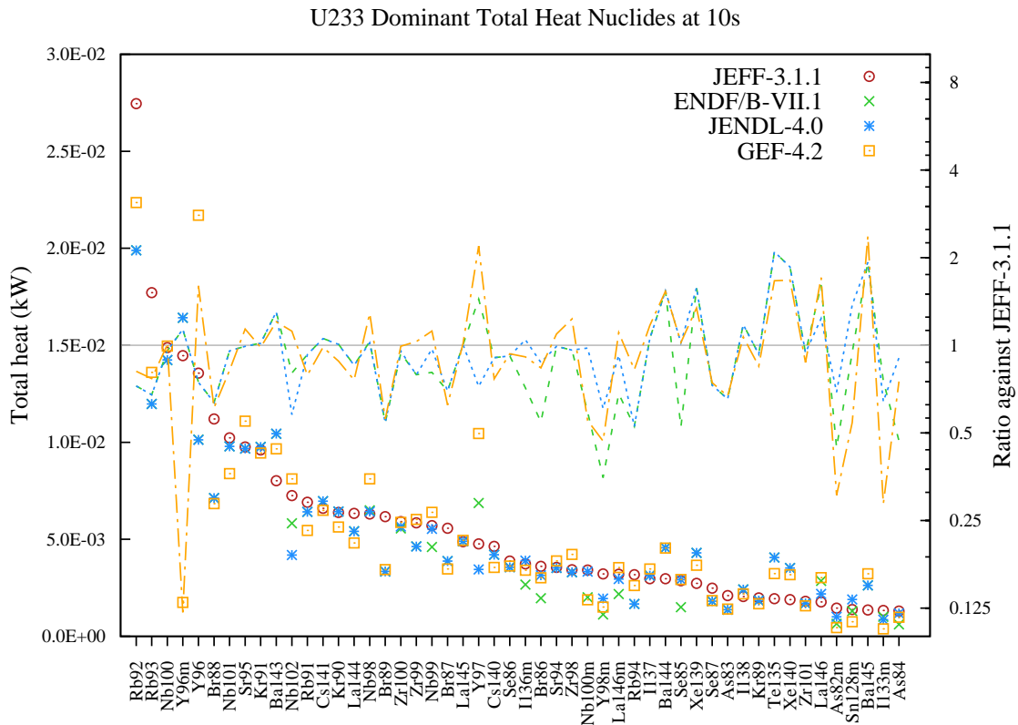
Figure 18: Total decay heat (in kW) fission yield comparison for U233 fission pulse after 10s cooling.
