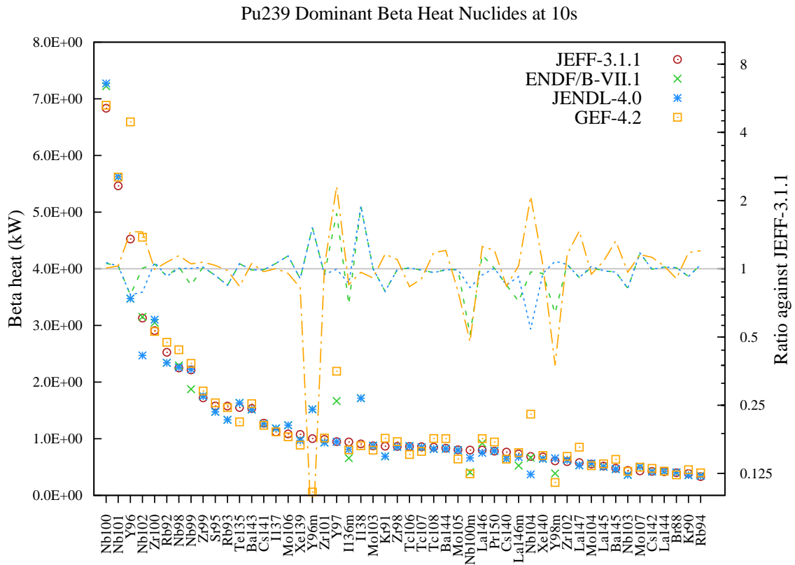
Figure 92: Beta decay heat (in kW) fission yield comparison for Pu239 fission pulse after 10s cooling.
