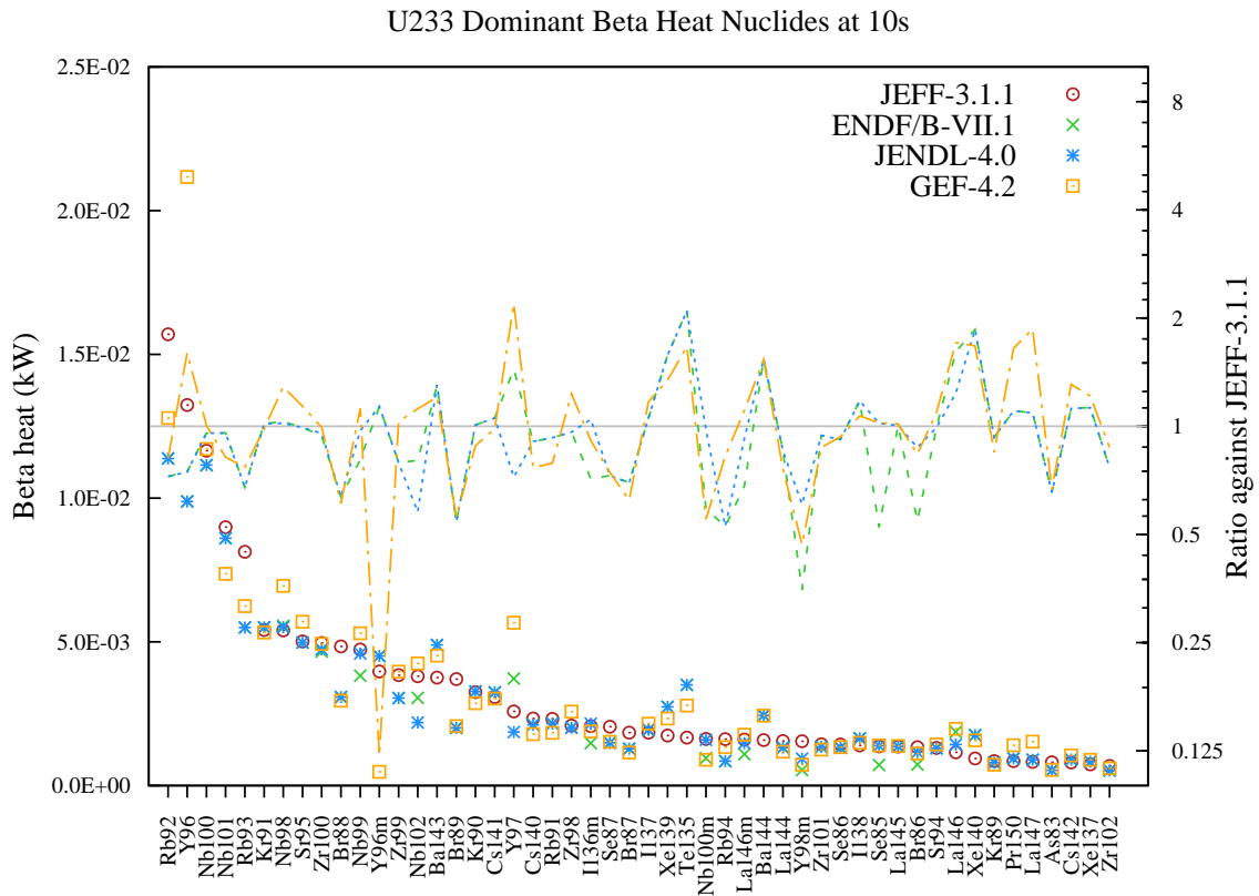
Figure 17: Beta decay heat (in kW) fission yield comparison for U233 fission pulse after 10s cooling.
