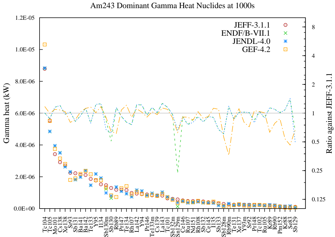
Figure 187: Gamma decay heat (in kW) fission yield comparison for Am243 fission pulse after 1000s cooling.
