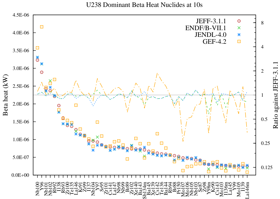
Figure 47: Beta decay heat (in kW) fission yield comparison for U238 fission pulse after 10s cooling.
