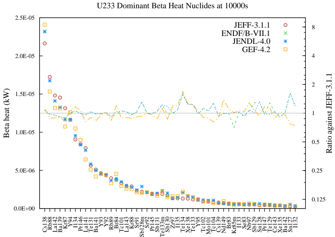
Figure 29: Beta decay heat (in kW) fission yield comparison for U233 fission pulse after 10000s cooling.
