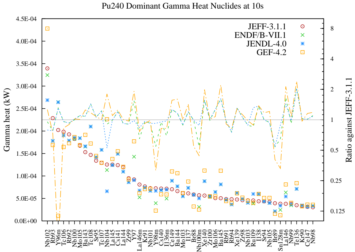
Figure 106: Gamma decay heat (in kW) fission yield comparison for Pu240 fission pulse after 10s cooling.
