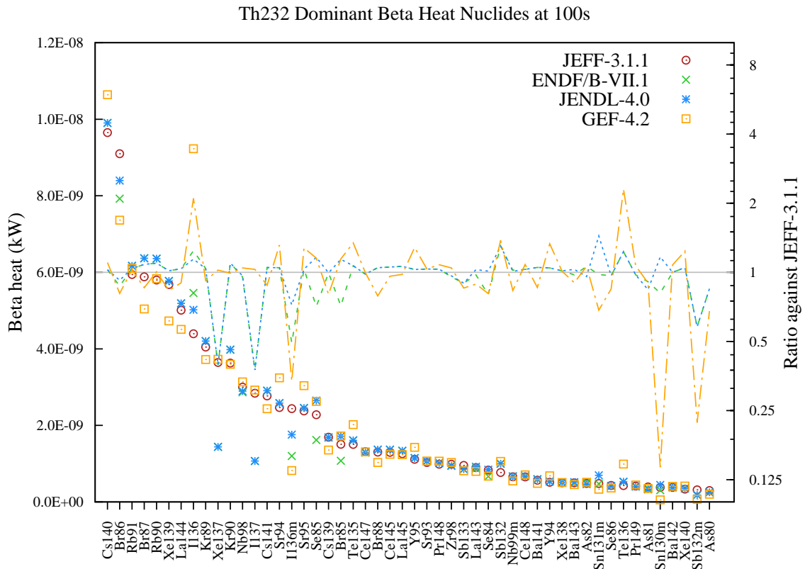
Figure 5: Beta decay heat (in kW) fission yield comparison for Th232 fission pulse after 100s cooling.
