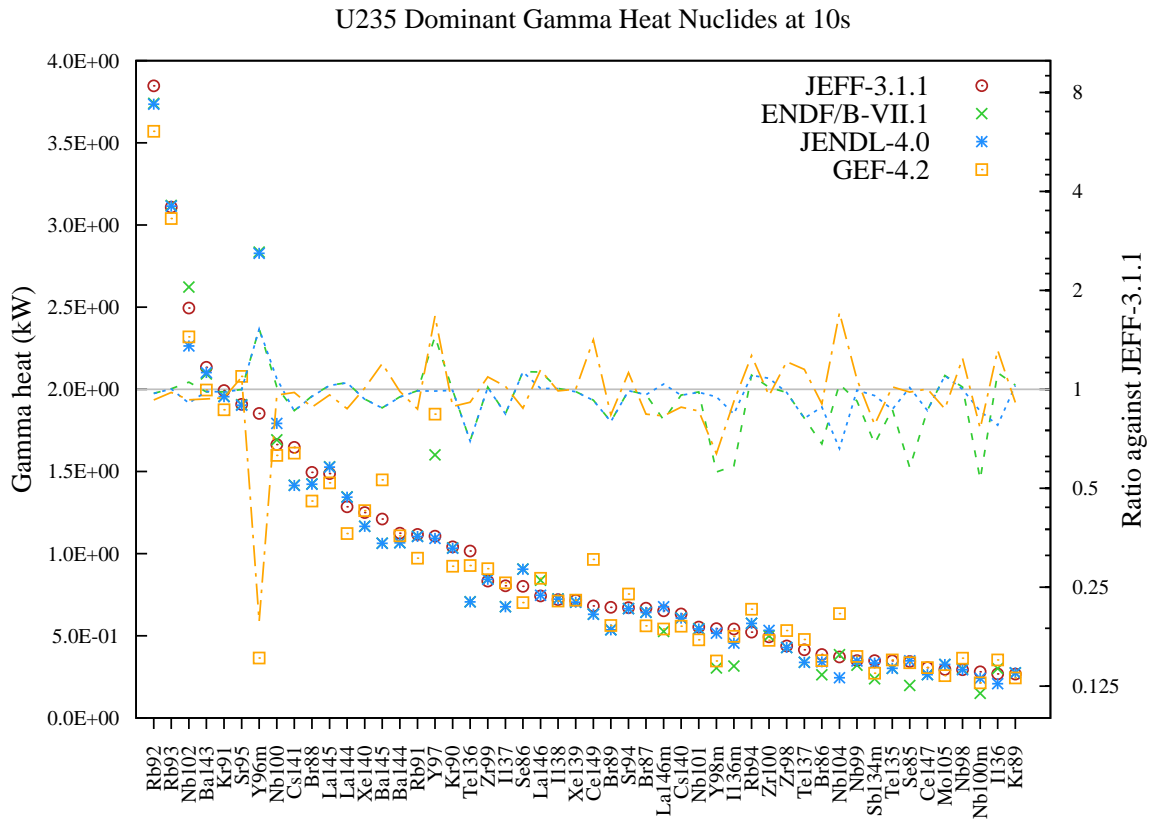
Figure 31: Gamma decay heat (in kW) fission yield comparison for U235 fission pulse after 10s cooling.
