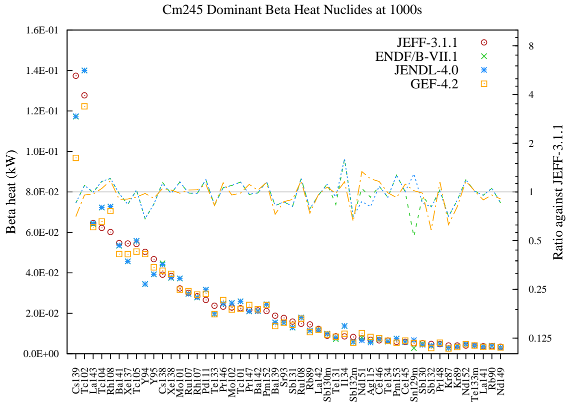
Figure 218: Beta decay heat (in kW) fission yield comparison for Cm245 fission pulse after 1000s cooling.
