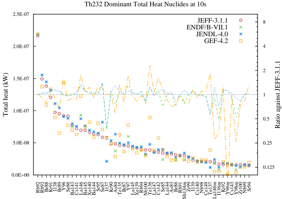
Figure 3: Total decay heat (in kW) fission yield comparison for Th232 fission pulse after 10s cooling.
