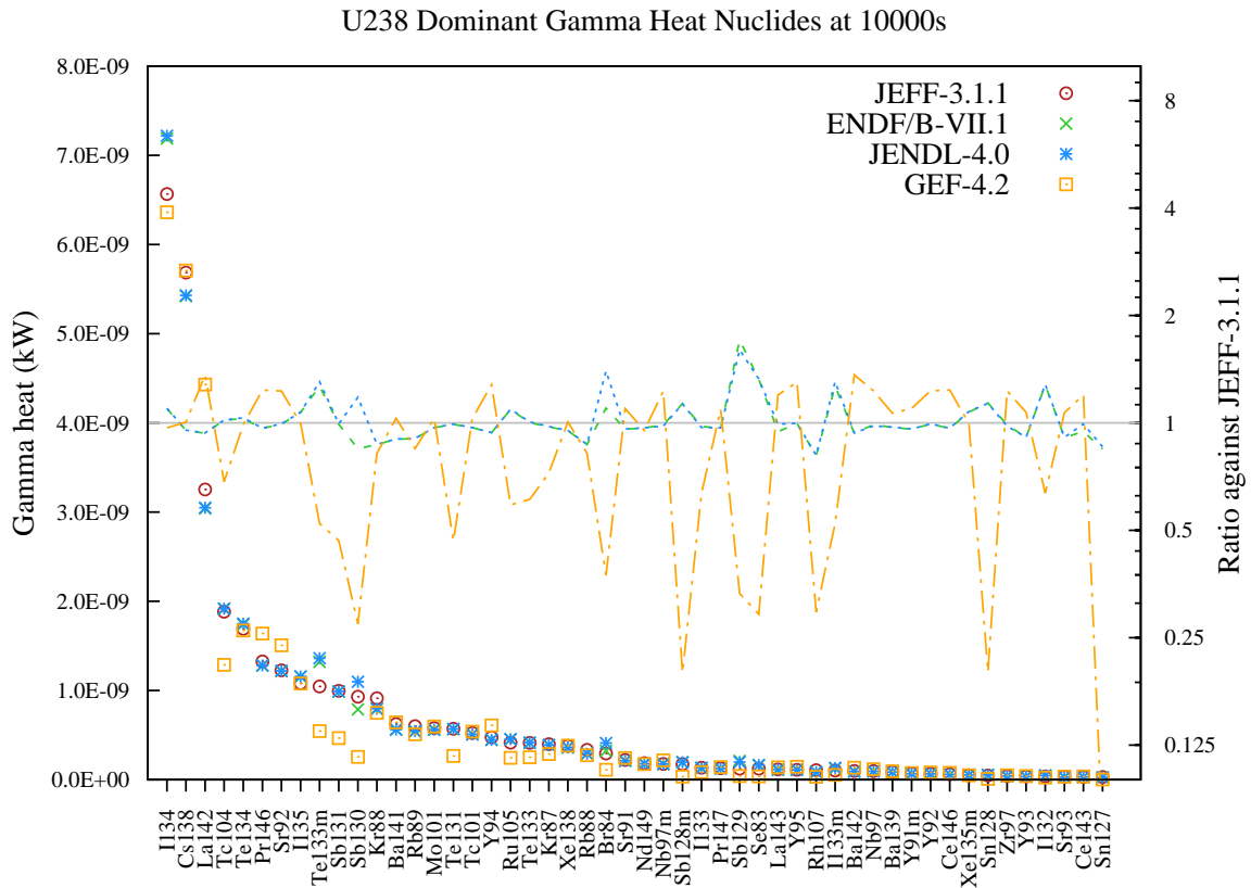
Figure 58: Gamma decay heat (in kW) fission yield comparison for U238 fission pulse after 10000s cooling.
