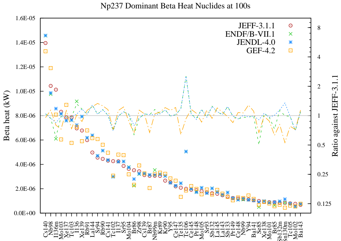
Figure 65: Beta decay heat (in kW) fission yield comparison for Np237 fission pulse after 100s cooling.
