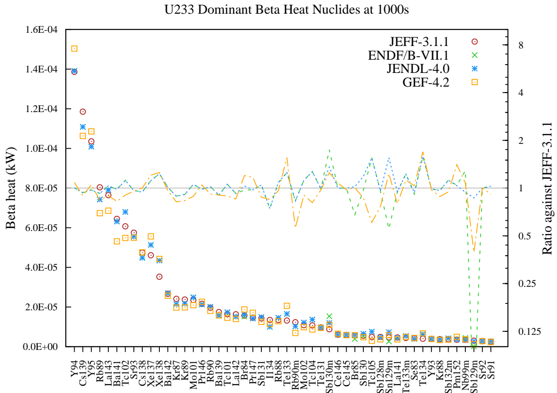
Figure 23: Beta decay heat (in kW) fission yield comparison for U233 fission pulse after 1000s cooling.
