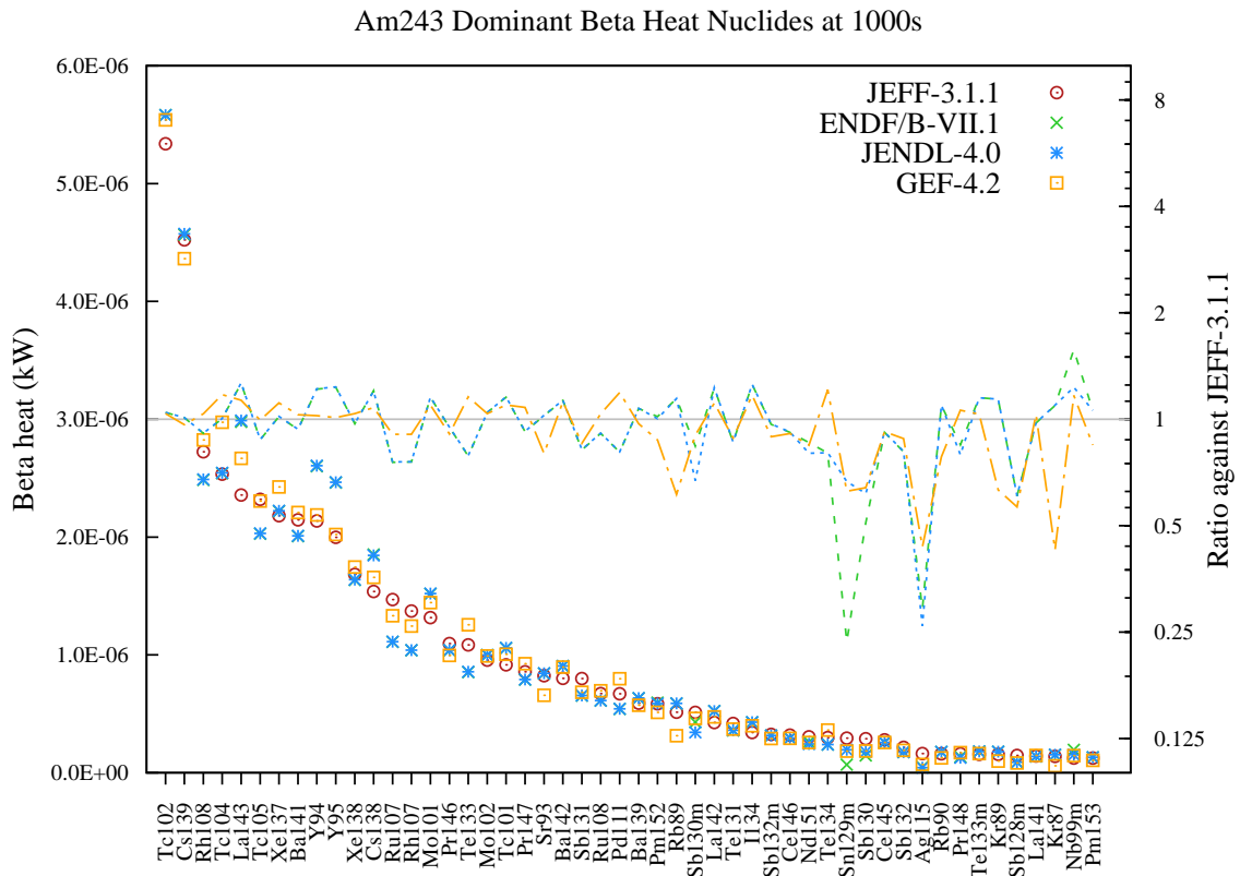
Figure 188: Beta decay heat (in kW) fission yield comparison for Am243 fission pulse after 1000s cooling.
