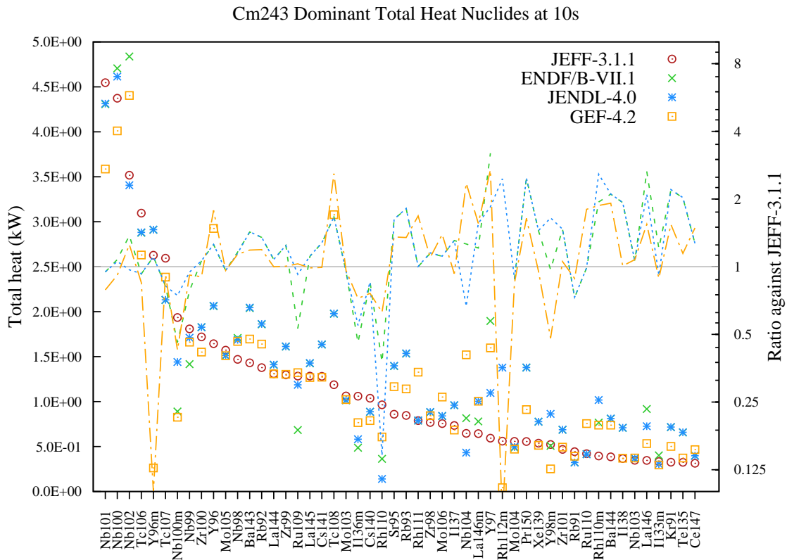
Figure 198: Total decay heat (in kW) fission yield comparison for Cm243 fission pulse after 10s cooling.
