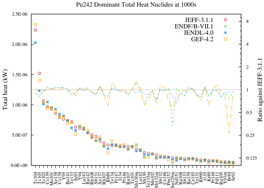
Figure 144: Total decay heat (in kW) fission yield comparison for Pu242 fission pulse after 1000s cooling.
