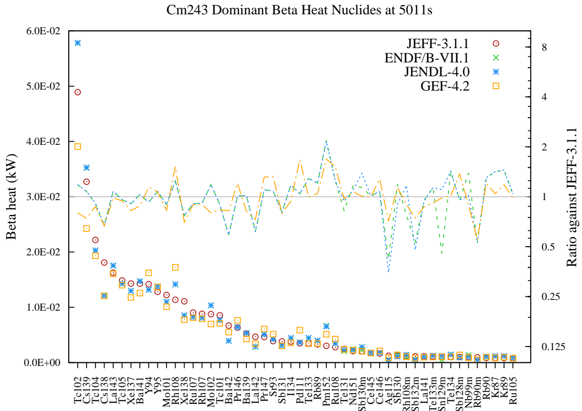
Figure 206: Beta decay heat (in kW) fission yield comparison for Cm243 fission pulse after 5011s cooling.
