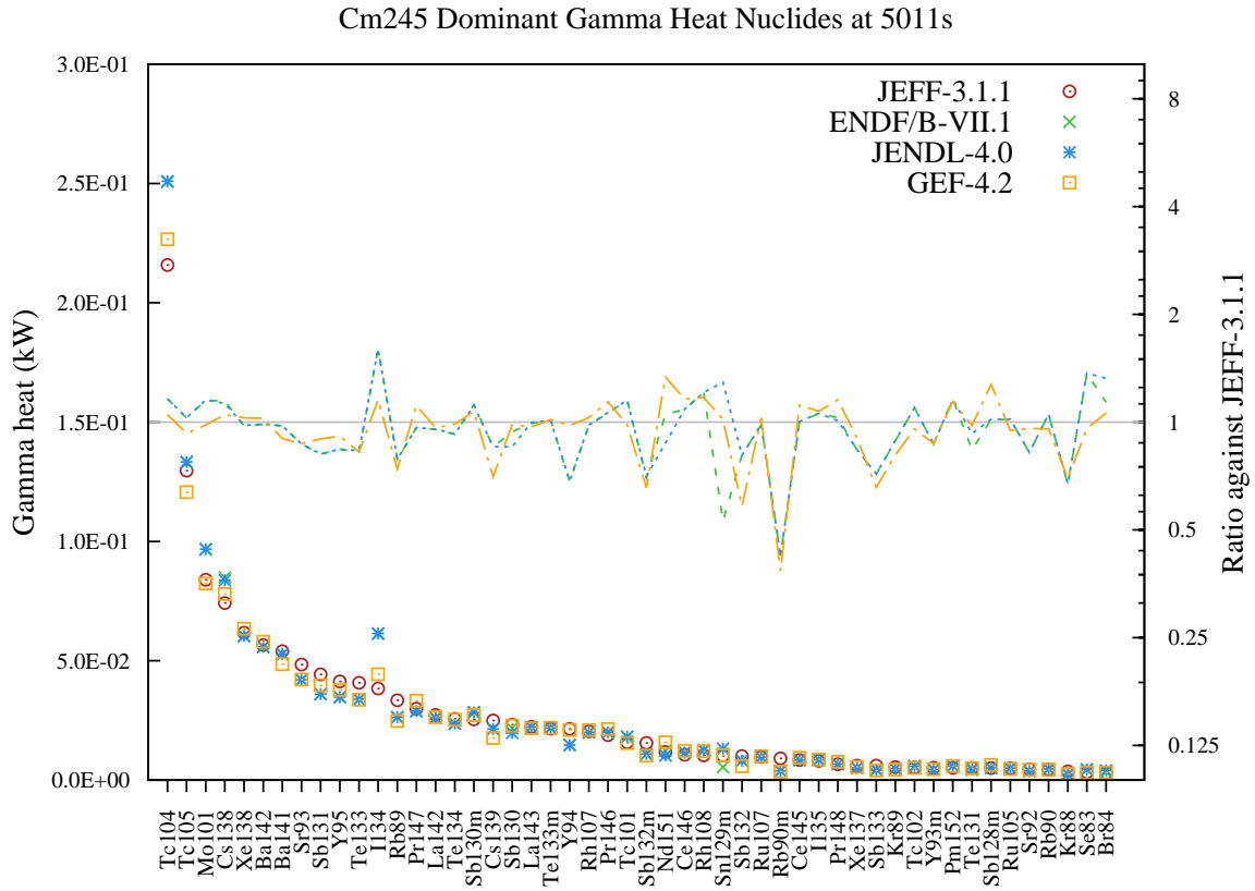
Figure 220: Gamma decay heat (in kW) fission yield comparison for Cm245 fission pulse after 5011s cooling.
