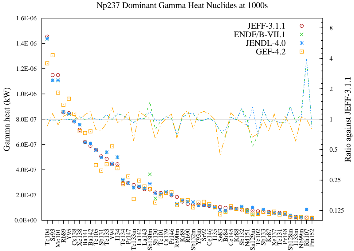
Figure 67: Gamma decay heat (in kW) fission yield comparison for Np237 fission pulse after 1000s cooling.
