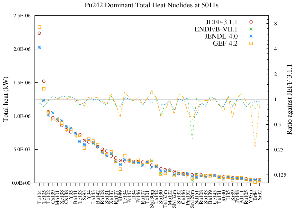
Figure 147: Total decay heat (in kW) fission yield comparison for Pu242 fission pulse after 5011s cooling.
