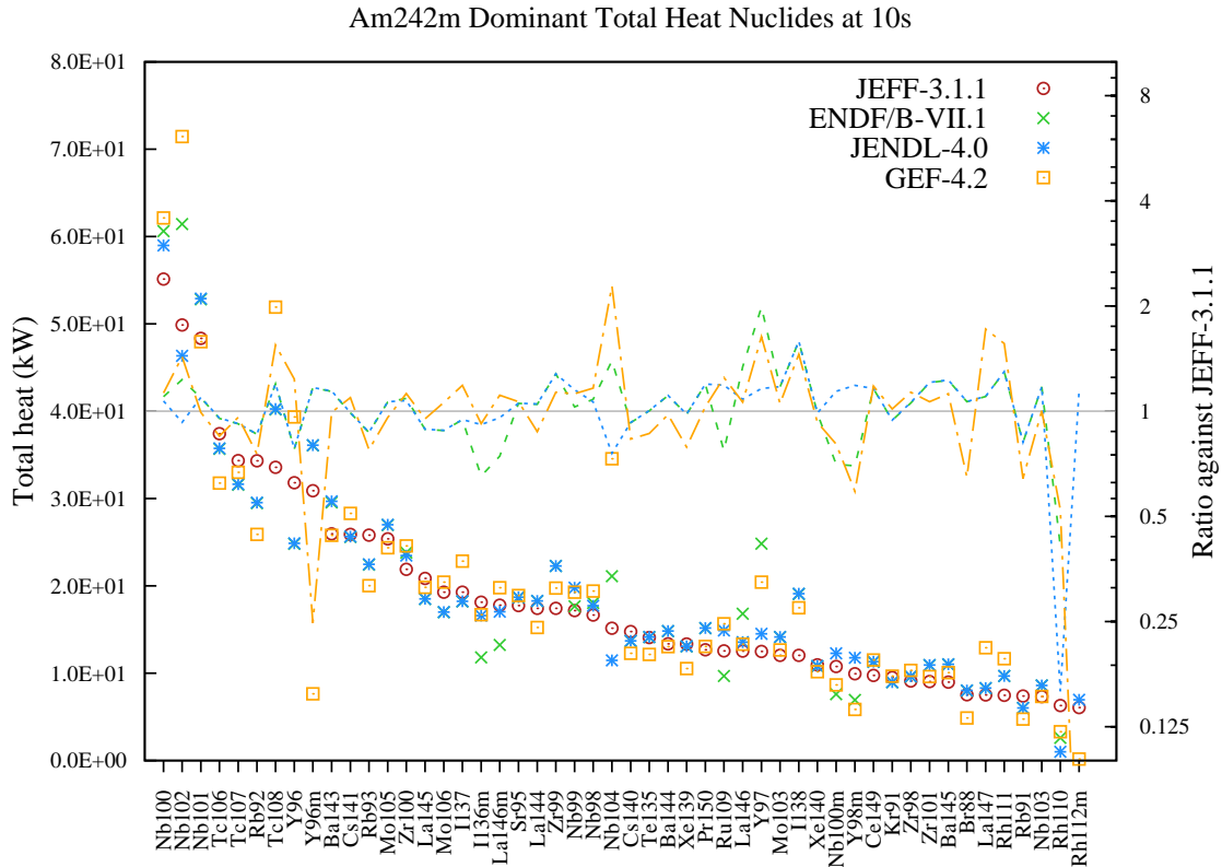
Figure 168: Total decay heat (in kW) fission yield comparison for Am242m fission pulse after 10s cooling.
