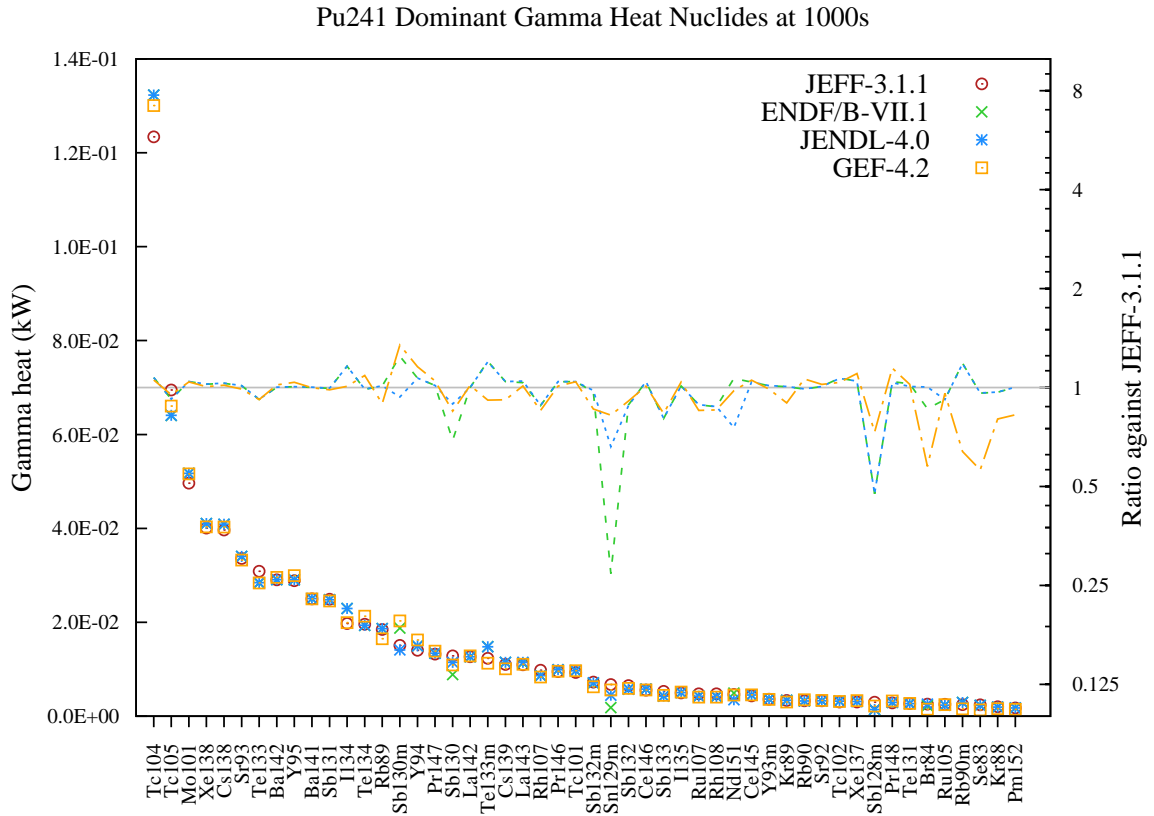
Figure 127: Gamma decay heat (in kW) fission yield comparison for Pu241 fission pulse after 1000s cooling.
