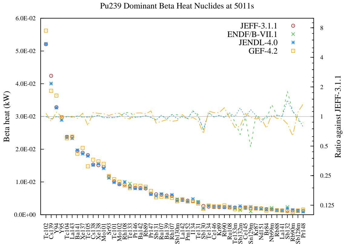
Figure 101: Beta decay heat (in kW) fission yield comparison for Pu239 fission pulse after 5011s cooling.
