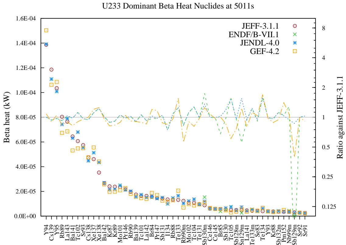
Figure 26: Beta decay heat (in kW) fission yield comparison for U233 fission pulse after 5011s cooling.
