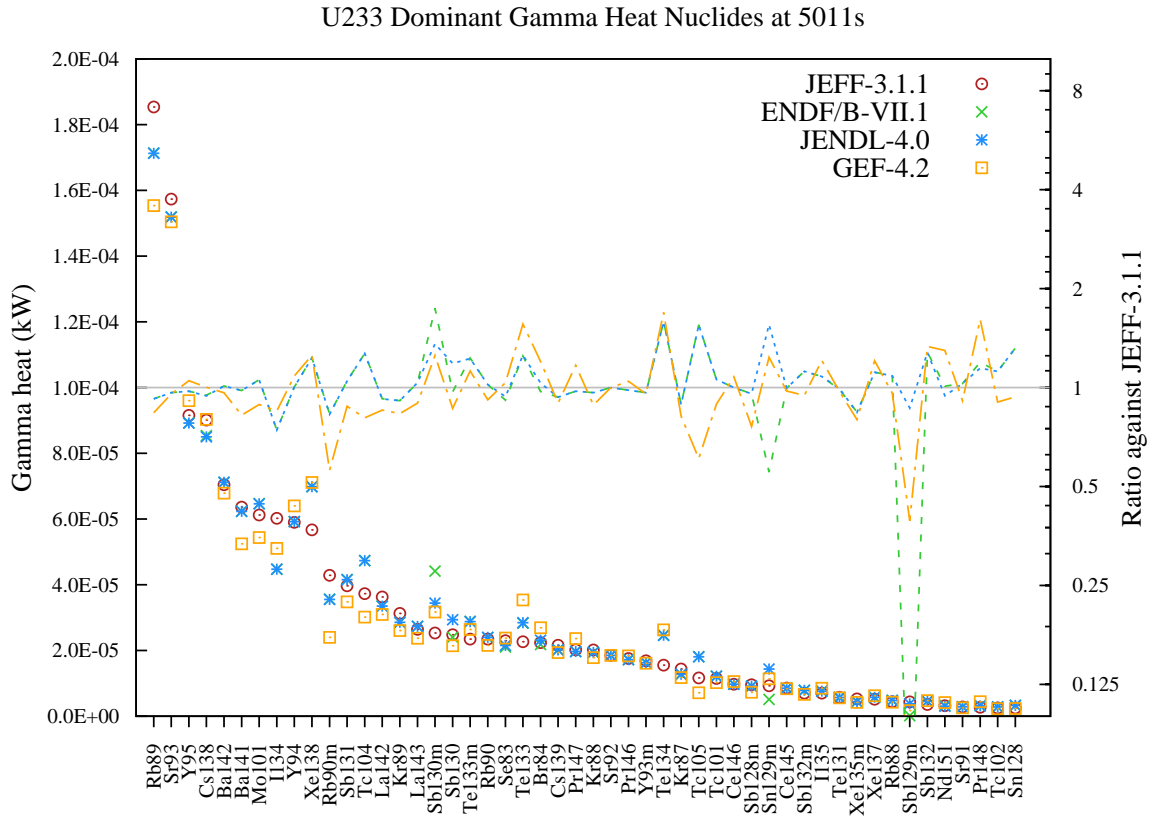
Figure 25: Gamma decay heat (in kW) fission yield comparison for U233 fission pulse after 5011s cooling.
