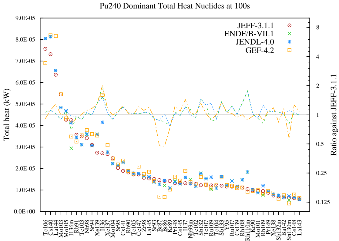
Figure 111: Total decay heat (in kW) fission yield comparison for Pu240 fission pulse after 100s cooling.
