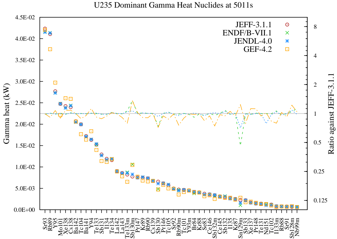
Figure 40: Gamma decay heat (in kW) fission yield comparison for U235 fission pulse after 5011s cooling.
