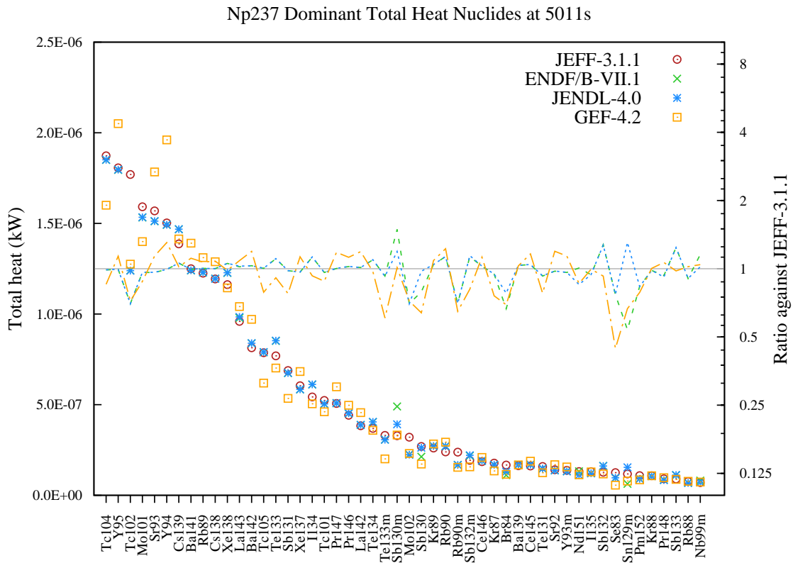
Figure 72: Total decay heat (in kW) fission yield comparison for Np237 fission pulse after 5011s cooling.
