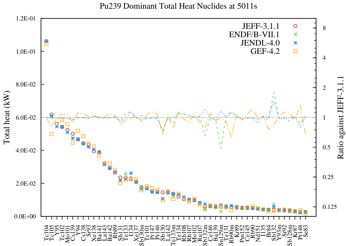
Figure 102: Total decay heat (in kW) fission yield comparison for Pu239 fission pulse after 5011s cooling.
