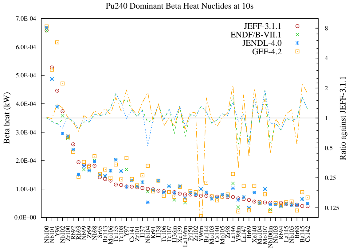
Figure 107: Beta decay heat (in kW) fission yield comparison for Pu240 fission pulse after 10s cooling.
