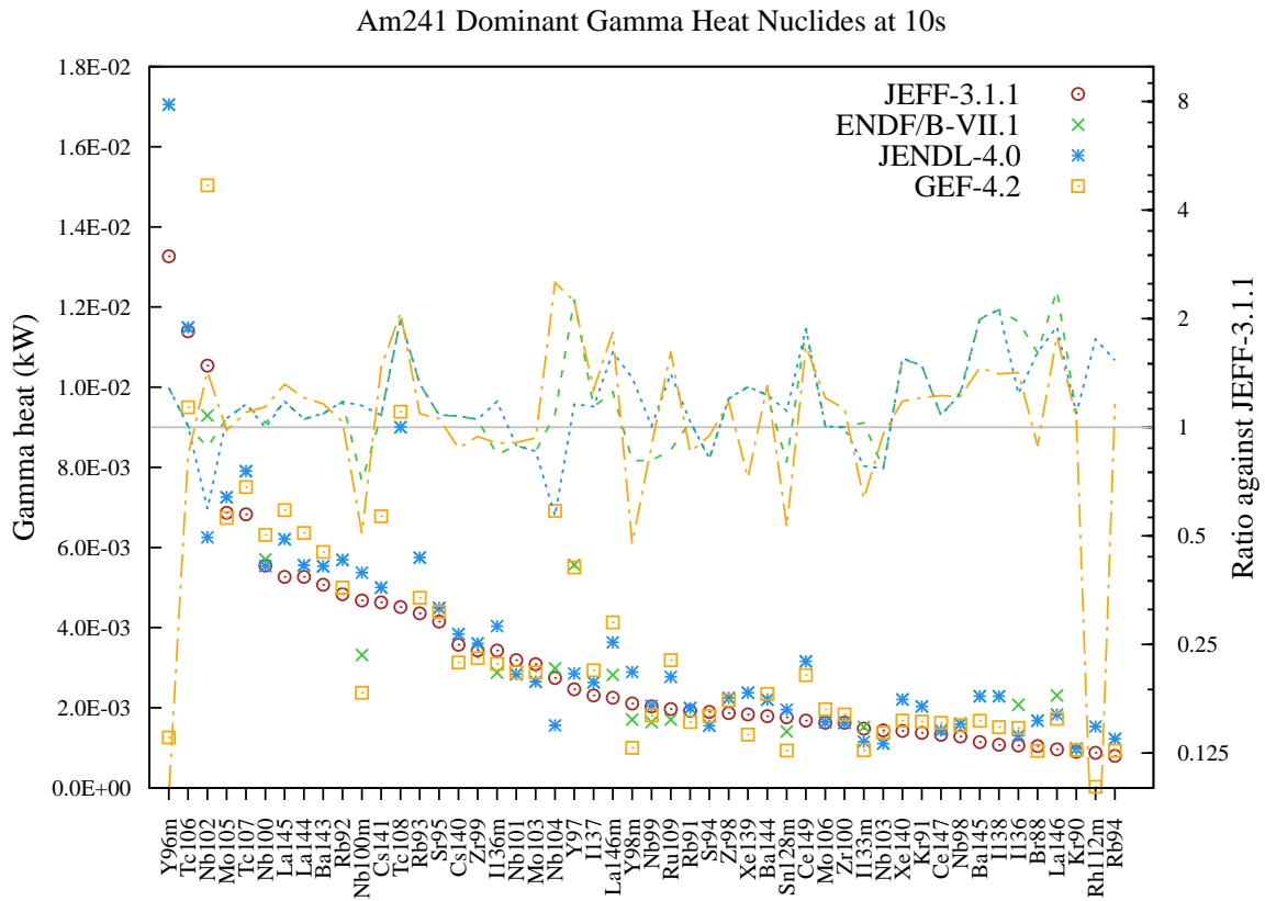
Figure 151: Gamma decay heat (in kW) fission yield comparison for Am241 fission pulse after 10s cooling.
