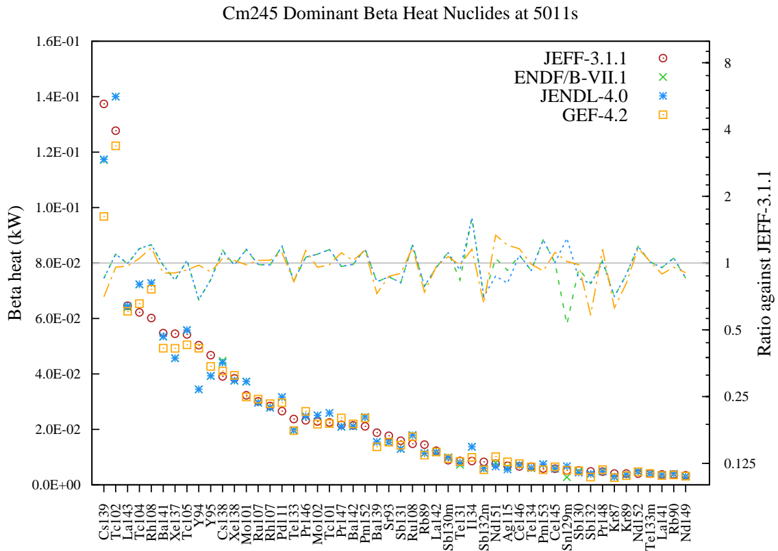
Figure 221: Beta decay heat (in kW) fission yield comparison for Cm245 fission pulse after 5011s cooling.
