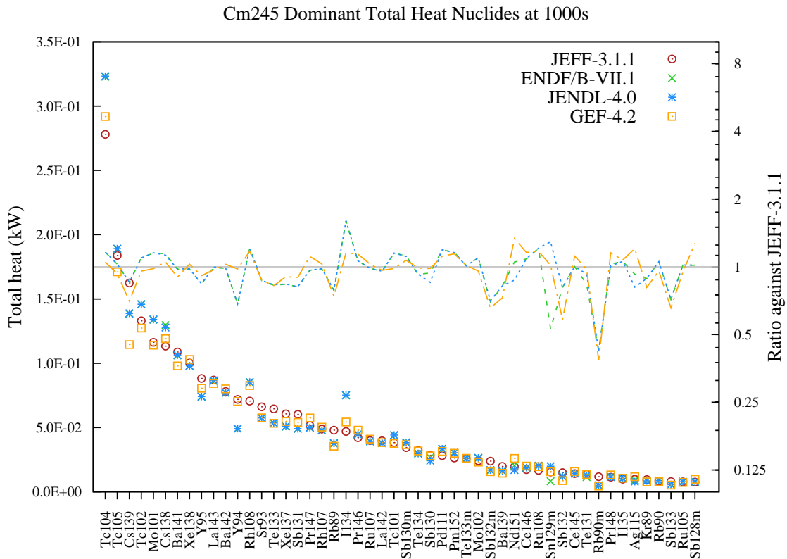
Figure 219: Total decay heat (in kW) fission yield comparison for Cm245 fission pulse after 1000s cooling.
