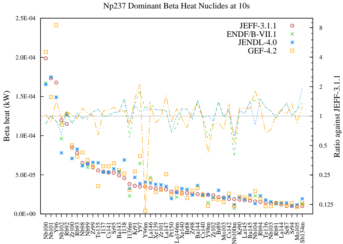
Figure 62: Beta decay heat (in kW) fission yield comparison for Np237 fission pulse after 10s cooling.
