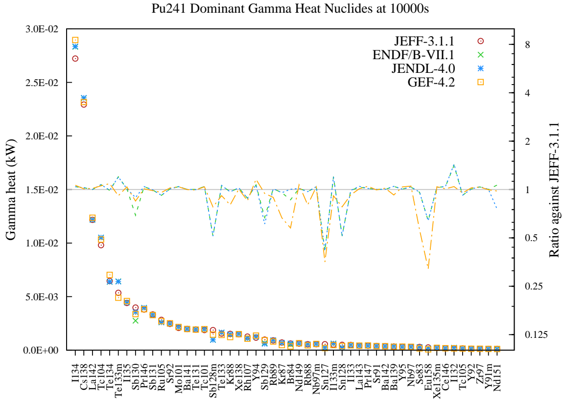
Figure 133: Gamma decay heat (in kW) fission yield comparison for Pu241 fission pulse after 10000s cooling.
