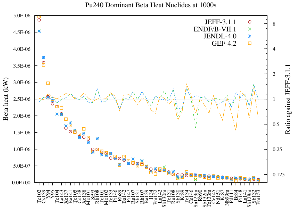
Figure 113: Beta decay heat (in kW) fission yield comparison for Pu240 fission pulse after 1000s cooling.
