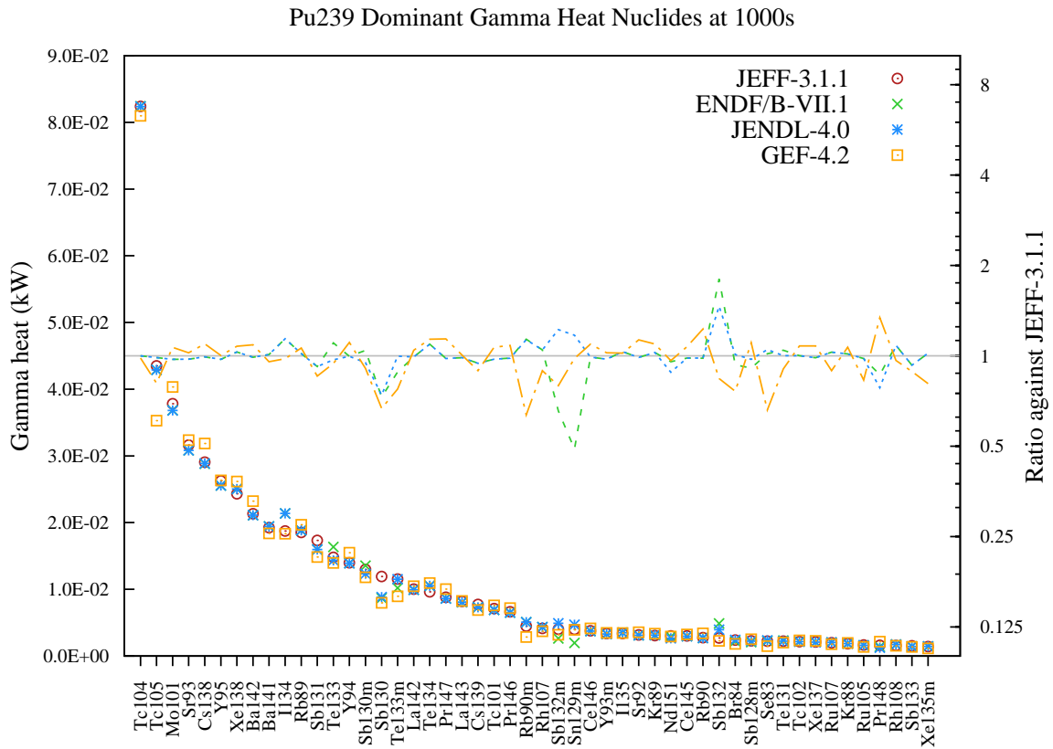
Figure 97: Gamma decay heat (in kW) fission yield comparison for Pu239 fission pulse after 1000s cooling.
