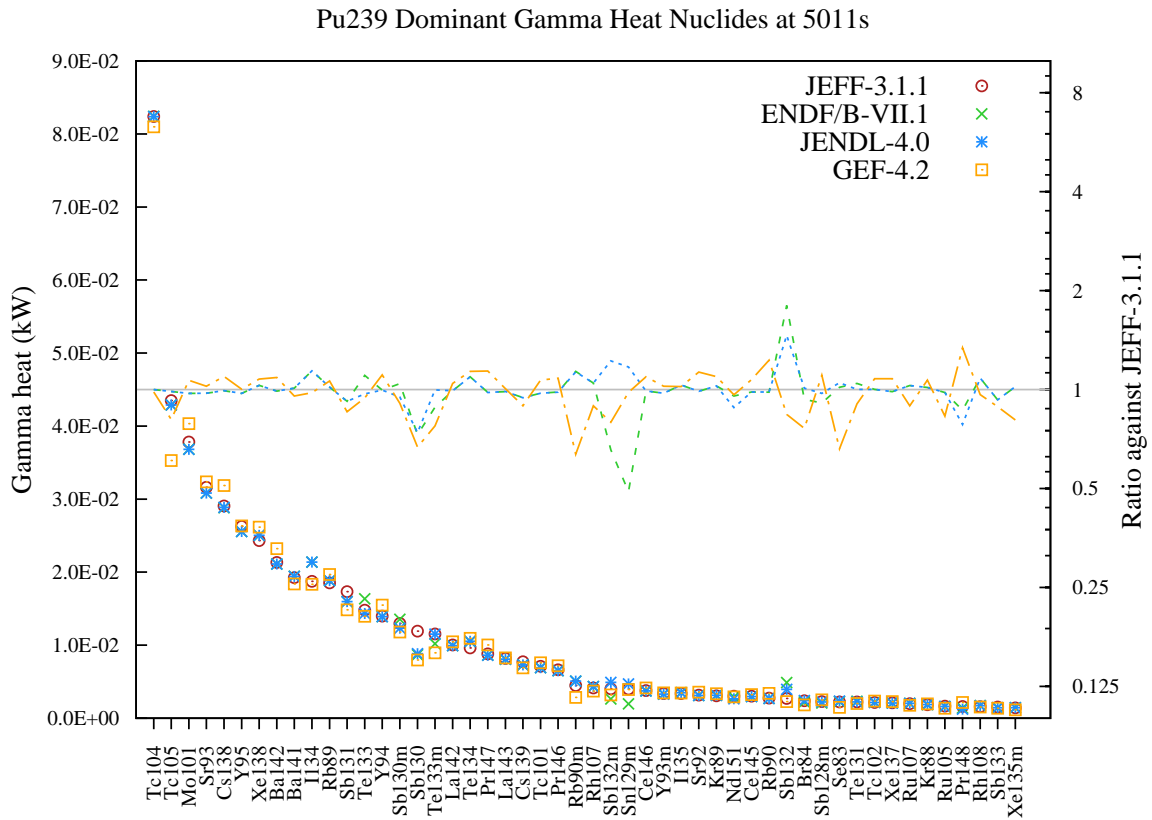
Figure 100: Gamma decay heat (in kW) fission yield comparison for Pu239 fission pulse after 5011s cooling.
