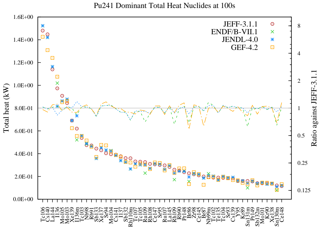
Figure 126: Total decay heat (in kW) fission yield comparison for Pu241 fission pulse after 100s cooling.
