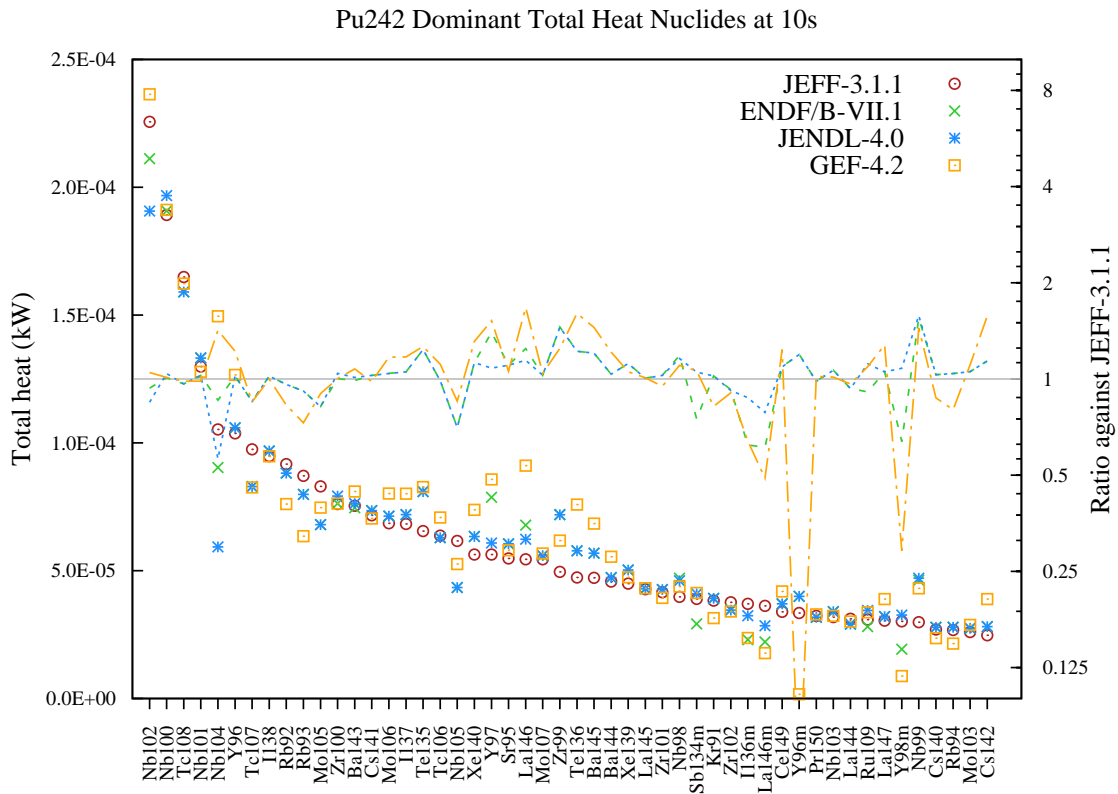
Figure 138: Total decay heat (in kW) fission yield comparison for Pu242 fission pulse after 10s cooling.
