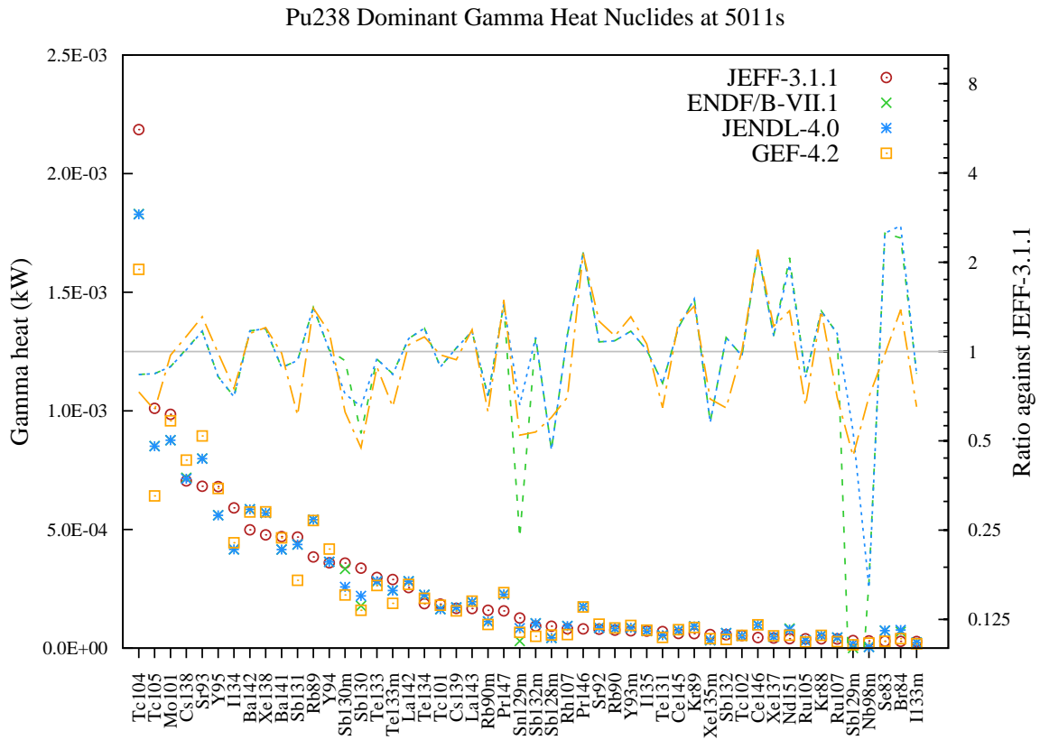
Figure 85: Gamma decay heat (in kW) fission yield comparison for Pu238 fission pulse after 5011s cooling.
