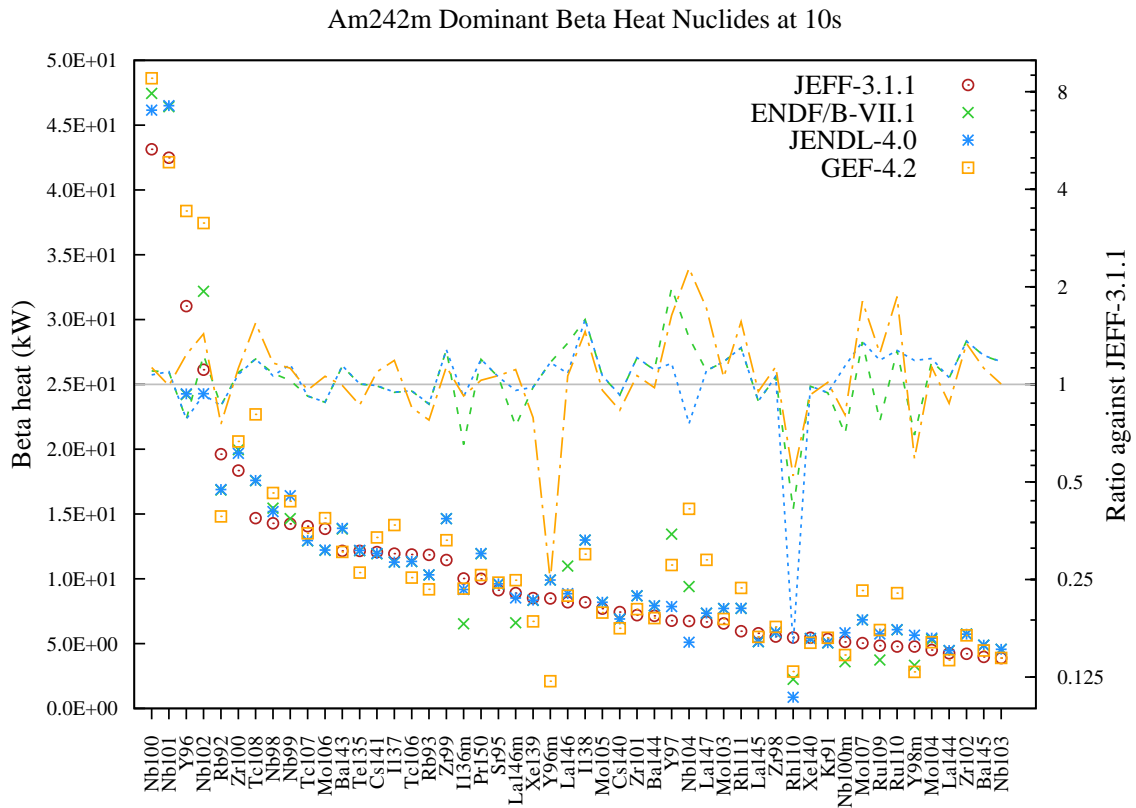
Figure 167: Beta decay heat (in kW) fission yield comparison for Am242m fission pulse after 10s cooling.
