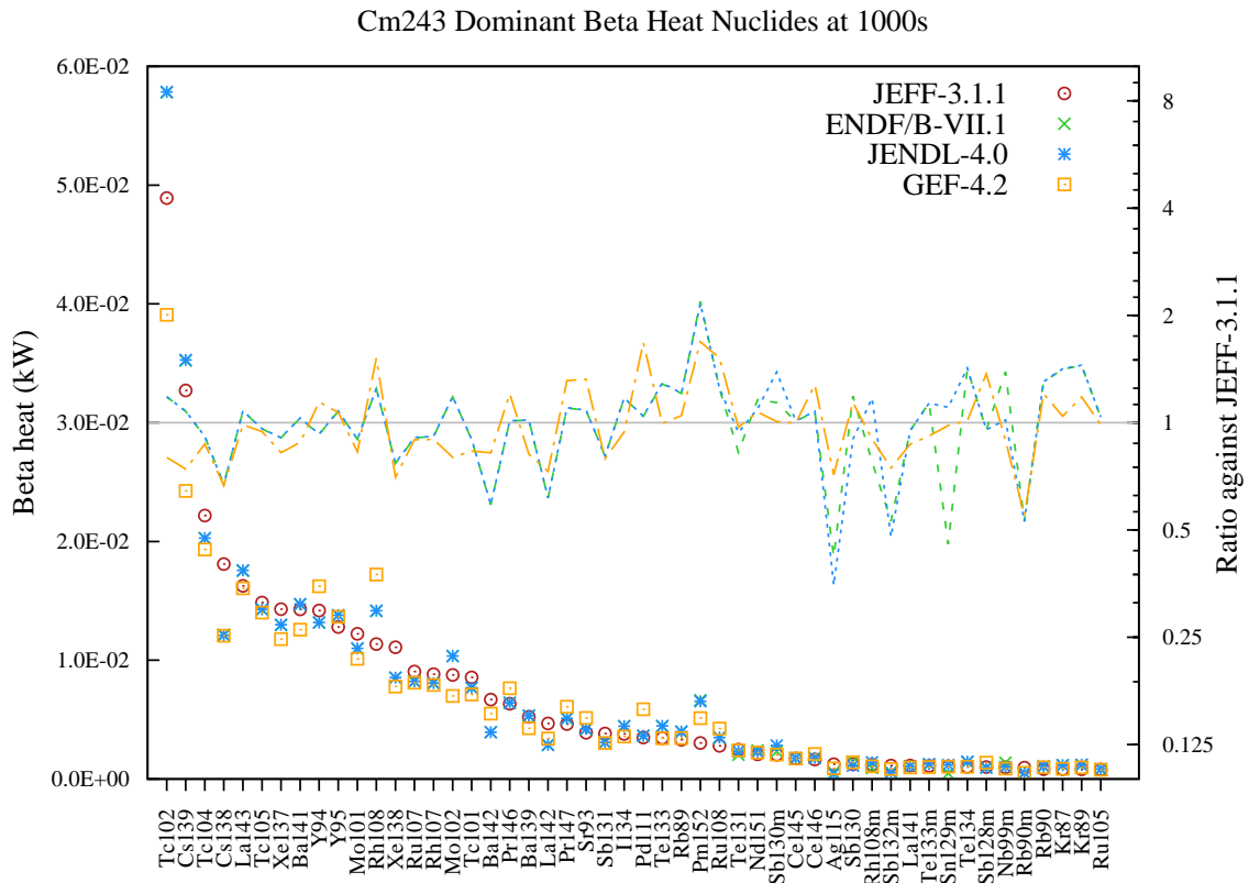
Figure 203: Beta decay heat (in kW) fission yield comparison for Cm243 fission pulse after 1000s cooling.
