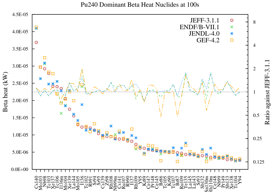
Figure 110: Beta decay heat (in kW) fission yield comparison for Pu240 fission pulse after 100s cooling.
