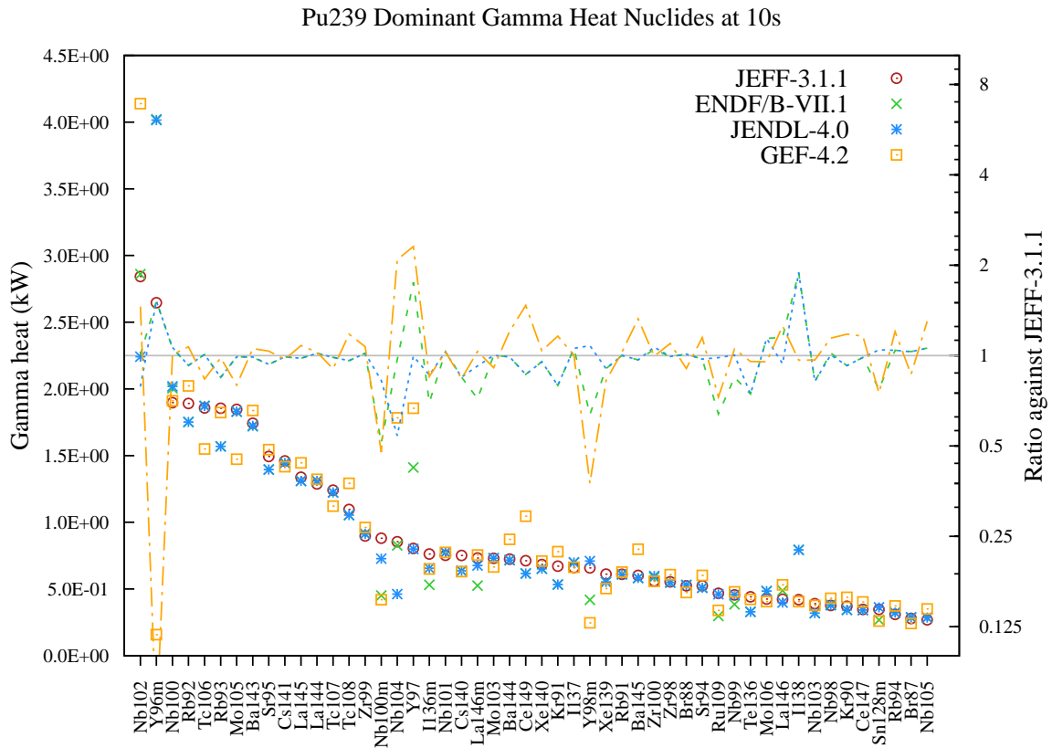
Figure 91: Gamma decay heat (in kW) fission yield comparison for Pu239 fission pulse after 10s cooling.
