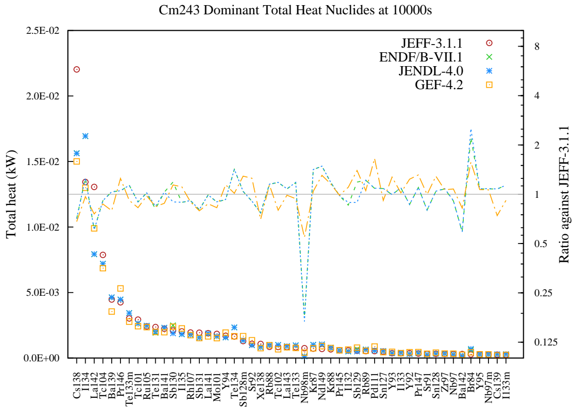
Figure 210: Total decay heat (in kW) fission yield comparison for Cm243 fission pulse after 10000s cooling.
