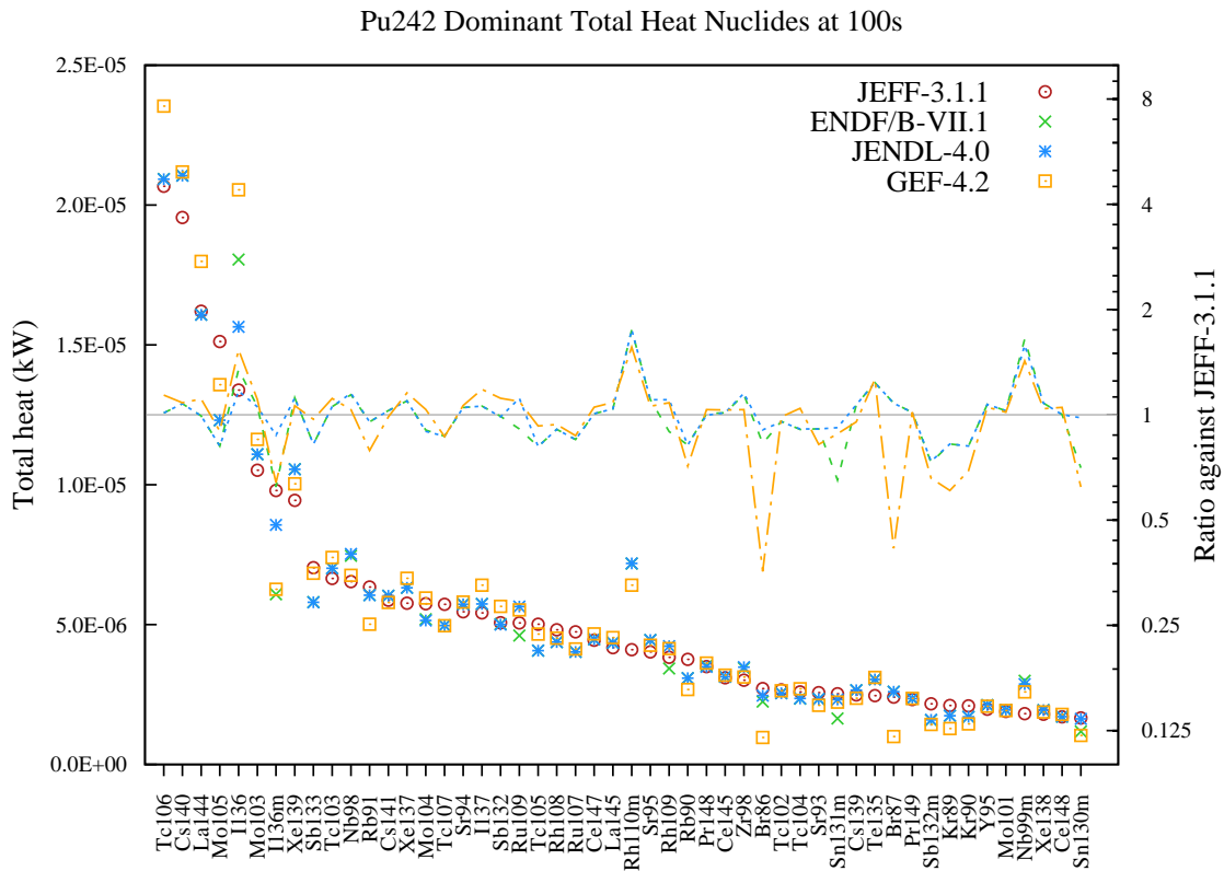
Figure 141: Total decay heat (in kW) fission yield comparison for Pu242 fission pulse after 100s cooling.
