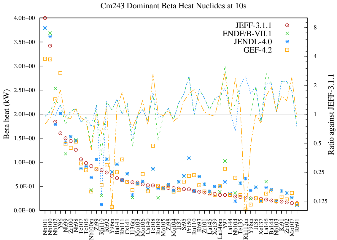
Figure 197: Beta decay heat (in kW) fission yield comparison for Cm243 fission pulse after 10s cooling.
