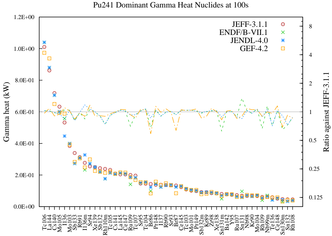
Figure 124: Gamma decay heat (in kW) fission yield comparison for Pu241 fission pulse after 100s cooling.
