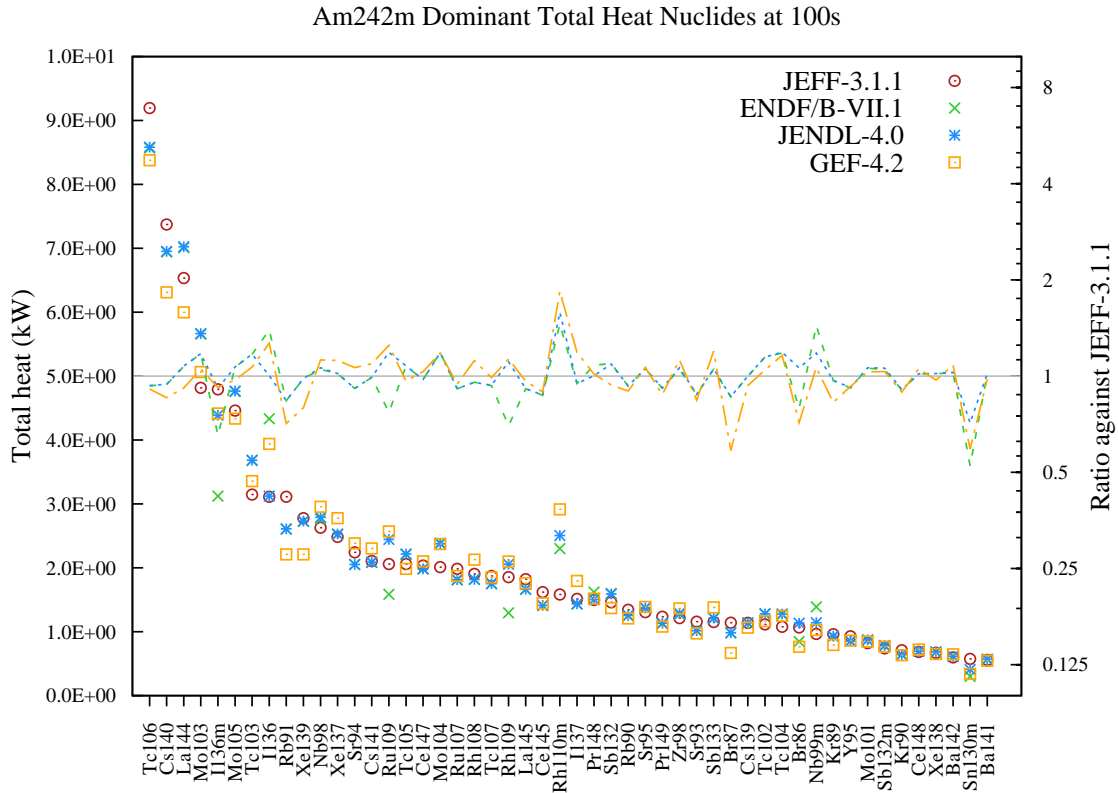
Figure 171: Total decay heat (in kW) fission yield comparison for Am242m fission pulse after 100s cooling.
