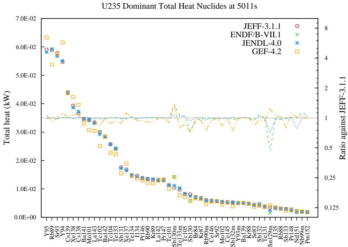
Figure 42: Total decay heat (in kW) fission yield comparison for U235 fission pulse after 5011s cooling.
