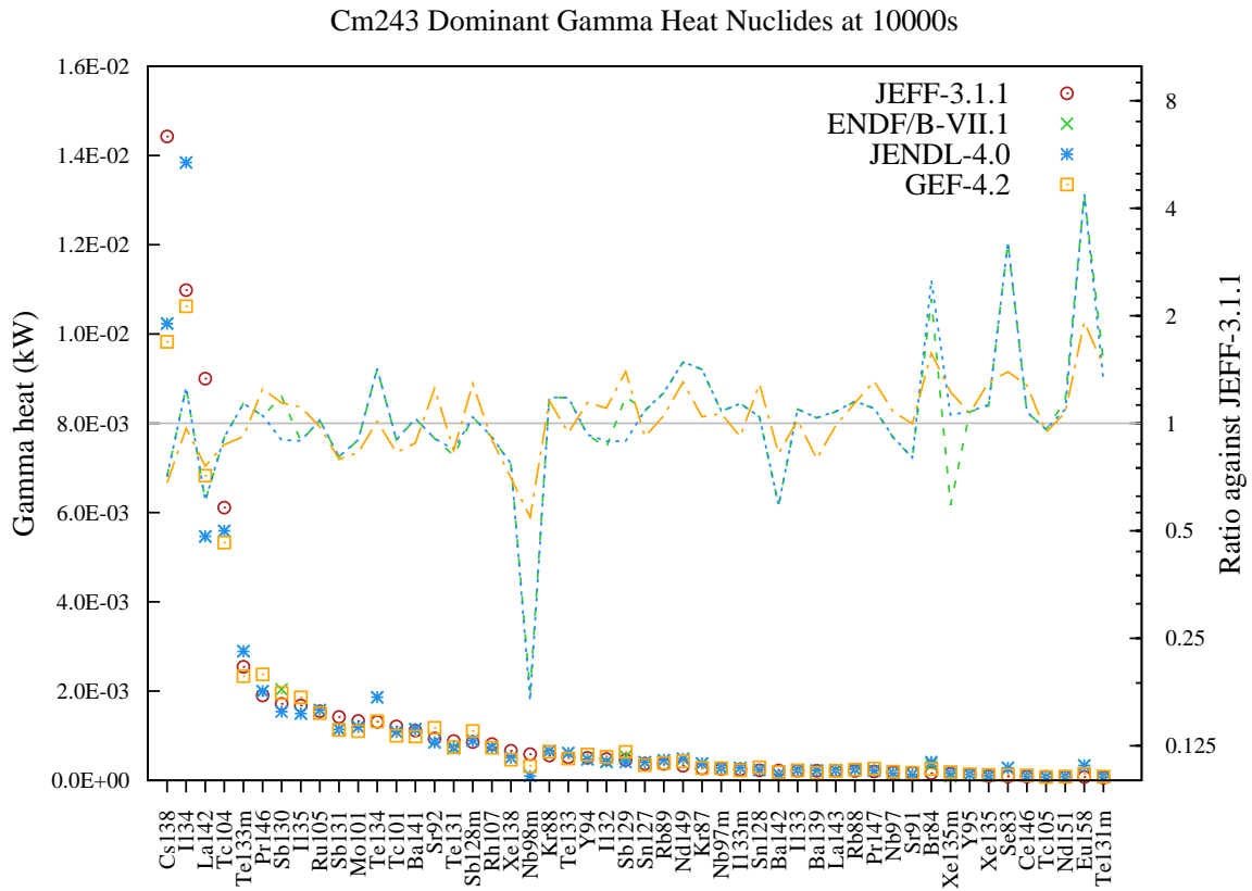
Figure 208: Gamma decay heat (in kW) fission yield comparison for Cm243 fission pulse after 10000s cooling.
