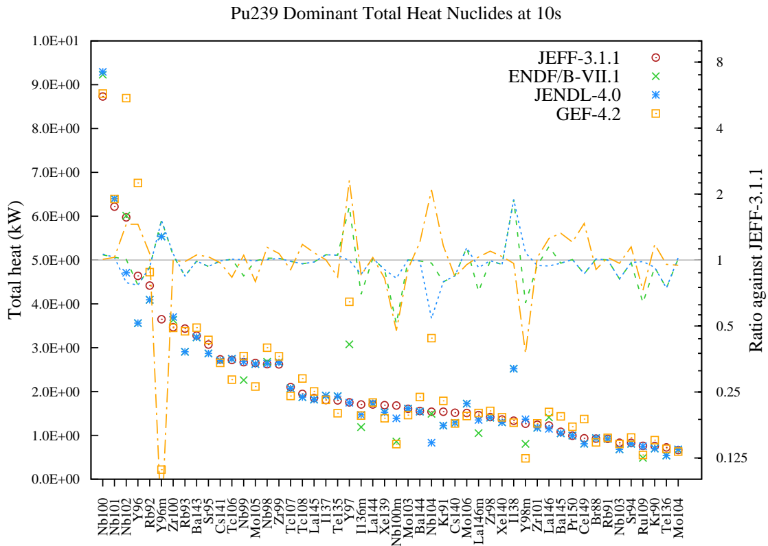
Figure 93: Total decay heat (in kW) fission yield comparison for Pu239 fission pulse after 10s cooling.
