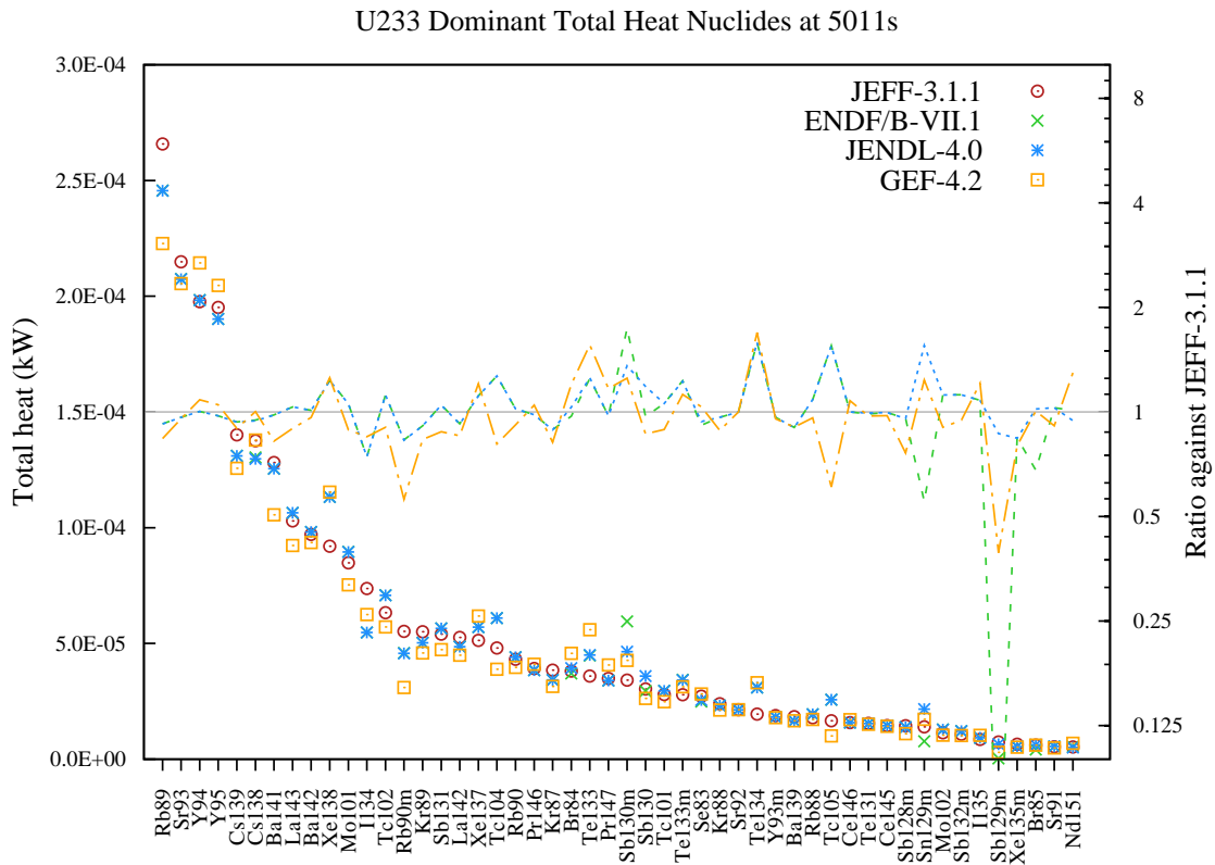
Figure 27: Total decay heat (in kW) fission yield comparison for U233 fission pulse after 5011s cooling.
