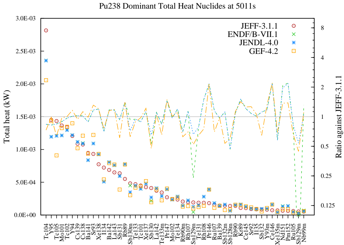
Figure 87: Total decay heat (in kW) fission yield comparison for Pu238 fission pulse after 5011s cooling.
