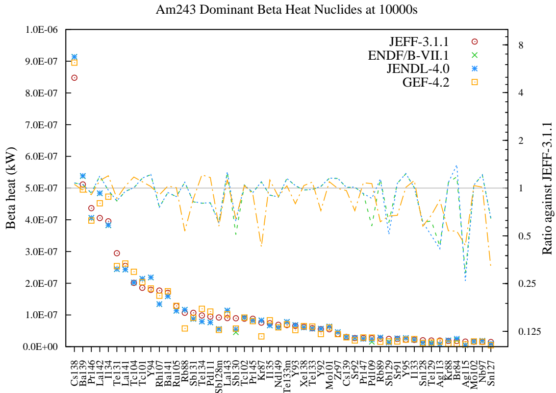
Figure 194: Beta decay heat (in kW) fission yield comparison for Am243 fission pulse after 10000s cooling.
