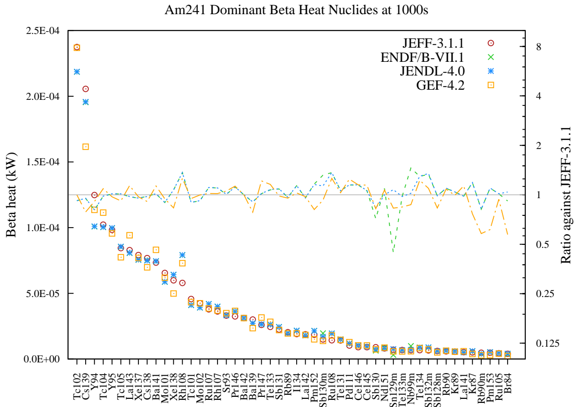
Figure 158: Beta decay heat (in kW) fission yield comparison for Am241 fission pulse after 1000s cooling.
