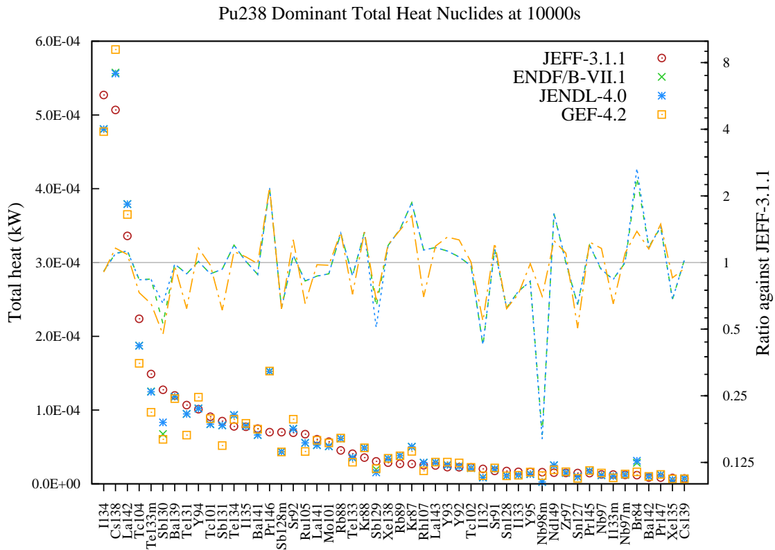
Figure 90: Total decay heat (in kW) fission yield comparison for Pu238 fission pulse after 10000s cooling.
