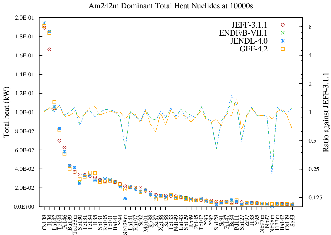
Figure 180: Total decay heat (in kW) fission yield comparison for Am242m fission pulse after 10000s cooling.
