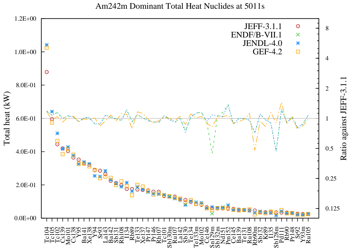
Figure 177: Total decay heat (in kW) fission yield comparison for Am242m fission pulse after 5011s cooling.
