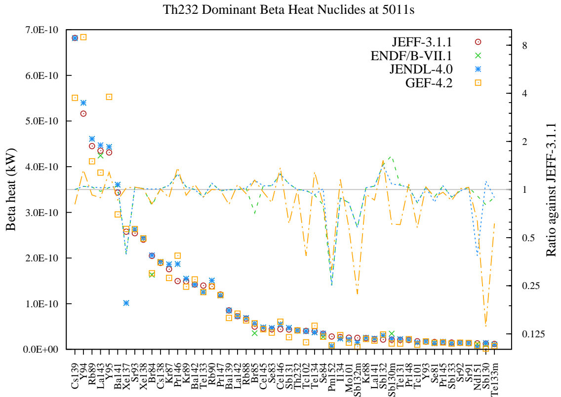
Figure 11: Beta decay heat (in kW) fission yield comparison for Th232 fission pulse after 5011s cooling.
