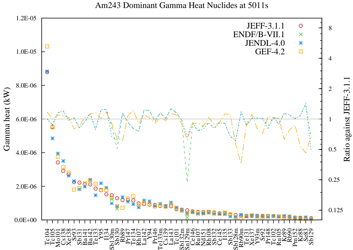
Figure 190: Gamma decay heat (in kW) fission yield comparison for Am243 fission pulse after 5011s cooling.
