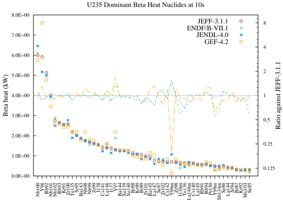
Figure 32: Beta decay heat (in kW) fission yield comparison for U235 fission pulse after 10s cooling.
