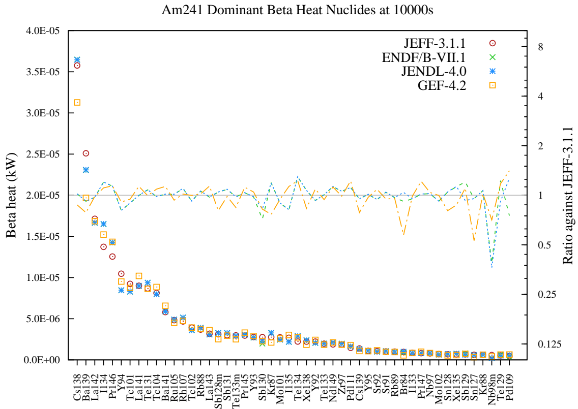
Figure 164: Beta decay heat (in kW) fission yield comparison for Am241 fission pulse after 10000s cooling.
