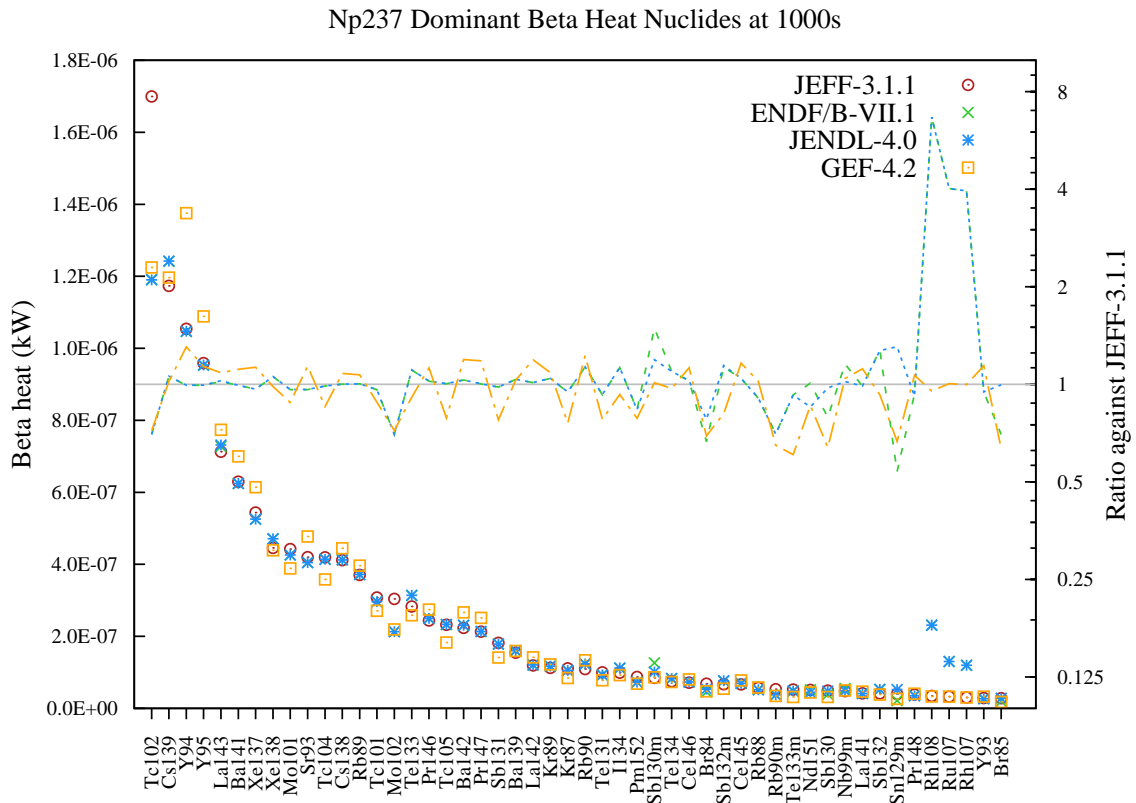
Figure 68: Beta decay heat (in kW) fission yield comparison for Np237 fission pulse after 1000s cooling.
