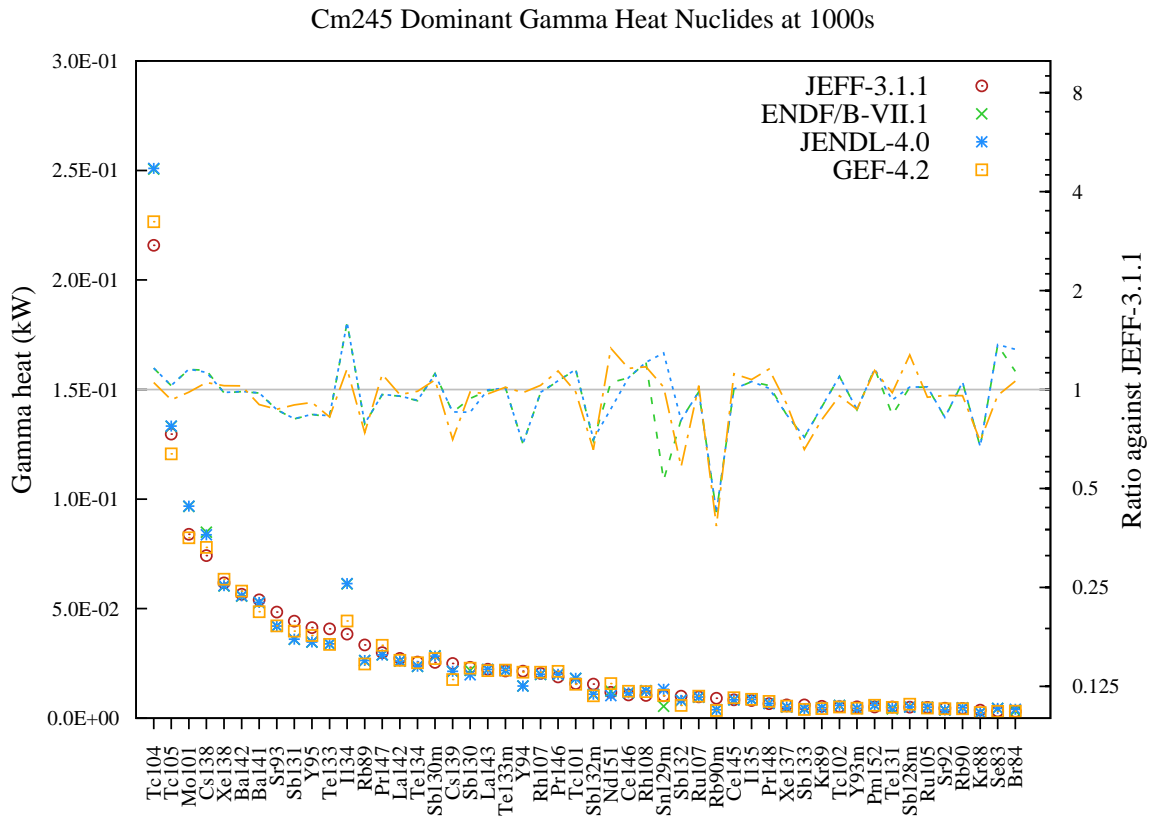
Figure 217: Gamma decay heat (in kW) fission yield comparison for Cm245 fission pulse after 1000s cooling.
