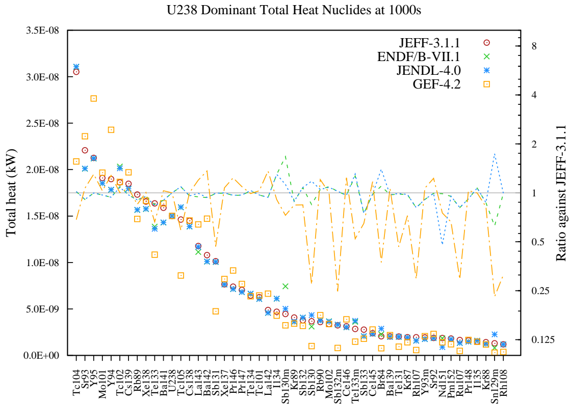
Figure 54: Total decay heat (in kW) fission yield comparison for U238 fission pulse after 1000s cooling.
