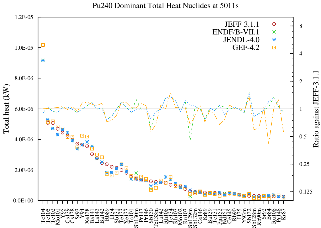
Figure 117: Total decay heat (in kW) fission yield comparison for Pu240 fission pulse after 5011s cooling.
