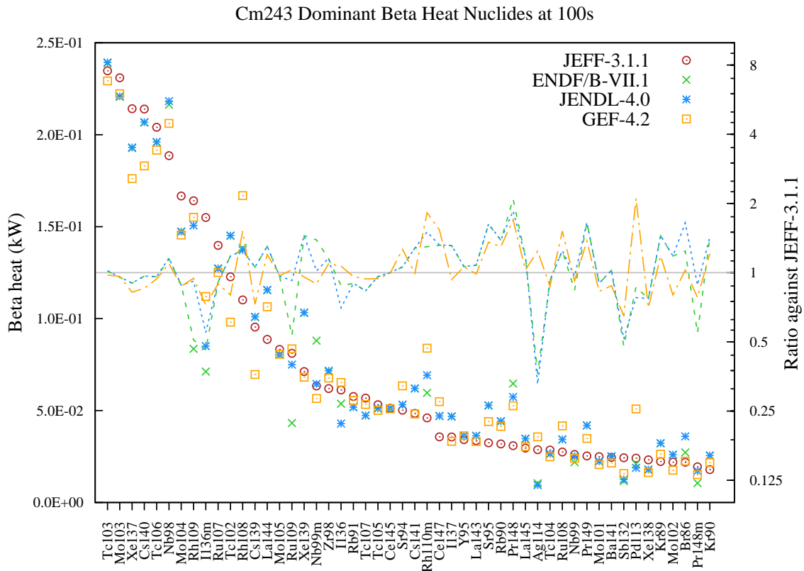
Figure 200: Beta decay heat (in kW) fission yield comparison for Cm243 fission pulse after 100s cooling.
