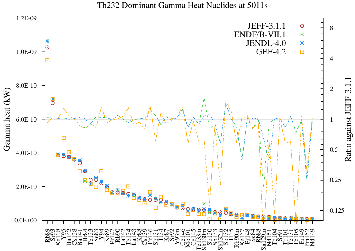
Figure 10: Gamma decay heat (in kW) fission yield comparison for Th232 fission pulse after 5011s cooling.
