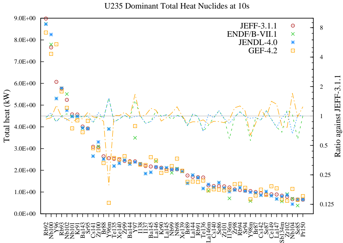
Figure 33: Total decay heat (in kW) fission yield comparison for U235 fission pulse after 10s cooling.
