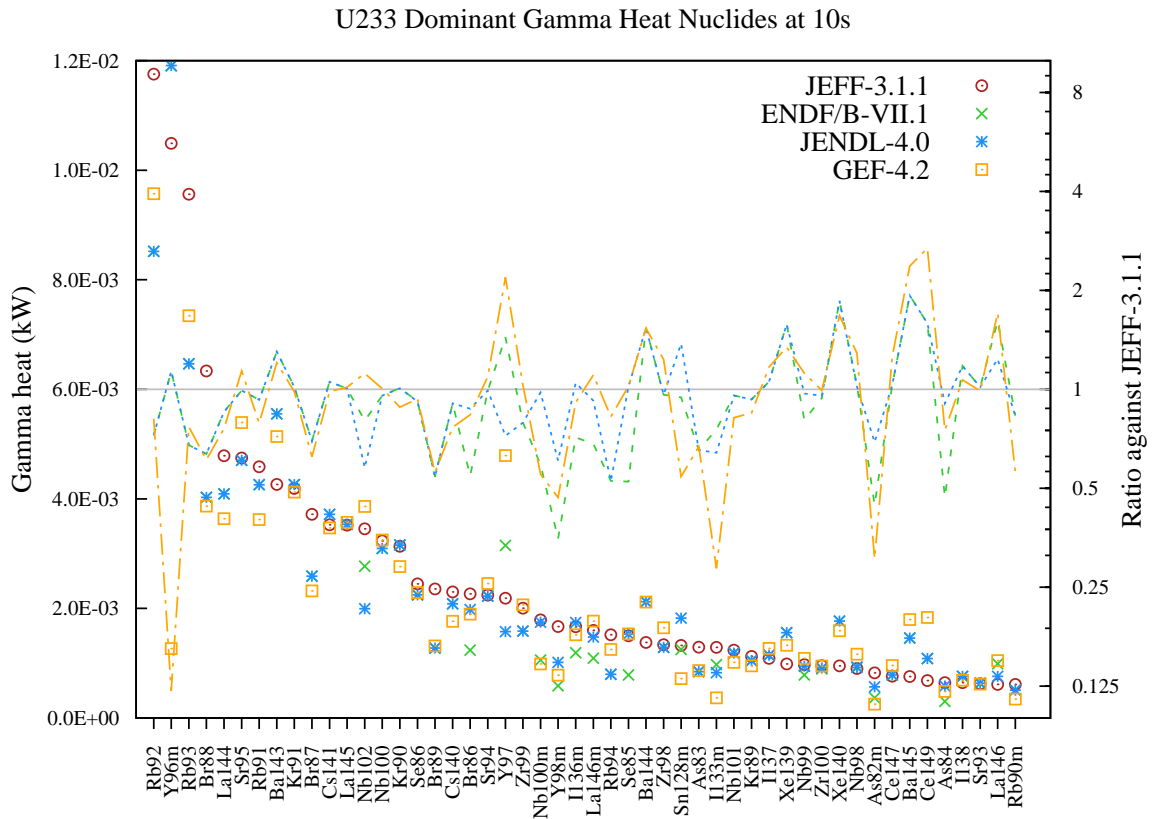
Figure 16: Gamma decay heat (in kW) fission yield comparison for U233 fission pulse after 10s cooling.
