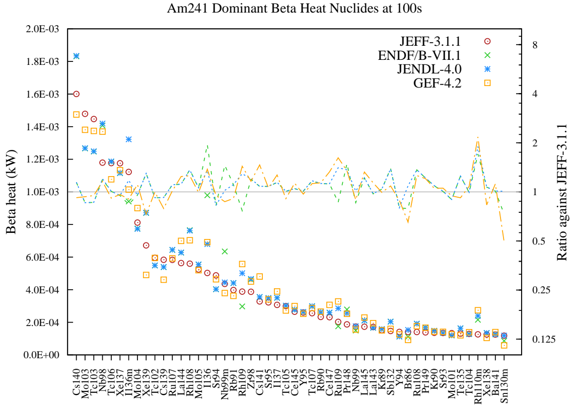
Figure 155: Beta decay heat (in kW) fission yield comparison for Am241 fission pulse after 100s cooling.
