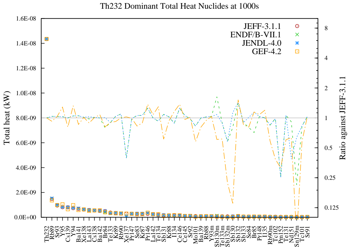
Figure 9: Total decay heat (in kW) fission yield comparison for Th232 fission pulse after 1000s cooling.
