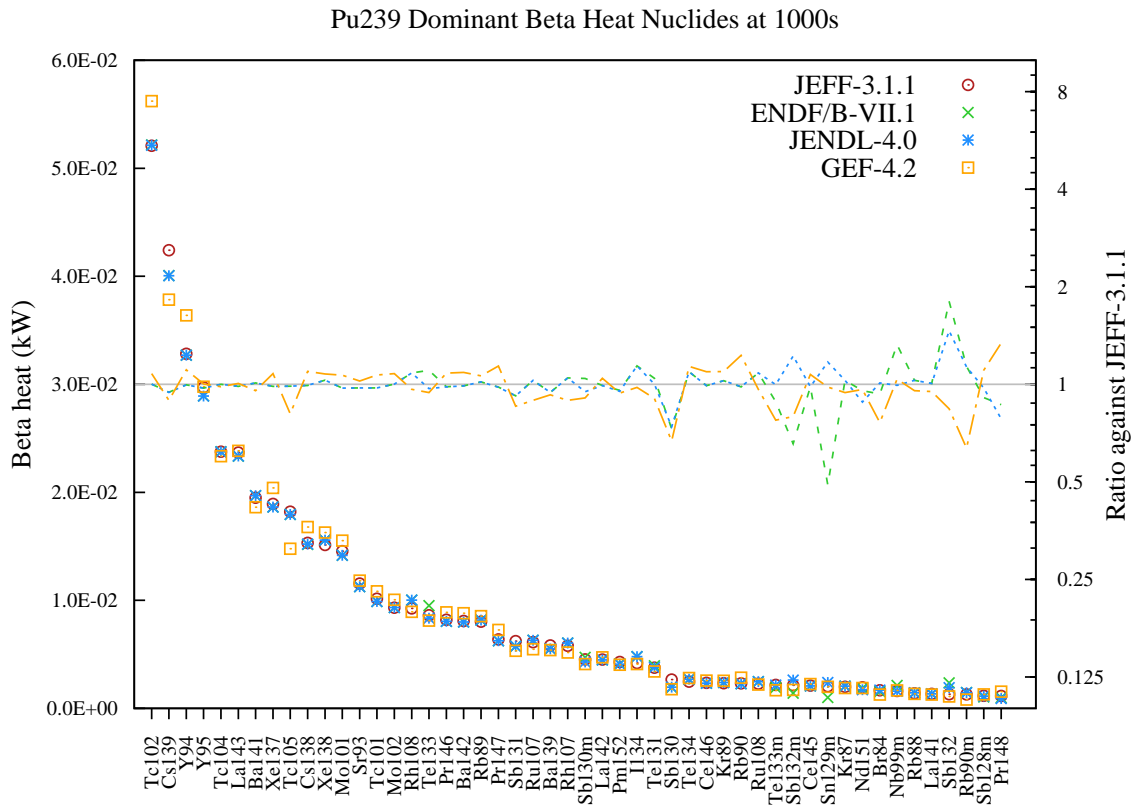
Figure 98: Beta decay heat (in kW) fission yield comparison for Pu239 fission pulse after 1000s cooling.
