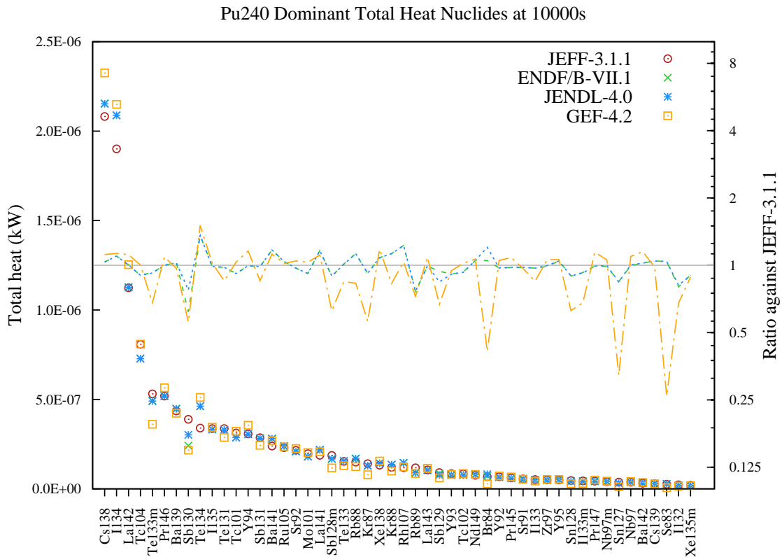
Figure 120: Total decay heat (in kW) fission yield comparison for Pu240 fission pulse after 10000s cooling.
