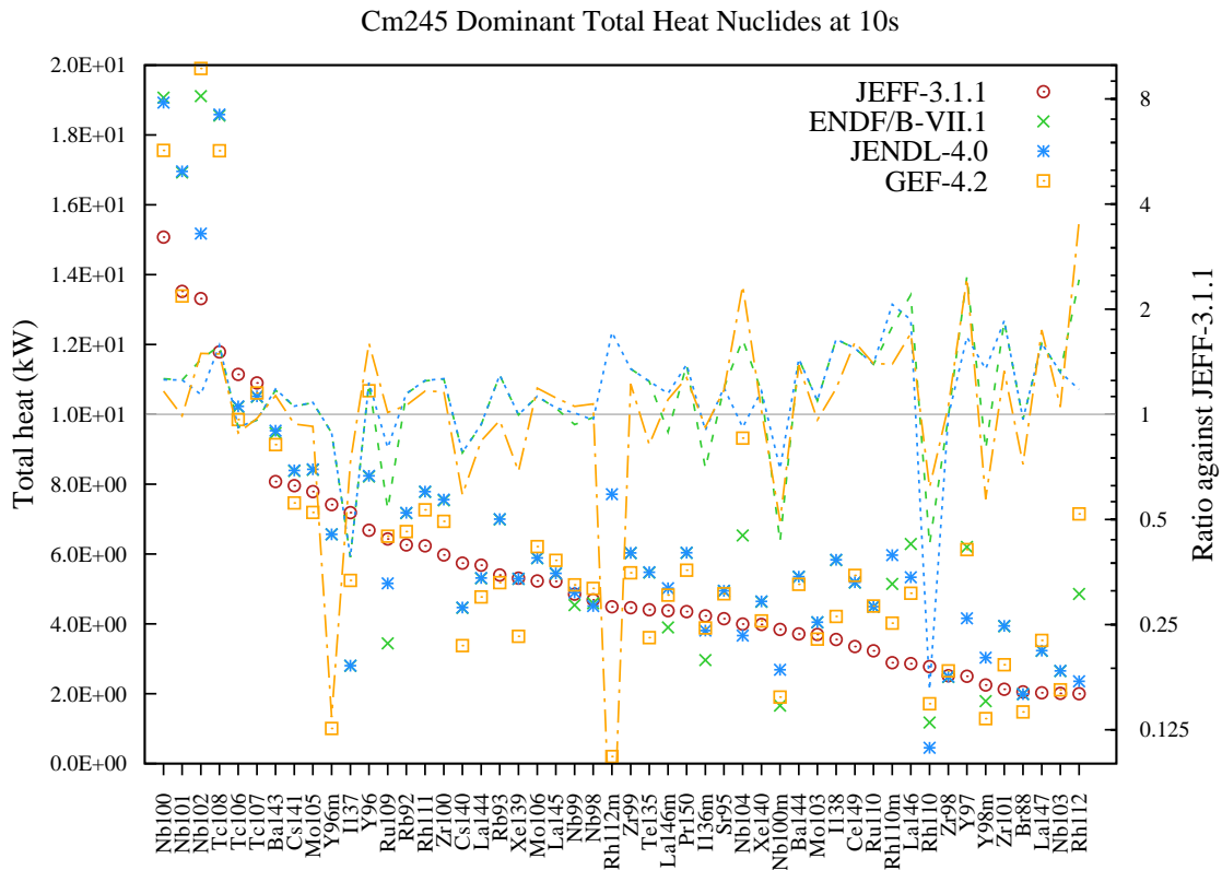
Figure 213: Total decay heat (in kW) fission yield comparison for Cm245 fission pulse after 10s cooling.
