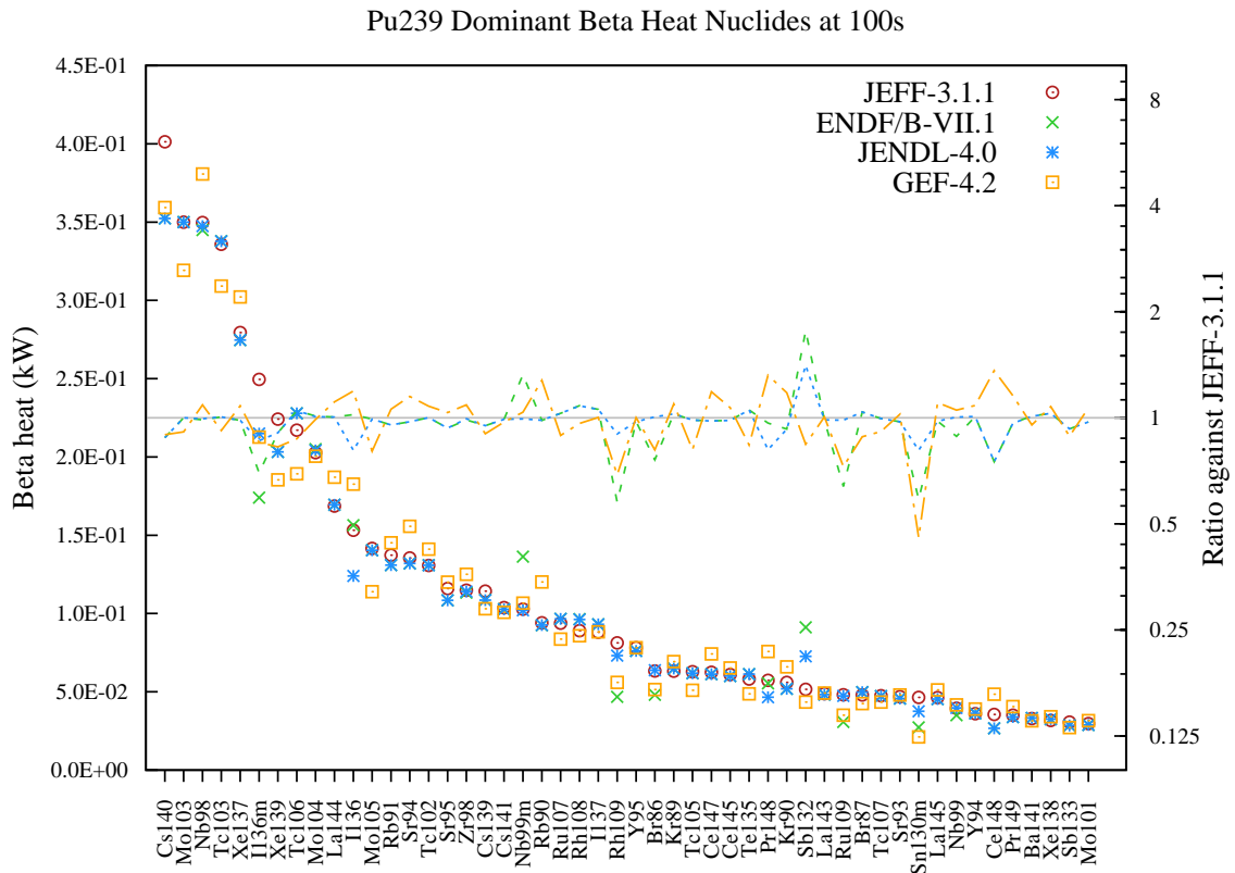
Figure 95: Beta decay heat (in kW) fission yield comparison for Pu239 fission pulse after 100s cooling.
