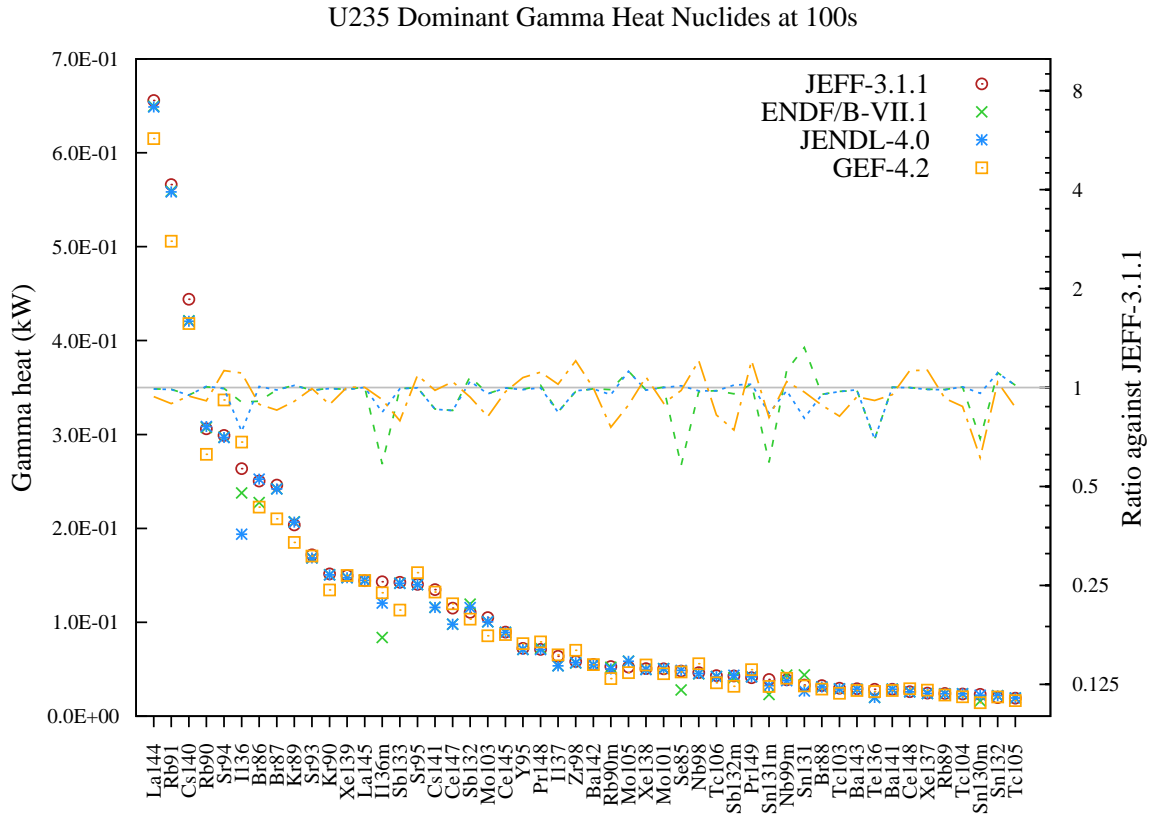
Figure 34: Gamma decay heat (in kW) fission yield comparison for U235 fission pulse after 100s cooling.
