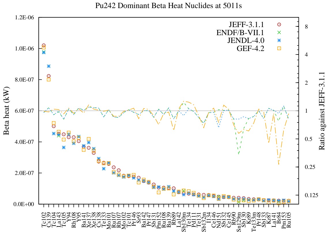
Figure 146: Beta decay heat (in kW) fission yield comparison for Pu242 fission pulse after 5011s cooling.
