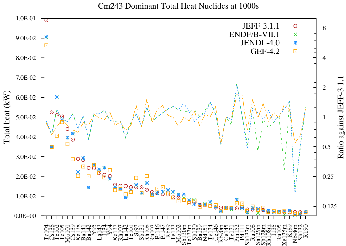
Figure 204: Total decay heat (in kW) fission yield comparison for Cm243 fission pulse after 1000s cooling.
