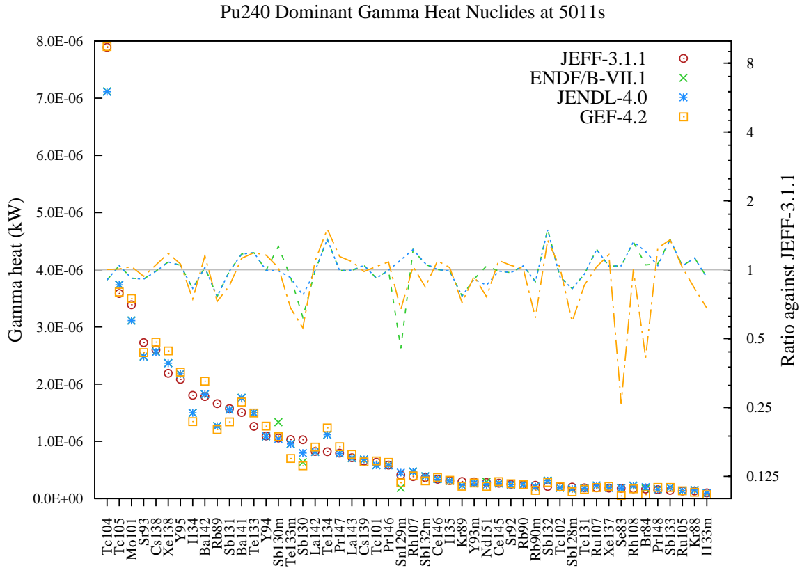
Figure 115: Gamma decay heat (in kW) fission yield comparison for Pu240 fission pulse after 5011s cooling.
