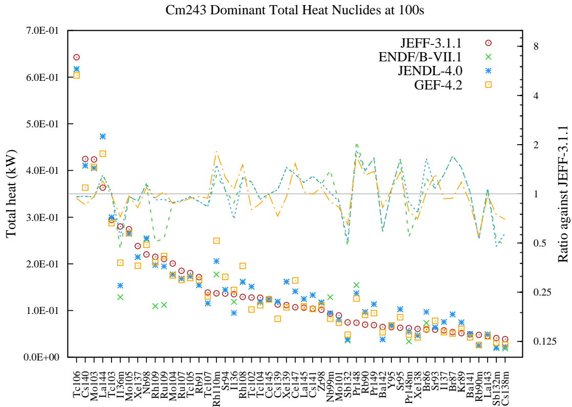
Figure 201: Total decay heat (in kW) fission yield comparison for Cm243 fission pulse after 100s cooling.
