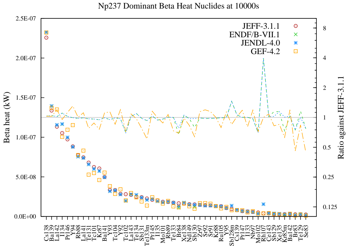
Figure 74: Beta decay heat (in kW) fission yield comparison for Np237 fission pulse after 10000s cooling.
