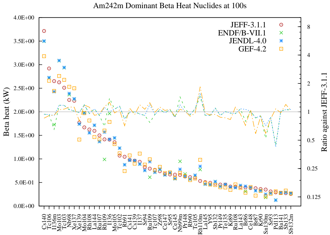
Figure 170: Beta decay heat (in kW) fission yield comparison for Am242m fission pulse after 100s cooling.
