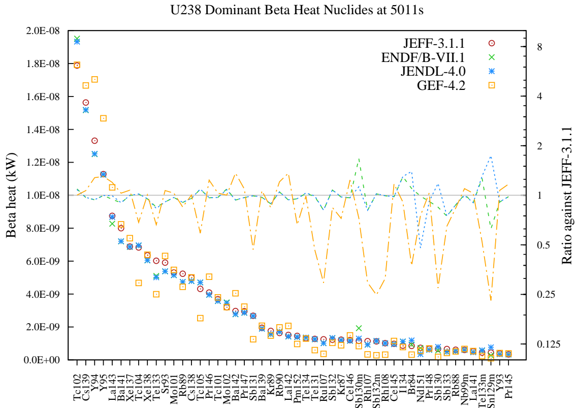
Figure 56: Beta decay heat (in kW) fission yield comparison for U238 fission pulse after 5011s cooling.
