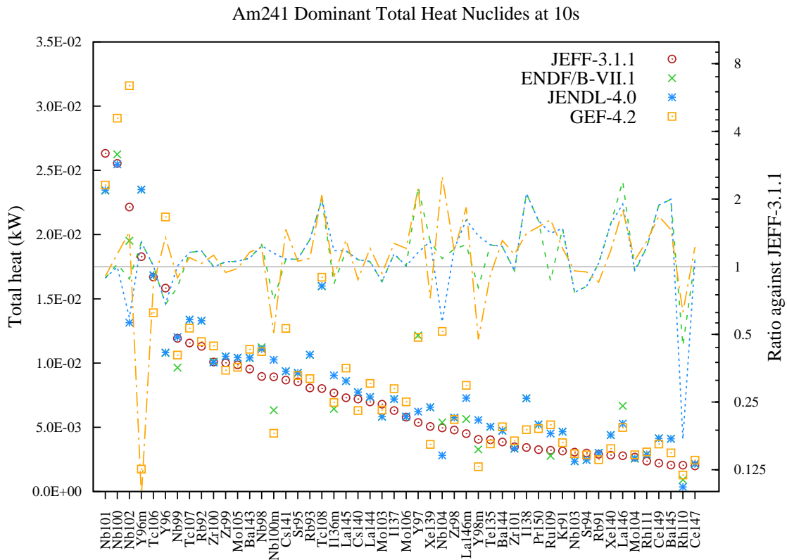
Figure 153: Total decay heat (in kW) fission yield comparison for Am241 fission pulse after 10s cooling.
