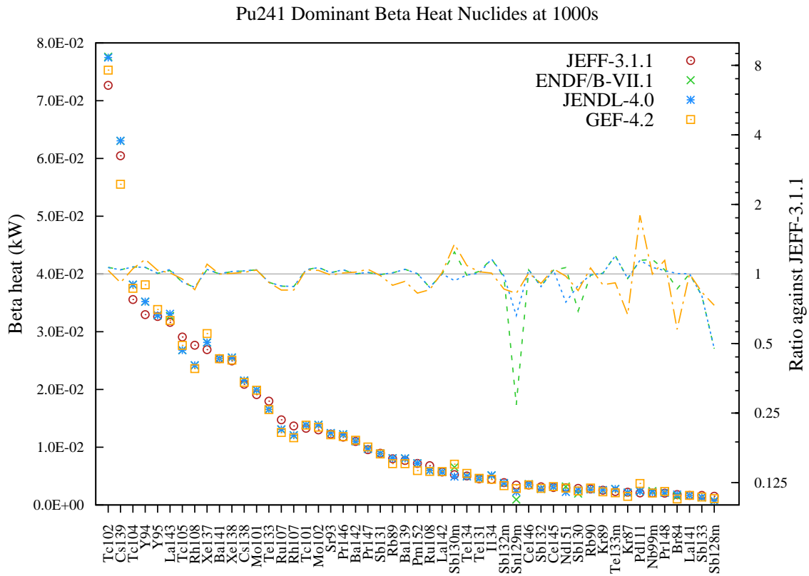
Figure 128: Beta decay heat (in kW) fission yield comparison for Pu241 fission pulse after 1000s cooling.
