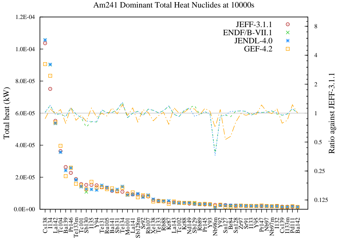
Figure 165: Total decay heat (in kW) fission yield comparison for Am241 fission pulse after 10000s cooling.
