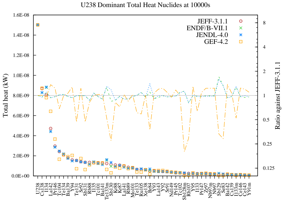
Figure 60: Total decay heat (in kW) fission yield comparison for U238 fission pulse after 10000s cooling.
