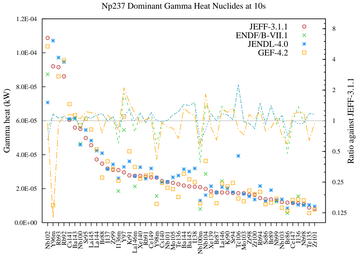
Figure 61: Gamma decay heat (in kW) fission yield comparison for Np237 fission pulse after 10s cooling.
