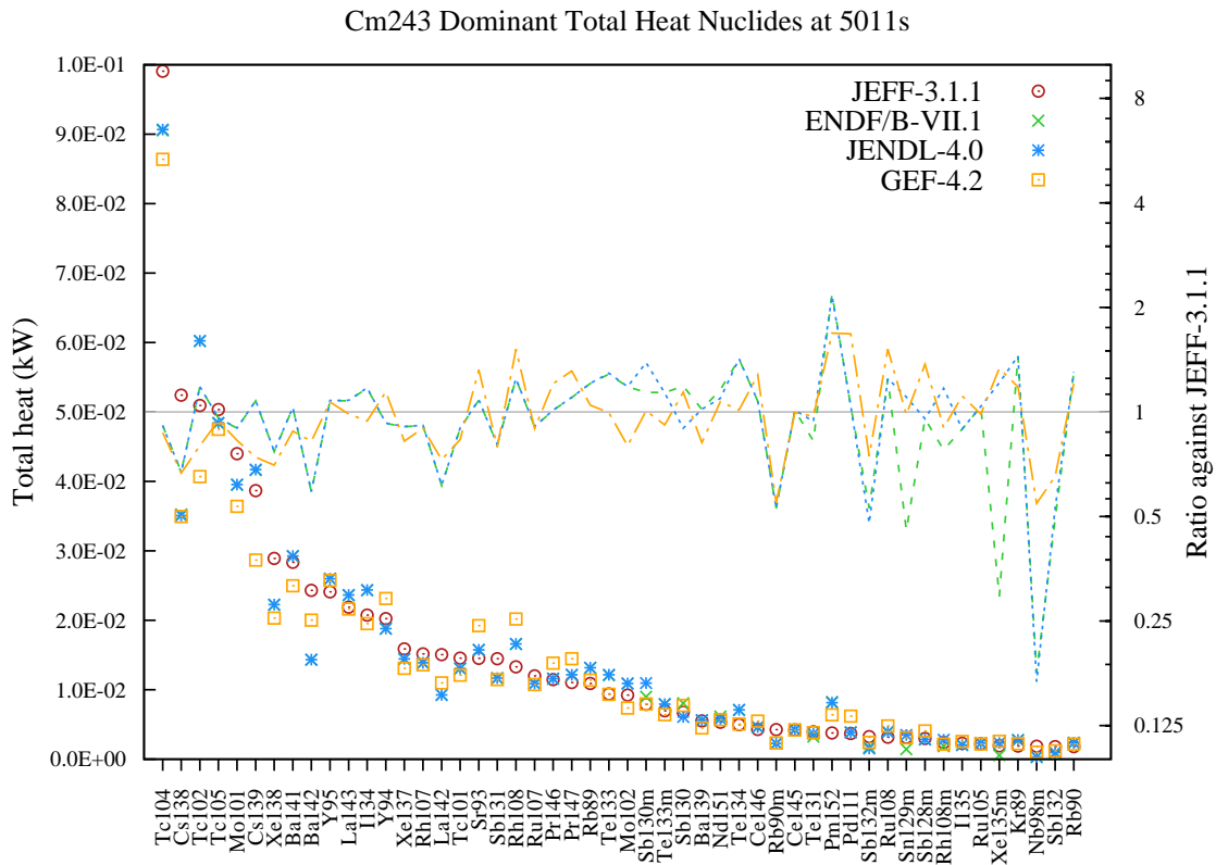
Figure 207: Total decay heat (in kW) fission yield comparison for Cm243 fission pulse after 5011s cooling.
