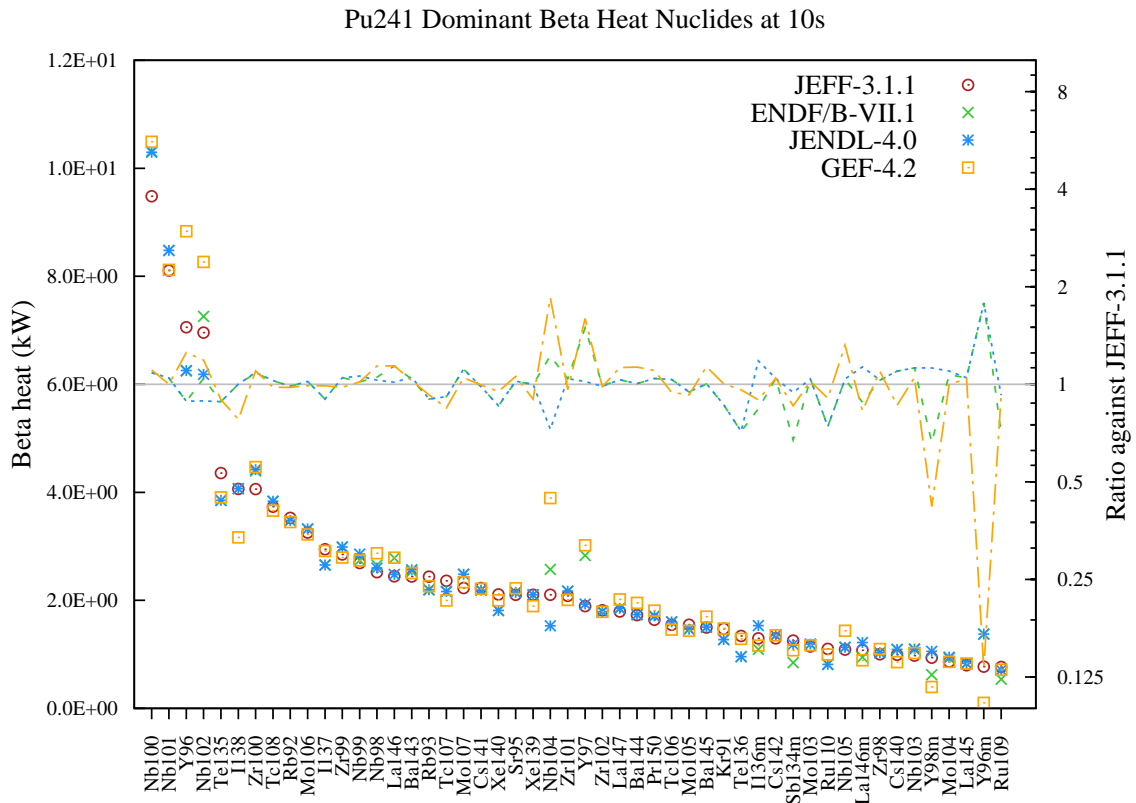
Figure 122: Beta decay heat (in kW) fission yield comparison for Pu241 fission pulse after 10s cooling.
