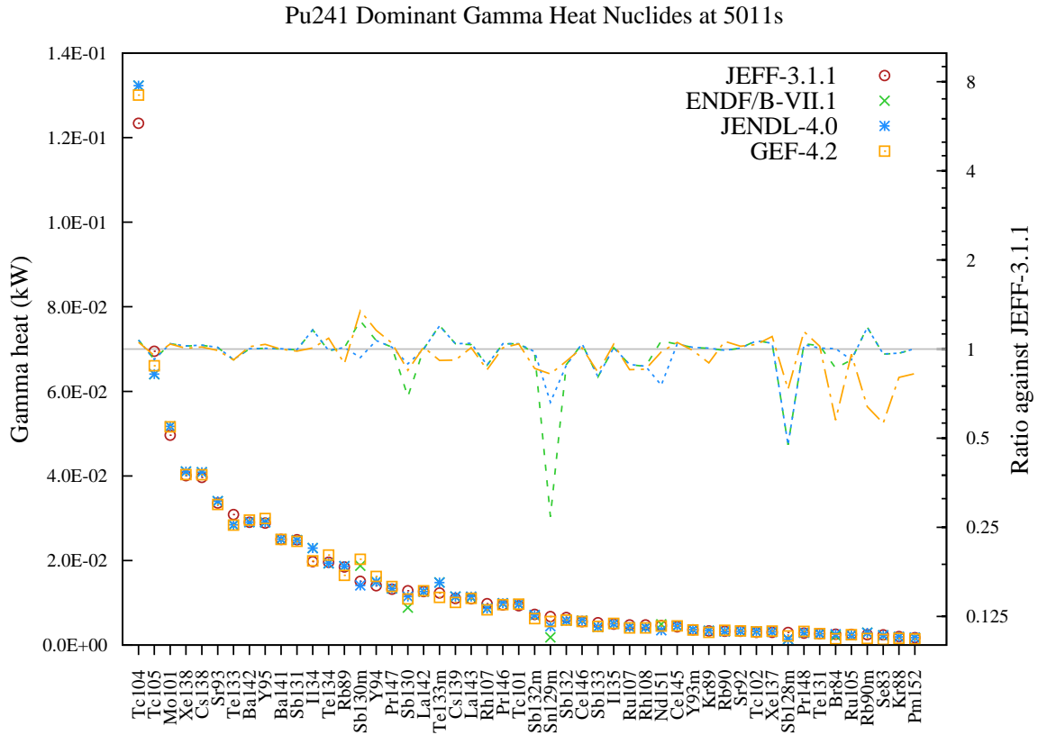
Figure 130: Gamma decay heat (in kW) fission yield comparison for Pu241 fission pulse after 5011s cooling.
