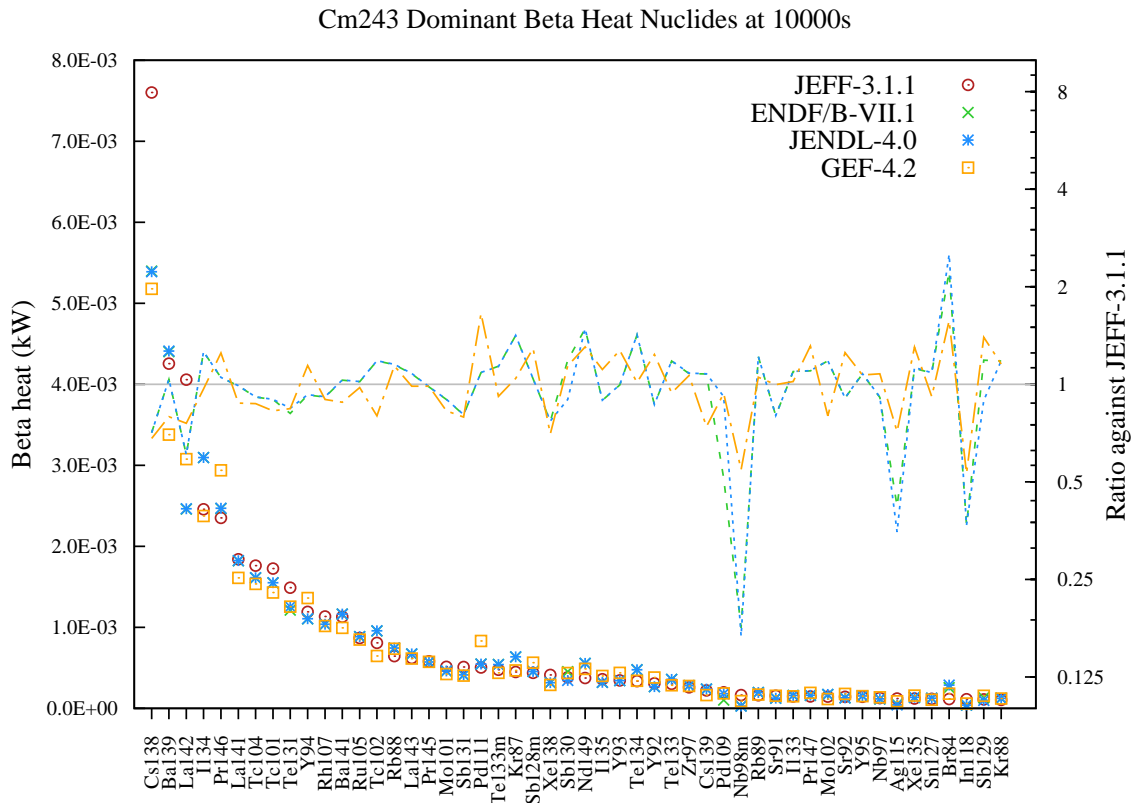
Figure 209: Beta decay heat (in kW) fission yield comparison for Cm243 fission pulse after 10000s cooling.
