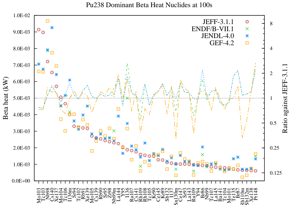
Figure 80: Beta decay heat (in kW) fission yield comparison for Pu238 fission pulse after 100s cooling.
