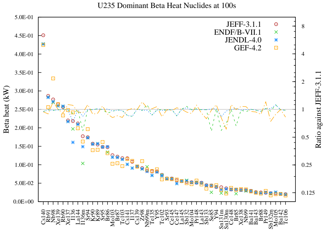
Figure 35: Beta decay heat (in kW) fission yield comparison for U235 fission pulse after 100s cooling.
