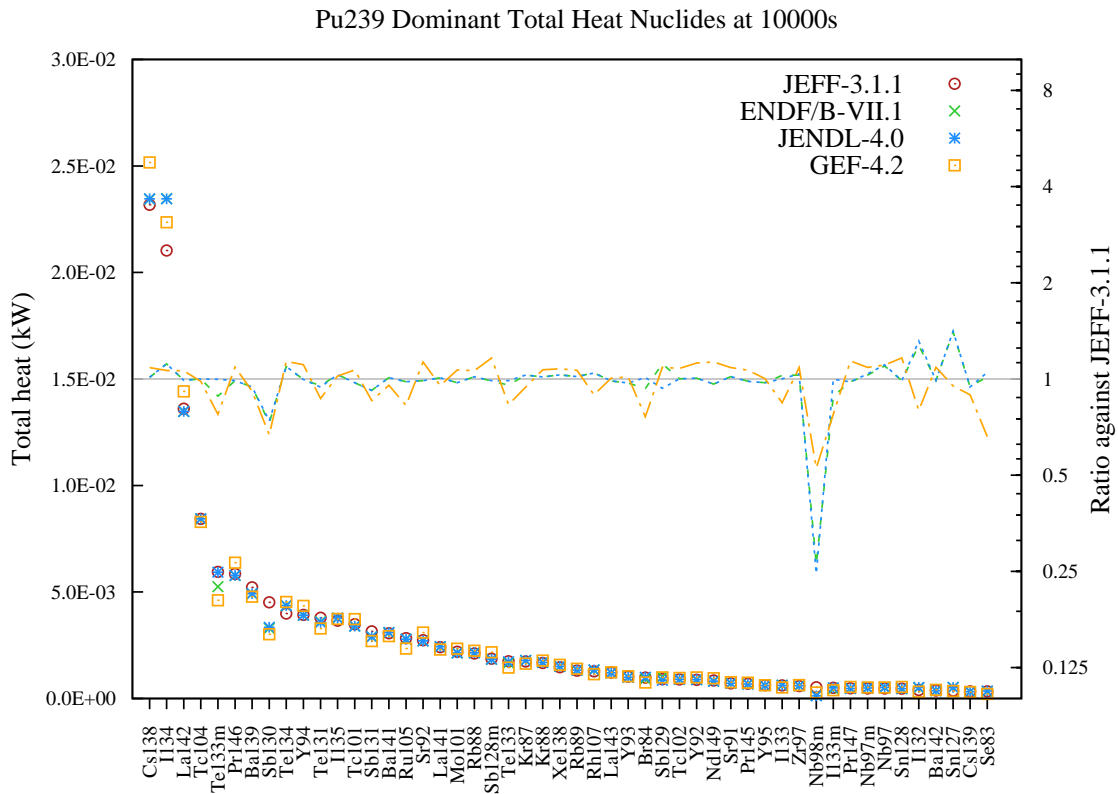
Figure 105: Total decay heat (in kW) fission yield comparison for Pu239 fission pulse after 10000s cooling.
