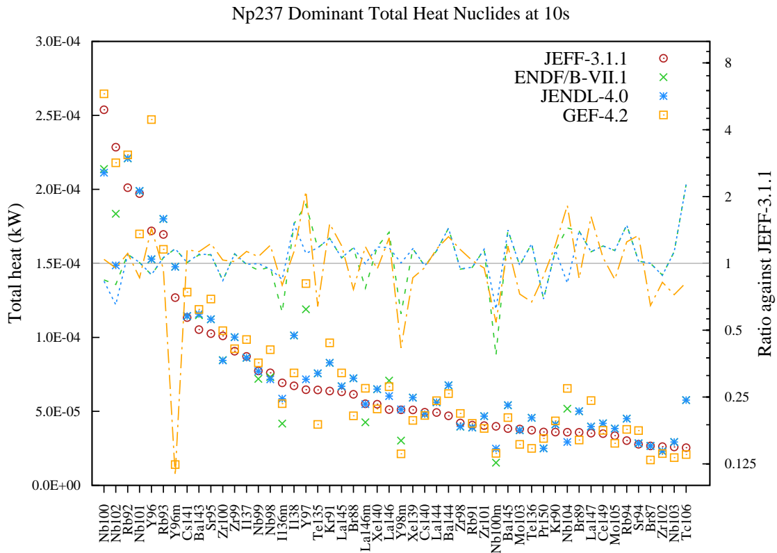
Figure 63: Total decay heat (in kW) fission yield comparison for Np237 fission pulse after 10s cooling.
