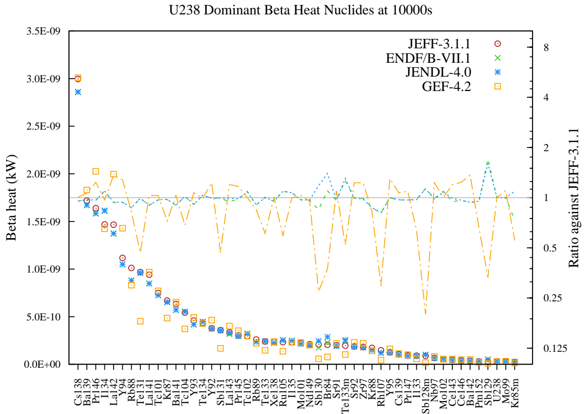
Figure 59: Beta decay heat (in kW) fission yield comparison for U238 fission pulse after 10000s cooling.
