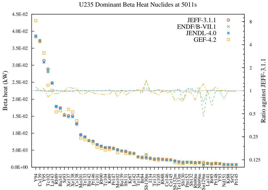
Figure 41: Beta decay heat (in kW) fission yield comparison for U235 fission pulse after 5011s cooling.
