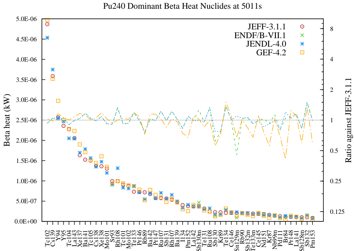
Figure 116: Beta decay heat (in kW) fission yield comparison for Pu240 fission pulse after 5011s cooling.
