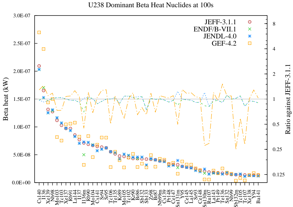
Figure 50: Beta decay heat (in kW) fission yield comparison for U238 fission pulse after 100s cooling.
