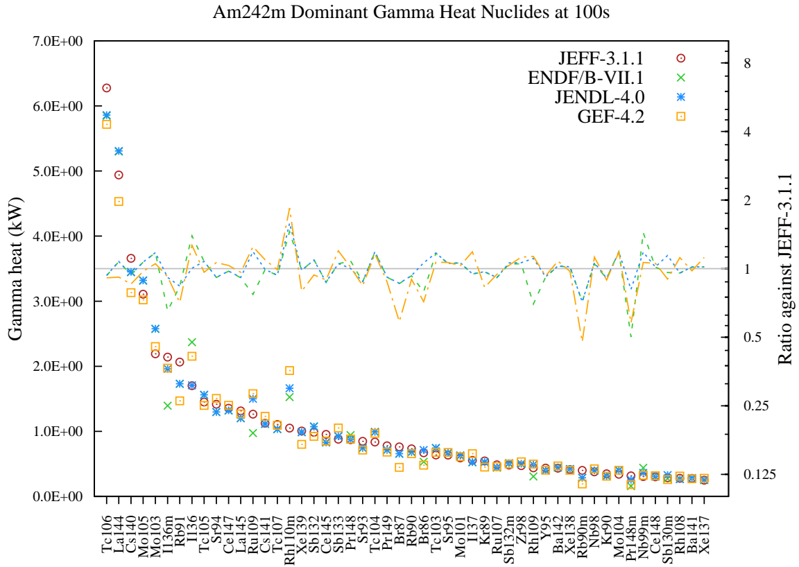
Figure 169: Gamma decay heat (in kW) fission yield comparison for Am242m fission pulse after 100s cooling.
