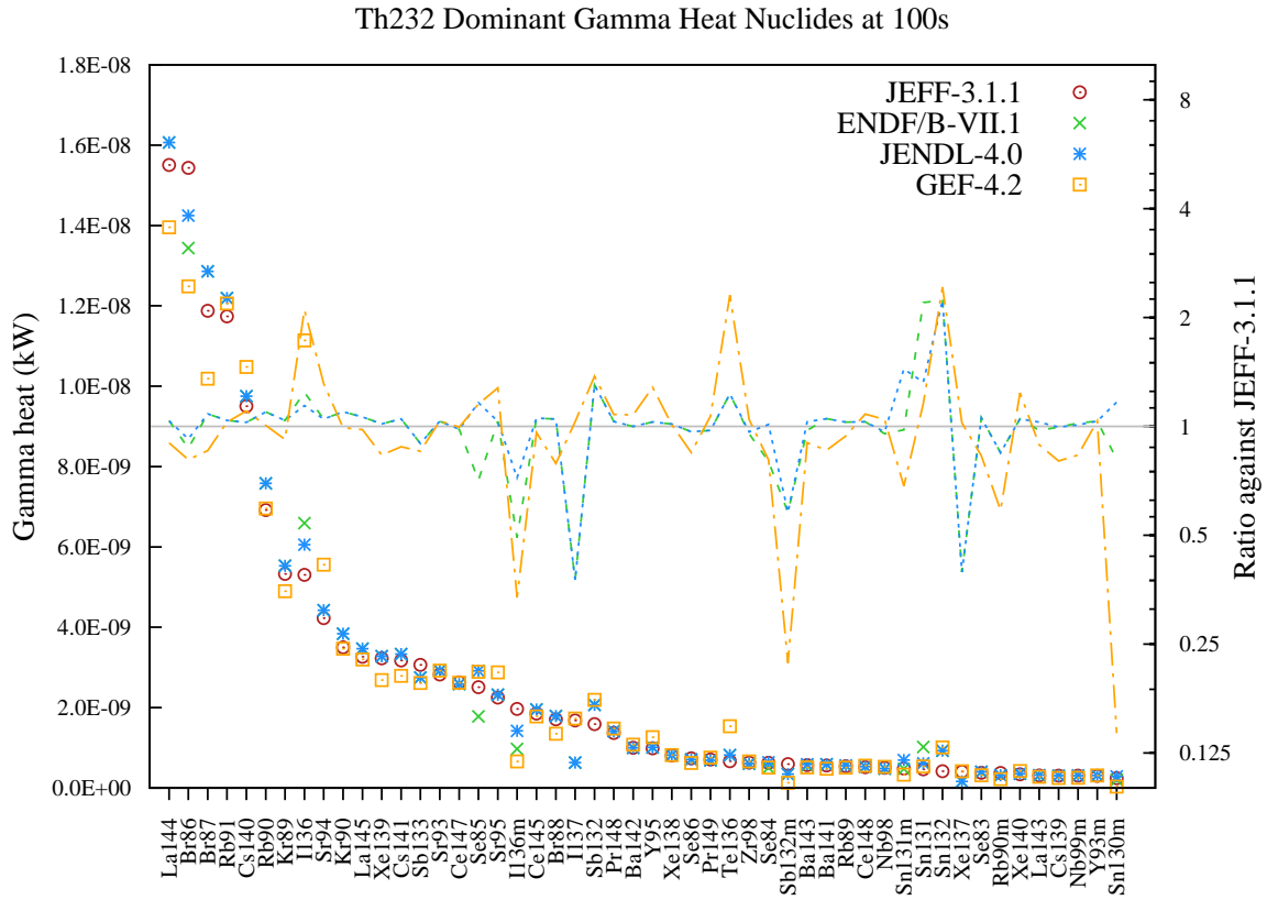
Figure 4: Gamma decay heat (in kW) fission yield comparison for Th232 fission pulse after 100s cooling.
