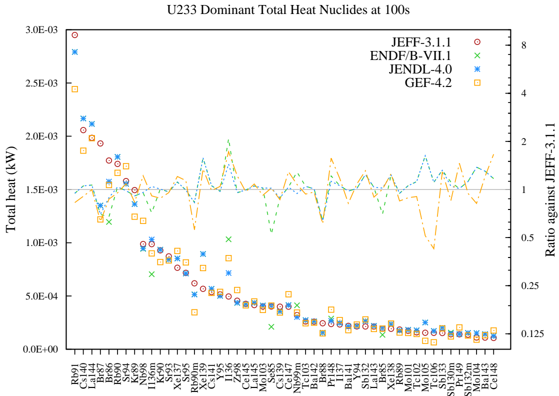
Figure 21: Total decay heat (in kW) fission yield comparison for U233 fission pulse after 100s cooling.
