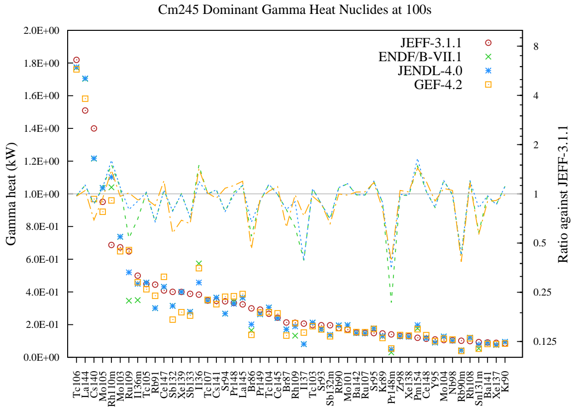
Figure 214: Gamma decay heat (in kW) fission yield comparison for Cm245 fission pulse after 100s cooling.
