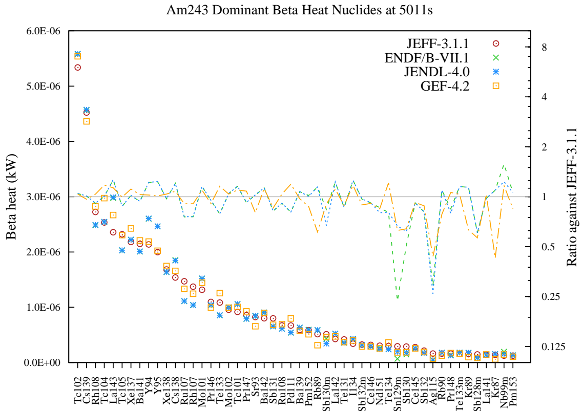
Figure 191: Beta decay heat (in kW) fission yield comparison for Am243 fission pulse after 5011s cooling.
