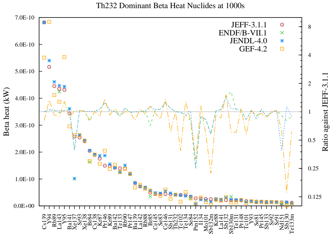
Figure 8: Beta decay heat (in kW) fission yield comparison for Th232 fission pulse after 1000s cooling.
