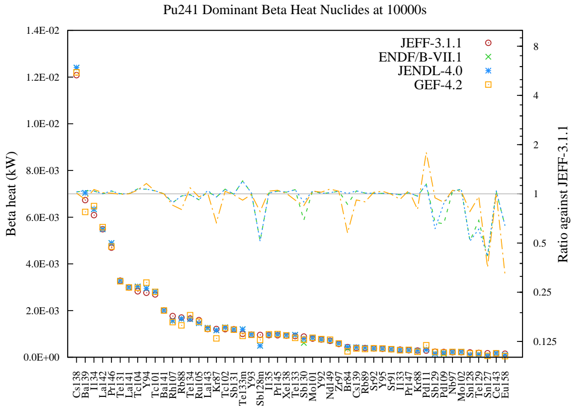
Figure 134: Beta decay heat (in kW) fission yield comparison for Pu241 fission pulse after 10000s cooling.
