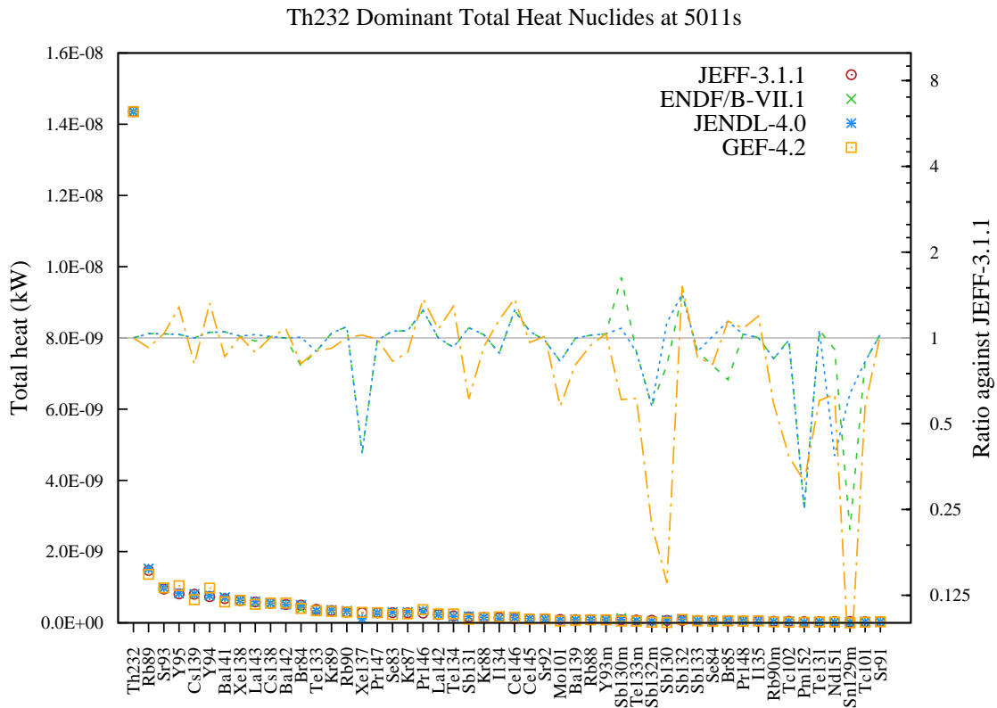
Figure 12: Total decay heat (in kW) fission yield comparison for Th232 fission pulse after 5011s cooling.
