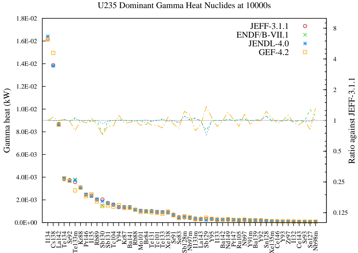
Figure 43: Gamma decay heat (in kW) fission yield comparison for U235 fission pulse after 10000s cooling.
