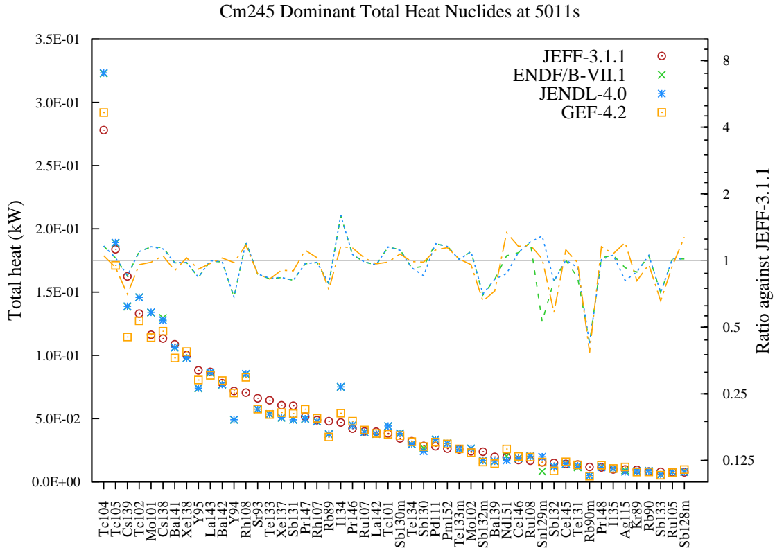
Figure 222: Total decay heat (in kW) fission yield comparison for Cm245 fission pulse after 5011s cooling.
