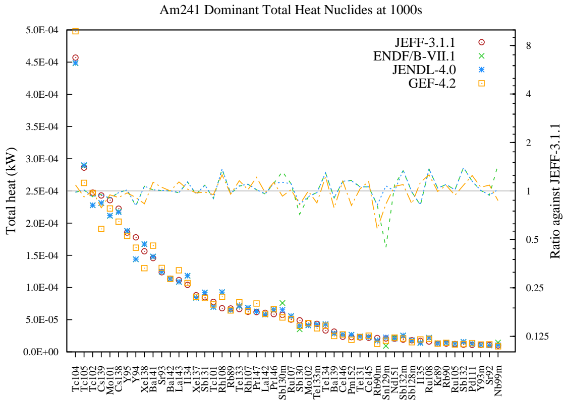
Figure 159: Total decay heat (in kW) fission yield comparison for Am241 fission pulse after 1000s cooling.
