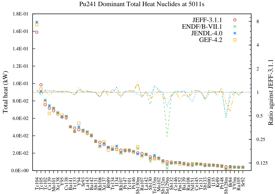
Figure 132: Total decay heat (in kW) fission yield comparison for Pu241 fission pulse after 5011s cooling.
