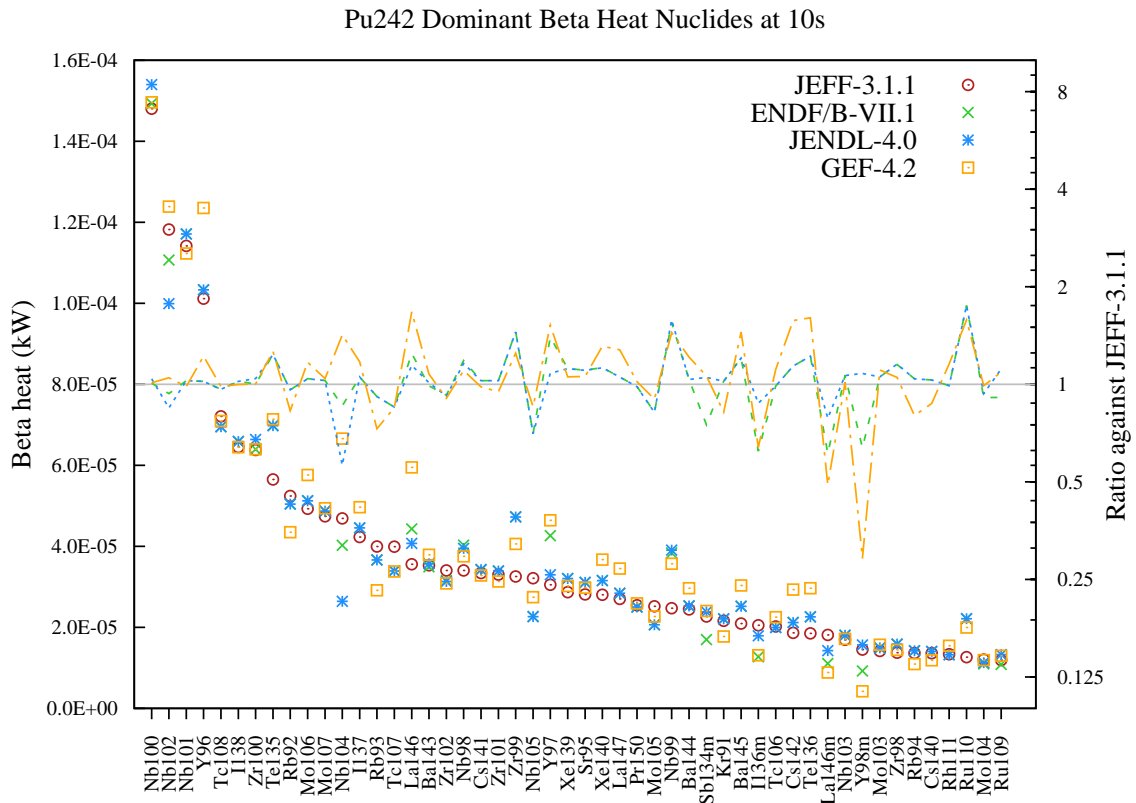
Figure 137: Beta decay heat (in kW) fission yield comparison for Pu242 fission pulse after 10s cooling.
