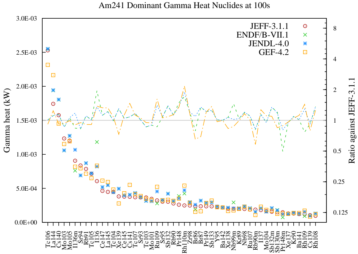
Figure 154: Gamma decay heat (in kW) fission yield comparison for Am241 fission pulse after 100s cooling.
