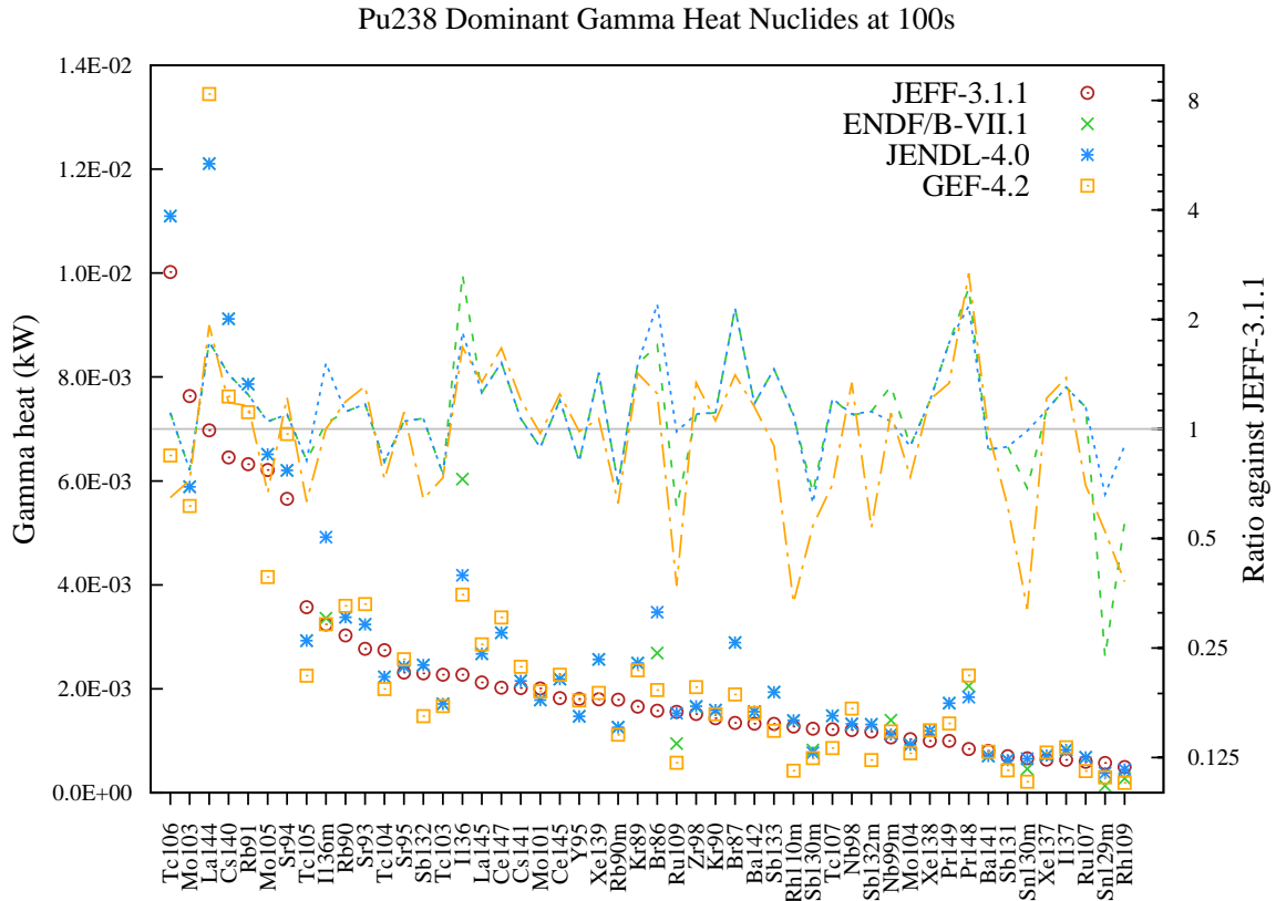
Figure 79: Gamma decay heat (in kW) fission yield comparison for Pu238 fission pulse after 100s cooling.
