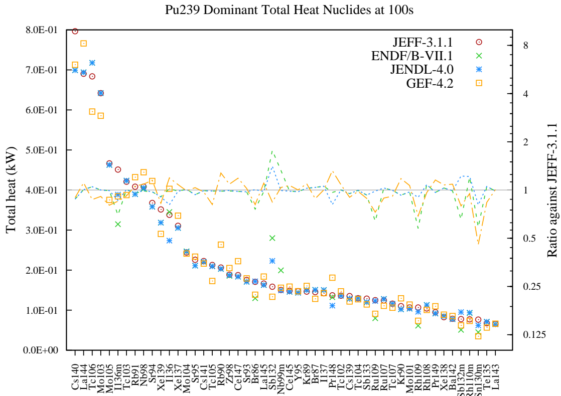
Figure 96: Total decay heat (in kW) fission yield comparison for Pu239 fission pulse after 100s cooling.
