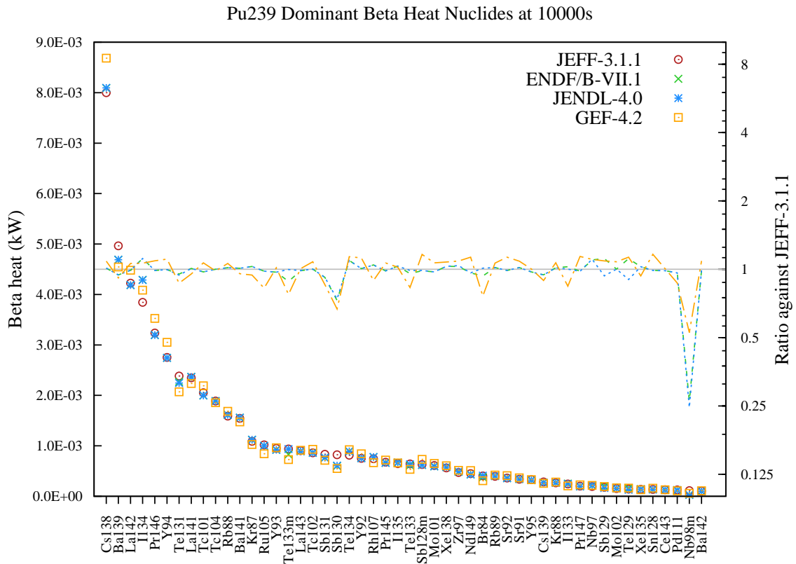
Figure 104: Beta decay heat (in kW) fission yield comparison for Pu239 fission pulse after 10000s cooling.
