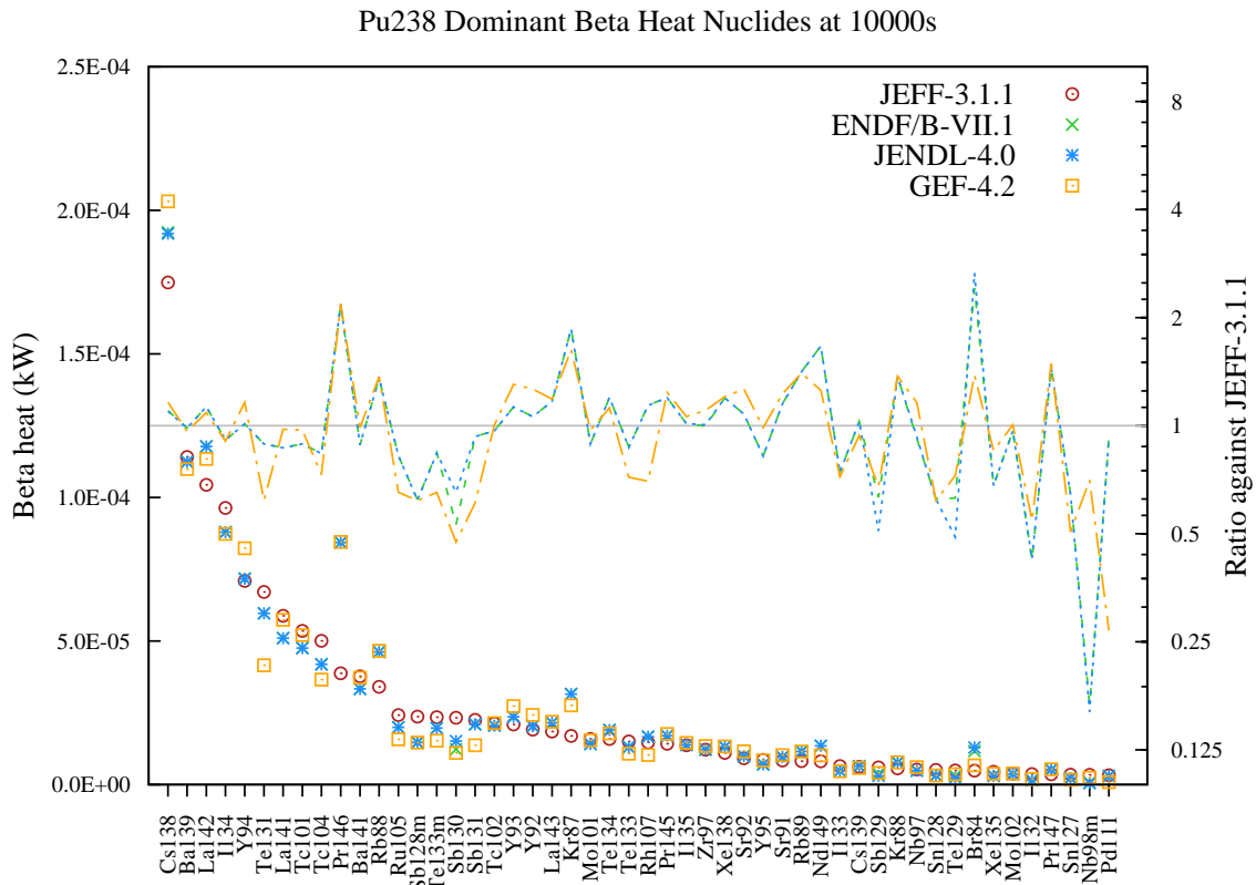
Figure 89: Beta decay heat (in kW) fission yield comparison for Pu238 fission pulse after 10000s cooling.
