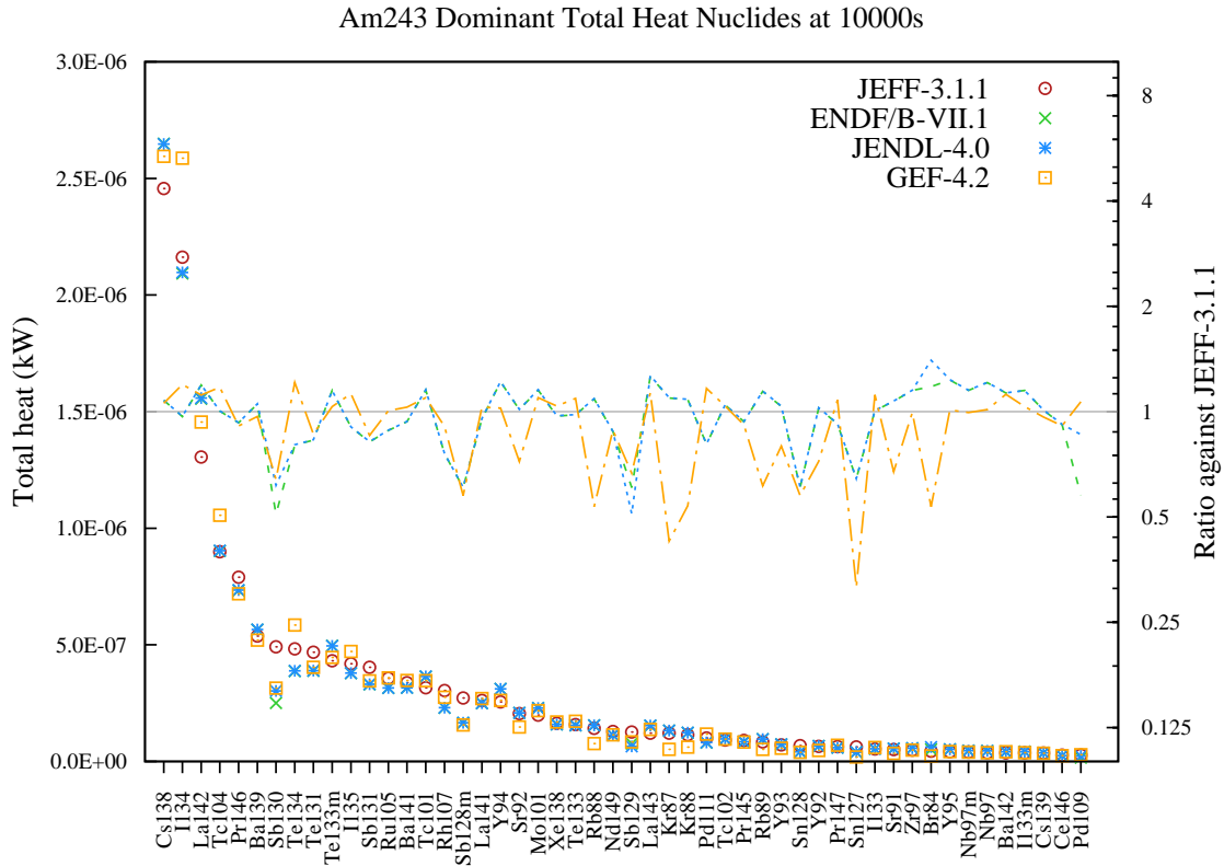
Figure 195: Total decay heat (in kW) fission yield comparison for Am243 fission pulse after 10000s cooling.
