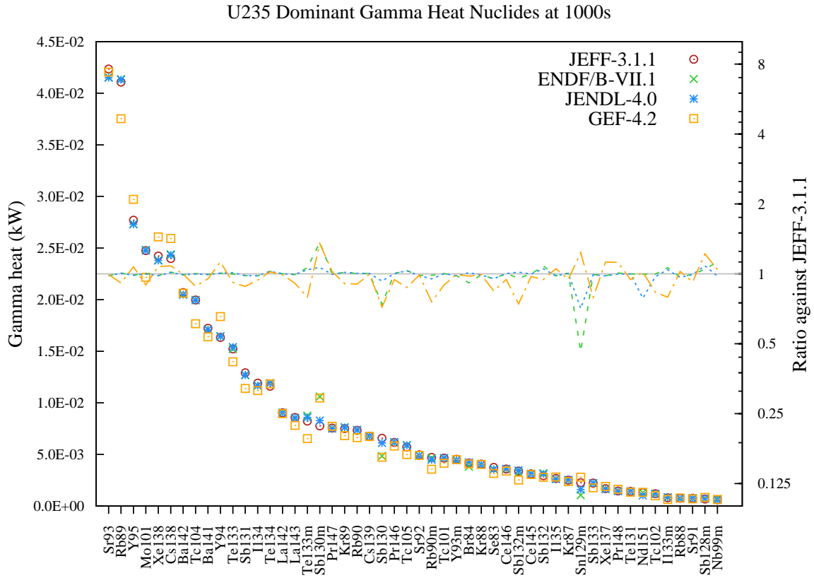
Figure 37: Gamma decay heat (in kW) fission yield comparison for U235 fission pulse after 1000s cooling.
