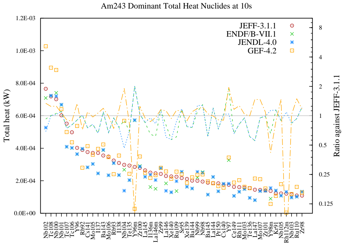
Figure 183: Total decay heat (in kW) fission yield comparison for Am243 fission pulse after 10s cooling.
