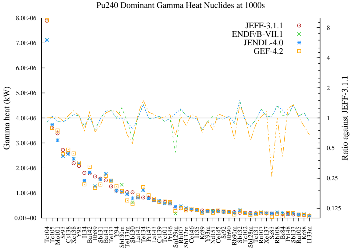
Figure 112: Gamma decay heat (in kW) fission yield comparison for Pu240 fission pulse after 1000s cooling.
