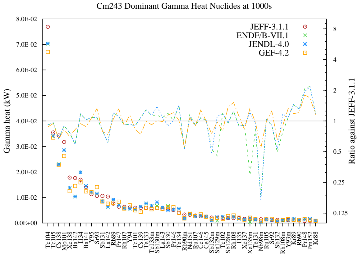
Figure 202: Gamma decay heat (in kW) fission yield comparison for Cm243 fission pulse after 1000s cooling.
