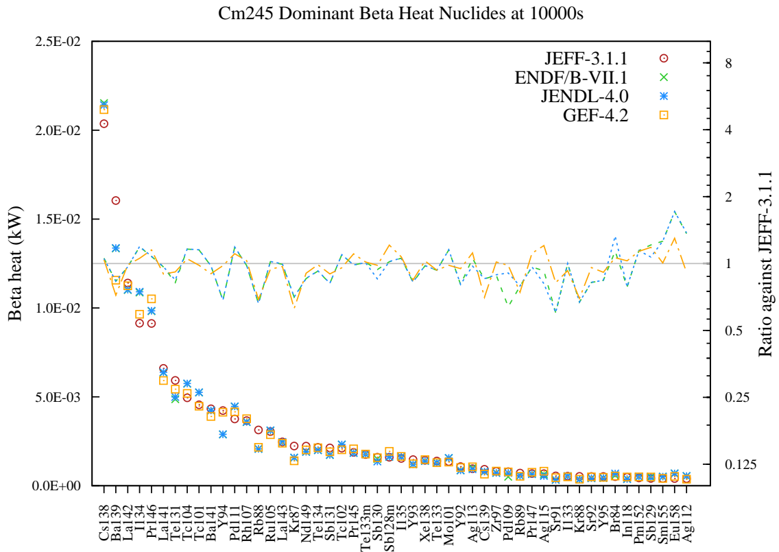
Figure 224: Beta decay heat (in kW) fission yield comparison for Cm245 fission pulse after 10000s cooling.
