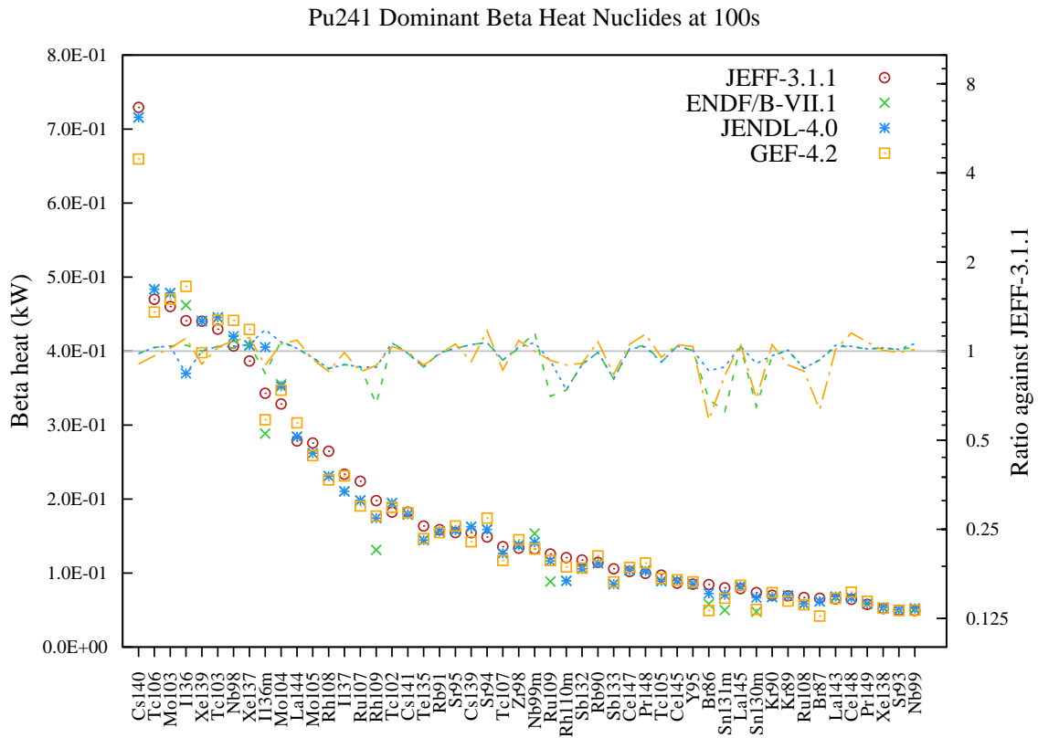
Figure 125: Beta decay heat (in kW) fission yield comparison for Pu241 fission pulse after 100s cooling.
