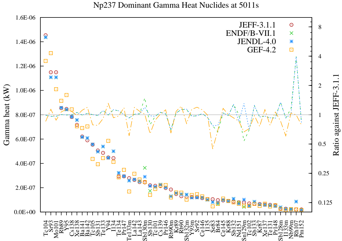
Figure 70: Gamma decay heat (in kW) fission yield comparison for Np237 fission pulse after 5011s cooling.
