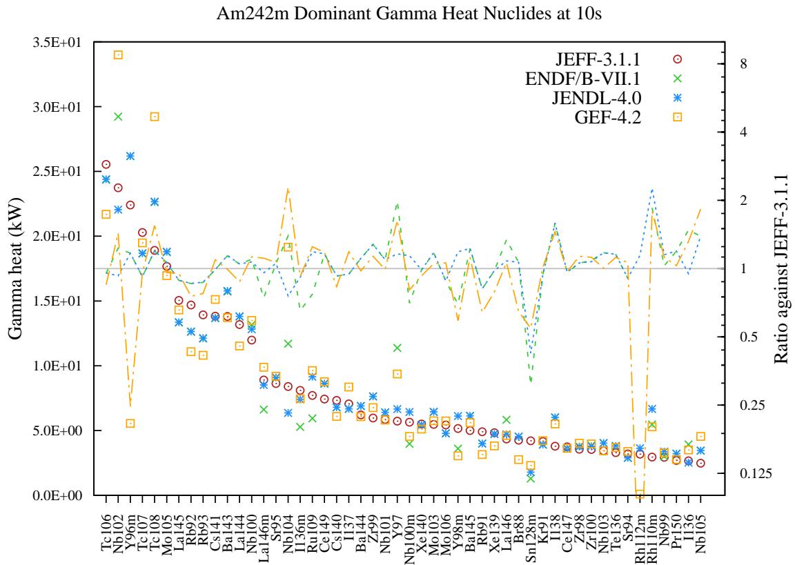
Figure 166: Gamma decay heat (in kW) fission yield comparison for Am242m fission pulse after 10s cooling.
