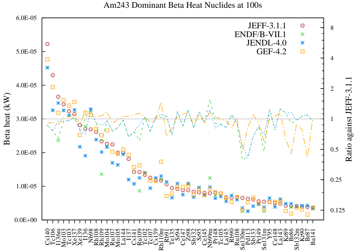
Figure 185: Beta decay heat (in kW) fission yield comparison for Am243 fission pulse after 100s cooling.
