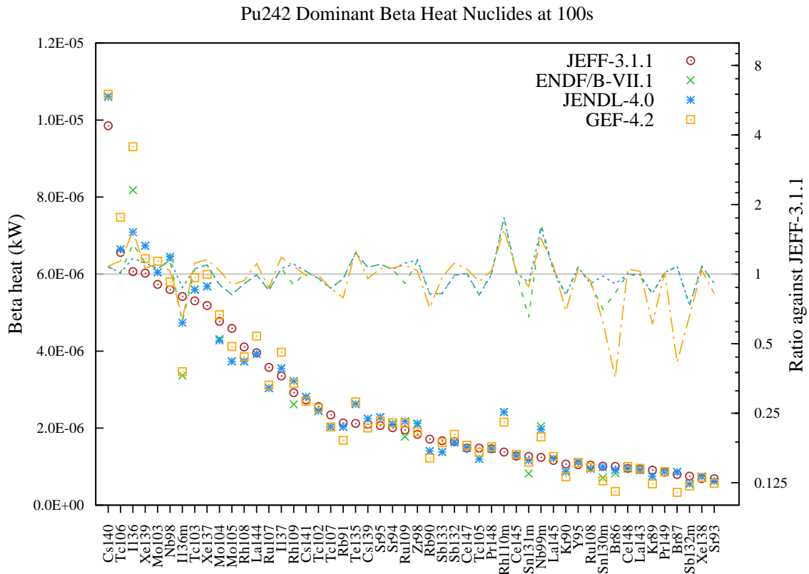
Figure 140: Beta decay heat (in kW) fission yield comparison for Pu242 fission pulse after 100s cooling.
