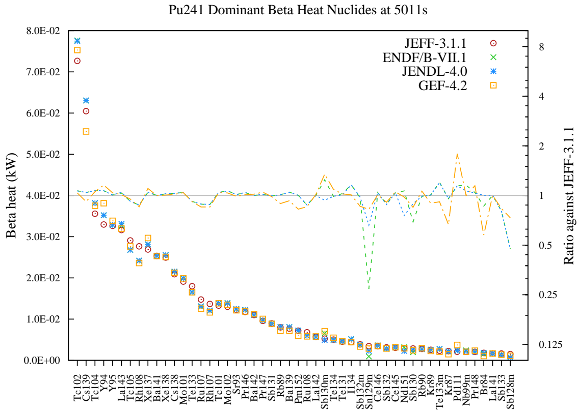
Figure 131: Beta decay heat (in kW) fission yield comparison for Pu241 fission pulse after 5011s cooling.
