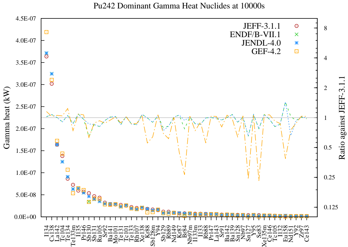
Figure 148: Gamma decay heat (in kW) fission yield comparison for Pu242 fission pulse after 10000s cooling.
