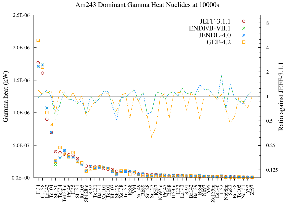
Figure 193: Gamma decay heat (in kW) fission yield comparison for Am243 fission pulse after 10000s cooling.
