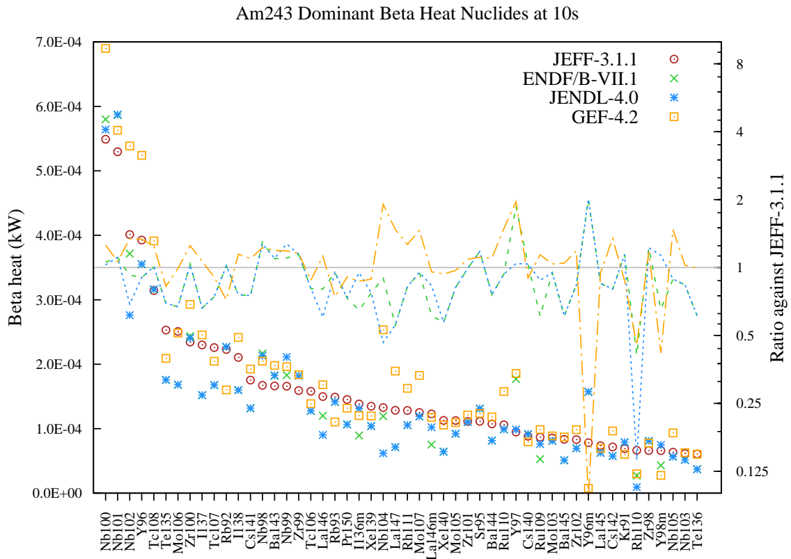
Figure 182: Beta decay heat (in kW) fission yield comparison for Am243 fission pulse after 10s cooling.
