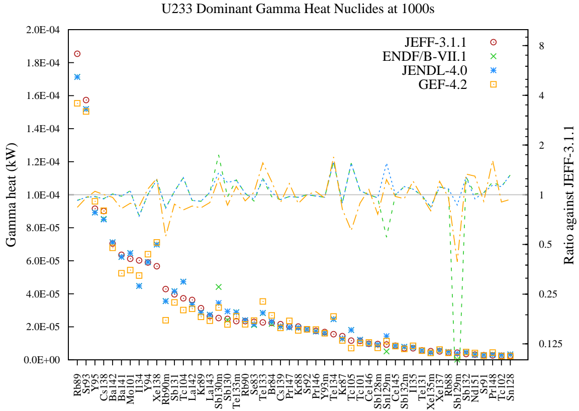
Figure 22: Gamma decay heat (in kW) fission yield comparison for U233 fission pulse after 1000s cooling.
