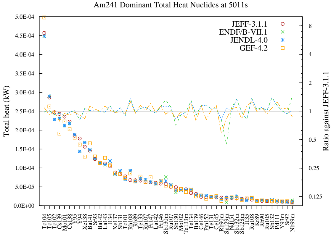
Figure 162: Total decay heat (in kW) fission yield comparison for Am241 fission pulse after 5011s cooling.
