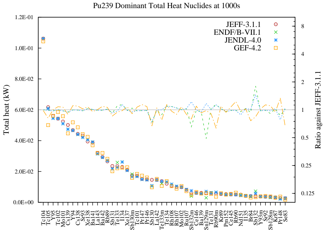
Figure 99: Total decay heat (in kW) fission yield comparison for Pu239 fission pulse after 1000s cooling.
