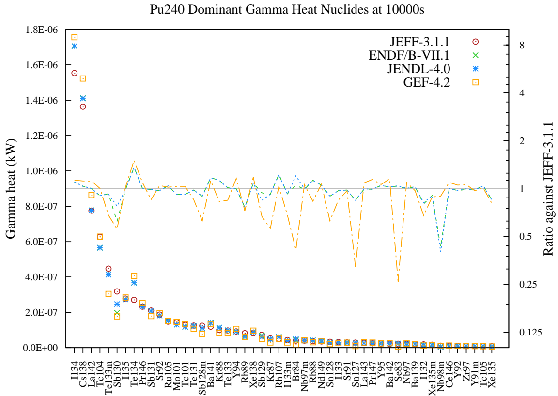
Figure 118: Gamma decay heat (in kW) fission yield comparison for Pu240 fission pulse after 10000s cooling.
