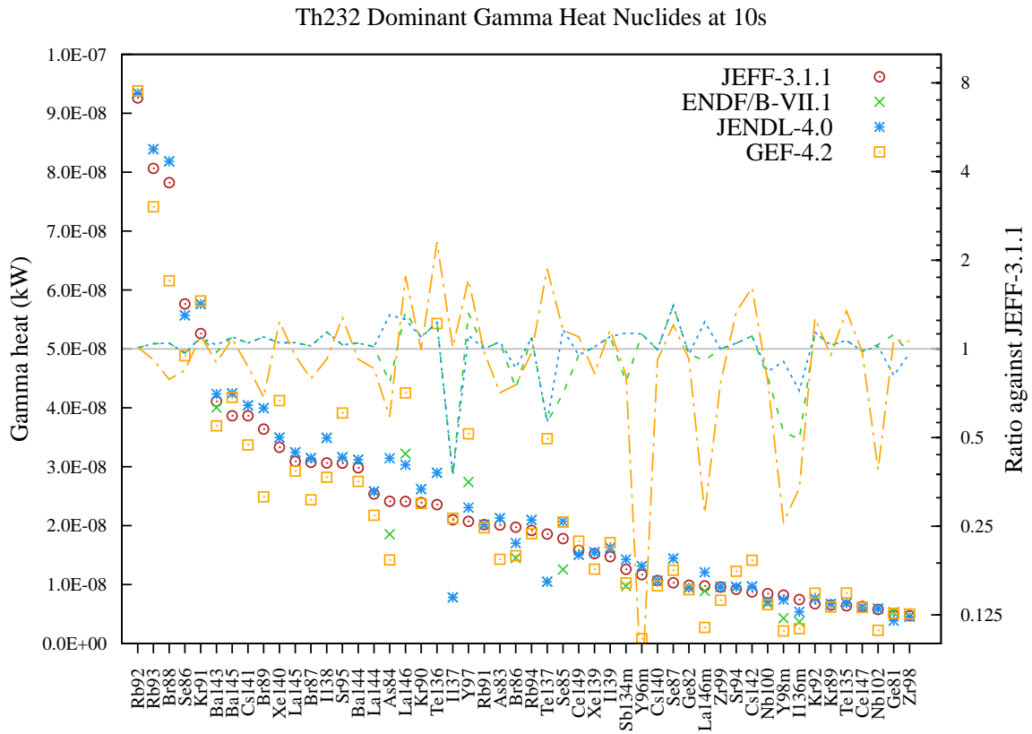
Figure 1: Gamma decay heat (in kW) fission yield comparison for Th232 fission pulse after 10s cooling.
