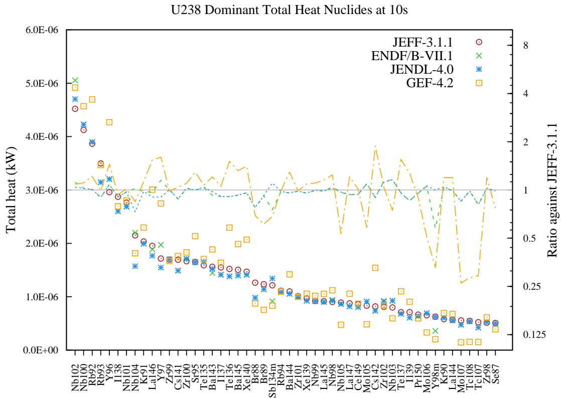
Figure 48: Total decay heat (in kW) fission yield comparison for U238 fission pulse after 10s cooling.
