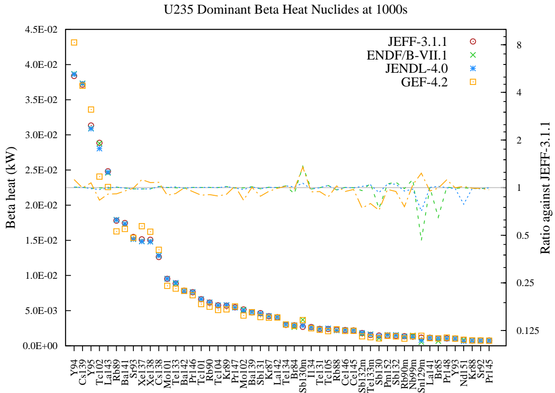
Figure 38: Beta decay heat (in kW) fission yield comparison for U235 fission pulse after 1000s cooling.
