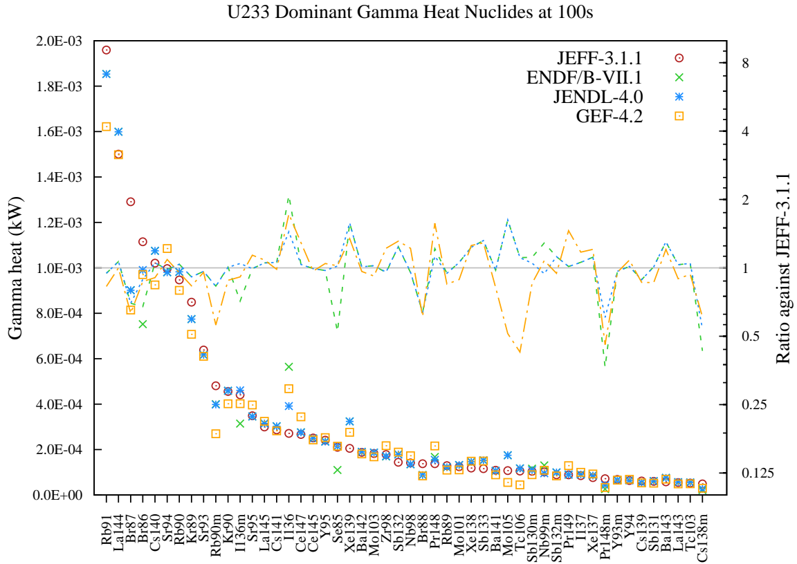
Figure 19: Gamma decay heat (in kW) fission yield comparison for U233 fission pulse after 100s cooling.
