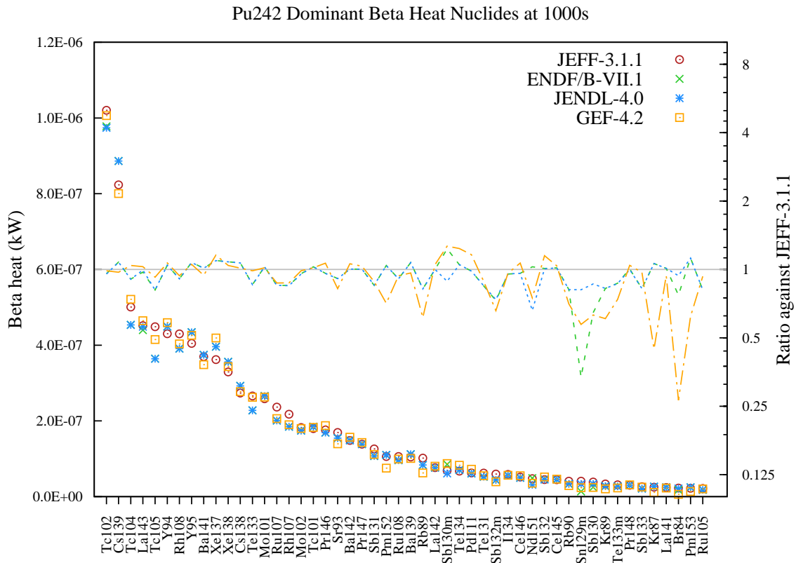
Figure 143: Beta decay heat (in kW) fission yield comparison for Pu242 fission pulse after 1000s cooling.
