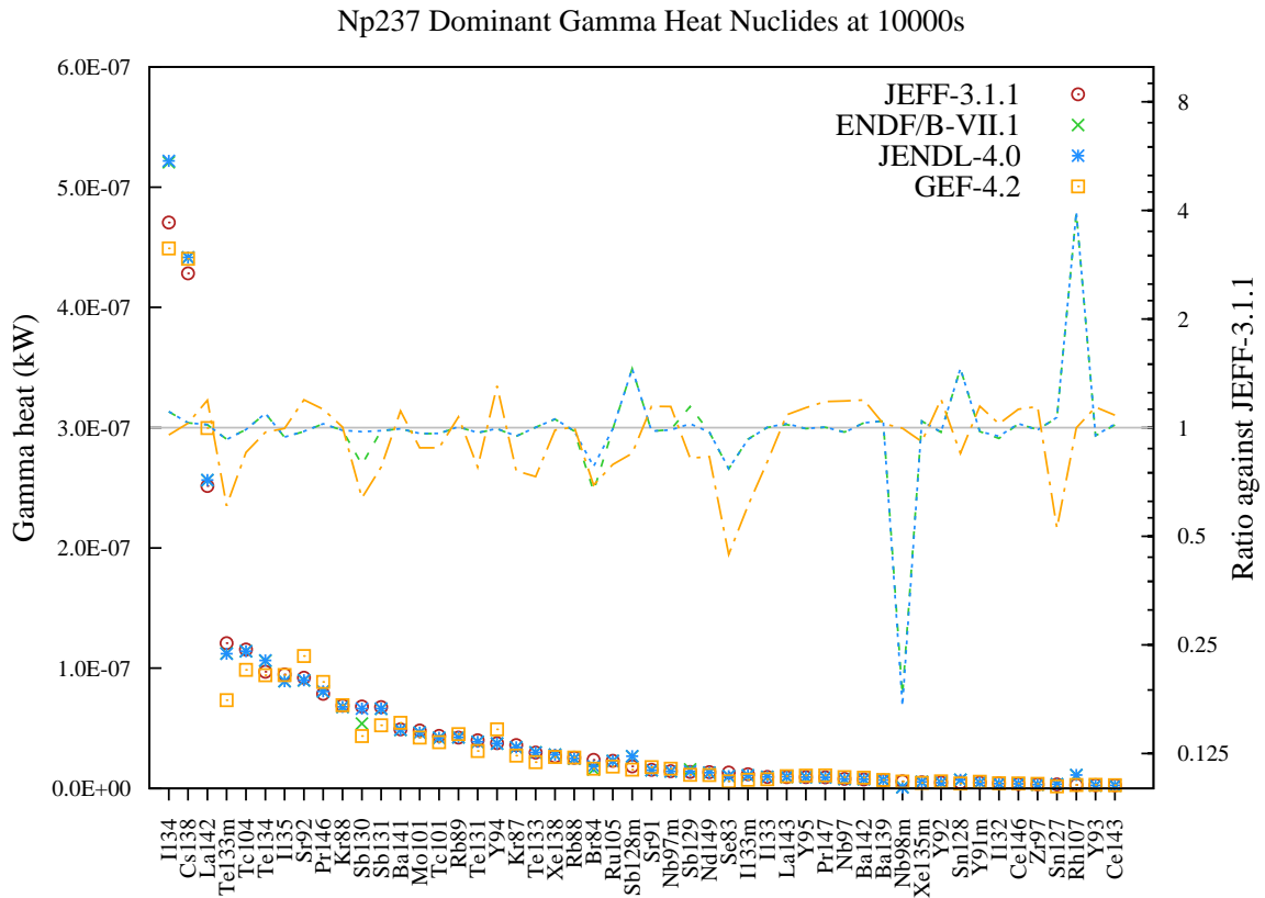
Figure 73: Gamma decay heat (in kW) fission yield comparison for Np237 fission pulse after 10000s cooling.
