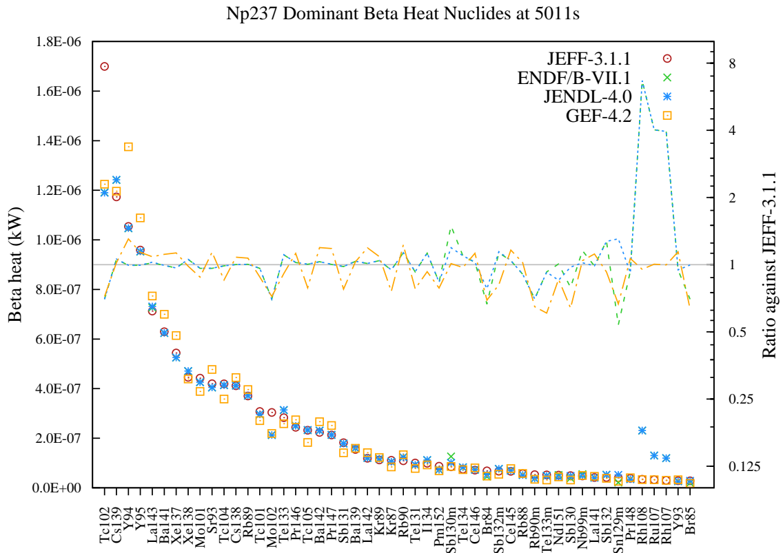
Figure 71: Beta decay heat (in kW) fission yield comparison for Np237 fission pulse after 5011s cooling.
