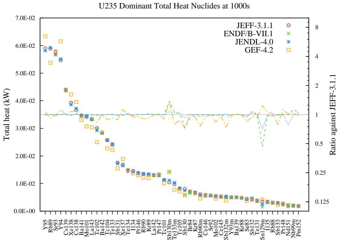
Figure 39: Total decay heat (in kW) fission yield comparison for U235 fission pulse after 1000s cooling.
