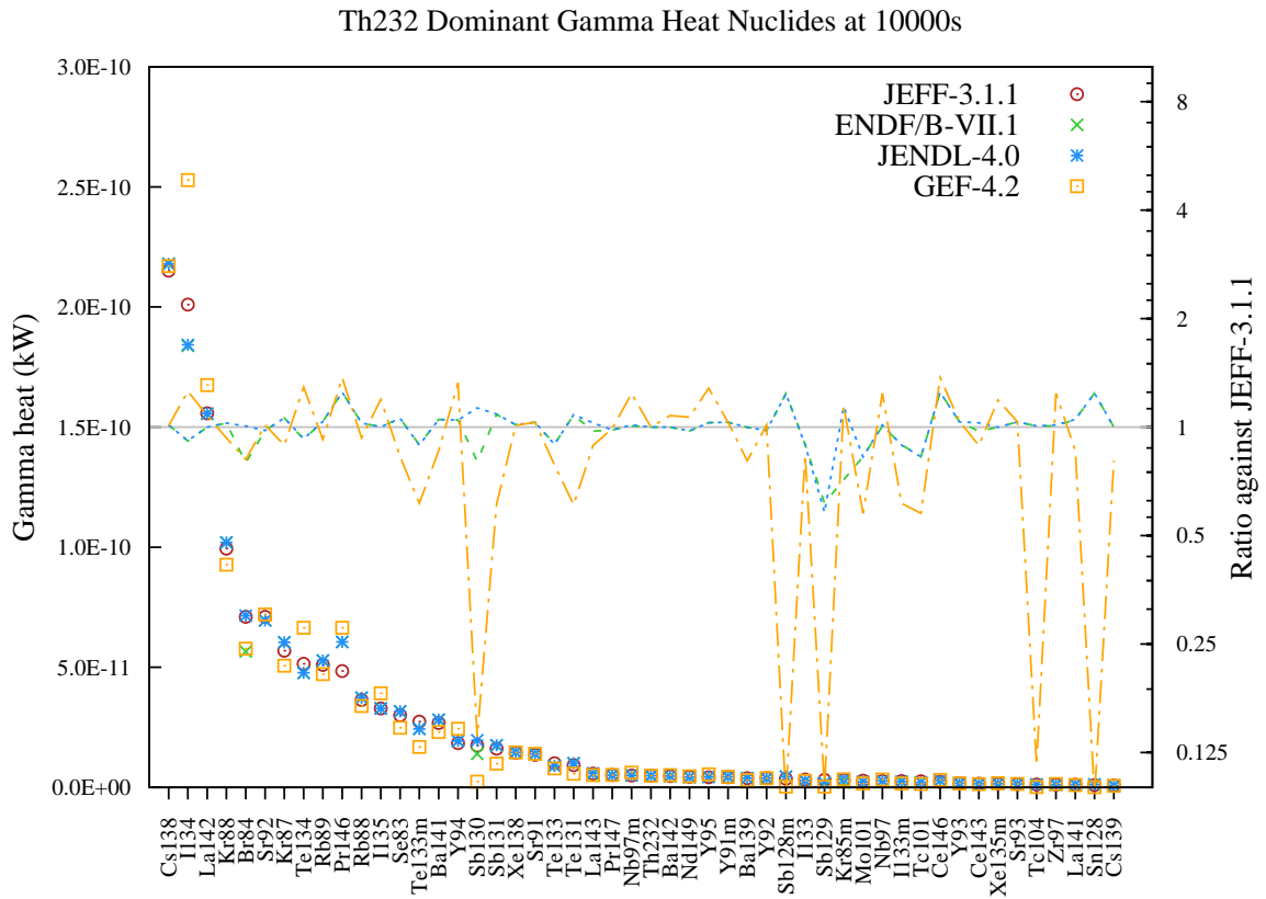
Figure 13: Gamma decay heat (in kW) fission yield comparison for Th232 fission pulse after 10000s cooling.
