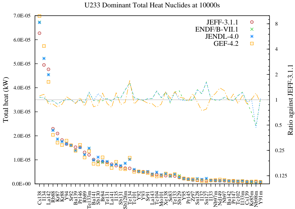
Figure 30: Total decay heat (in kW) fission yield comparison for U233 fission pulse after 10000s cooling.
