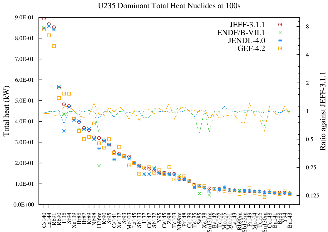
Figure 36: Total decay heat (in kW) fission yield comparison for U235 fission pulse after 100s cooling.
