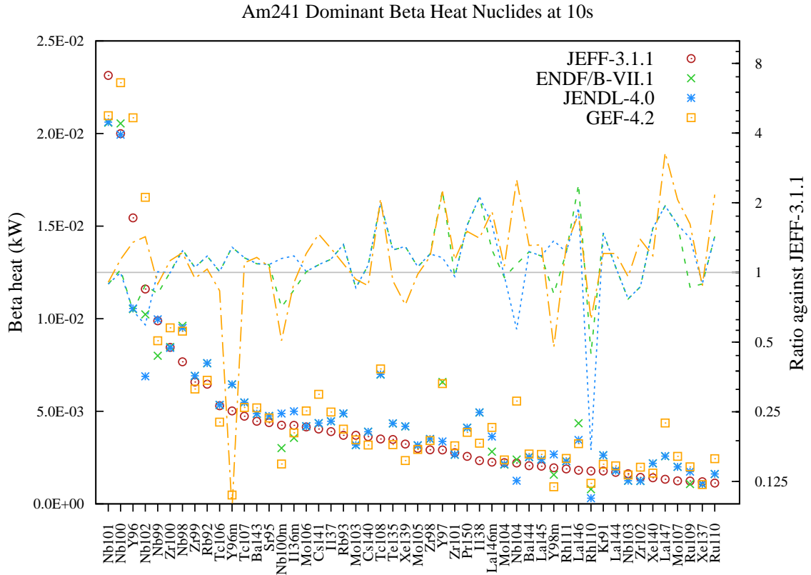
Figure 152: Beta decay heat (in kW) fission yield comparison for Am241 fission pulse after 10s cooling.
