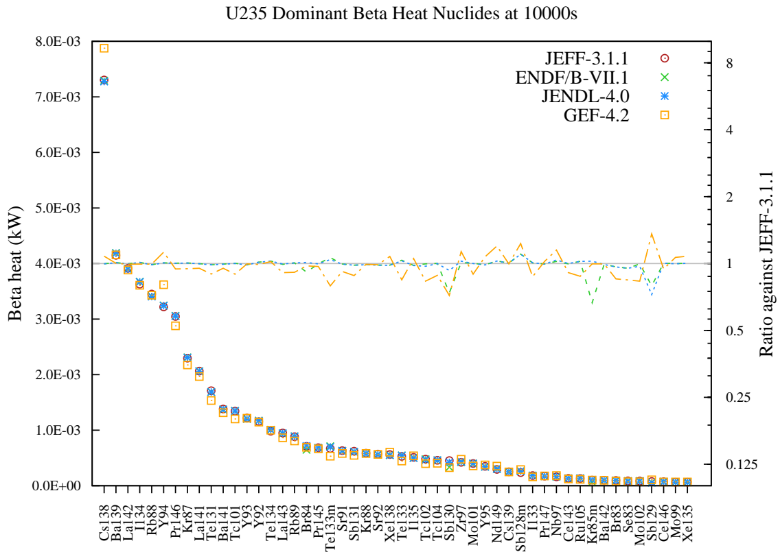
Figure 44: Beta decay heat (in kW) fission yield comparison for U235 fission pulse after 10000s cooling.
