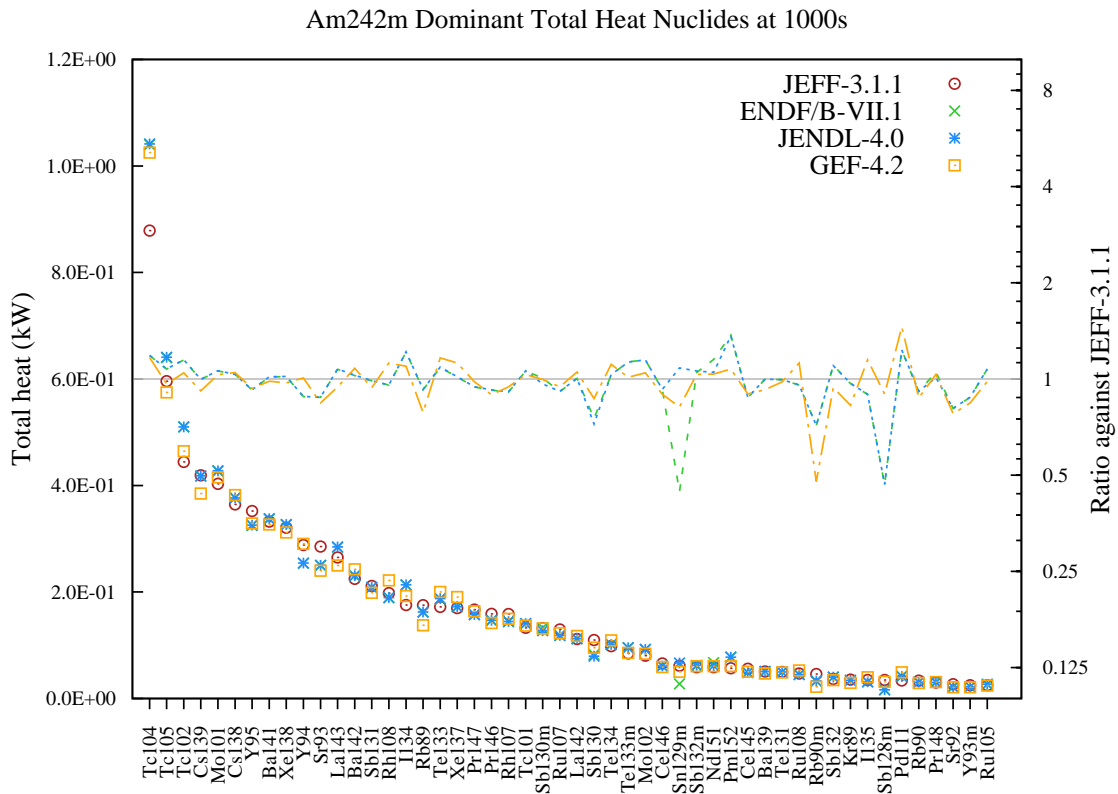
Figure 174: Total decay heat (in kW) fission yield comparison for Am242m fission pulse after 1000s cooling.
