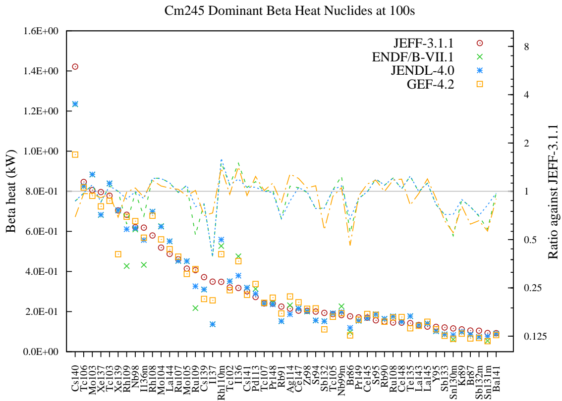
Figure 215: Beta decay heat (in kW) fission yield comparison for Cm245 fission pulse after 100s cooling.
