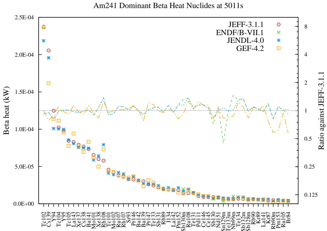
Figure 161: Beta decay heat (in kW) fission yield comparison for Am241 fission pulse after 5011s cooling.
