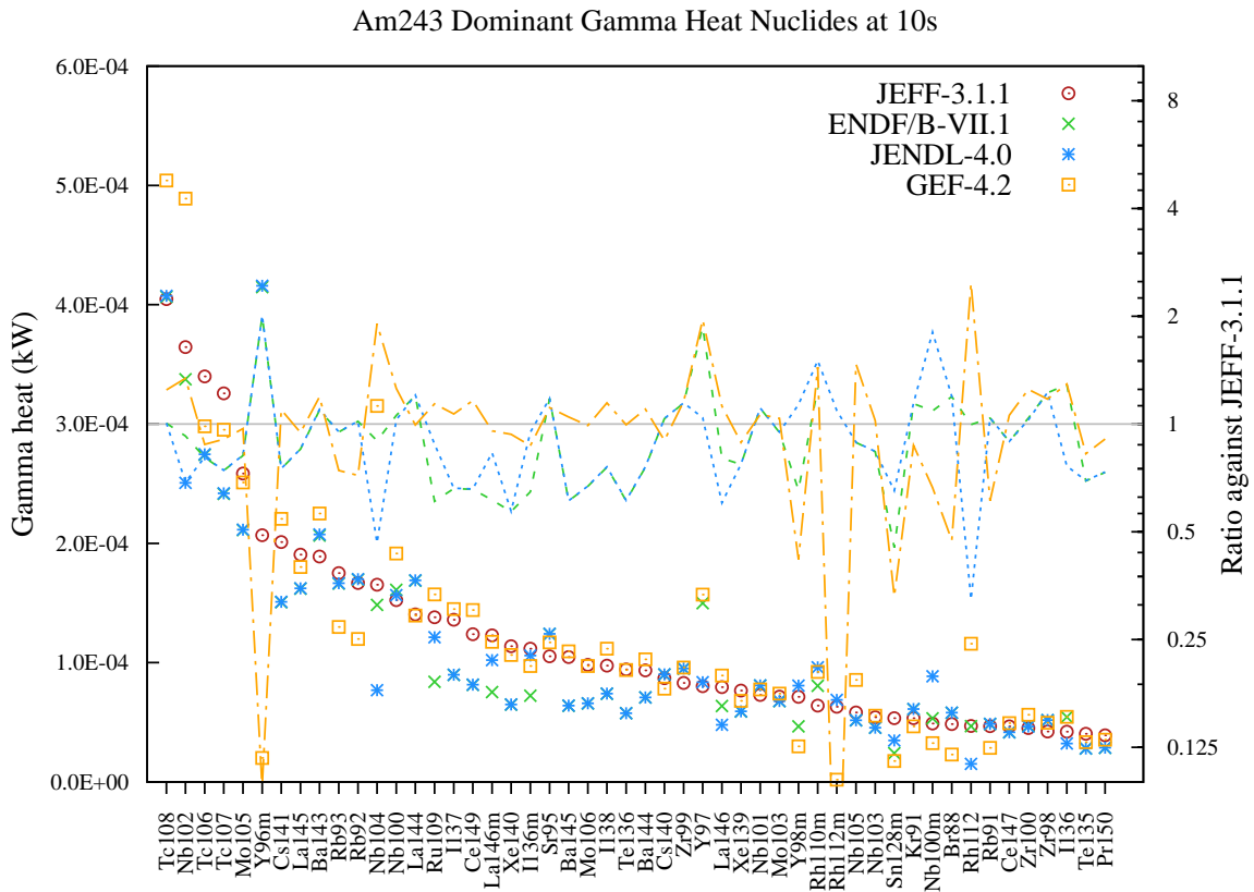
Figure 181: Gamma decay heat (in kW) fission yield comparison for Am243 fission pulse after 10s cooling.
