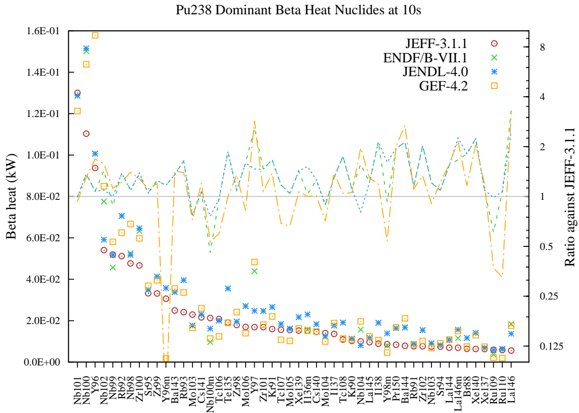
Figure 77: Beta decay heat (in kW) fission yield comparison for Pu238 fission pulse after 10s cooling.
