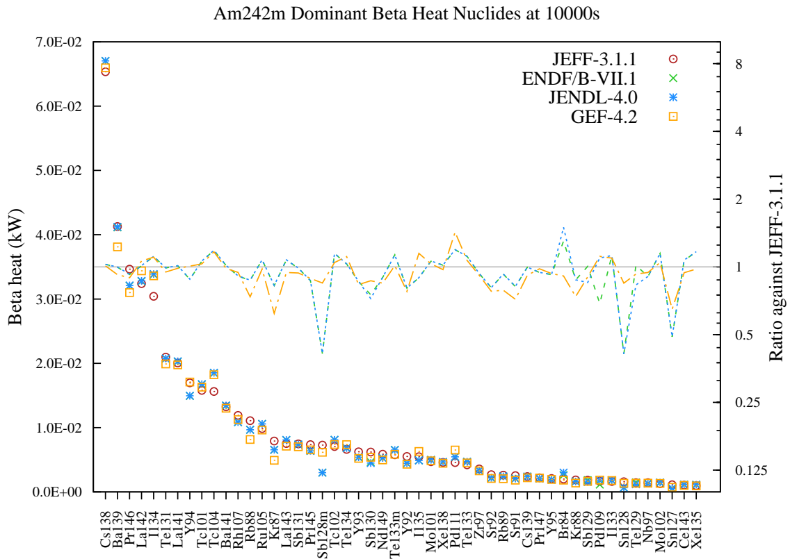
Figure 179: Beta decay heat (in kW) fission yield comparison for Am242m fission pulse after 10000s cooling.
