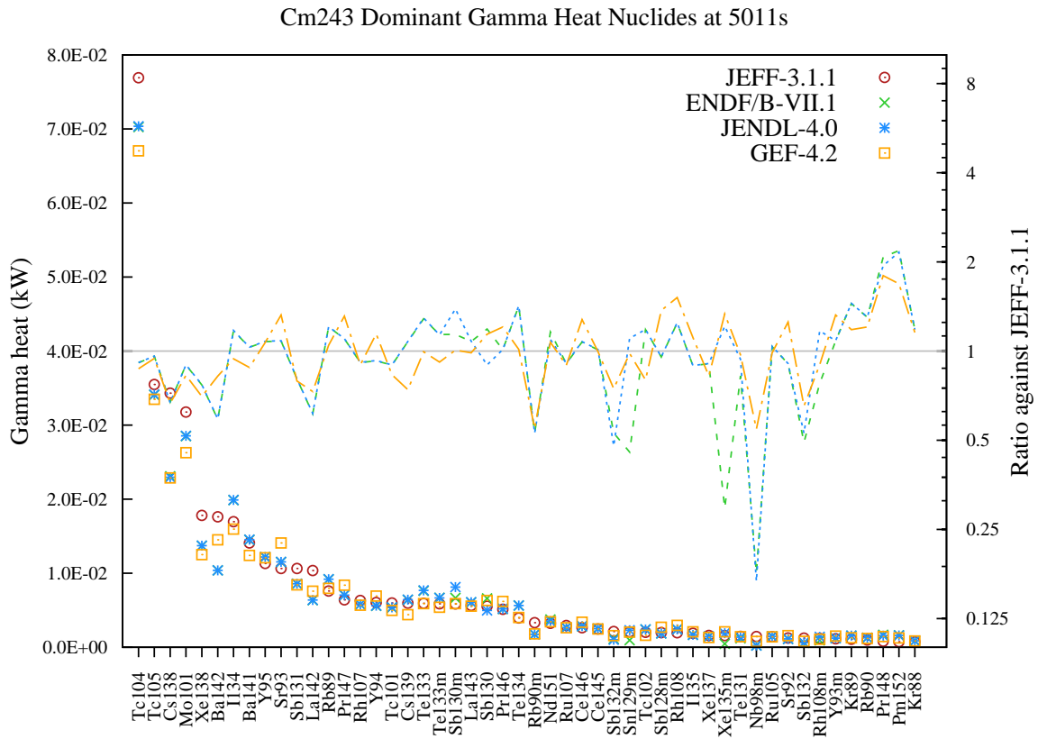
Figure 205: Gamma decay heat (in kW) fission yield comparison for Cm243 fission pulse after 5011s cooling.
