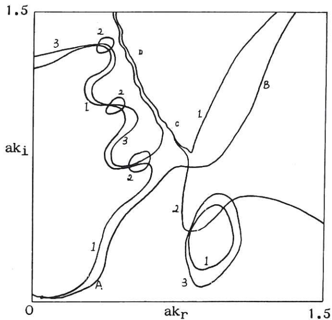
CLM-P 55 Fig. 3 The dispersion function D = U + iV (equation 33) in the complex k plane for a travelling wave with m = 1 and \Omega_e \tau = 10 curve 1 : contours of U = 0 curve 2 : contours of V = 0 curve 3 : contours of V = 0.1 Curve AB: Contour corresponding to the trivial solution for which wave field vanishes, i.e. \beta_1 = \beta_2
