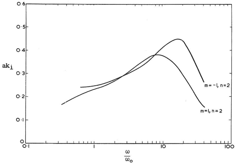
CLM-P 55 Fig. 6 The attenuation constants for travelling waves with m = 1 and m = -1, n = 2 and \Omega_e \tau = 30
