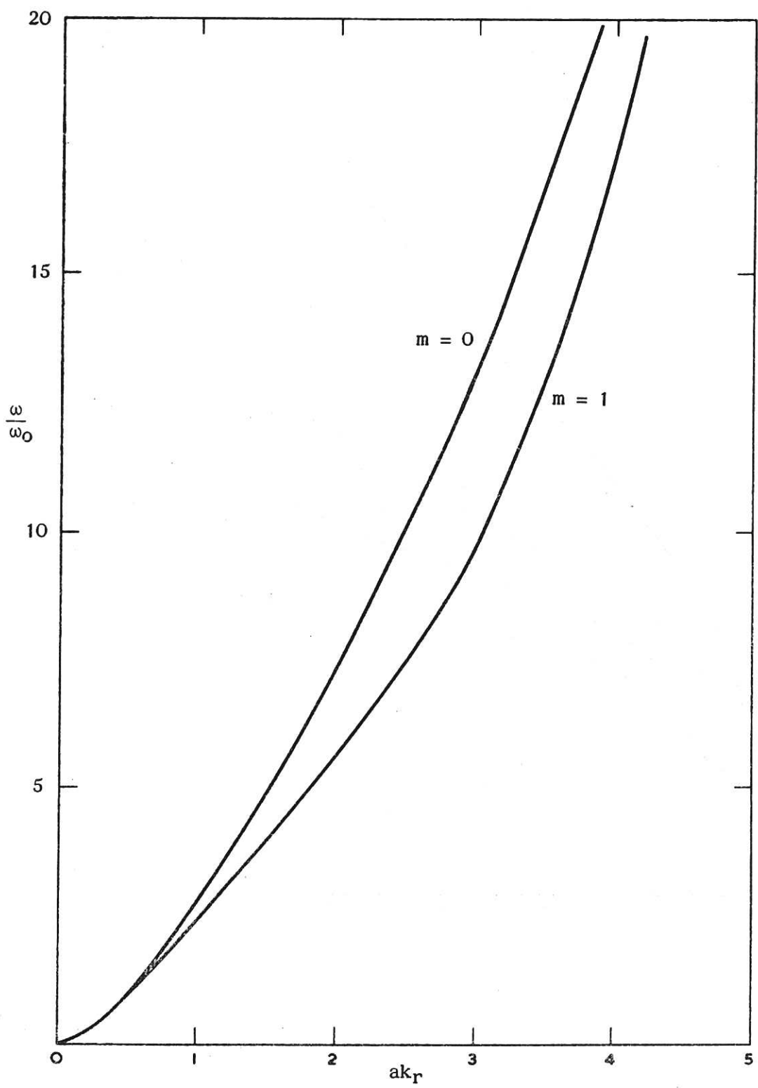
CLM-P 55 Fig. 7 The dispersion relation for standing waves with m = 0, m = 1 and n = 1
