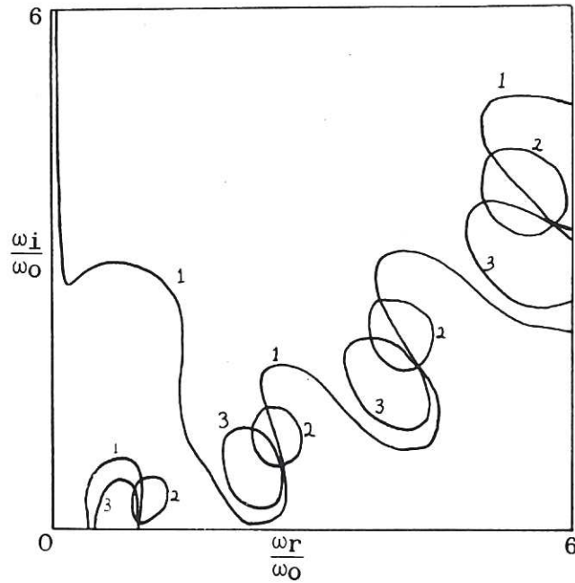
CLM-P 55 Fig. 2 The dispersion function D = U + iV (equation 33) in the complex \omega plane for a standing wave with m = 1 and \Omega_e \tau = 10 curve 1 : contours of U = 0 curve 2 : contours of V = 0 curve 3 : contours of V = 0.1
