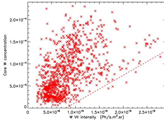
Figure 21. Core W concentration against 261.39 Å, W VII line intensity averaged over intervals of 0.25 s.
