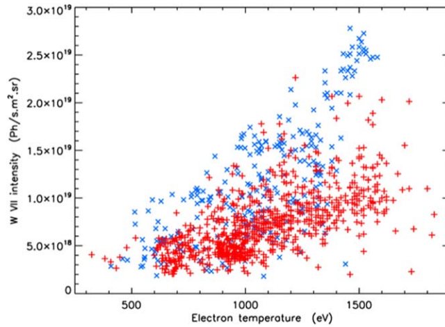
Figure 20. Intensity of 261.39 Å, W VII line averaged over 0.25 s intervals against electron temperature measured using high resolution Thomson scattering at a major radius of 3.7 m. × plasma-wall distance (measured from wall point R = 3.33 m, z = -1.07 m) less than 15 mm (in blue); + plasma-wall distance greater than 15 mm (in red).
