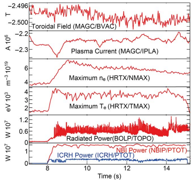
Figure 23. Plasma parameters for pulse 94605.
