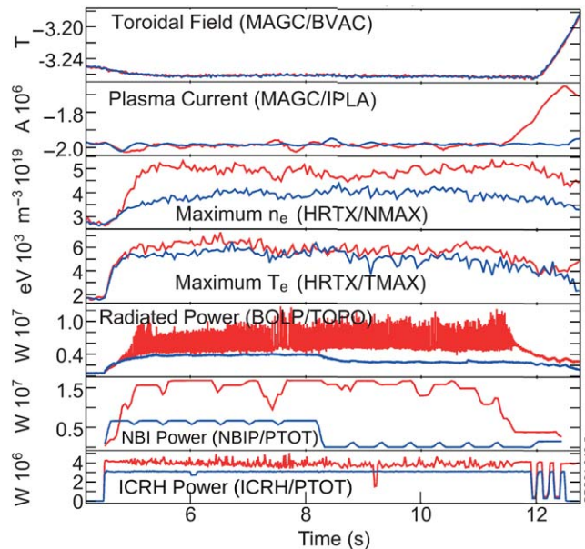
Figure 27. Plasma parameters for pulses 95457 (in blue) and 95458 (in red).
