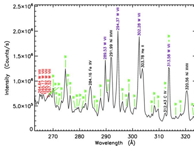
Figure 6. Spectrum of pulse 95012 during a large influx at 14.37 s covering a wavelength range of 263 to 324 Å.
