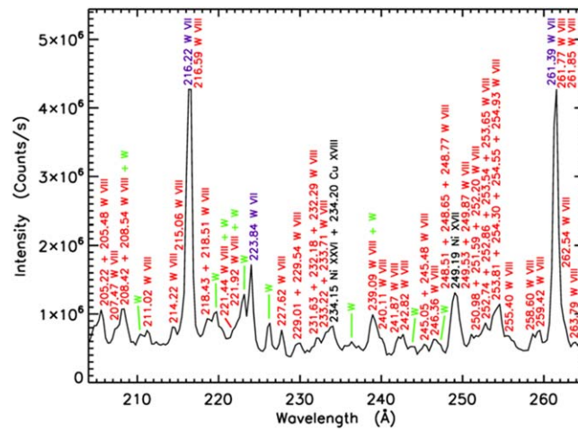
Figure 5. Spectrum of pulse 95012 during a large influx at 14.37 s covering a wavelength range of 204 to 265 Å.
