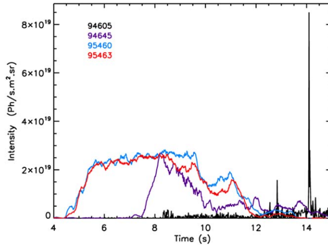
Figure 22. Time histories of intensity of the 261.39 Å, W VII line in pulses 94605, 94645, 95460 and 95463.
