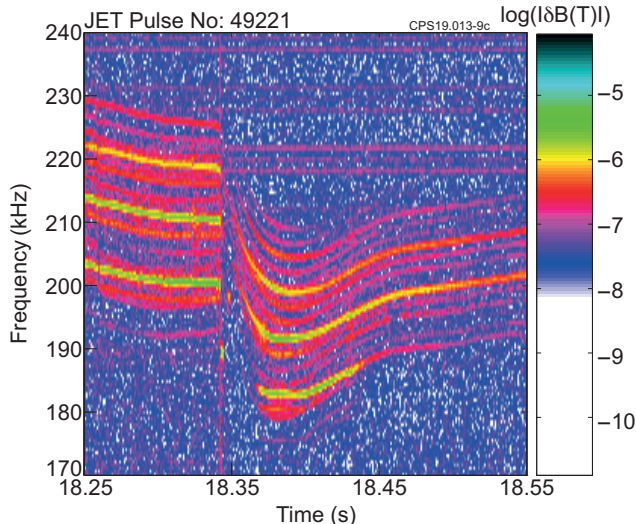
Figure 6: Magnetic spectrograph showing the amplitude of the magnetic perturbation caused by a TAE in discharge #49221. A pellet was injected on the outboard track at time t = 18.34 s.
