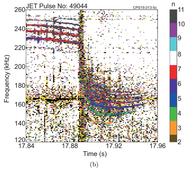
Figure 5: (a) Magnetic spectrograph showing the amplitude of the magnetic perturbation caused by a TAE in discharge #49044; (b) a phase magnetic spectrograph showing the toroidal mode numbers of the same TAE. A pellet was injected on the inboard track at time t = 17.89 s.
