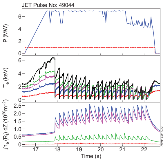
Figure 4: Heating waveforms and plasma parameters for JET discharge #49044. Top: ICRH (solid blue) and NBI (dashed red) heating power, P . Middle: Electron temperature T_e as measured by ECE radiometry at R = 3.06, 3.29, 3.40, 3.54, and 3.78 m (from top to bottom). Bottom: Line integrated electron density \int n_e(R_I) dZ as measured by far infrared interferometry along the line of sights at radii R_I , shown in Figure 1.
