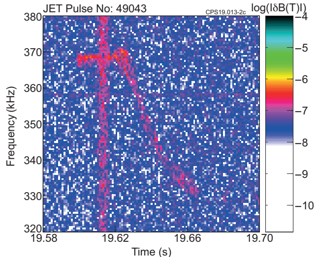
Figure 7: Magnetic spectrograph showing the amplitude of the magnetic perturbation due to an EAE in discharge #49043. A pellet was injected on the inboard track at time t = 19.62 s.
