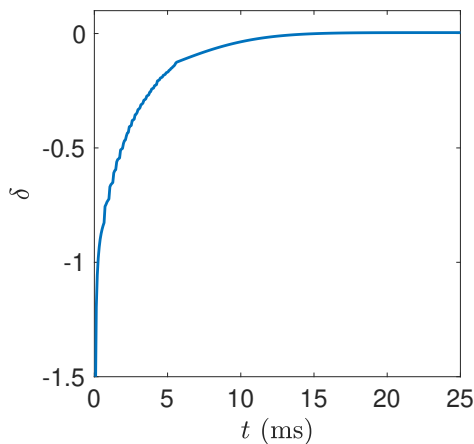
Figure 16: The size of poloidal inhomogeneity, \delta , is initially a large negative number due to the initial position of the wake on the high field side. \delta \rightarrow 0 as the wake expands with time, t .
