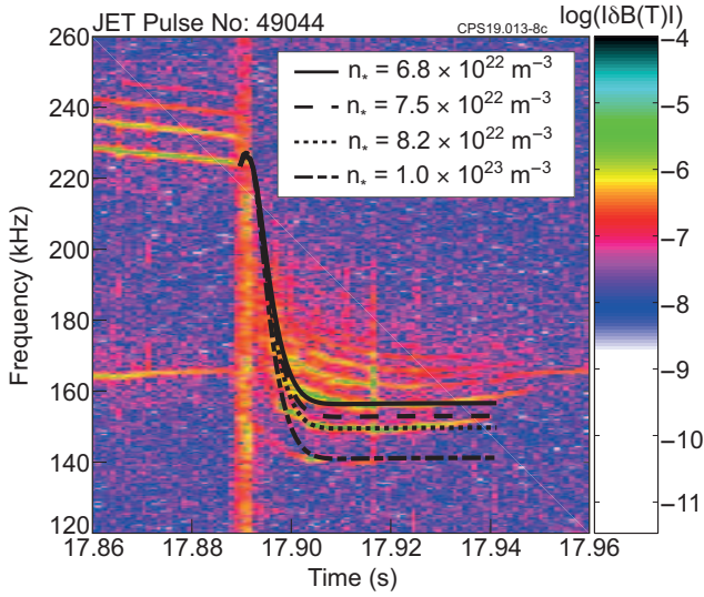
Figure 13: As the wake expands around the tokamak, the frequency of the n = 6 TAE drops. Numerical estimates of the TAE eigenfrequency (black) are overlaid on the experimental magnetic spectrograph for shot #49044. The eigenfrequency is calculated for four estimates of the initial ion density n_* .
