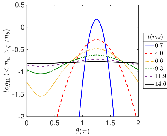
Figure 14: The logarithm of the wake density averaged over toroidal angle \zeta normalised to the background density n_b , \log_{10}(\langle n_w \rangle_\zeta / n_b) , as a function of poloidal angle, \theta .
