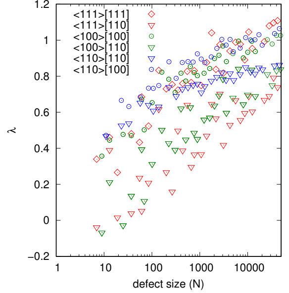
FIG. 15. Calculated surface area correction for a planar void due to the perimeter strip. The surface area measure by qhull is A = 2\pi r^2/\zeta + \lambda p\zeta b , where p is the perimeter length.
