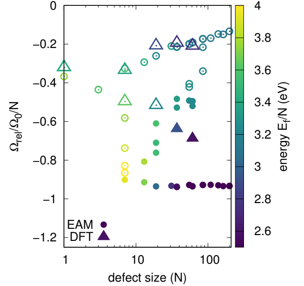
FIG. 13. The relaxation volume per vacancy of \frac{1}{2}\langle 111 \rangle [111] vacancy loops (closed symbols) and \frac{1}{2}\langle 111 \rangle [111] planar voids (open symbols) computed with DFT (this work) and the empirical embedded-atom MNB potential [53]. Points are coloured by formation energy per point defect.
