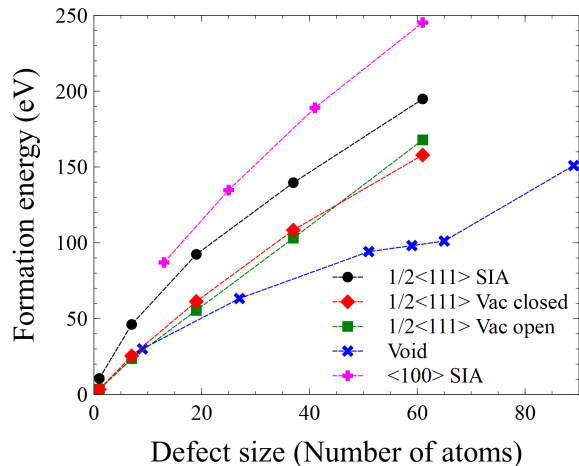
FIG. 2. Formation energies of \frac{1}{2}\langle 111 \rangle SIA, vacancy open and vacancy closed loops, \langle 100 \rangle SIA loops and voids, calculated using density functional theory package OpenMX. Lines connecting the data points are not interpolations, rather they are shown to guide the eye.
