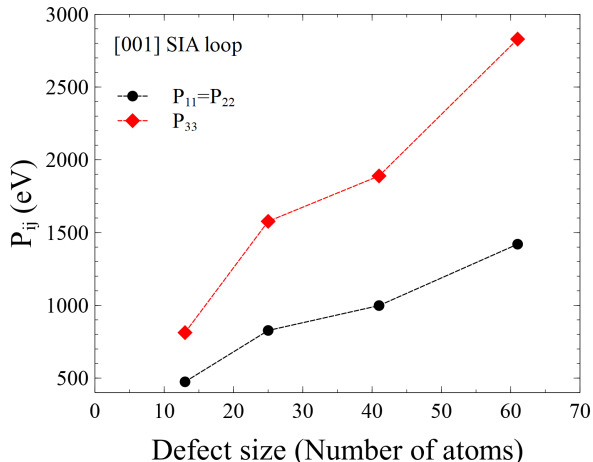
FIG. 4. Elastic dipole tensors of \langle 100 \rangle SIA loops with the Burgers vector \mathbf{b} = [001] , calculated using OpenMX. All the elements not shown in the Figure, vanish because of symmetry considerations.
