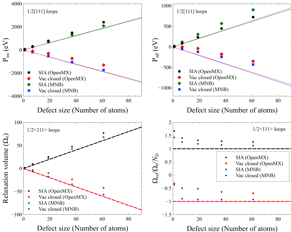
FIG. 8. Calculated elastic dipole tensor P_{ij} and relaxation volume of \frac{1}{2}\langle 111 \rangle SIA and vacancy closed loops with \mathbf{b} = \frac{1}{2}\langle 111 \rangle using OpenMX and MNB potential, and linear elasticity predictions according to Eq. (13) and (14). The fact that the relaxation volumes of loops derived from simulations are larger than predictions derived from the theory of elasticity, highlights the contribution to the relaxation volumes from the highly distorted core regions at the perimeter of the loops. The contribution to the relaxation volume of dislocation loops from the core effects results in that interstitial loops appear somewhat larger, and vacancy loops somewhat smaller than what should be expected from the elasticity considerations.
