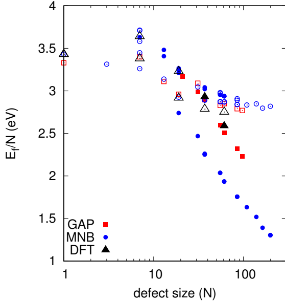
FIG. 12. The formation energy E_f per vacancy of \frac{1}{2}\langle 111 \rangle [111] vacancy closed loops (closed symbols) and \frac{1}{2}\langle 111 \rangle [111] planar voids (open symbols) computed with DFT (this work), results taken from a newly developed GAP potential in Ref. [55], and the empirical embedded-atom MNB potential [53]. Note that the MNB potential has a higher vacancy formation energy than the other two, so has been shifted down by 0.3eV.
