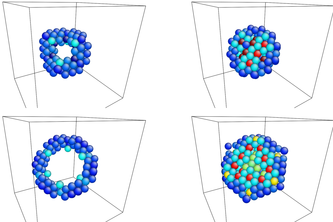
FIG. 5. Atomic configuration of a circular vacancy \frac{1}{2}\langle 111 \rangle loop. Bulk atoms were filtered out according to the central symmetry parameter criterion. (Top left) 37 atoms closed loop. (Top right) 37 atoms open loop. (Bottom left) 61 atoms closed loop. (Bottom right) 61 atoms open loop.
