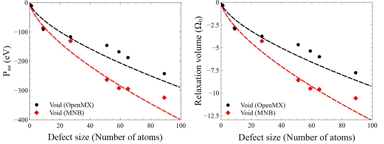
FIG. 11. Elastic dipole tensors and relaxation volumes of voids calculated using OpenMX and MNB potential, plotted together with linear elasticity predictions derived from Eqns. (20) and (19). All the off-diagonal elements of dipole tensors vanish because of symmetry considerations.
