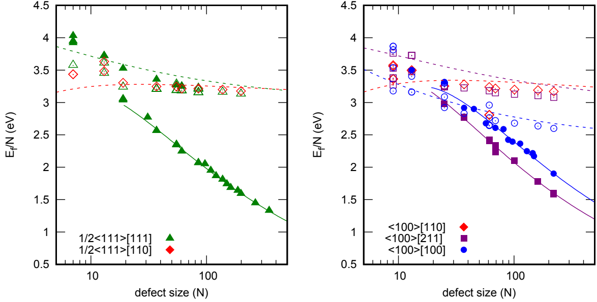
FIG. 14. Formation energy of vacancy defects computed with the MNB potential. Dislocation loops, determined using DXA, are shown as closed symbols, and planar voids as open symbols. Solid lines are empirical fits to dislocation loop energy ( see table III ) and dashed lines use the loop geometry and surface energy only ( equation C3).
