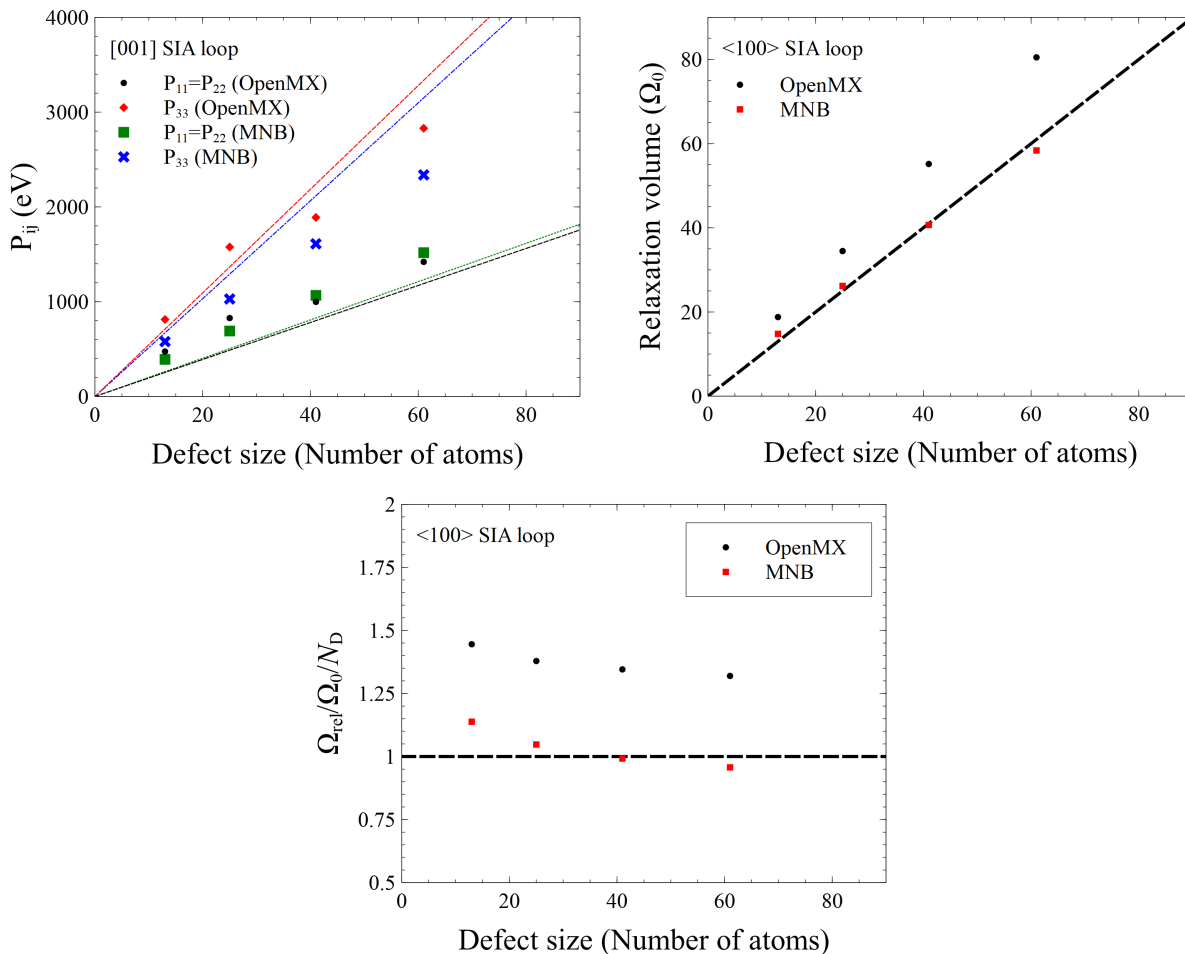
FIG. 9. Calculated elastic dipole tensor P_{ij} and relaxation volume of \langle 100 \rangle SIA loops with \mathbf{b} = [001] using OpenMX and MNB potential, and linear elasticity predictions according to Eqns. (13) and (14).
