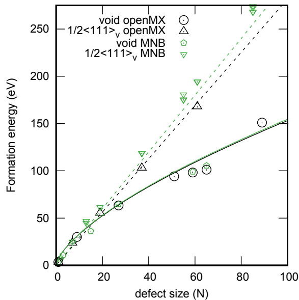
FIG. 10. Formation energies of \frac{1}{2}\langle 111 \rangle open vacancy loops and voids calculated using OpenMX and MNB potential, compared with values derived from Eqs. (16) and (18).
