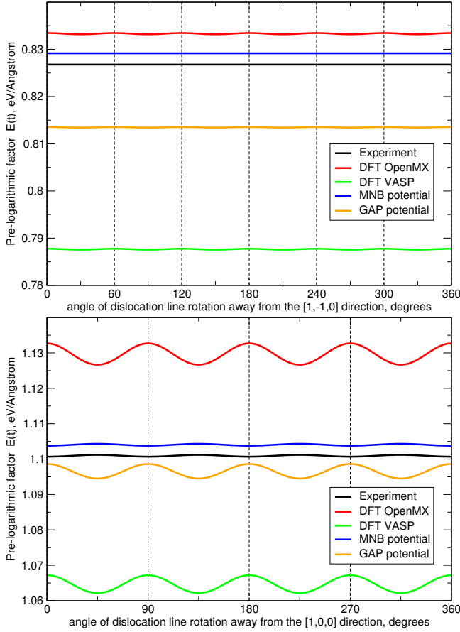
FIG. 6. Pre-logarithmic factor E(\mathbf{t}) entering the first term of equation (5) plotted as a function of the orientation of the tangent vector of the dislocation line. The curves are computed using equation (6) for the (top) \frac{1}{2}\langle 111 \rangle and (bottom) \langle 001 \rangle edge dislocations using the elastic parameters given in Table I. The orientation-average values of pre-logarithmic factors are summarised in Table II.
