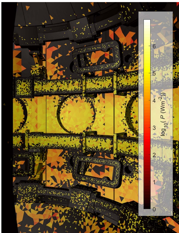
Figure 12. Power loads from fast CX atoms estimated by ASCOT on a sector of the wall.
