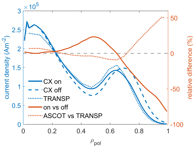
Figure 9. Radial profiles of electron-shielded current drive by beam ions simulated by ASCOT, with and without the CX model, and by TRANSP. Relative differences are shown on a separate scale.
