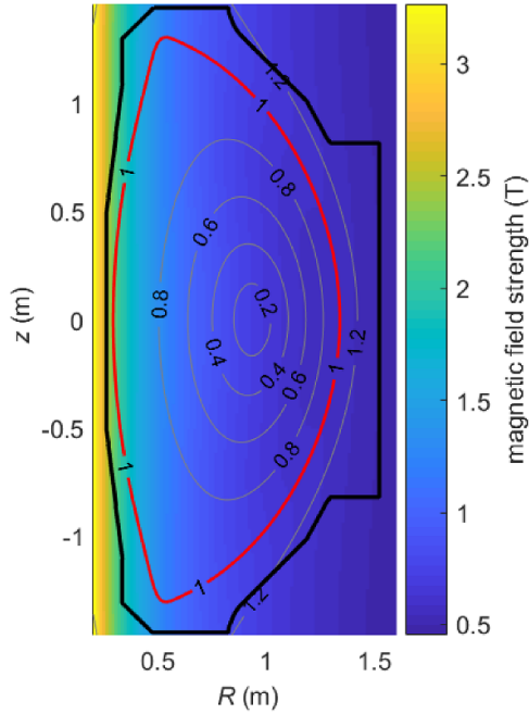
Figure 1. Total magnetic field strength, separatrix (red), other flux surfaces (gray) and reduced 2D wall (black) [30] in the Rz plane, where R is the major radius and z the vertical coordinate. The flux surfaces are labelled with the normalized poloidal flux
