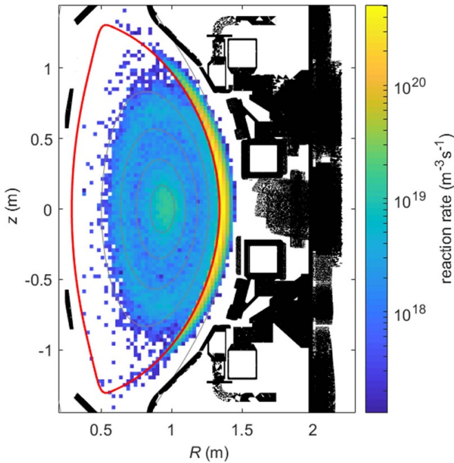
Figure 11. 2D projection of the reaction rate of CX neutralization of beam ions simulated by ASCOT. The same flux surfaces as in figure 1 and a 2D projection of the 3D wall (black) are shown.
