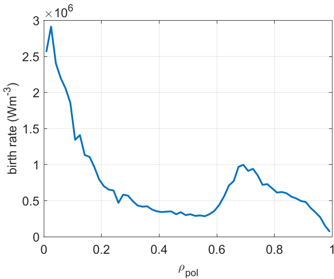
Figure 4. Radial beam-ion birth profile.
