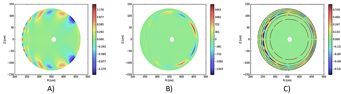
Figure.1 The non-axisymmetric A) normal magnetic field \delta B_n [Gs], B) pressure p [Ba] and C) parallel current density \delta j_{\parallel} [Frs -1 cm -3 ] as obtained for an even N = 3 external resonant MP field of the \beta_N = 2.36 equilibrium.
