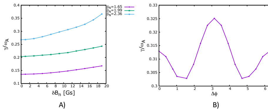
Figure.2 A) The normalized growth rate \gamma/\omega_A of a n = 15 ballooning mode as a function of applied resonant N = 3 MP normal field \delta B_n for different values of normalized beta \beta_N . B) The normalized growth rate \gamma/\omega_A as a function normal field phase \Delta\phi for \delta B_n = 10 [Gs] of the \beta_N = 2.36 equilibrium case.
