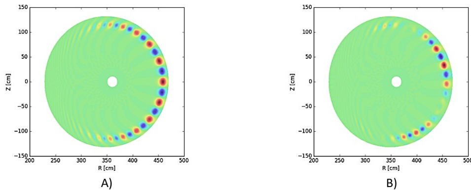
Figure.3 The mode structure of A) an axisymmetric n = 15 PB mode and the mode structure of B) a non-axisymmetric n = 15 PB mode under the influence of a N = 3 MP with \Delta\phi = 0 , \delta B_n = 10 [Gs] of the \beta_N = 2.36 equilibrium case.
