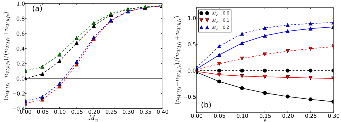
Figure 9. (a) In-out asymmetry of W^{33+} as function of the hydrogen Mach number M_\phi for \mathcal{T}_H = 8 and \epsilon = 0.1 (the inverse-aspect ratio of the magnetic surface). The colours have the same meaning of figures 6-8. (b) In-out asymmetry of W^{33+} as function of the inverse-aspect ratio, \epsilon , of the magnetic surface tangent to the IC resonance layer and for \mathcal{T}_H = 8 . In (b) the dashed lines show the corresponding in-out asymmetry in the absence of ICRF effects.
