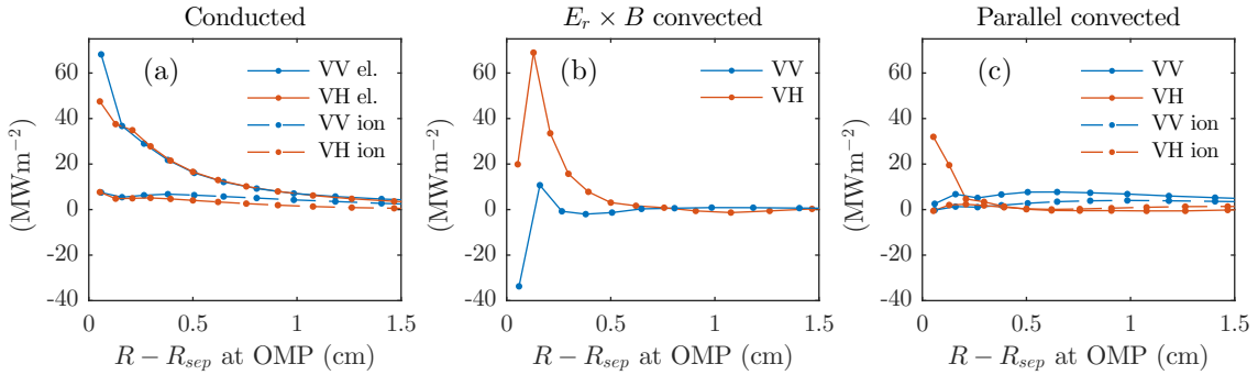
Figure 7. The components of q_{\theta u}(B_u/B_{\theta u}) for the default VV and VH simulations, in the presence of drifts and parallel current. LEGEND NEEDS TO SAY EL.
