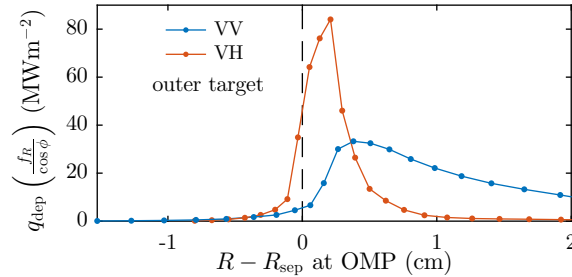
Figure 9. Deposited heat flux at the outer divertor in the VV and VH simulations, without accounting for total flux expansion and target inclination angle.
