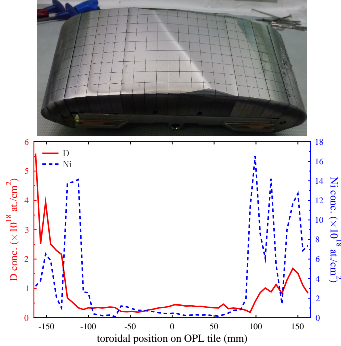
FIG. 1: (Color online) Toroidal distribution of D on the mid-plane OPL tile as obtained with NRA measurements and analyzed with WiNDF. Also shown the Ni marker interlayer results from EBS and PIXE measurement: low Ni concentration values correlate with thinning or erosion of the OPL tile surface. The centre part region ( -60 mm. . . +60 mm) of the OPL is the eroded zone and has low D concentration values of \sim 3.3 \times 10^{17} at./cm 2 .
