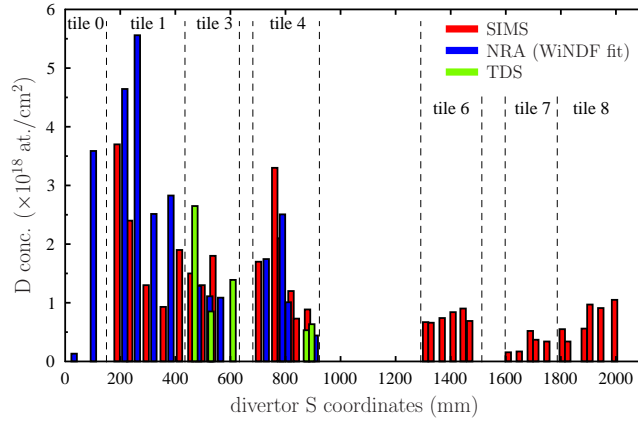
FIG. 3: (Color online) The poloidal distribution of retained D in the JET-ILW divertor tiles as measured with SIMS, NRA and TDS. D concentration is presented as a function of S coordinates. The divertor tile positions at corresponding S coordinates are separated with dashed lines.
