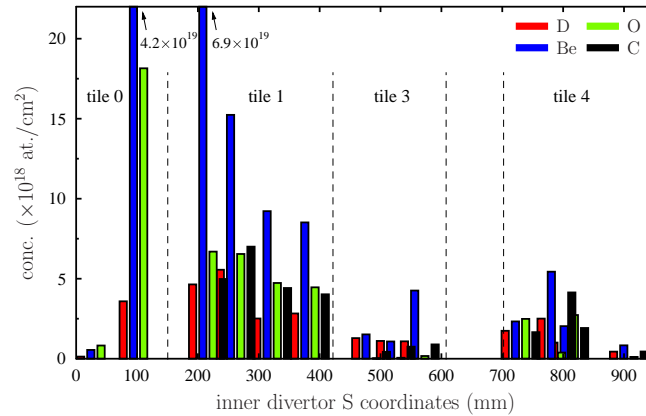
FIG. 4: (Color online) The D, Be, C and O poloidal distribution in the JET-ILW inner divertor tiles as a function of S coordinate. The concentrations shown were obtained with NRA and EBS and fitted with WinDF. Most of the deposition takes place on the plasma wetted region on tile 0 (S coordinates 60...160 mm) and on the apron of tile 1 (162...230 mm), where also most of the D co-deposition takes place \sim 5 \times 10^{18} at./cm 2 . The plasma shadowed region on tile 0 ( < 60 mm) show concentrations for D: 1.3 \times 10^{17} at./cm 2 , Be: 6 \times 10^{17} at./cm 2 and O: 0.8 \times 10^{17} at./cm 2 , which are similar as obtained for tile 4 shadowed region ( > 900 mm).
