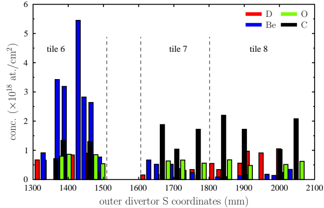
FIG. 5: (Color online) The D, Be, C and O poloidal distribution in the JET-ILW outer divertor tiles as a function of S coordinate. D concentrations were obtained with SIMS and Be with NRA [7], C and O impurities with ERDA [8]. D retention values do not exceed 1 \times 10^{18} at./cm 2 . Highest Be values were measured on the sloping part of Tile 6.
