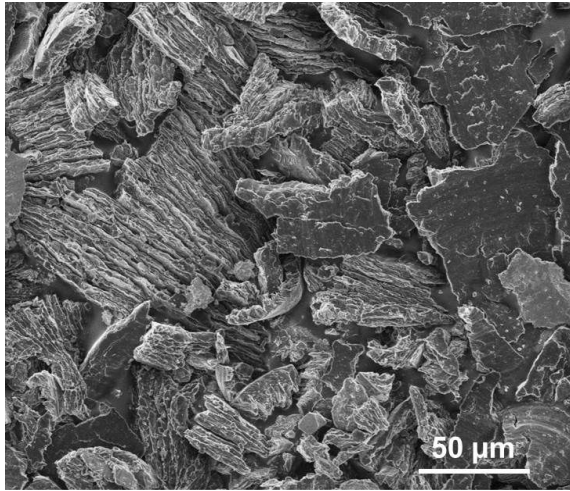
Figure 2. Be particulates produced during cutting.
