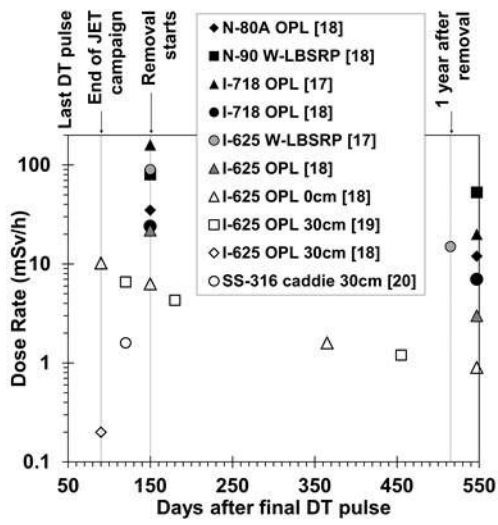
Figure 3. Summary of contact dose rates (closed black and grey symbols) and shutdown dose rate (open symbols) data from [17][18][19][20].
