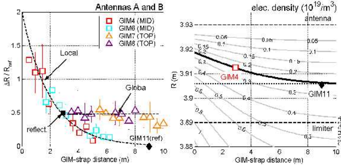
Figure 4: (left) Relative coupling resistance increase of the individual antenna straps with respect to a divertor fuelled discharge (GIM11, 1.85 \times 10^{22} e/s) for two mid-plane (GIM4 and GIM6, 1.65 \times 10^{22} e/s) and two top gas injection pulses (GIM7 and GIM8, 1.6 \times 10^{22} e/s) as function of the toroidal GIM-strap distance; (right) 2D density profile reconstructed from RF coupling modelling by finding the density profiles (parameterized to the reflectometry data) that best fit the experimental coupling measurements in each toroidal position for mid-plane gas injection. The thick solid curve represents the cut-off density for the mid-plane gas injection case while the dotted line indicates the cut-off position if divertor fuelling would be used (assuming toroidally homogeneous far-SOL density).
