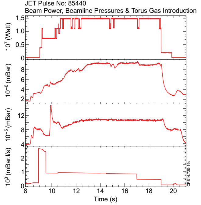
Figure 7: Actively cooled duct. 8x 125kV EP2 PINIs ~ 110kV, 15.2MW/10.9s. Beam power, Duct and NIB pressures (mbar) and Torus gas injection rate. JET Pulse Number: 85440.
