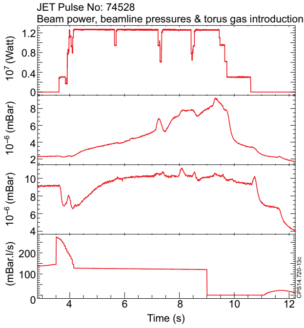
Figure 5: Inertial Duct. 8x 130kV EP1 PINIs 111–118kV, 12.7MW. Beam power, Duct and NIB pressures (mbar) and Torus gas injection rate. JET Pulse Number: 74528.
