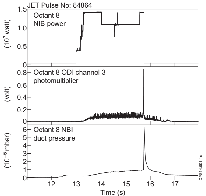
Figure 3: Doppler shifted D_\alpha emission measured from the neutral beams duct during a fast pressure excursion [JET pulse 84864].
