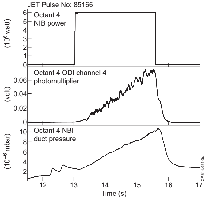
Figure 2: Doppler shifted D_\alpha emission measured from the neutral beams duct with constant beam power and increasing duct pressure [JET pulse 85166].
