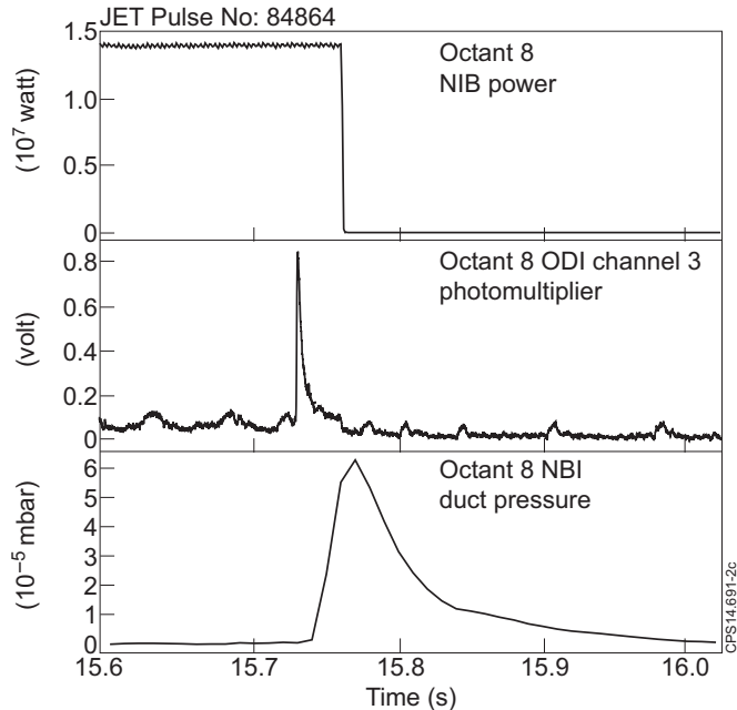
Figure 4: Comparison of time response of the Doppler shifted D_{\alpha} emission and the duct penning gauge during a fast pressure excursion [JET pulse 84864].
