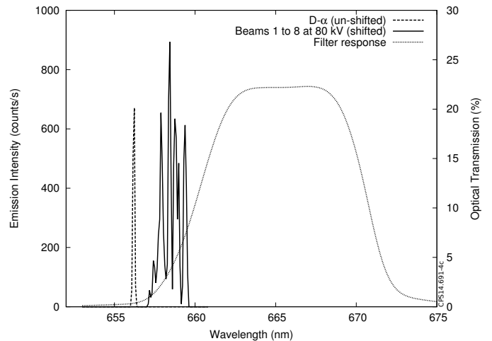
Figure 1: Calculated beam emission for 80 kV deuterium beams. The Doppler shifted emission from full, half, and one third energy components is plotted. The transmission of the angle tuned (15°) interference filter is included.
