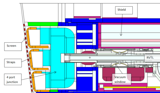
Fig. 1. ICH MCNP model, front of single quadrant.
