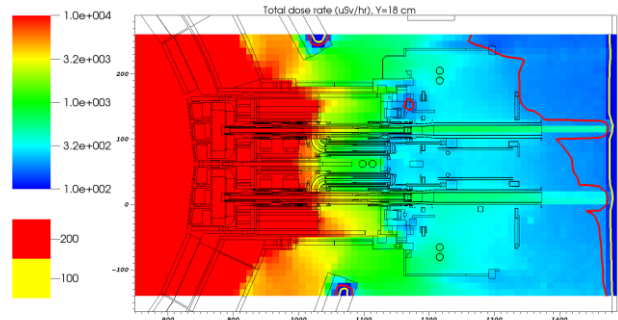
Fig. 3. Total gamma dose rate (global neutron transport and activation), 10^6 s decay time (Y=18 cm)
