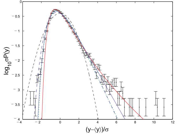
Fig. 8. PDF for Cygnus X-1 X-ray time-series, normalised with respect to \langle y \rangle and \sigma ; black dashed line Gaussian, dotted (green dotted) line log-normal, thick (red) solid line Fréchet a = 1.1 , thin solid (blue dashed) line Gumbel a = 1 , dot-dash (blue solid) line Gumbel a = 2 . The colour codes refer to the electronic version of this figure.
