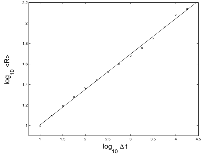
Fig. 9. Logarithmic plot of growth of range R(\Delta t) (Eq. (1)) with \Delta t for Cygnus X-1 X-ray time-series; slope gives Hurst exponent 0.34 < H < 0.36 .
