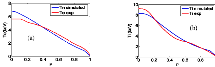
FIGURE 3. Comparison between experimental electron temperature profile for shot 77895 and simulated one (a) Comparison between experimental ion temperature profile for shot 77895 and simulated one (b).
