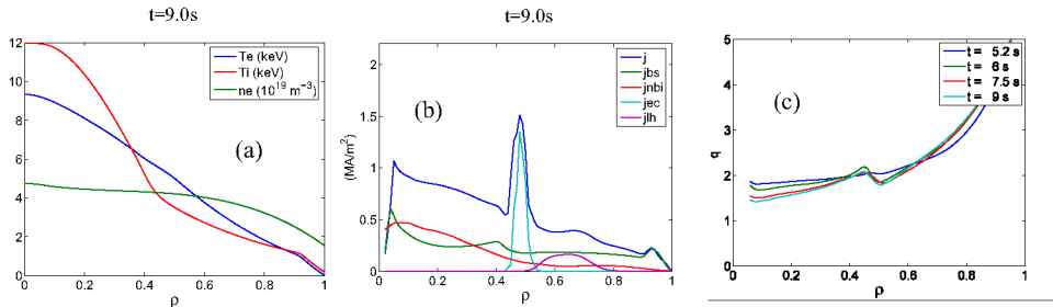
FIGURE 4. Electron, ion temperature and density profiles at t=9s (a). Total current ( j ), bootstrap current ( jbs ), NBI ( jnbi ), lower hybrid ( jlh ) and electron cyclotron ( jec ) current drive density profiles at t=9s (b). Evolution of the q profile calculated with CRONOS(c)
