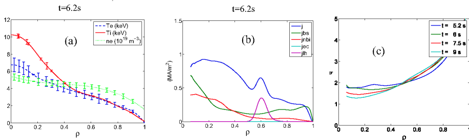
FIGURE 1. Electron, ion temperature and density profiles at t=6.2s for shot 77895 (a). Total current ( j ), bootstrap current ( j_{bs} ), NBI ( j_{nbi} ) and lower hybrid ( j_{lh} ) current drive density profiles at t=6.2s for shot 77895 (b). Evolution of the q profile calculated with CRONOS for shot 77895 (c)
