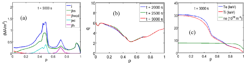
FIGURE 6. Total current ( j ), bootstrap current ( j_{bs} ), fast wave ( j_{fwd} ), electron cyclotron ( j_{ec} ) and lower hybrid ( j_{lh} ) current drive density profiles at t=3000 s(a). Evolution of the q profile (b). Electron, ion temperature and density profiles at t=3000 s. (c)
