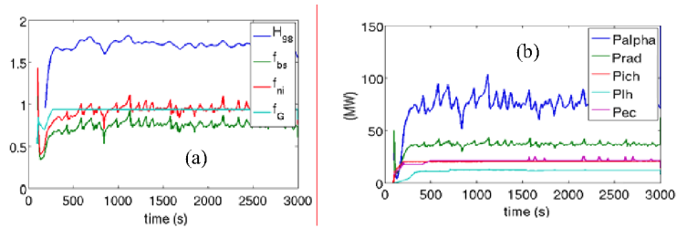
FIGURE 5. Time evolution of H_{98} , f_{bs} , f_{ni} and f_G . (a) Time evolution of alpha ( P_{alpha} ), radiated ( P_{rad} ), ICRH ( P_{ich} ), LH ( P_{lh} ) and EC ( P_{ec} ) power (b).
