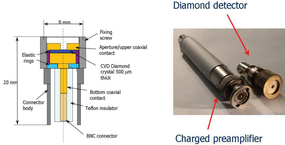
FIGURE 1. Diamond detector and preamplifier
