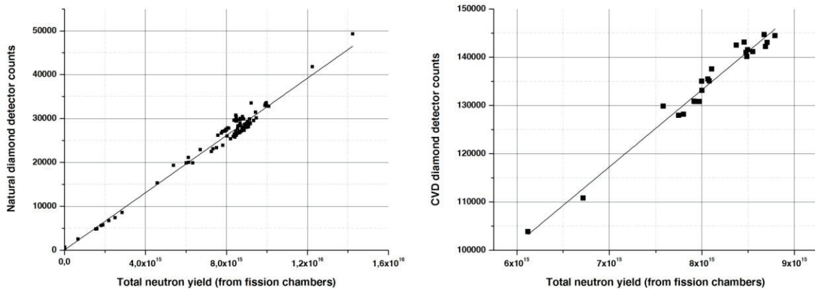
FIGURE 4. Counts of natural (left) and CVD diamond detectors and total neutron yield calculated from fission chambers JET diagnostic in different JET pulses
