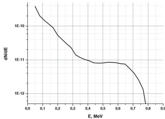
FIGURE 2. Calculated response of the CVD diamond detector for DD-plasma based on MCNP spectra
