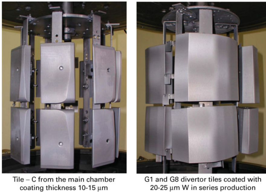
Fig. 8. Tungsten coated CFC tiles in the coating device. 29
