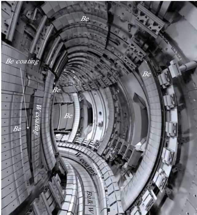
Fig. 1. Material configuration for the ITER-like Wall.
