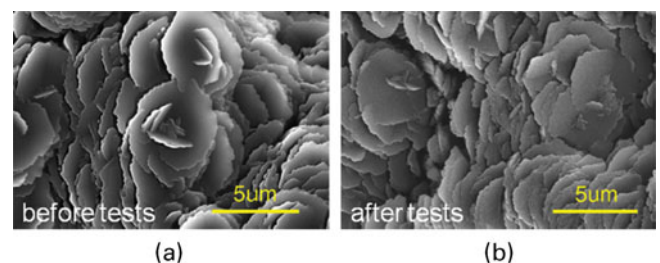
Fig. 3. Beryllium coatings on INCONEL substrate ( 7\text{--}9 \mu\text{m} thick films) Thermal loads 1 \text{ MW/m}^2 for 10 s, 50 cycles. 16
