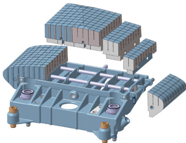
Fig. 2. Detailed view of an outer poloidal limiter (S65J HIP beryllium) with tile carrier fixing bolts and vacuum cast INCONEL 625 support.
