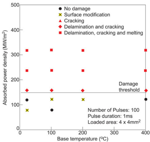
Fig. 9. Failure occurrence of tungsten coatings under ELM-like heat loads in dependence on absorbed power density and test temperature. 32
