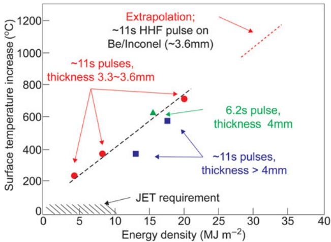
Fig. 4. Surface temperature increase as a function of deposited energy (thickness indicates the thickness of the INCONEL substrate). 16
