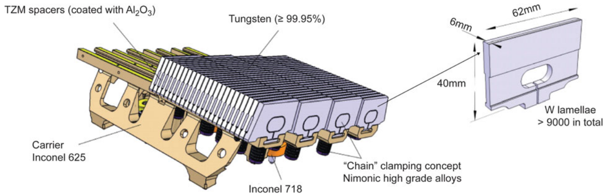
Fig. 5. Schematic picture of a bulk tungsten divertor tile (left side); in total over 9000 shaped bulk tungsten lamellas (right side) are installed in the JET-ITER-like Wall.
