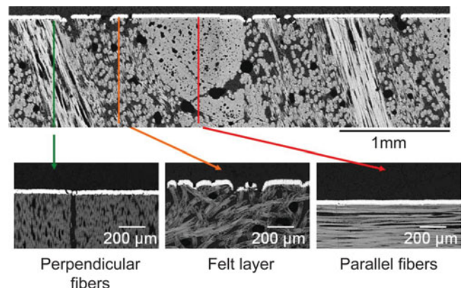
Fig. 7. Metallographic images of longitudinal (top) and transverse (bottom row) cross sections of the CFC substrate and the tungsten coating. 30
