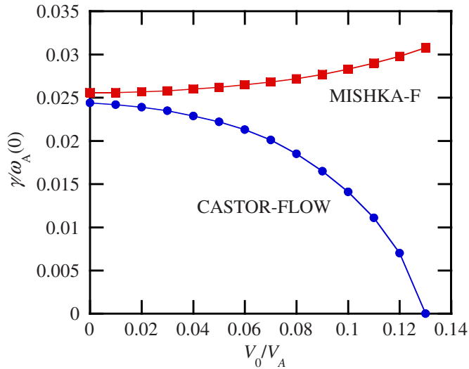
FIG. 12. (Color online) The effect of toroidal rotation on the n=1 internal kink mode growth rate for the equilibrium profiles shown in Fig. 11, calculated with both the static (MISHKA-F) and flowing (CASTOR-FLOW) treatments. It can be seen that including flow in the equilibrium has a significant effect on the stability boundary for this kind of equilibrium.
