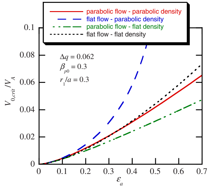
FIG. 7. (Color online) Critical rotation velocity V_{0,crit} required for stabilization of the kink mode vs the inverse aspect ratio \epsilon_a . V_{0,crit} is shown for the four combinations of the profiles of \rho_0 and \Omega indicated and is calculated from Eq. (20) using \sigma_1 = \sigma_2 = 1 , q_0 = 0.938 , r_1/a = 0.3 , \beta_{p0} = 0.3 , and \beta_0 = 2\beta_{p0}\epsilon_a^2 .
