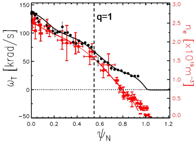
FIG. 9. (Color online) The density and rotation profiles in MAST discharge 18416.
