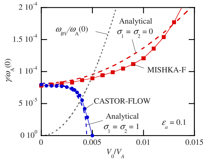
FIG. 1. (Color online) Growth rate vs rotation velocity at the axis calculated for a self-consistent equilibrium ( \sigma_1 = \sigma_2 = 1 ) and for a nonself-consistent equilibrium ( \sigma_1 = \sigma_2 = 0 ). The dashed curves show the analytical predictions from Eq. (20) while the symbols give the numerical results obtained with the two different numerical codes indicated. The plasma parameters are \varepsilon_a = 0.1 , q_0 = 0.938 , r_1/a = 0.3 , \beta_{p0} = 0.3 , and \beta_0 = 0.66\% and the density and rotation profiles are both parabolic. The dotted curve shows the BV frequency in Eq. (1), and stabilization in the consistent case is seen to occur approximately when this frequency exceeds the static growth rate.
