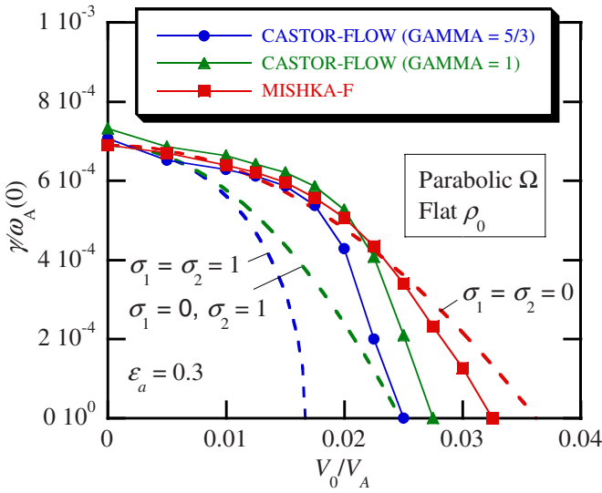
FIG. 5. (Color online) Growth rate vs rotation velocity at the axis in the case of a flat density and a parabolic rotation profile with \epsilon_\Omega = \epsilon_a = 0.3 . Other plasma parameters are q_0 = 0.938 , r_1/a = 0.3 , \beta_{p0} = 0.3 , and \beta_0 = 5.6\% and stabilization occurs both for inconsistent ( \sigma_1 = \sigma_2 = 0 ) and consistent ( \sigma_1 = \sigma_2 = 1 ) equilibria. The intermediate case \sigma_1 = 0 and \sigma_2 = 1 is simulated numerically by running CASTOR-FLOW with the adiabatic constant \Gamma = 1 , and the result is shown by the triangles. The dashed curves are calculated analytically and the symbols with the numerical codes indicated.
