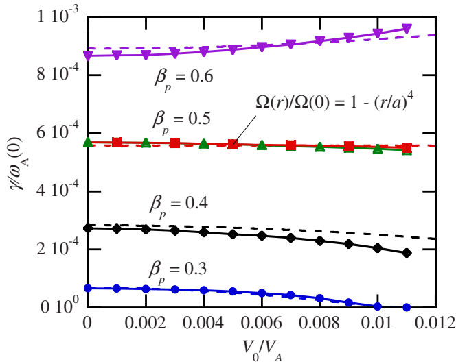
FIG. 2. (Color online) Growth rate vs rotation velocity at the axis for an inconsistent equilibrium \sigma_1 = \sigma_2 = 0 with \varepsilon_a = 0.1 , q_0 = 0.95 , r_1/a = 0.3 , and different \beta_p . The density is flat and the rotation profile parabolic. In addition, for \beta_p = 0.5 the growth rate is computed also for the rotation profile \Omega(r)/\Omega(0) = 1 - (r/a)^4 , shown by the squares. The dashed curves are calculated analytically and the symbols with MISHKA-F.
