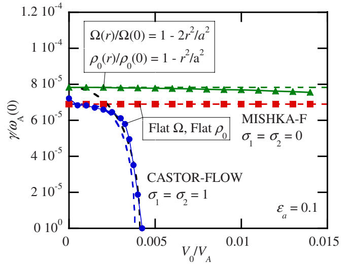
FIG. 3. (Color online) Growth rate vs rotation velocity at the axis for two combinations of the profiles of \rho_0 and \Omega such that the flow does not modify the static growth rate when an inconsistent equilibrium ( \sigma_1 = \sigma_2 = 0 ) is used. For comparison, the corresponding analytical growth rates in the consistent case ( \sigma_1 = \sigma_2 = 1 ) are also shown for these two combinations of profiles, together with the CASTOR-FLOW result for the case when the profiles of both \rho_0 and \Omega are flat. The plasma parameters are \varepsilon_a = 0.1 , q_0 = 0.938 , r_1/a = 0.3 , \beta_{p0} = 0.3 , and \beta_0 = 0.66\% . The dashed curves are calculated analytically and the symbols with the numerical codes indicated.
