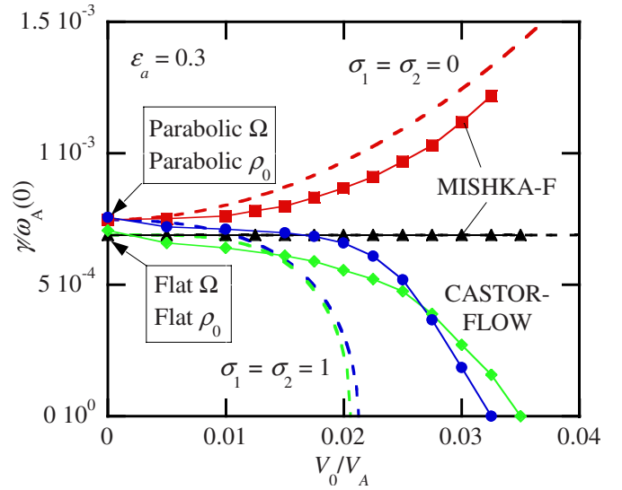
FIG. 6. (Color online) Growth rate vs rotation velocity at the axis for two combinations of the profiles of \rho_0 and \Omega in a plasma with \epsilon_a = 0.3 , q_0 = 0.938 , r_1/a = 0.3 , \beta_{p0} = 0.3 , and \beta_0 = 5.6\% . Results both for inconsistent (upper curves) and consistent (lower curves) equilibria are shown. The dashed curves are calculated analytically and the symbols with the numerical codes indicated.
