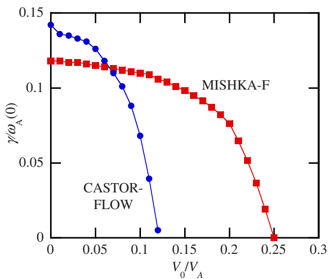
FIG. 10. (Color online) The effect of toroidal rotation on the n=1 internal kink mode growth rate in the MAST equilibrium in Fig. 9, calculated with either static (HELENA+MISHKA-F) or flowing (DIVA+CASTOR-FLOW) equilibria. It can be seen that including flow in the equilibrium has a significant effect on the stability boundary for this MAST plasma.
