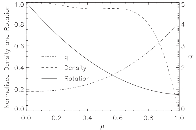
FIG. 11. Density, rotation, and q -profiles for a typical conventional aspect ratio tokamak plasma.
