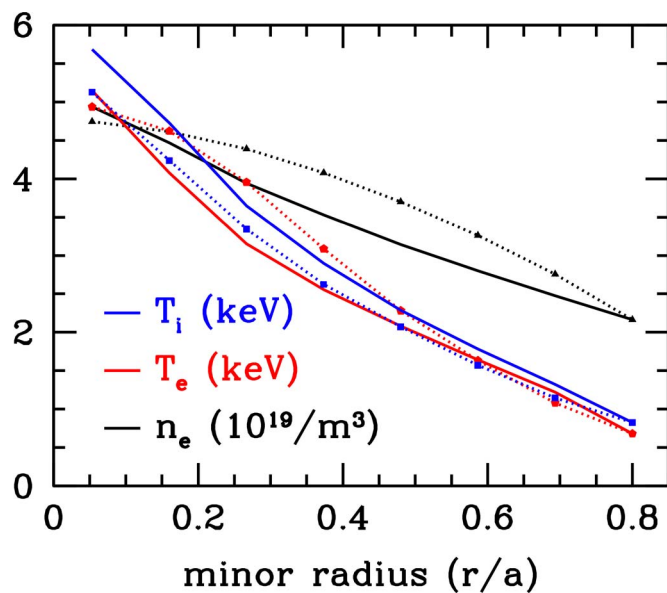
FIG. 2. (Color online) Comparison of steady-state density and temperature profiles constructed from JET shot 19649 by TRANSP (points and dotted lines) with those calculated in TRINITY (solid lines).
