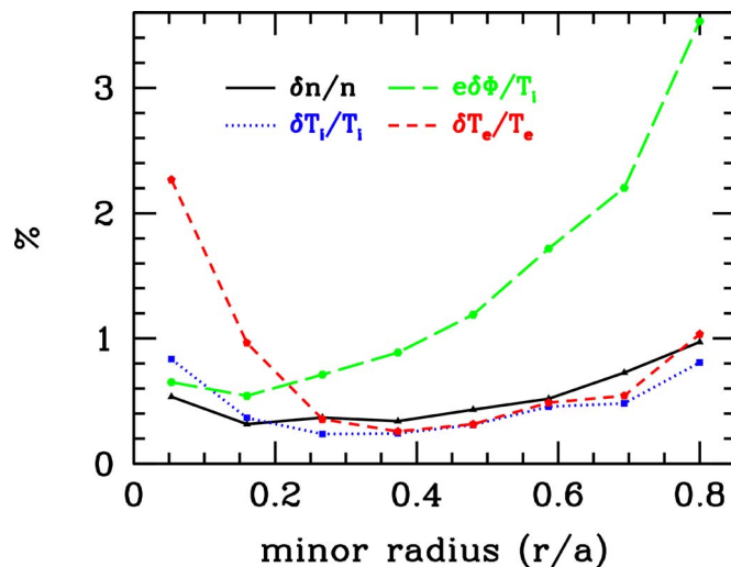
FIG. 5. (Color online) Radial profiles for fluctuations of density, temperature, and electrostatic potential calculated in GS2 for JET shot 19649. These fluctuations are obtained by time averaging the instantaneous fluctuations computed in GS2 over the steady-state period at the end of the TRINITY simulation.
