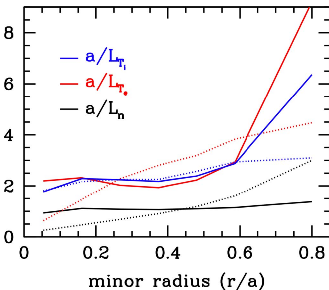
FIG. 3. (Color online) Comparison of experimental (dotted lines) and simulated (solid lines) gradient scale lengths for JET shot 19649.
