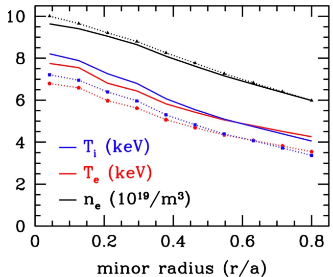
FIG. 9. (Color online) Comparison of steady-state density and temperature profiles for TRINITY simulations of JET shot 42982 with different edge temperatures. The dotted lines with points correspond to a simulation using the edge temperatures reported by the experiment and the solid lines correspond to a simulation with the edge temperatures increased by 20%. We see that the increased edge temperatures lead to an increase in the temperatures near the magnetic axis of about 14%.
