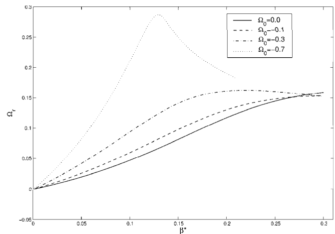
FIG. 8. The normalized real frequency \Omega_r of the RWM as functions of the EPs beta* for various values of \Omega_0 . The wall position is taken as b=1.2 .
