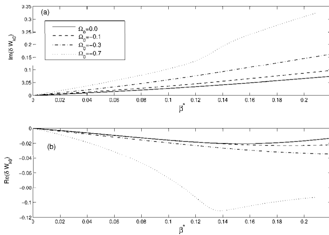
FIG. 7. Imaginary part \text{Im}(\delta W_{K0}) and the real part \text{Re}(\delta W_{K0}) of the perturbed energy of the trapped EPs vs the trapped EPs beta* for the different choices of the plasma rotation frequency \Omega_0 . The wall position is taken as b=1.2 .
