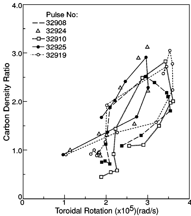
FIG. 7. The hollowness of the carbon profiles against the toroidal rotation in a number of discharges.
