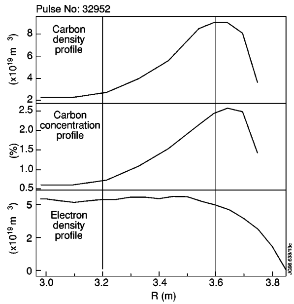
FIG. 5. Hollow carbon density and concentration profiles and the electron density profile in a typical JET H -mode plasma. The two lines indicate the positions R_1 and R_2 , where the ratio of the carbon density and concentration are taken in the analysis.
