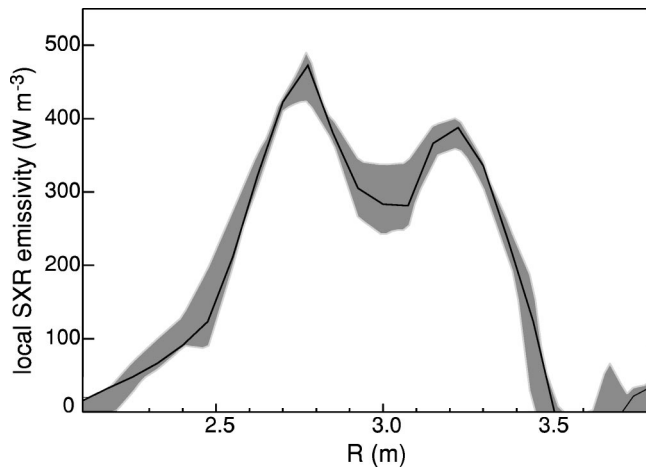
FIG. 10. Soft x-ray emissivity in the middle plane, and the gray area represents the uncertainty from the tomographic reconstruction.
