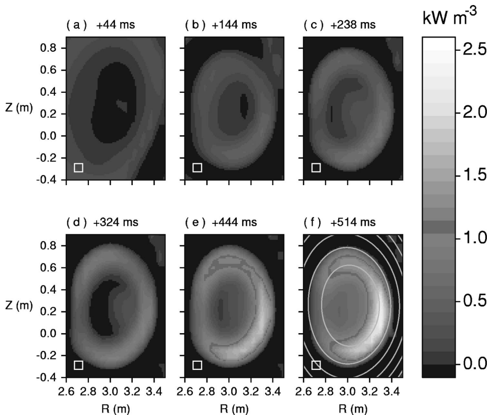
FIG. 2. The background-subtracted emission images from the soft x-ray tomographic reconstruction. The times given are relative to the injection time.
