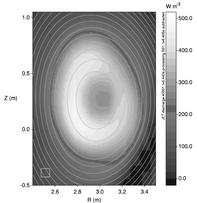
FIG. 9. Tomographic reconstruction (background subtracted) for the nickel injection in the rf heated plasma at 35 ms after the nickel injection.
