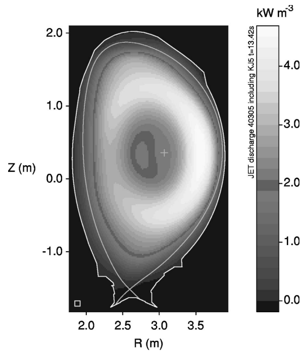
FIG. 8. The poloidally asymmetric emission from mostly light impurities.
