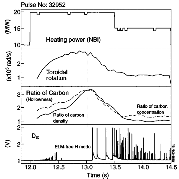
FIG. 6. The time history of the heating, toroidal rotation, and the hollowness of carbon density together with the edge condition of a H -mode plasma.
