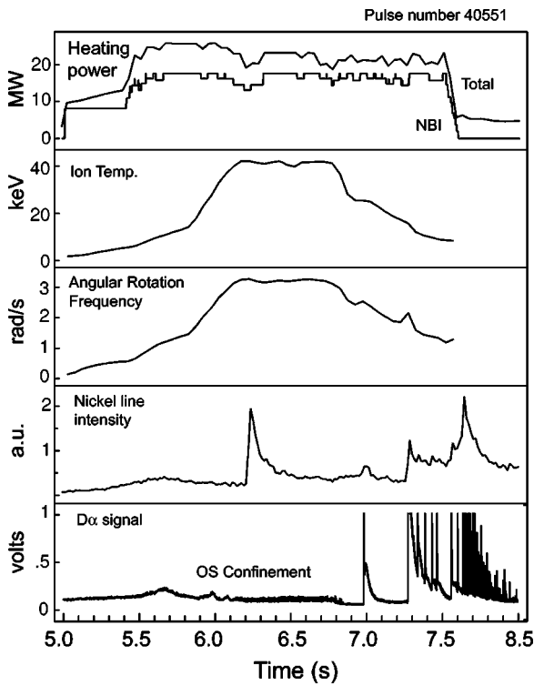
FIG. 1. An overview of an OS discharge. Nickel was injected at 6.206 s.
