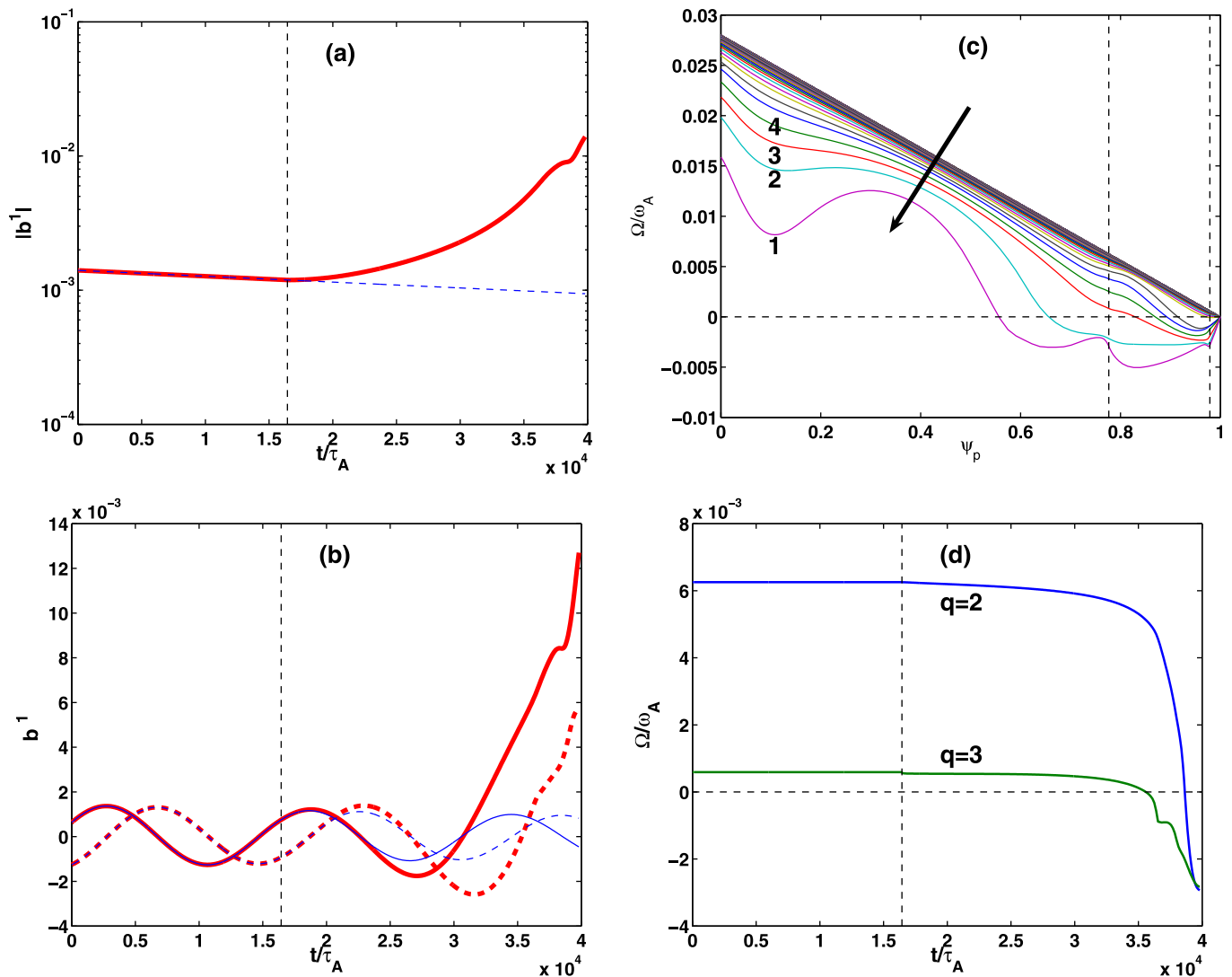
FIG. 13. Evolution of an initially stable RWM: (a) the amplitude of the perturbed radial field b^1 at the q=2 surface, (b) the real and imaginary parts of the perturbed radial field b^1 at the q=2 surface, (c) the radial profile of the plasma rotation frequency, and (d) the plasma rotation frequency at the q=2 and q=3 surfaces. The dashed vertical lines in (a), (b), and (d) indicate the moment of time when the non-linear coupling between the mode and the plasma flow is switched on. The dashed vertical lines in (c) indicate the location of the q=2 and q=3 rational surfaces, respectively. The numbered lines in (c) correspond to time: 1– 3.98 \times 10^4 \tau_A , 2– 3.91 \times 10^4 \tau_A , 3– 3.85 \times 10^4 \tau_A , and 4– 3.79 \times 10^4 \tau_A . The initial mode amplitude, normalized by B_0 , is |b^1|(q=2) = 1.4 \times 10^{-3} . Both the electromagnetic and the NTV torques are included in this simulation.
