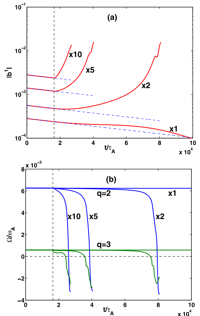
FIG. 16. Time traces of (a) the amplitude of the perturbed radial field b^1 at the q=2 surface, and (b) the plasma rotation frequency at the q=2 and q=3 surfaces, with various choices of the initial mode amplitude. The dashed curves in (a) correspond to the exponential decay of the initially stable linear mode. The dashed vertical lines indicate the moment of time when the non-linear coupling between the mode and the plasma flow is switched on. Both the electromagnetic and the NTV torques are included in the simulations.
