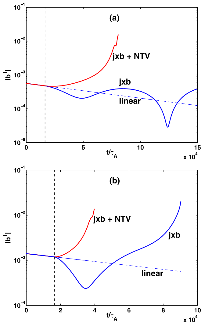
FIG. 15. Time traces of the amplitude of the perturbed radial field b^1 at the q=2 surface, with and without inclusion of the NTV torque in the simulations for an initially stable RWM, with the initial mode amplitude at (a) |b^1|(q=2) = 5.6 \times 10^{-4} and (b) |b^1|(q=2) = 1.4 \times 10^{-3} . The dashed curves correspond to the exponential decay of the initially stable linear mode. The dashed vertical lines indicate the moment of time when the non-linear coupling between the mode and the plasma flow is switched on.
