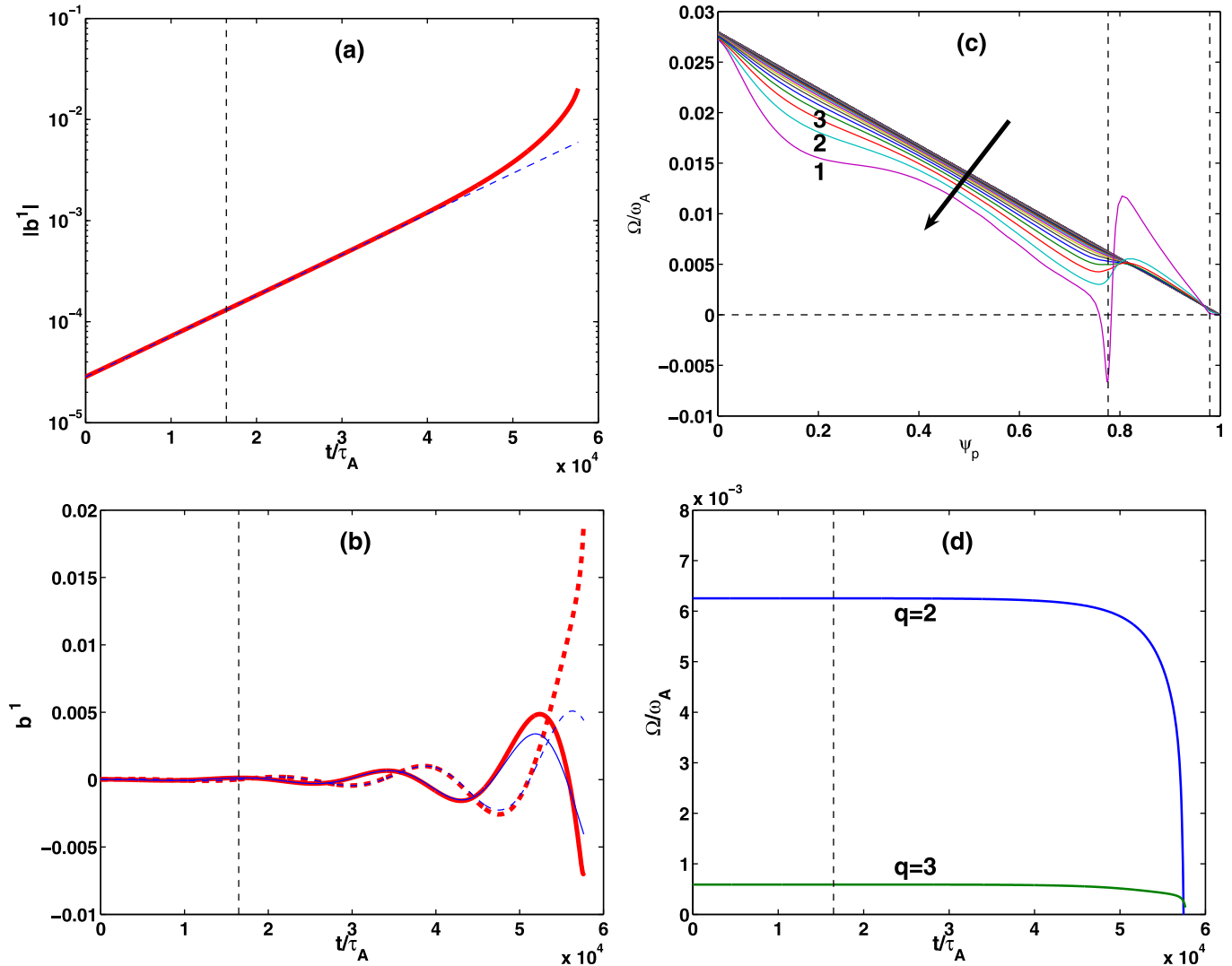
FIG. 7. Evolution of an initially unstable RWM: (a) the amplitude of the perturbed radial field b^1 at the q=2 surface, (b) the real and imaginary parts of the perturbed radial field b^1 at the q=2 surface, (c) the radial profile of the plasma rotation frequency, and (d) the plasma rotation frequency at the q=2 and q=3 surfaces. The dashed vertical lines in (a), (b), and (d) indicate the moment of time when the non-linear coupling between the mode and the plasma flow is switched on. The dashed vertical lines in (c) indicate the location of the q=2 and q=3 rational surfaces, respectively. The numbered lines in (c) correspond to time: 1– 5.77 \times 10^4 \tau_A , 2– 5.67 \times 10^4 \tau_A , and 3– 5.58 \times 10^4 \tau_A . Only the electromagnetic is included in this simulation.
