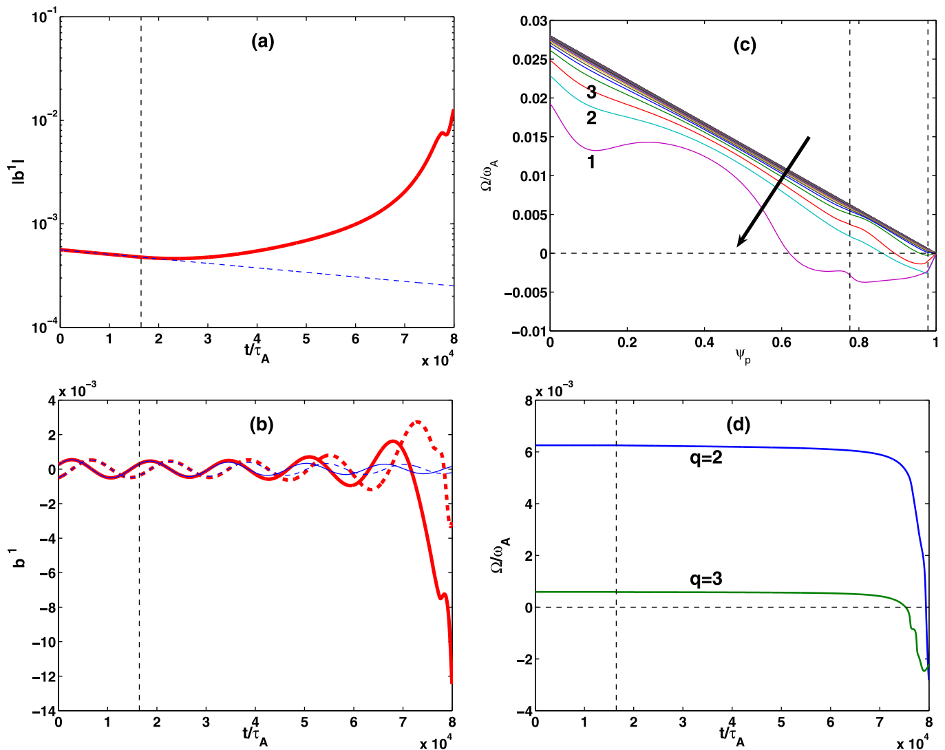
FIG. 10. Evolution of an initially stable RWM: (a) the amplitude of the perturbed radial field b^1 at the q=2 surface, (b) the real and imaginary parts of the perturbed radial field b^1 at the q=2 surface, (c) the radial profile of the plasma rotation frequency, and (d) the plasma rotation frequency at the q=2 and q=3 surfaces. The dashed vertical lines in (a), (b), and (d) indicate the moment of time when the non-linear coupling between the mode and the plasma flow is switched on. The dashed vertical lines in (c) indicate the location of the q=2 and q=3 rational surfaces, respectively. The numbered lines in (c) correspond to time: 1– 8.00 \times 10^4 \tau_A , 2– 7.86 \times 10^4 \tau_A , and 3– 7.73 \times 10^4 \tau_A . The initial mode amplitude, normalized by B_0 , is |b^1|(q=2) = 5.6 \times 10^{-4} . Both the electromagnetic and the NTV torques are included in this simulation.
