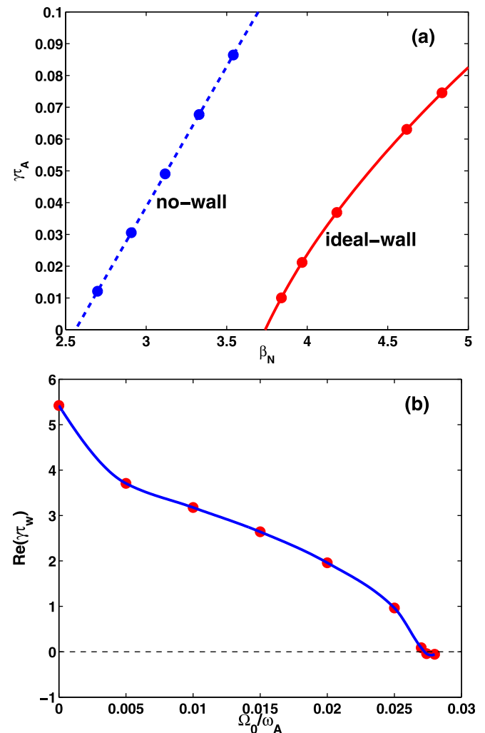
FIG. 3. Linear stability of (a) the ideal external, pressure-driven kink mode and (b) the resistive wall mode in the presence of the plasma flow.
