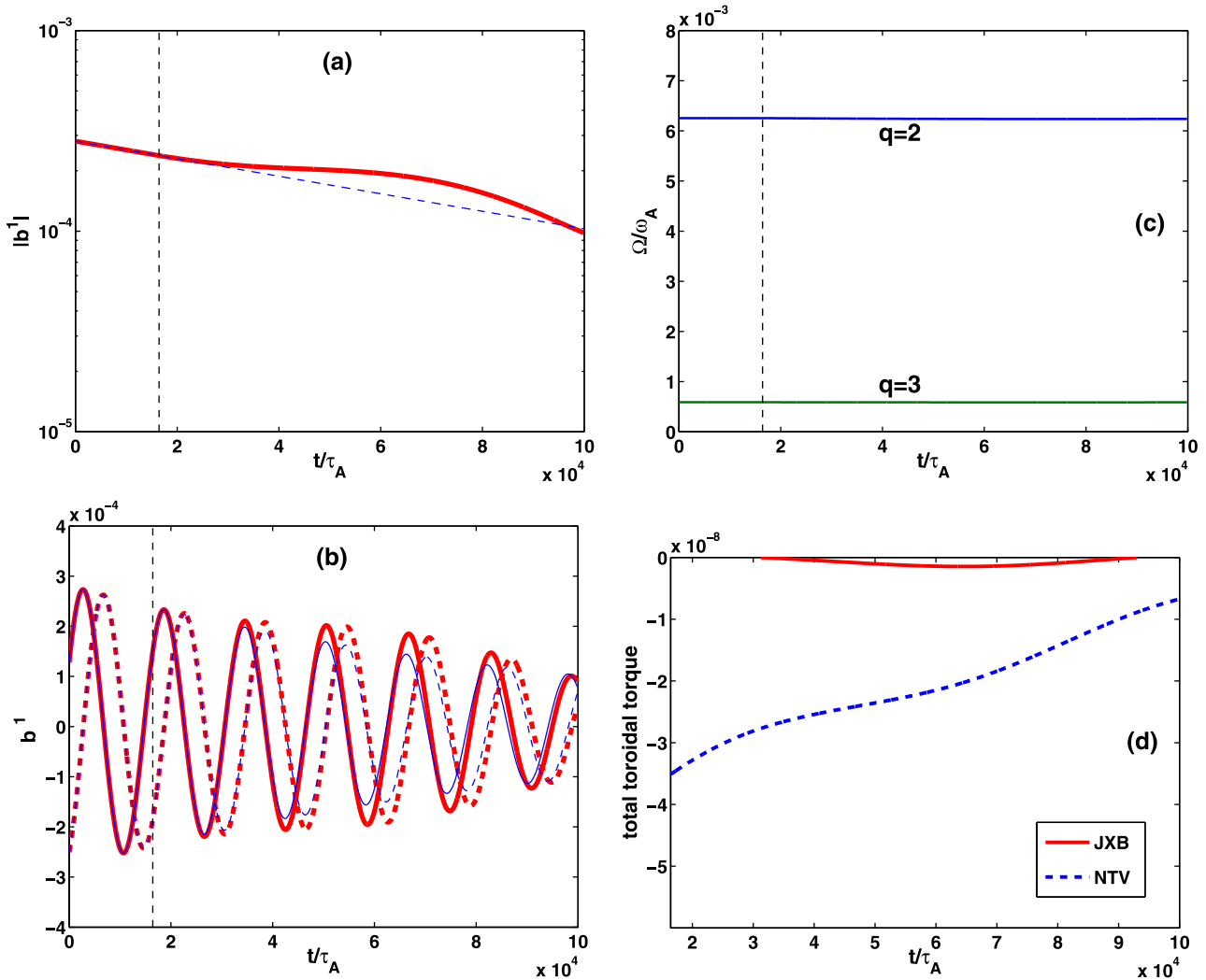
FIG. 9. Evolution of an initially stable RWM: (a) the amplitude of the perturbed radial field b^1 at the q=2 surface, (b) the real and imaginary parts of the perturbed radial field b^1 at the q=2 surface, (c) the plasma rotation frequency at the q=2 and q=3 surfaces, and (d) the net toroidal electromagnetic and NTV torques acting on the plasma. The dashed vertical lines in (a), (b), and (c) indicate the moment of time when the non-linear coupling between the mode and the plasma flow is switched on. The initial mode amplitude, normalized by B_0 , is |b^1|(q=2) = 2.8 \times 10^{-4} .
