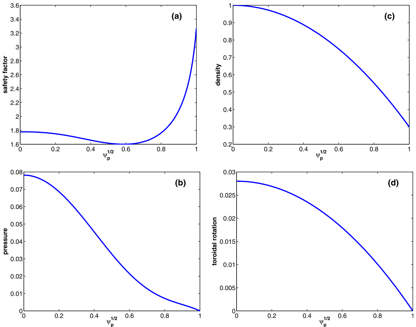
FIG. 2. Radial profiles of the equilibrium quantities for (a) the safety factor q , (b) the plasma pressure normalized by B_0^2/\mu_0 , (c) the plasma density normalized to unity at the magnetic axis, and (d) the toroidal rotation frequency of the plasma, normalized by the on-axis Alfvén frequency.
