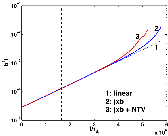
FIG. 8. Time traces of the amplitude of the perturbed radial field b^1 at the q=2 surface, with and without inclusion of the NTV torque in the simulation. The dashed curve corresponds to the exponential growth of the initially unstable linear mode. The dashed vertical line indicates the moment of time when the non-linear coupling between the mode and the plasma flow is switched on.
