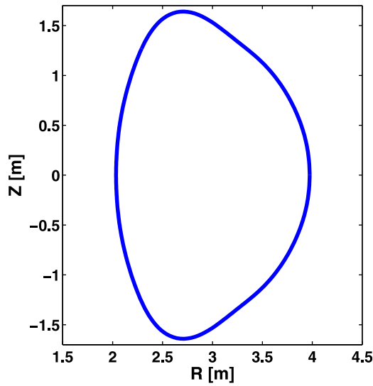
FIG. 1. The plasma boundary shape of the toroidal equilibrium.
