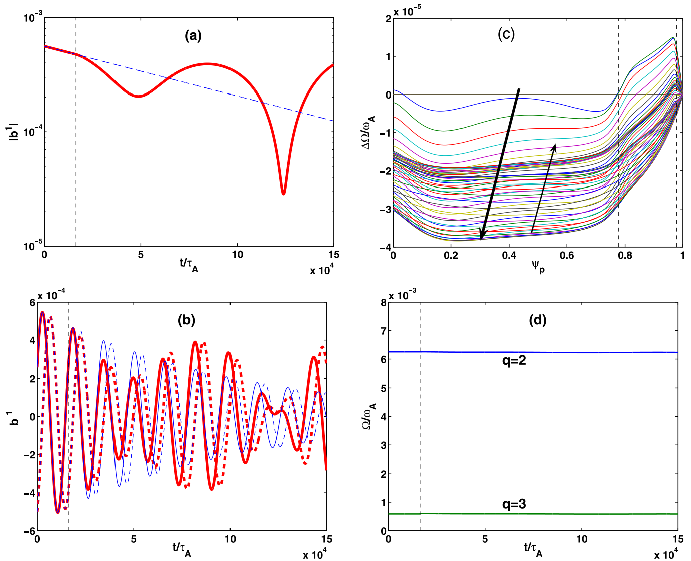
FIG. 11. Evolution of an initially stable RWM: (a) the amplitude of the perturbed radial field b^1 at the q=2 surface, (b) the real and imaginary parts of the perturbed radial field b^1 at the q=2 surface, (c) the radial profile of the change of the plasma rotation frequency, and (d) the plasma rotation frequency at the q=2 and q=3 surfaces. The dashed vertical lines in (a), (b), and (d) indicate the moment of time when the non-linear coupling between the mode and the plasma flow is switched on. The dashed vertical lines in (c) indicate the location of the q=2 and 3 rational surfaces, respectively. The initial mode amplitude, normalized by B_0 , is |b^1|(q=2) = 5.6 \times 10^{-4} . Only the electromagnetic torque is included in this simulation.
