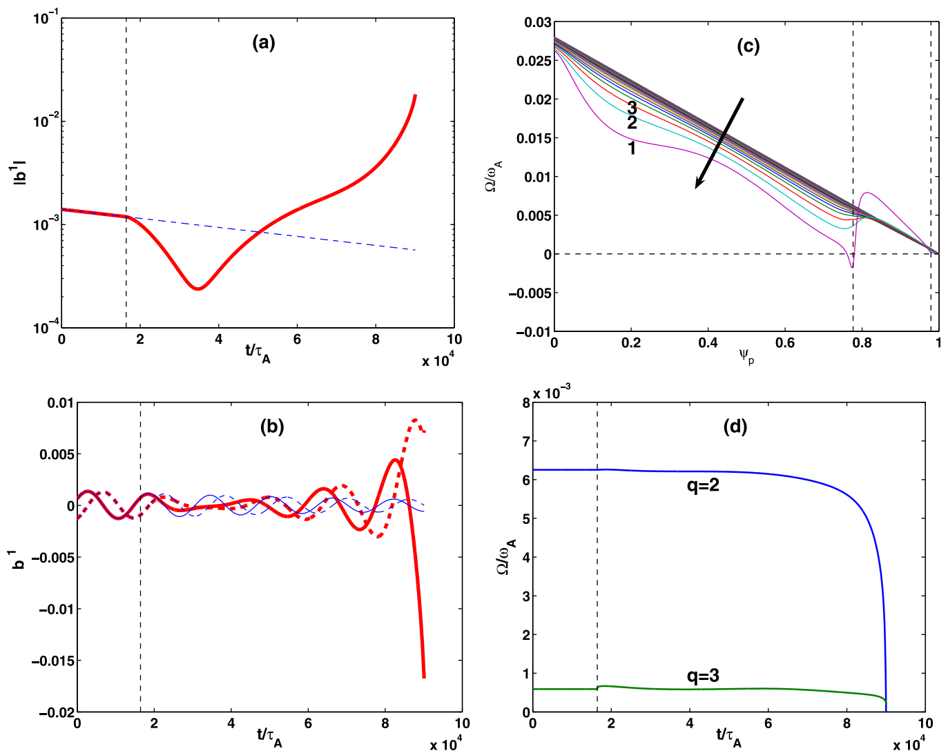
FIG. 14. Evolution of an initially stable RWM: (a) the amplitude of the perturbed radial field b^1 at the q=2 surface, (b) the real and imaginary parts of the perturbed radial field b^1 at the q=2 surface, (c) the radial profile of the plasma rotation frequency, and (d) the plasma rotation frequency at the q=2 and q=3 surfaces. The dashed vertical lines in (a), (b), and (d) indicate the moment of time when the non-linear coupling between the mode and the plasma flow is switched on. The dashed vertical lines in (c) indicate the location of the q=2 and q=3 rational surfaces, respectively. The numbered lines in (c) correspond to time: 1– 9.00 \times 10^4 \tau_A , 2– 8.85 \times 10^4 \tau_A , and 3– 8.70 \times 10^4 \tau_A . The initial mode amplitude, normalized by B_0 , is |b^1|(q=2) = 1.4 \times 10^{-3} . Only, the electromagnetic torque is included in this simulation.
