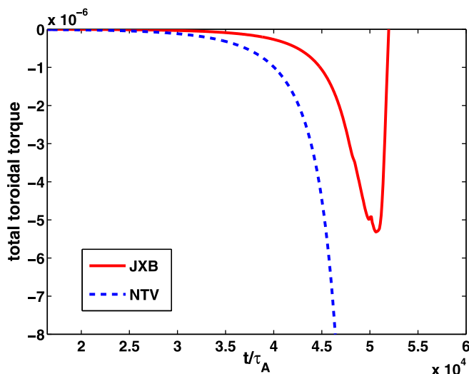
FIG. 5. Time trace of the net toroidal electromagnetic (solid line) and NTV (dashed line) torques acting on the plasma during the non-linear evolution of an initially unstable RWM as described in Fig. 4.
