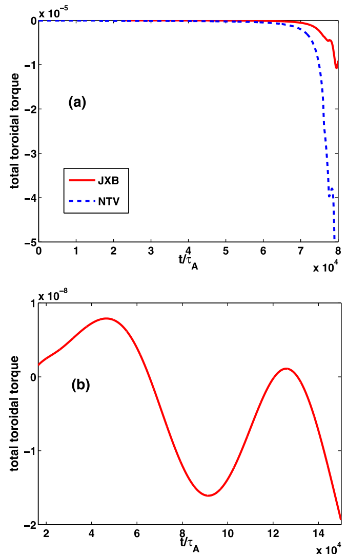
FIG. 12. Time traces of the net toroidal electromagnetic (solid line) and NTV (dashed line) torques acting on the plasma, during the non-linear evolution of an initially stable RWM, with the initial mode amplitude |b^1|(q=2) = 5.6 \times 10^{-4} : (a) both electromagnetic and NTV torques are included in the toroidal torque balance and (b) only the electromagnetic torque is included.
