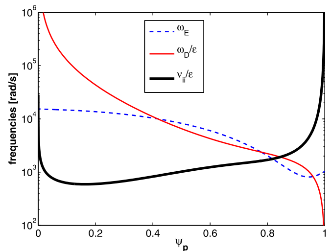
FIG. 6. Radial profiles of the initial (i.e., before closing the non-linear coupling loop) \mathbf{E} \times \mathbf{B} rotation frequency \omega_E , the precessional drift frequency \omega_D of deeply trapped thermal ions at thermal velocity, and the ion-ion collision frequency \nu_{ii} . \epsilon is approximately the inverse aspect ratio.
