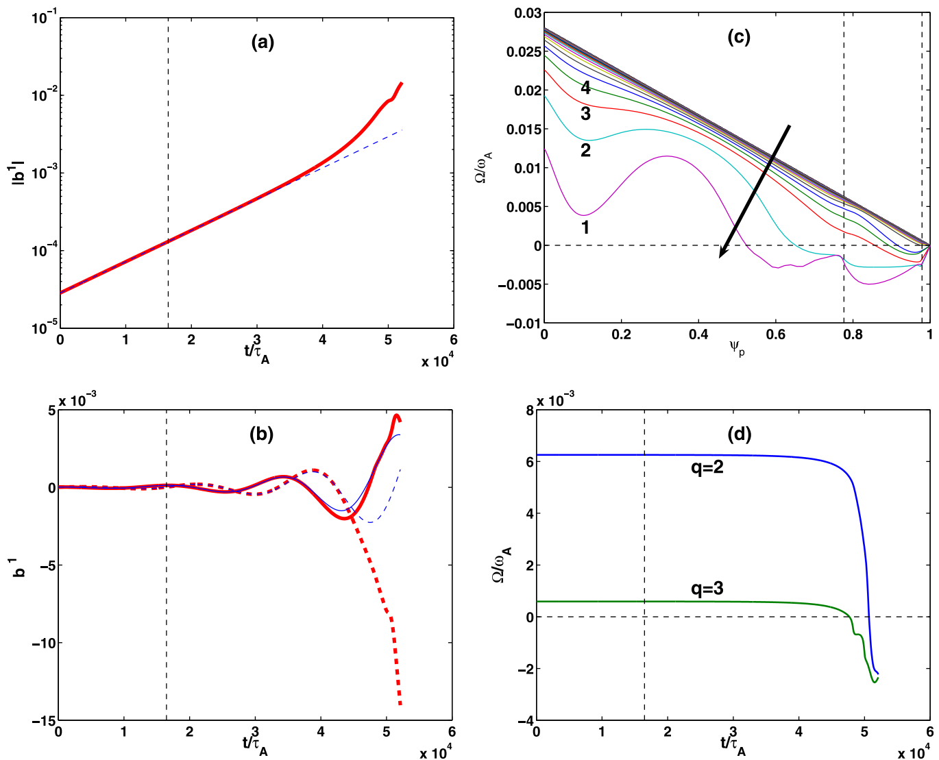
FIG. 4. Evolution of an initially unstable RWM: (a) the amplitude of the perturbed radial field b^1 at the q=2 surface, (b) the real and imaginary parts of the perturbed radial field b^1 at the q=2 surface, (c) the radial profile of the plasma rotation frequency, and (d) the plasma rotation frequency at the q=2 and q=3 surfaces. The dashed vertical lines in (a), (b), and (d) indicate the moment of time when the non-linear coupling between the mode and the plasma flow is switched on. The dashed vertical lines in (c) indicate the location of the q=2 and 3 rational surfaces, respectively. The numbered lines in (c) correspond to time: 1– 5.21 \times 10^4 \tau_A , 2– 5.13 \times 10^4 \tau_A , 3– 5.03 \times 10^4 \tau_A , and 4– 4.95 \times 10^4 \tau_A . Both the electromagnetic and the NTV torques are included in this simulation.
