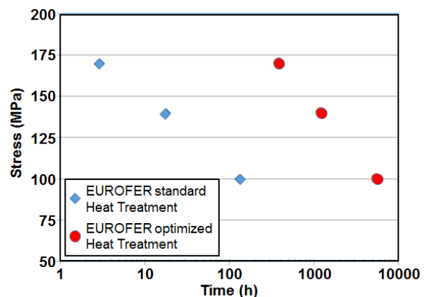
Fig 3: Creep lifetime (time to rupture) for EUROFER in the standard metallurgical condition and after non-standard, optimized heat treatments
