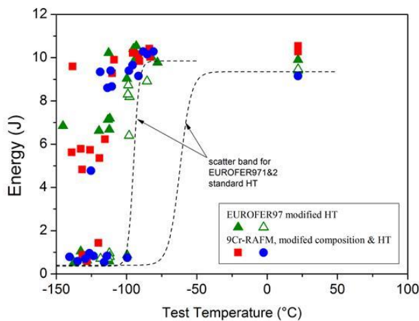
Fig 2: Charpy impact test data (KLST) for optimized RAFM steels in comparison to EUROFER97 1&2 (standard heat treatment)
