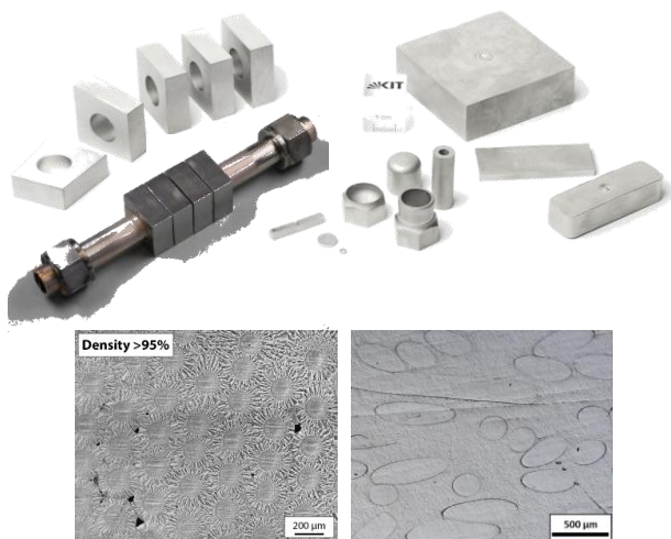
Fig 4: Various tungsten pieces produced via PIM and the produced mock-up after exposure to 20\text{ MW/m}^2 (top); microstructure of long and short fiber reinforced tungsten (bottom)
