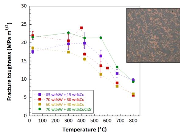
Fig 5: Fracture toughness of W-particle reinforced Cu and CuCrZr; microstructure of one of three industrially produced batches of W_p\text{-CuCrZr}
