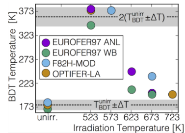
Fig 1: Temperatures of brittle to ductile transitions (BDT) in several fusion steels. A model [12] based on the analysis of screw dislocation mobility suggests that the BDT temperature doubles if irradiation is performed at relatively low temperature.
