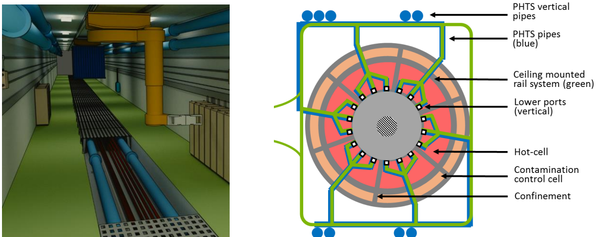
FIG. 5. Maintenance corridor with manipulator and pipe ducts (left) and plan view of the lower port level maintenance corridors combined with the heat transfer system pipes (right).
