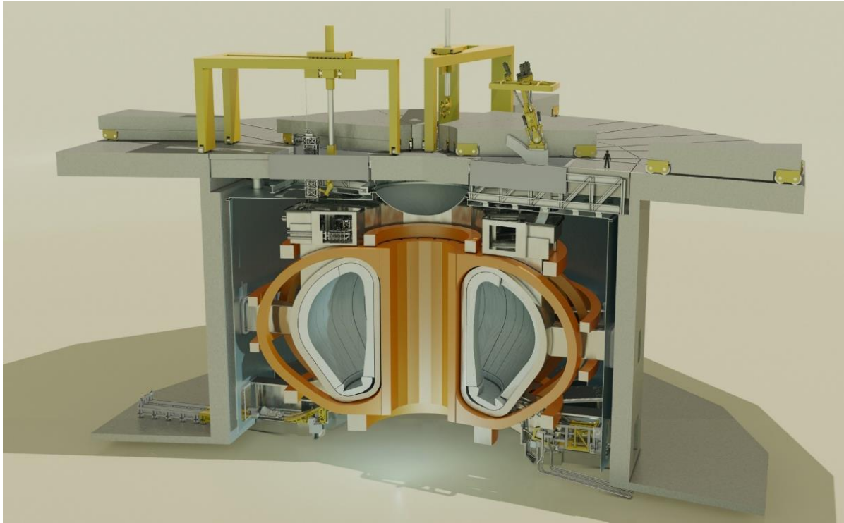
FIG. 3. Four maintenance systems working in parallel through upper ports
