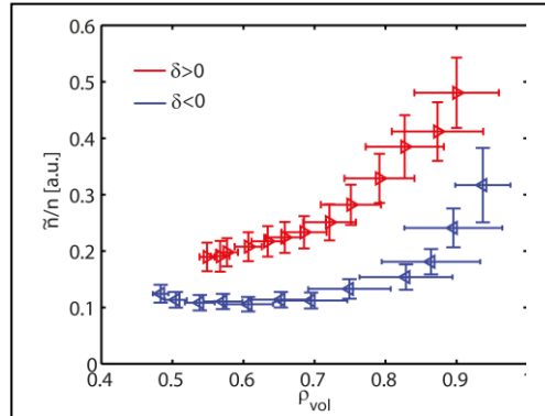
FIG. 6. Density fluctuation amplitude profile measured by tPCI in two plasmas with edge triangularity +0.5 and -0.3, respectively, with 0.45 MW central ECH. (Reproduced from [52].)
