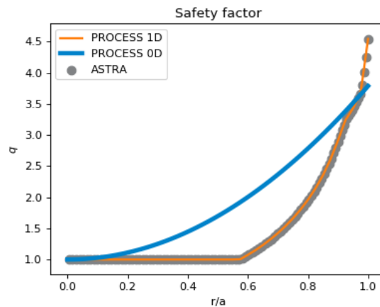
Figure 2: Safety factor, or q profile output from PROCESS 0D and 1D, and ASTRA
