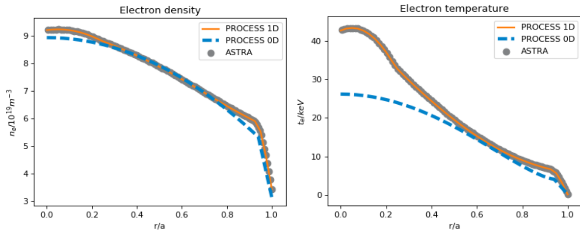
Figure 1: Electron density and temperature radial profiles output from PROCESS 0D and 1D, and ASTRA. PROCESS 0D uses a simple parametrisation from core to pedestal for the electron density and temperature radial profiles. Figure 1 shows that in this case, the electron density profile is a good approximation for the more complex model, but electron temperature is significantly underestimated in the core. For simplicity, PROCESS optimises only one parameter per profile, i.e. the density and temperature at the ‘core’ and therefore does not output physically consistent profiles. Hence the argument for a 1D model.
