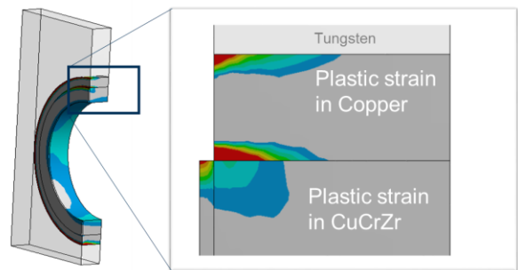
Fig. 5. calculated plastic strain regions in copper and CuCrZr (at 20MW/m 2 heat load)
