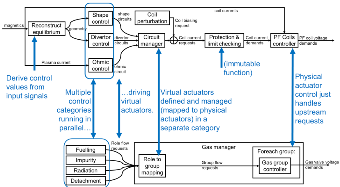
Figure 4 functional flow diagrams for PCS categories involved in (upper) PF coil control and (lower) gas control
