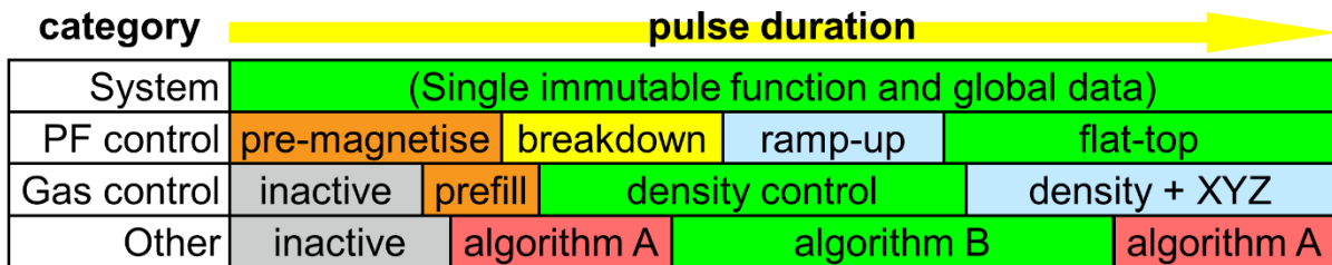
Figure 3 Representative category execution timing diagram for a fictitious example PCS installation
