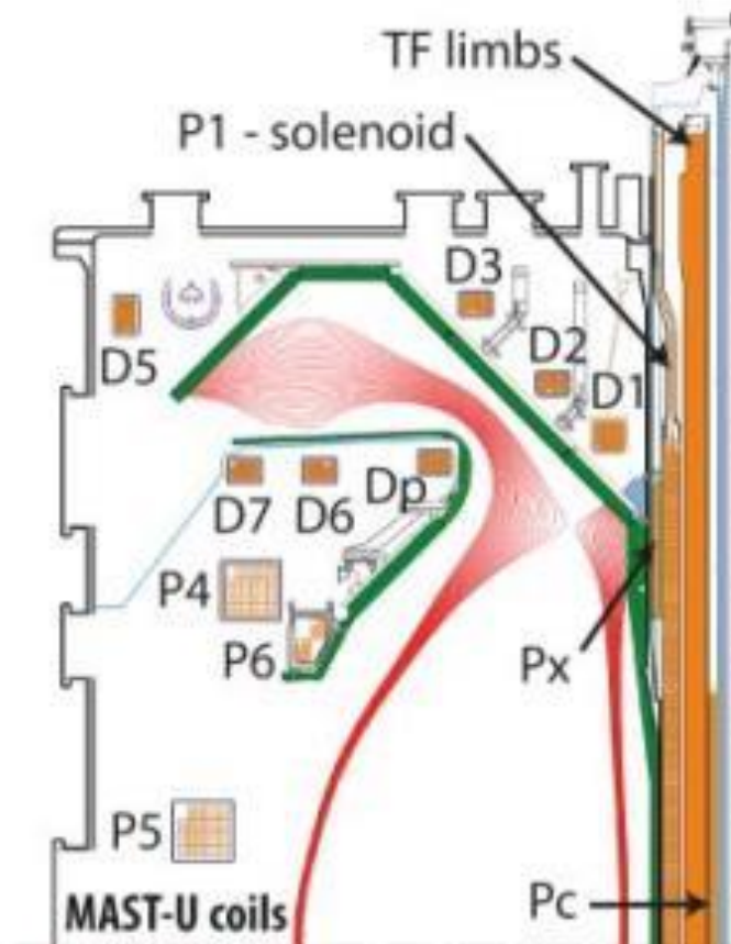
Figure 1: MAST-U upper left vessel cross-section showing PF coil locations)
