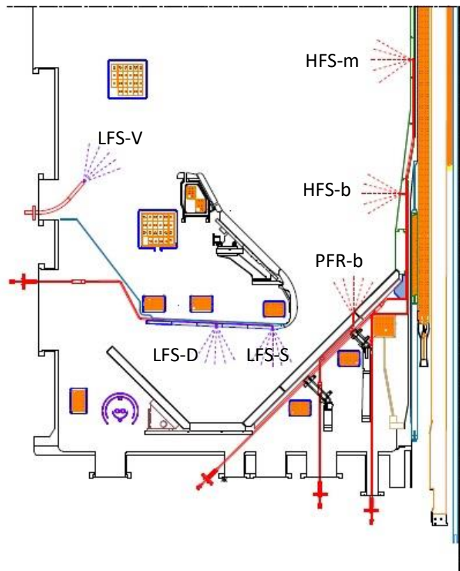
Figure 2 MAST-U lower left vessel cross-section showing gas injection locations
