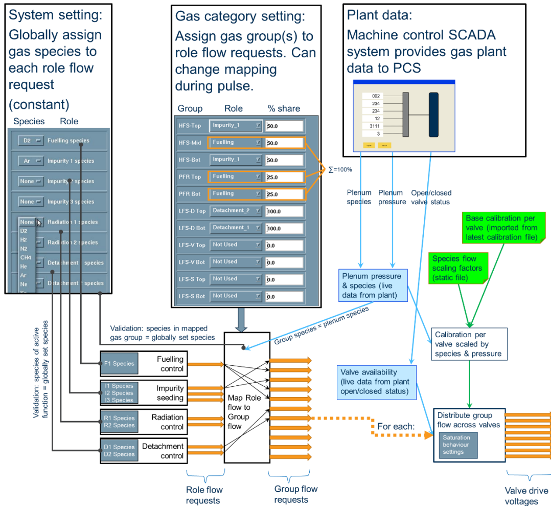
Figure 5 Diagram showing the detailed information flow in the gas control functional chain.
