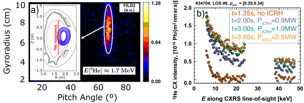
Figure 11. 3 ion H- 3 He-D heating: a) energy and pitch angle resolved fast-ion loss measured with FILD during on-axis heating, b) energy spectrum of He ions from CXRS during off-axis heating at different ICRF powers.
