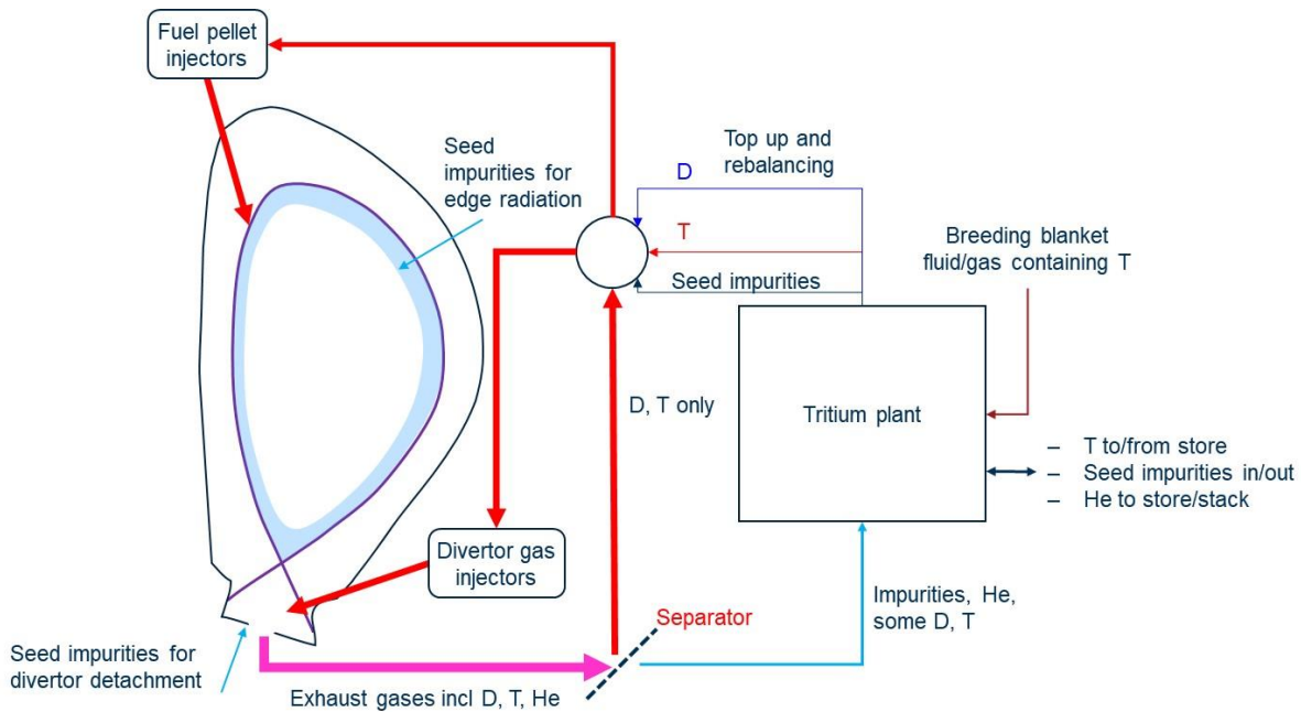
Figure 6: Schematic of gas and fuel injection and pumping/purification cycle (after [69]). Presently the separators are proposed to be in the divertor ports, before two sets of pumps (for the permeate and retentate).
