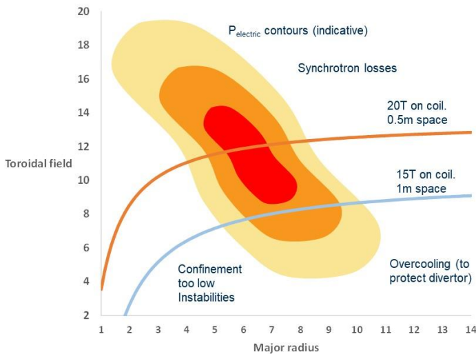
Figure 3: Indicative (not calculated) net electrical power in B , R space, based on ITER-like confinement scaling (using general features from [26] but allowing for some improved performance with higher elongation, for example). The curves are simple estimates for the field at the geometric axis for a given maximum field at the outer edge of the inboard leg of the toroidal field coil and allowing a gap for a shield and blanket, for an A=3.1 plasma.
