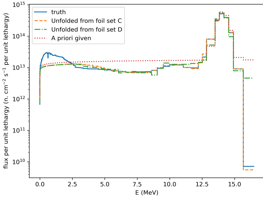
Fig. 2 An ITER-DT spectrum unfolded with MAXED using foil set C (Table 3) and set D (Table 4), with target \chi^2 = 0.01 .
