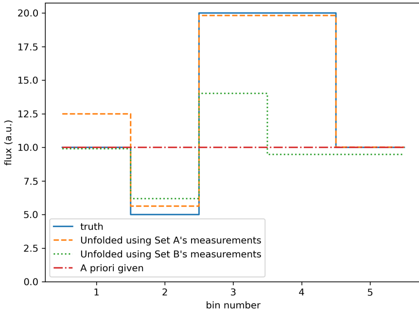
Fig. 1 The toy model spectrum unfolded with MAXED using a target \chi^2 = 0.01 .
