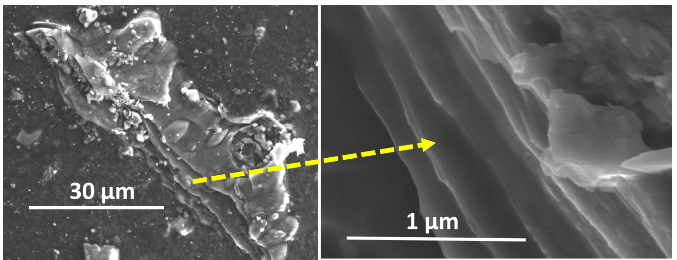
Figure 17. A flake of a stratified co-deposit containing mainly Be and C found on the Mascot wrist. Reproduced from [PWI-29].
