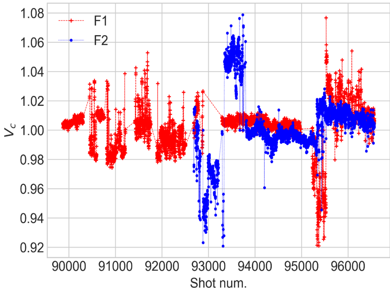
Figure 23. The normalised Verdet constant for FOCS 1 (F1, red) and FOCS 2 (F2, blue) systems during JET operation for shots from 89870 to 96563. The estimated values are 0.696 \pm 0.010 and 0.672 \pm 0.013 rad/MA, respectively ([from [ref]).
