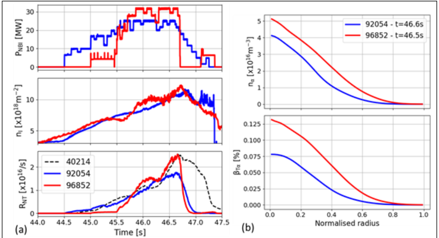
Figure 4 - Comparison of JET pulses 92054, 96852. (a) Time traces: NBI power, core line-integrated density (interferometry), DD neutron rate; Also shown is the neutron rate for reference JET carbon wall pulse 40214, shifted by -0.31s. (b) TRANSP extrapolation to DT of pulses 92054 and 96852: (top) alpha density; (bottom) normalised alpha beta. Figure is from [ref, permission to be requested]
