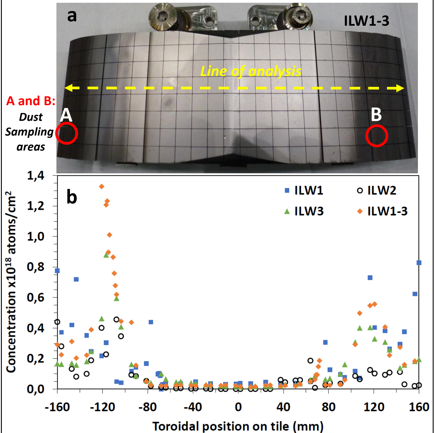
Figure 11. (a) Castellated beryllium mid-plane IWGL tile after exposure during all three ILW campaigns, areas of the co-deposit and dust sampling are marked; (b) Deuterium areal concentrations at mid-plane measured after consecutive campaigns and after all three campaigns ILW1-3; data for ILW-1 and ILW2, reproduced with permission of copyright holder UKAEA and author [PWI-1, PWI-2].
