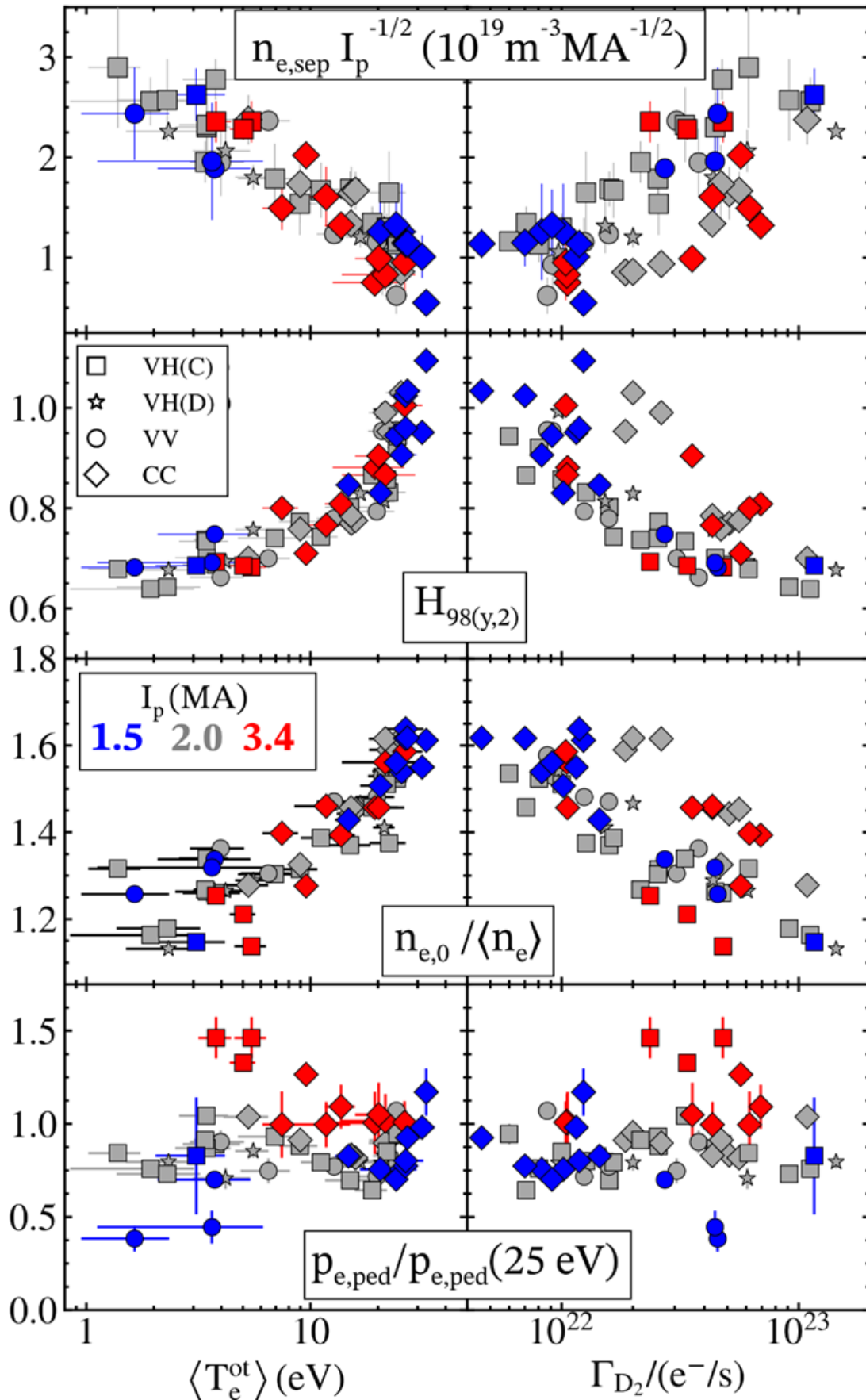
Figure 7 - Dataset of unseeded discharges showing the range of variation in the D2 fueling rate \Gamma_{D2} and the averaged outer target electron temperature \langle T_{e,ot} \rangle and correlations with n_{e,sep} I_p^{-0.5} , H_{98(y,2)} , density peaking factor n_{e,0} / \langle n_e \rangle and p_{e,ped} normalized by p_{e,ped} at \langle T_{e,ot} \rangle = 25 eV. Marker colour denotes I_p with 1.5 MA (blue), 2.0 MA (grey) and 3.4 MA (red). The database includes divertor configurations with the strike point locations on the inner-vertical, outer-horizontal targets, VH(C) and VH(D) with C and D denoting the position of the outer strike point on stack C and D of tile 5; inner and outer vertical (VV) and inner and outer corner (CC). Figure is from [ref] permission to be requested
