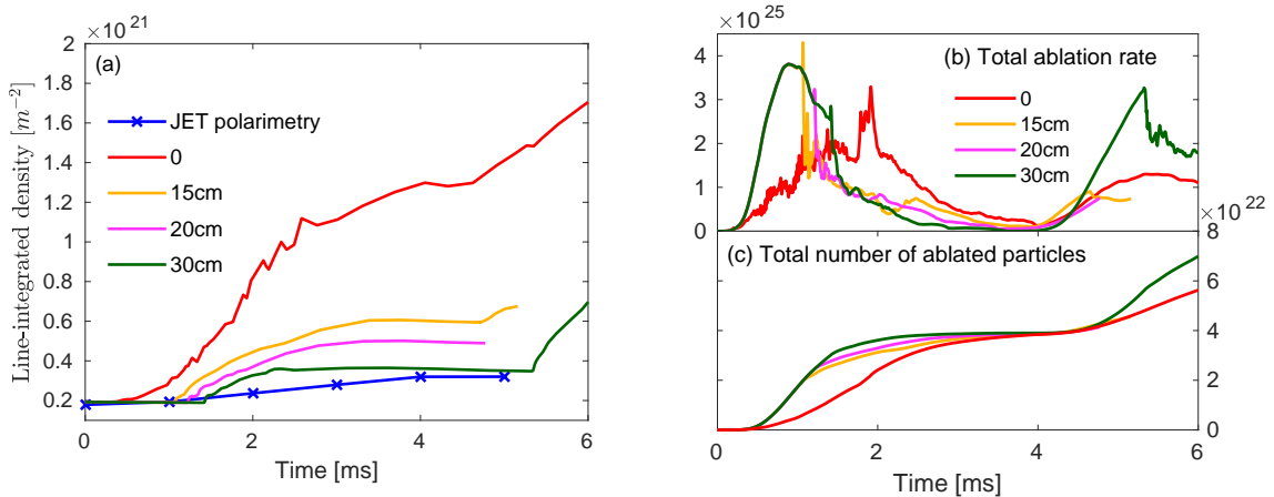
Figure 1: Scan of drift distance with 1 \times 10^{17} m^{-3} background neon and 4.5 \times 10^{15} m^{-3} tungsten.
