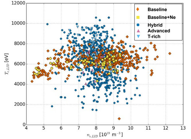
Figure 3: Electron density ( n_e ), and temperature ( T_e ) of database points corresponding to flat-top phases for each pulse.
