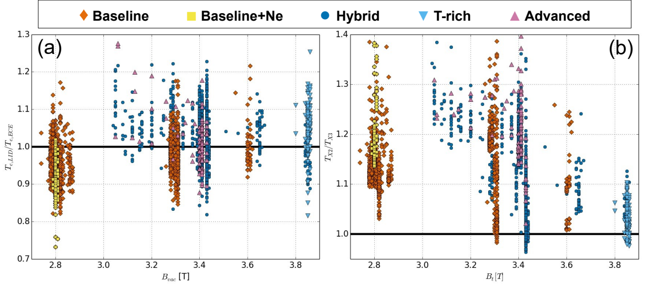
Figure 8: Ratio of ECE and LIDAR measurements (a) and ratio between the peaks of X2 and X3 emission (b) as a function of the vacuum magnetic field B_{vac} .
