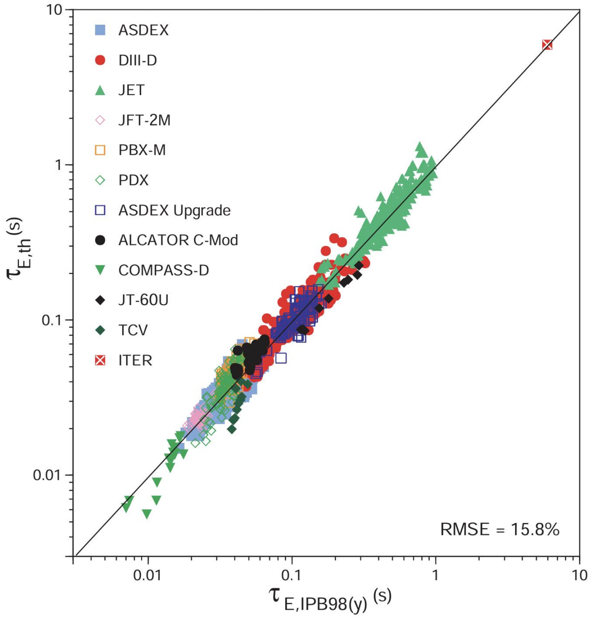
Figure 3 : Comparison of H-mode thermal energy confinement time with the scaling expression in Eq. (18) of reference [13] for ELM data in the ITER H-mode database version DB3. Reproduced with permission from [13].
