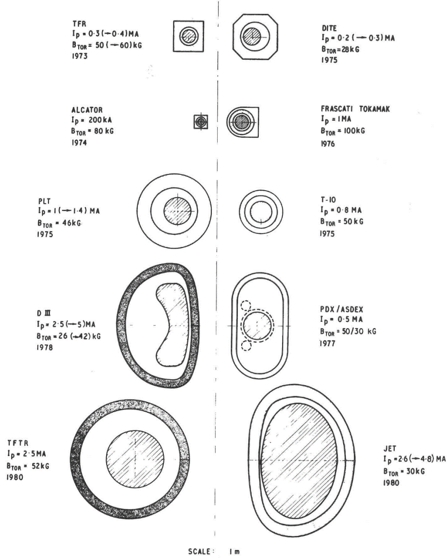
Figure 1 : Size and magnetic fields of the JET tokamak compared with the devices operating at the time of JET Design. Reproduced from [1].
