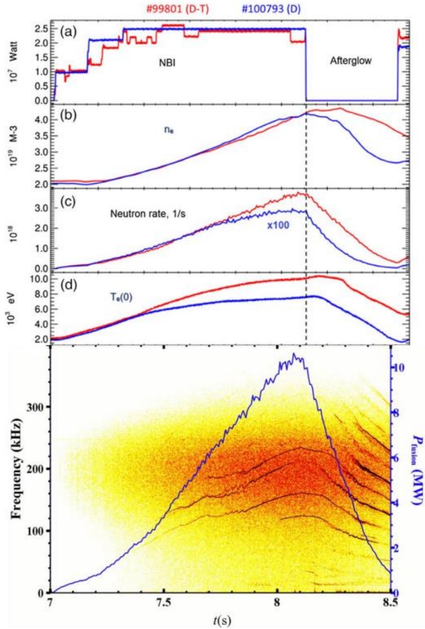
Figure 14 : Time evolution of the main parameters of the afterglow scenario in D-T, #99801 in red, compared with its reference in deuterium, #100793 in blue, together with the fusion power trace and Fourier spectrogram of magnetics measurements of TAE activity for the D-T pulse. Adapted from [69]
