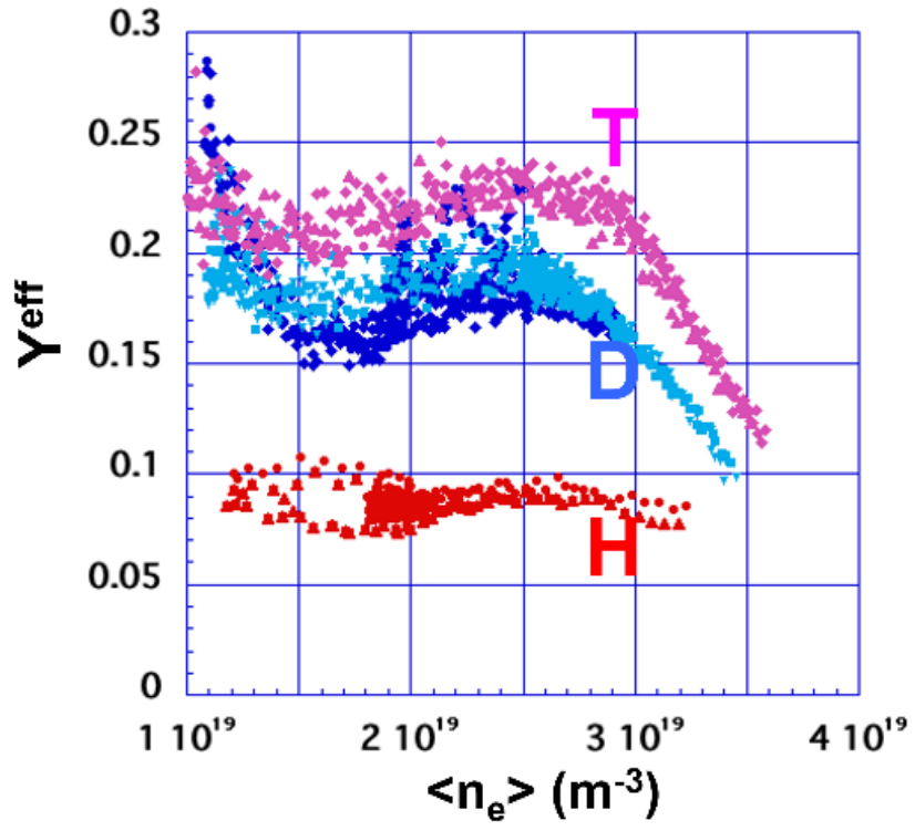
Figure 7 : Effective Be sputtering yields measured at JET's inner Be limiters by visible spectroscopy. Reproduced with permission from [34].
