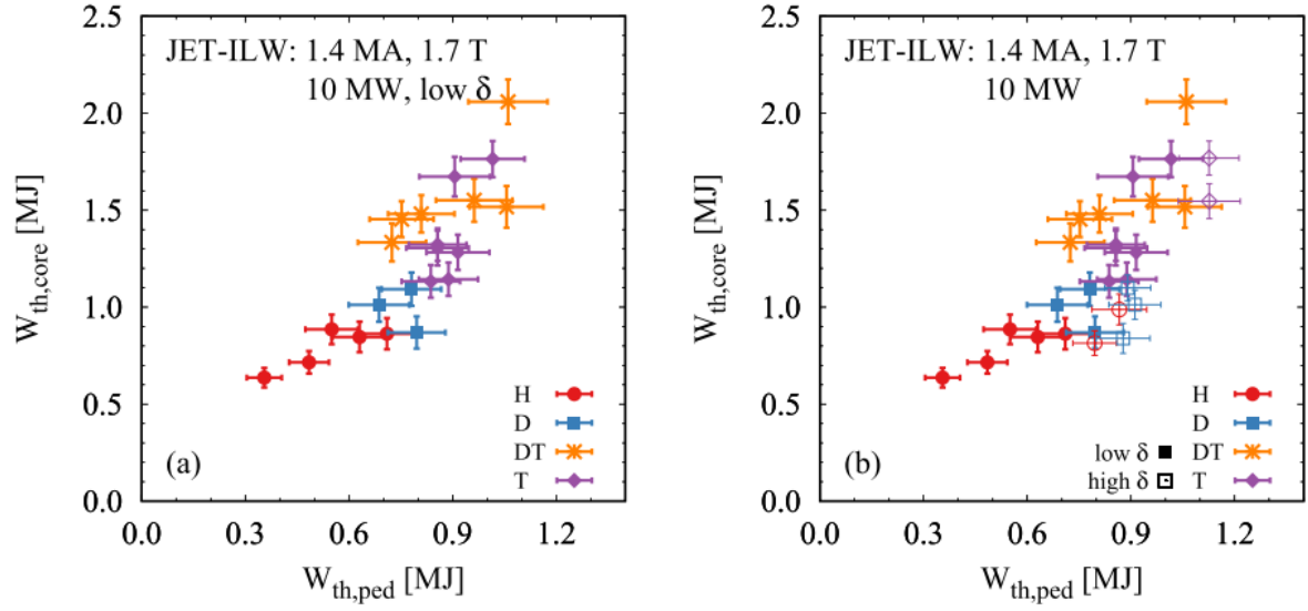
Figure 5 : Core thermal stored energy as a function of the pedestal thermal stored energy for 10 MW plasmas of a gas puffing scan for different isotopes with low \delta only in (a) and also high \delta plasmas in (b). Reproduced with permission from [21].
