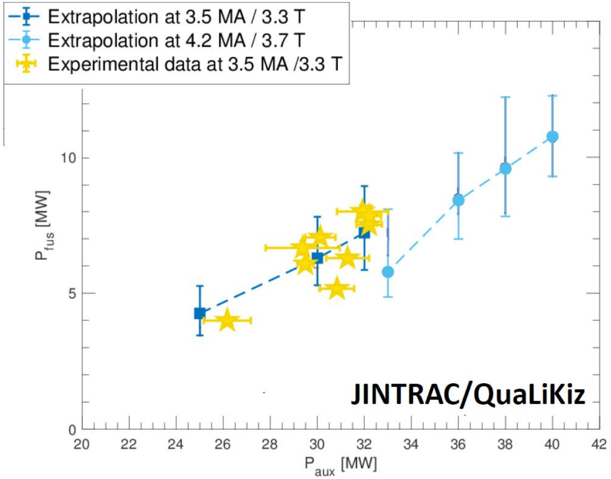
Figure 15 : Comparison of D-T fusion power achieved in DTE2 in the baseline scenario at 3.5 MA (gold stars) with predictive modelling based on extrapolations from D plasmas at \beta_N \sim 1.8 (blue squares) using JETTO-Qualikiz within the JINTRAC workflow. Figure adapted from [80].
