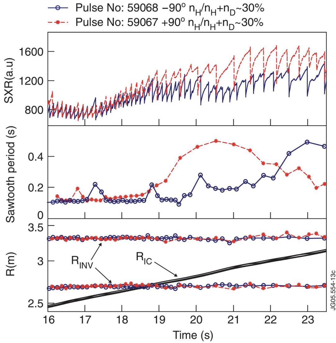
Figure 11 : Soft x-ray signals, showing the core sawtooth activity, for two discharges with n_H/(n_H + n_D) \approx 30\% and positions of the inversion radius ( R_{inv} ) and ion cyclotron resonance ( R_{IC} ). Solid line and rings, #59068 with -90^\circ ICCD; dashed lines and stars #59067 with +90^\circ ICCD. Reproduced with permission from [55].
