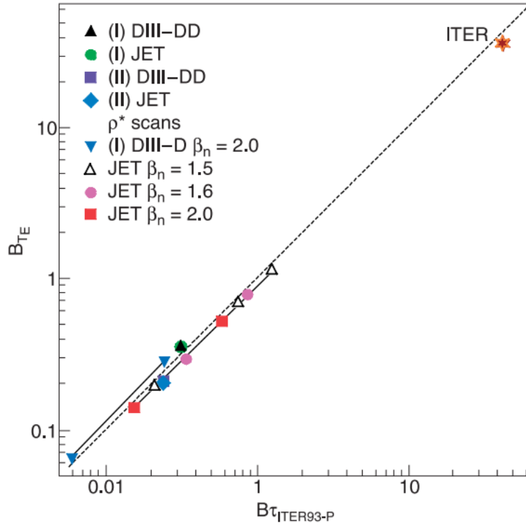
Figure 4 : Comparison of B\tau_E measured in \rho^* scans on JET and DIII-D with the ITER93H-P scaling relation. Reproduced with permission from [13].
