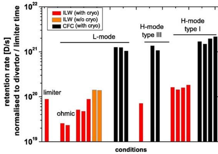
Figure 6 : Long-term fuel retention rates in the JET-ILW, measured by global gas balance, and compared with equivalent conditions in Carbon wall. Reproduced with permission from [31].
