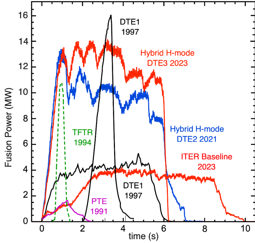
Figure 13 : D-T fusion energy records obtained in TFTR and in JET, PTE, DTE1, DTE2 and DTE3, in different transient and steady H-mode scenarios. With “ITER Baseline” it’s designed the seeded H-mode scenario at high current and high triangularity.
