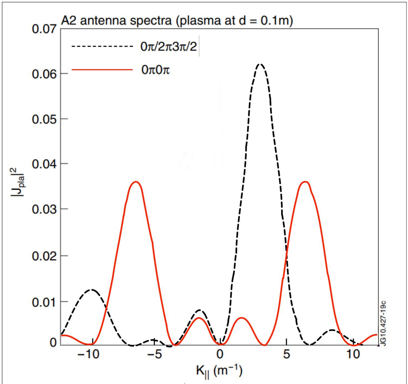
Figure 10 : normalized power spectra for representative heating and current drive for the JET A2 ICRF antenna system. Adapted from figure 5 of reference [79]
