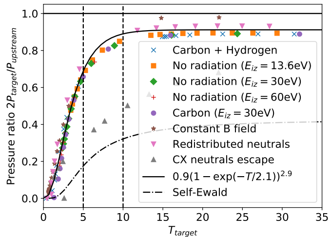
Figure 4. Ratio of target to upstream pressure, as a function of target temperature T_{target} . The almost universality of the curve indicates that this measure of pressure loss is mainly a function of T_{target} , in agreement with results from experiment and modelling [16]. All scans have a total flux expansion factor of 2 from upstream to target except “Constant B field” which has no flux expansion; all have neutrals recycling at the target except “Redistributed neutrals” in which 50% of recycled neutrals are distributed evenly along the divertor; all have charge exchange (CX) reactions which conserve momentum between plasma and neutral fluids, except “CX neutrals escape” in which fast neutrals are assumed to leave the plasma, lose their momentum, and return at a random point along the divertor.
