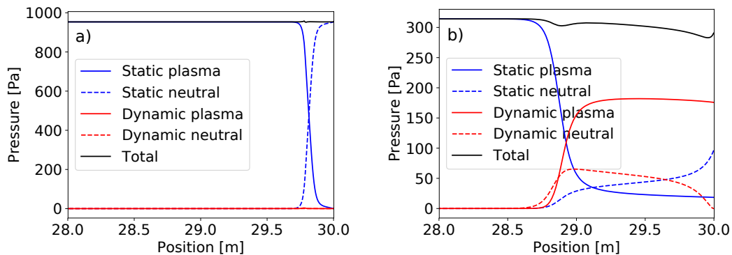
Figure 9. Parallel pressure balance a) with charge exchange at n_{up} = 5 \times 10^{19} \text{m}^{-3} and b) without charge exchange at n_{up} = 1.7 \times 10^{19} \text{m}^{-3} .
