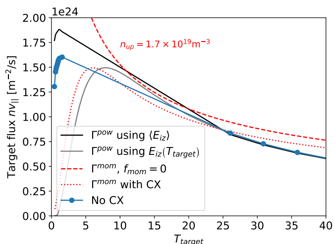
Figure 10. SD1D results for a case with no charge exchange (blue circles, labelled “No CX”); Target particle flux calculated from power balance (eq 4) using E_{iz} at the target temperature (gray solid line), and power balance using the average E_{iz} over the simulation (black solid line). Dashed red lines show flux from momentum balance (eq 9) assuming no momentum loss. At low upstream densities the momentum balance curve (dashed red) and power balance curve (gray solid) intersect the SD1D results. At upstream densities above n_{up} \sim 1.7 \times 10^{-3}\text{m}^{-3} the momentum balance curve does not intersect the power balance curve, and a transition is seen. For comparison the momentum balance curve for the case with charge exchange is shown as a dotted red line. At n_{up} \sim 1.7 \times 10^{-3}\text{m}^{-3} the dotted line does intersect the power balance curve and so no transition is seen until higher upstream density when charge exchange is included.
