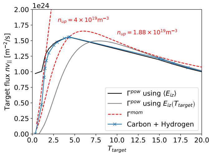
Figure 7. Target particle flux as a function of target temperature for the density scan with varying E_{iz} (hydrogen excitation radiation) and 1% carbon impurity. The gray solid curve shows \Gamma^{pow} calculated using equation 4 with fixed P_{recl} and the value of E_{iz} at T_{target} . The black solid curve shows \Gamma^{pow} calculated using the volume averaged \langle E_{iz} \rangle shown in figure 6. Red dashed curves (again self-similar shape as n_{up} is varied) show \Gamma^{mom} calculated using equation 9, with the fit for f_{mom} from figure 4 and equation 7.
