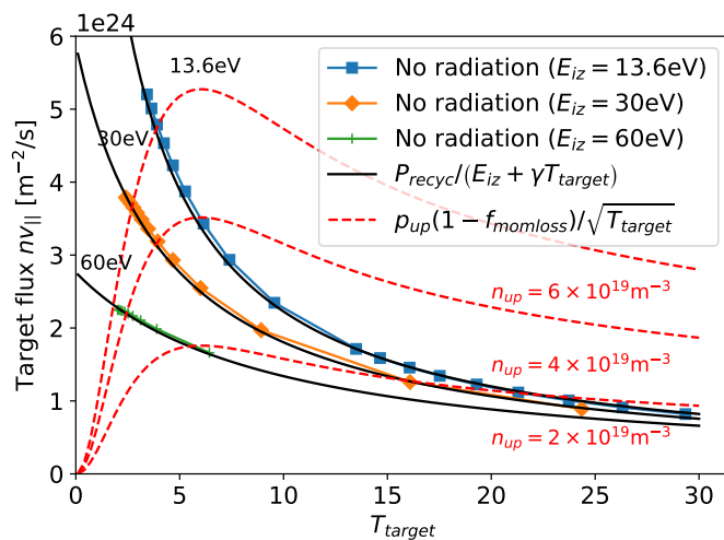
Figure 5. Target particle flux as a function of target temperature for three upstream density scans with fixed energy cost per ionisation E_{iz} and no impurity radiation, taking into account the 3.5\text{eV} with which neutral atoms are recycled. Black solid curves show \Gamma^{pow} calculated using equation 4 with fixed P_{in} for each value of E_{iz} . Red dashed curves show \Gamma^{mom} calculated using equation 9, with the fit for f_{mom} from figure 4 and equation 7. The intersection of these curves is the consistent solution for a given upstream density. Since the curves for \Gamma^{pow} are monotonic, no flux rollover is seen in these scans.
