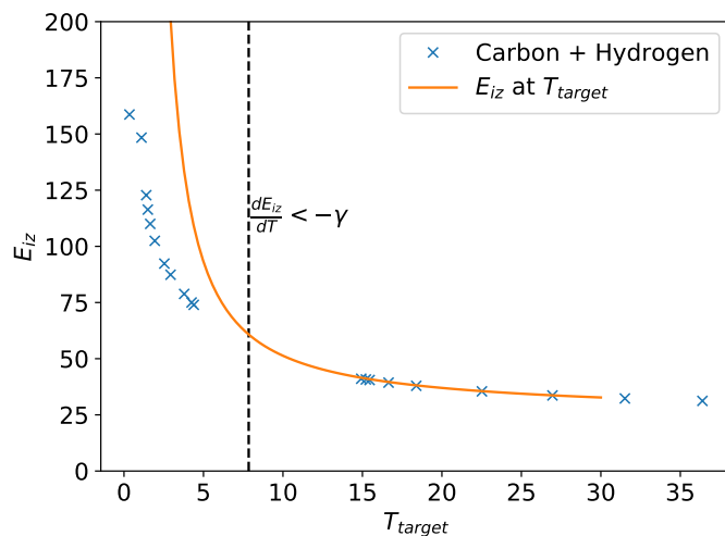
Figure 6. Effective E_{iz} for the ‘‘Carbon + Hydrogen’’ case (Blue crosses), calculated as the ratio of the total power lost to hydrogen ionisation and excitation, divided by the rate of ionisations, and averaged over the domain. The value of E_{iz} from the rate coefficients used in SD1D at the target temperature T_{target} are shown for comparison (red line). The threshold in equation 11 is marked by a vertical dashed line.
