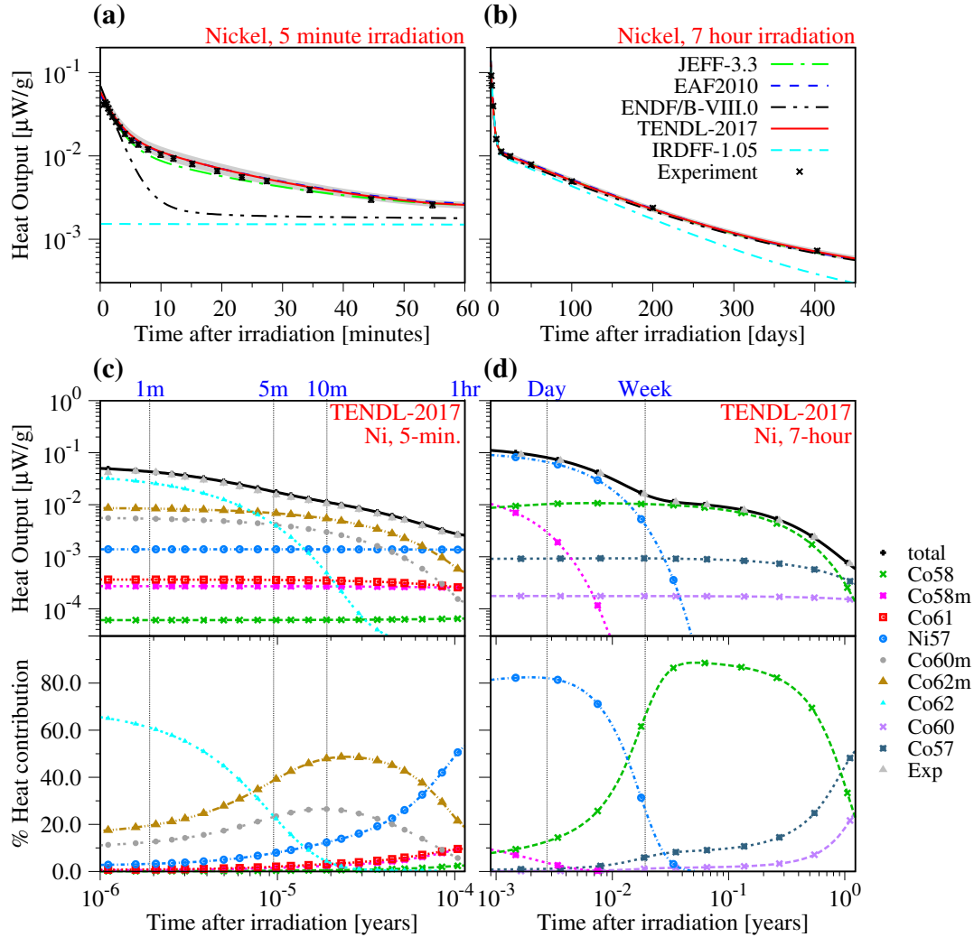
Figure 2: (colour online). Simulated decay-heat experiment for nickel in the FNS benchmark. (a) and (c) correspond to decay-heat following 5-minute irradiations, (b) and (d) are the equivalent data after 7-hour irradiations. (a) and (b) show total decay-heat curves on linear time-after-irradiation scales for the different nuclear library simulations with FISPACT-II, the experimental measurements as points with vertical lines showing experimental uncertainty, and the nuclear-data-uncertainty band (in grey) for the TENDL-2017 [30] library. (c) and (d) present the radionuclide breakdown of contributions to the total decay heat from the TENDL-2017 simulations in absolute \mu\text{W/g} terms (top halves) and as % contributions (bottom halves) – on logarithmic time-after-irradiation scales. See main text for more details.
