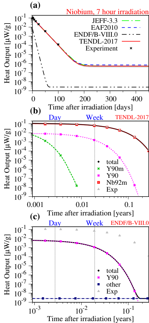
Figure 4: (colour online) Simulated decay-heat experiment for a 7-hour irradiation of niobium in the FNS benchmark. (a) shows total decay-heat curves on a linear time-after-irradiation scale for inventory simulations with different nuclear libraries, as well as the experimental measurements as points with vertical lines showing experimental uncertainty, and the nuclear-data-uncertainty band (in grey) for the TENDL-2017 [30] library. (b) presents the radionuclide breakdown of contributions to the total decay heat from the TENDL-2017 simulation in absolute \mu\text{W/g} terms on a logarithmic time-after-irradiation scale. (c) shows the equivalent profiles for the simulation with ENDF/B-VIII.0 [31].
