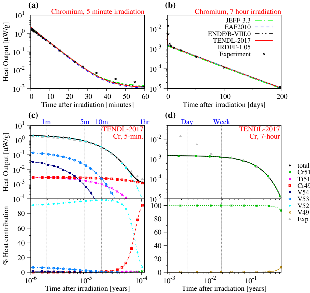
Figure 8: (colour online). Simulated decay-heat experiment for chromium in the FNS benchmark. (a) and (c) correspond to decay-heat following 5-minute irradiations, (b) and (d) are the equivalent data after 7-hour irradiations. (a) and (b) show total decay-heat curves on linear time-after-irradiation scales for the different nuclear library simulations with FISPACT-II and the experimental measurements as points. Note that the experimental errors and TENDL-2017 uncertainties are plotted (as elsewhere in this paper), but are comparatively small in this case and barely visible on the plotting scales used. (c) and (d) present the radionuclide breakdown of contributions to the total decay heat from the TENDL-2017 simulations in absolute \mu\text{W/g} terms (top halves) and as % contributions (bottom halves) – on logarithmic time-after-irradiation scales. Note that the IRDFF-1.05 was not considered in simulations of the cooling after the 5-minute irradiation. See main text for more details.
