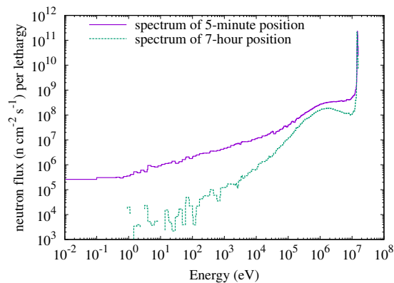
Figure 1: (colour online). Simulated neutron spectra experienced by the two experimental batches performed at JAEA’s FNS facility and discussed in this paper. Flux values are scaled (divided) by lethargy to remove weighting bias caused by the varying energy-bin widths. Lethargy is the natural log of the ratio of an energy bin’s upper and lower bounds.
