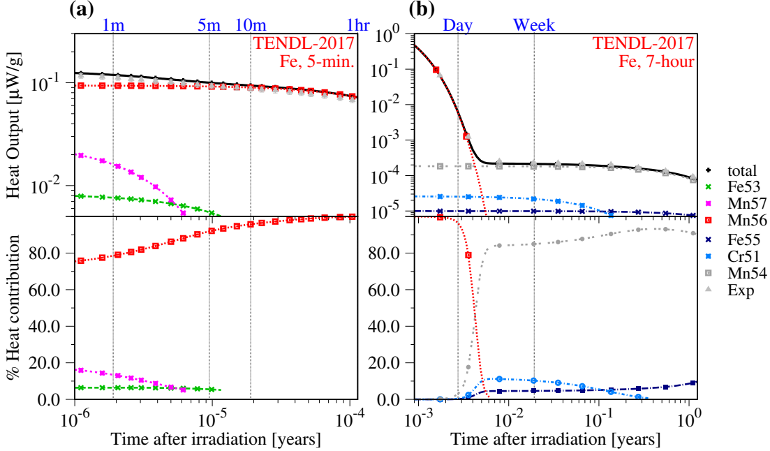
Figure 3: (colour online) Radionuclide breakdown of contributions to the total decay-heat from the TENDL-2017 simulations of pure iron after (a) 5-minute and (b) 7-hour irradiations. Absolute \mu\text{W/g} curves are shown in the top halves of both plots, with % contribution-curves shown in the lower halves. The FNS benchmark experimental decay-heat measurements are also shown in the upper plots. All times are given as time-after-irradiation in years on a logarithmic scale.
