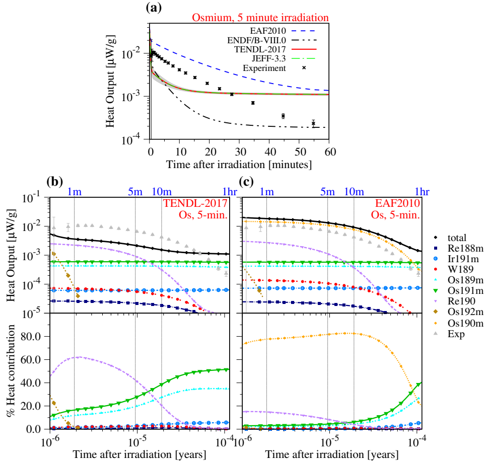
Figure 9: (colour online) Simulated decay-heat experiment for a 5-minute irradiation of osmium in the FNS benchmark. (a) shows total decay-heat curves on a linear time-after-irradiation scale for inventory simulations with different nuclear libraries, as well as the experimental measurements as points. Vertical error lines show the experimental uncertainty and a grey band indicates the TENDL-2017 nuclear-data uncertainty. (b) presents the radionuclide breakdown of contributions to the total decay heat from the TENDL-2017 simulation in absolute \mu\text{W/g} terms (top half) and as % contributions (bottom half) – on logarithmic time-after-irradiation scale. (c) shows the equivalent absolute and % radionuclide profiles for a FISPACT-II simulation with EAF2010 [33].
