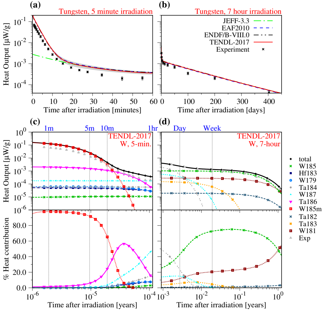
Figure 6: (colour online). Simulated decay-heat experiment for tungsten in the FNS benchmark. (a) and (c) correspond to decay-heat following 5-minute irradiations, (b) and (d) are the equivalent data after 7-hour irradiations. (a) and (b) show total decay-heat curves on linear time-after-irradiation scales for the different nuclear library simulations with FISPACT-II, the experimental measurements as points with vertical lines showing experimental uncertainty, and the nuclear-data-uncertainty band (in grey) for the TENDL-2017 [30] library. (c) and (d) present the radionuclide breakdown of contributions to the total decay heat from the TENDL-2017 simulations in absolute \mu\text{W/g} terms (top halves) and as % contributions (bottom halves) – on logarithmic time-after-irradiation scales. See main text for more details.
