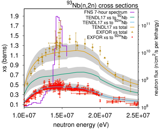
Figure 5: (colour online) TENDL-2017 and EXFOR-differential cross sections for (n,2n) on ^{93}\text{Nb} . Grey uncertainty bands shown for each cross section (xs) curve are based on covariance data in the TENDL-2017 library. The TENDL-2017 total is the sum of the channels to the different daughter isomeric states (and the uncertainty band in this case comes from the individual errors summed in quadrature). EXFOR [16] data is separated into differential points (a mixture of experimental, derived, and calculated values) identified as corresponding to the metastable ^{92m}\text{Nb} or total (no EXFOR data is directly attributed to the xs to the ground-state). Quoted uncertainties in energy and xs for each differential point are shown as horizontal and vertical error-bars. The neutron energy-flux spectrum for the 7-hour FNS irradiation is also shown (using the right hand y-axis flux scale).
