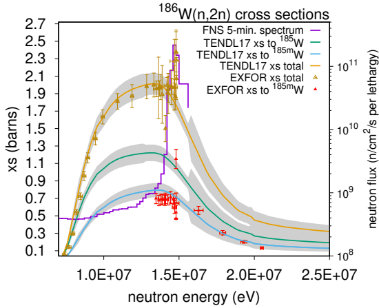
Figure 7: (colour online) TENDL-2017 and EXFOR-differential cross sections for (n,2n) on ^{186}\text{W} . Grey uncertainty bands shown for each cross section (xs) curve are based on covariance data in the TENDL-2017 library. The TENDL-2017 total is the sum of the channels to the different daughter isomeric states (and the uncertainty band in this case comes from the individual errors summed in quadrature). EXFOR [16] data is separated into differential points (a mixture of experimental, derived, and calculated values) identified as corresponding to production of the metastable ^{185m}\text{W} or to the total xs. Quoted uncertainties in neutron energy and xs for each differential point are shown as horizontal and vertical error-bars. The neutron energy-flux spectrum for the 5-minute FNS irradiation is also shown (using the right hand y-axis flux scale).
